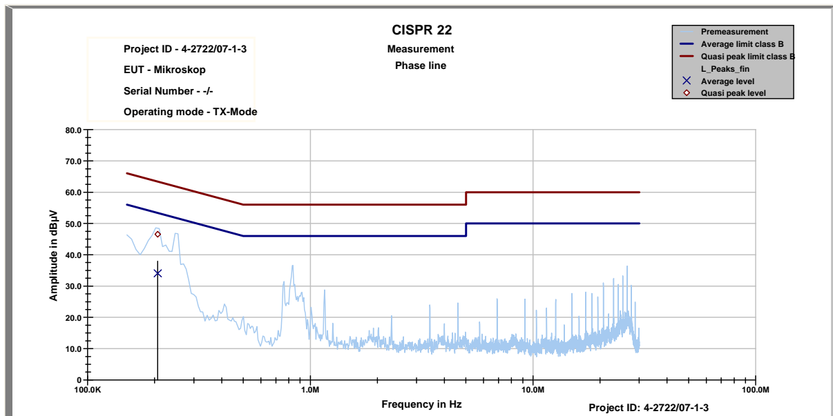
Plot 2: TX-Mode (Phase line)
