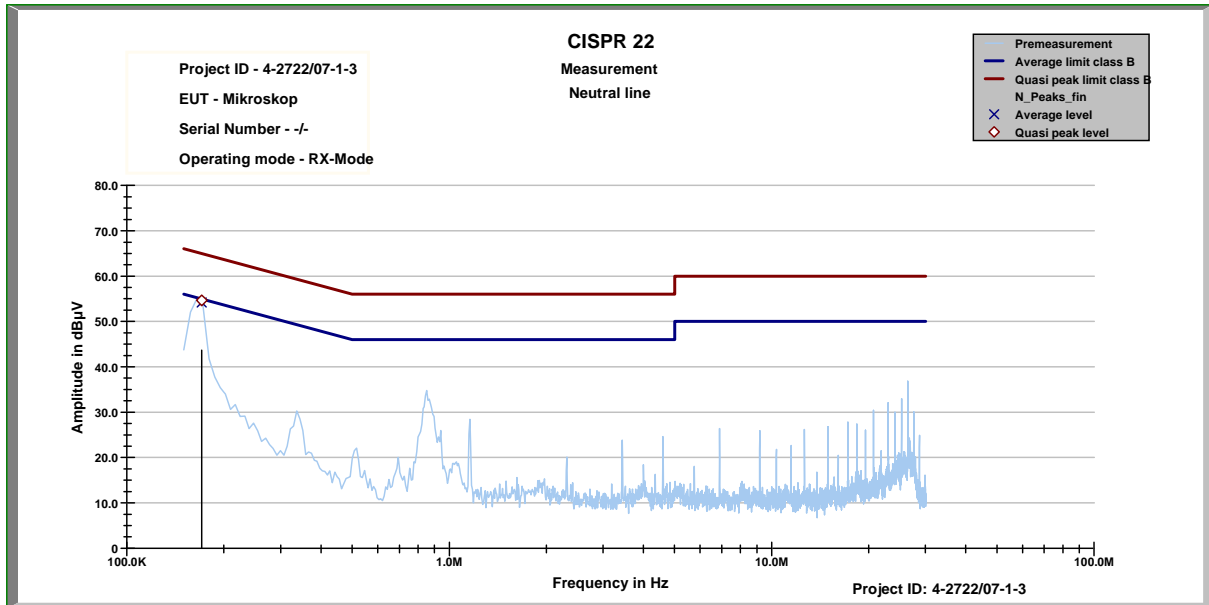
Plot 3: RX-Mode (Neutral line)
