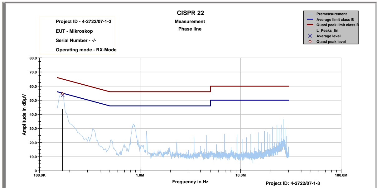
Plot 4: RX-Mode (Phase line)
