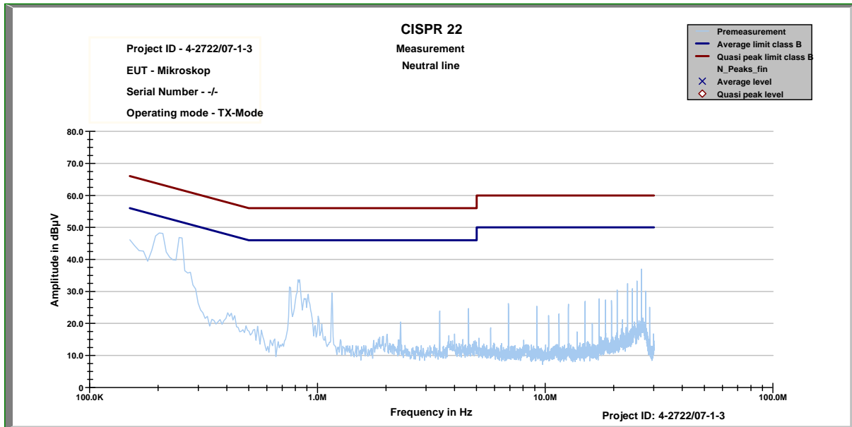
Plot 1: TX-Mode (Neutral line)
