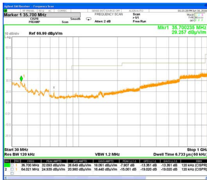
Plot # 27. Investigation result in 30 - 1000 MHz frequency range.
