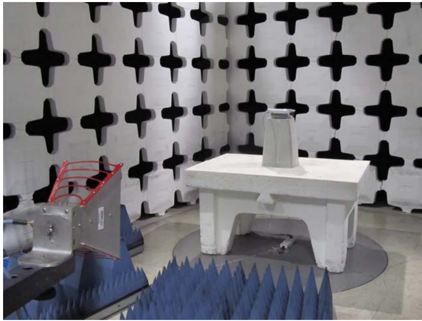
Photo 3. Radiated emissions test setup with Horn antenna in 1-18GHz.
