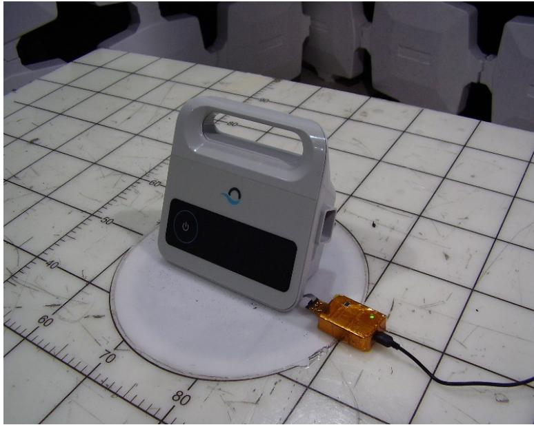
Photo 5. Radiated emissions test setup front view.
