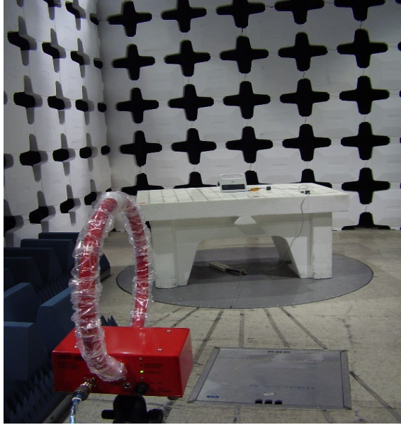
Photo 1.. Radiated emissions test setup with Loop antenna.
