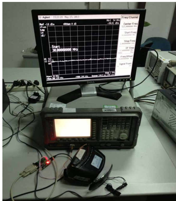
SPURIOUS EMISSION TEST SETUP
