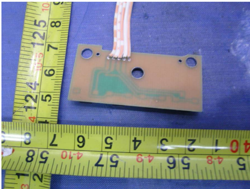
TX-PCB1 - Back View
