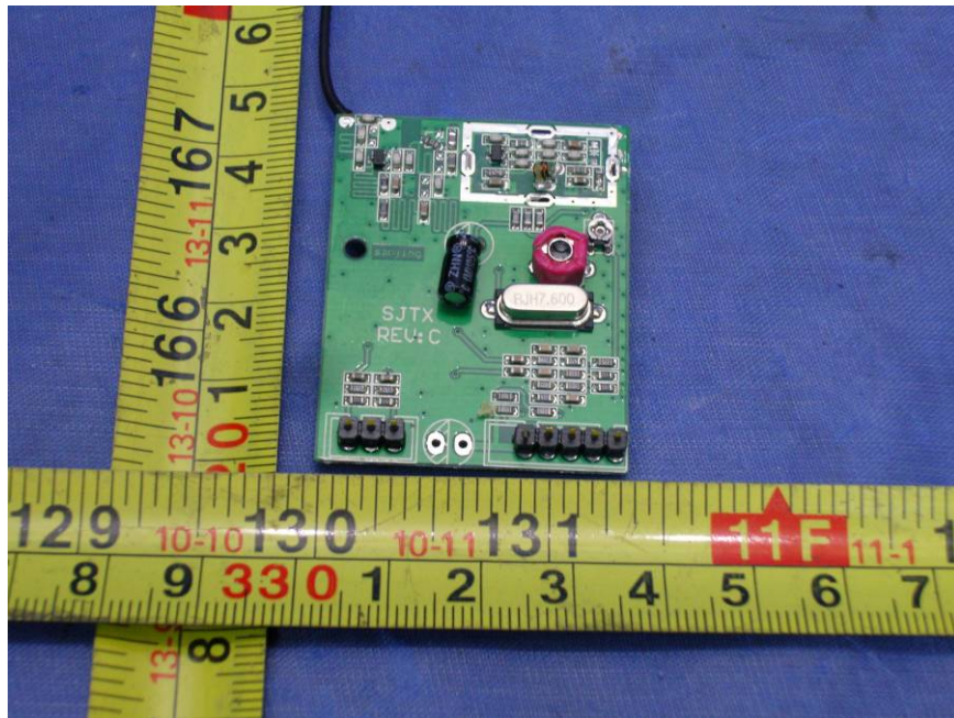
PCB2 of EUT- Front View
