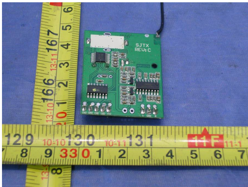
PCB2 of EUT- Back View
