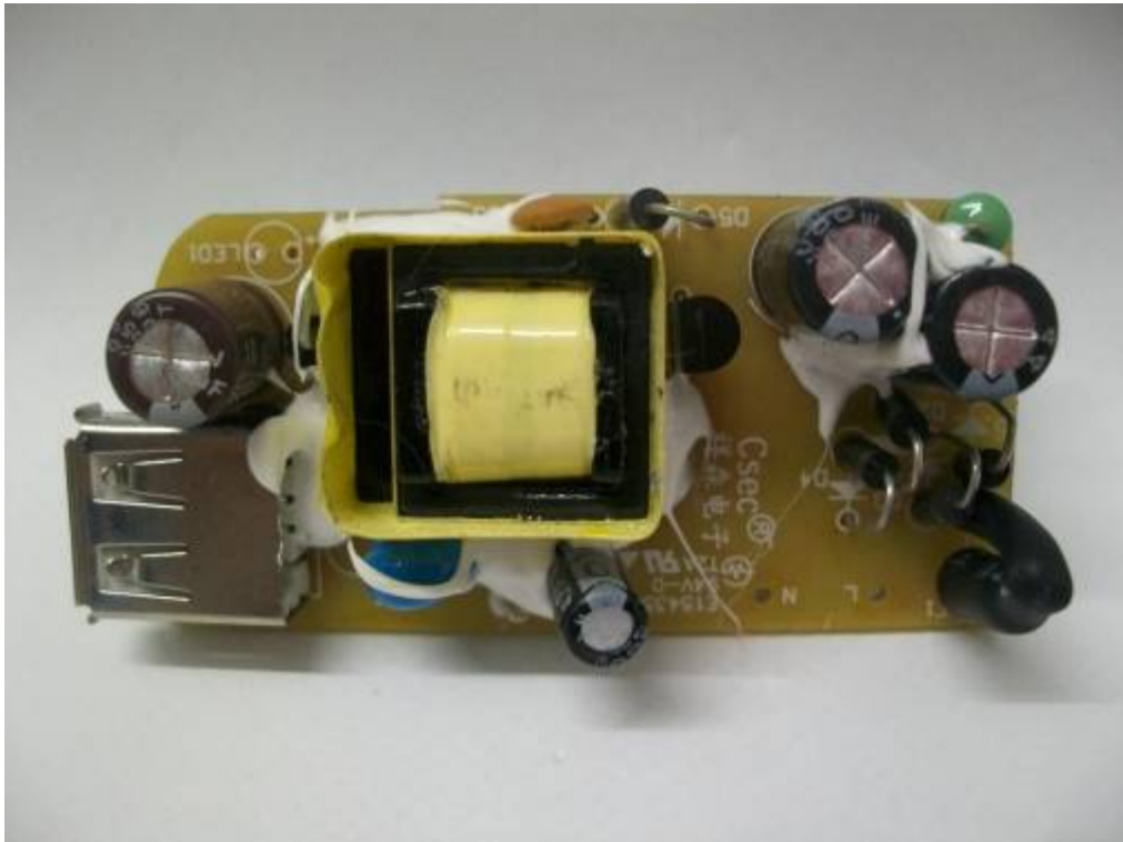
INTERNAL PHOTO OF POWER SUPPLY1 - 2
