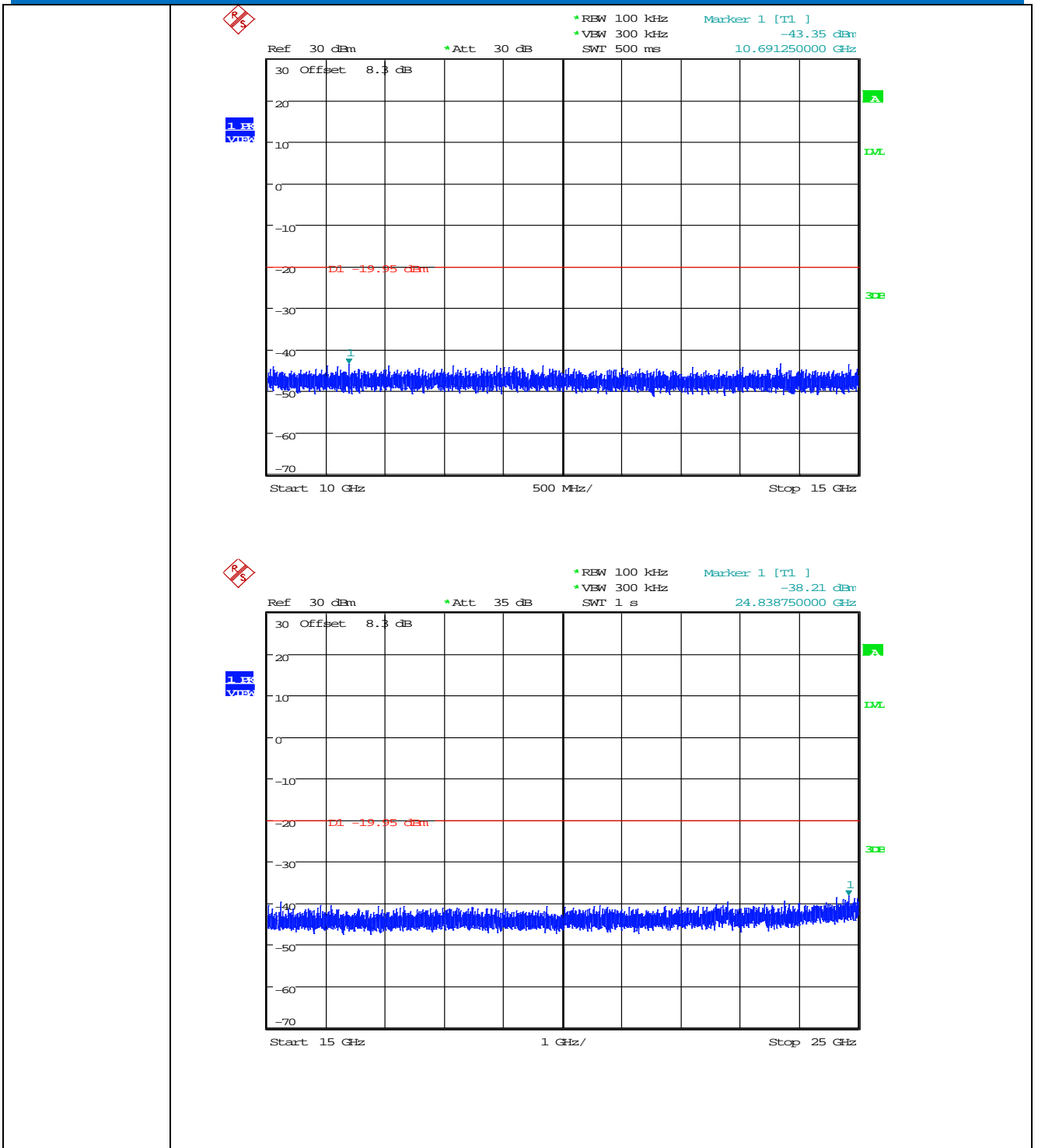
\pi/4 DQPSK_HCH_Graphs
