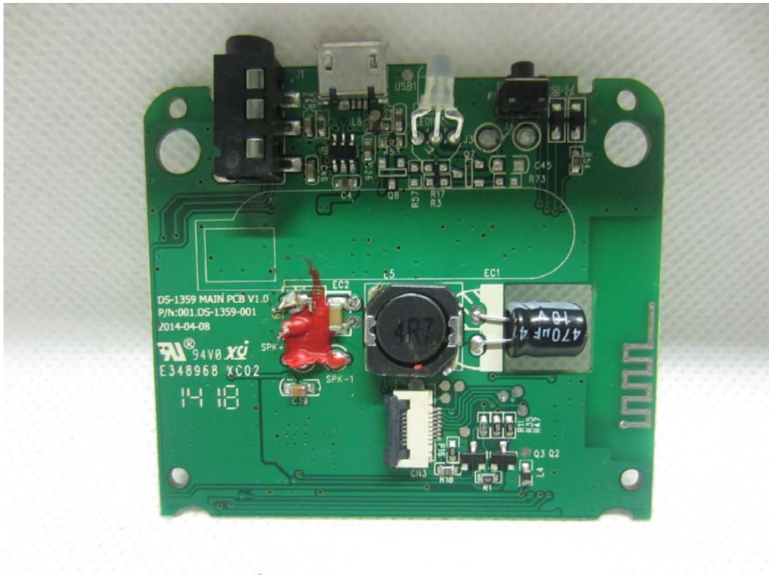
INTERNAL PHOTO OF SAMPLE- Speaker B - 6
