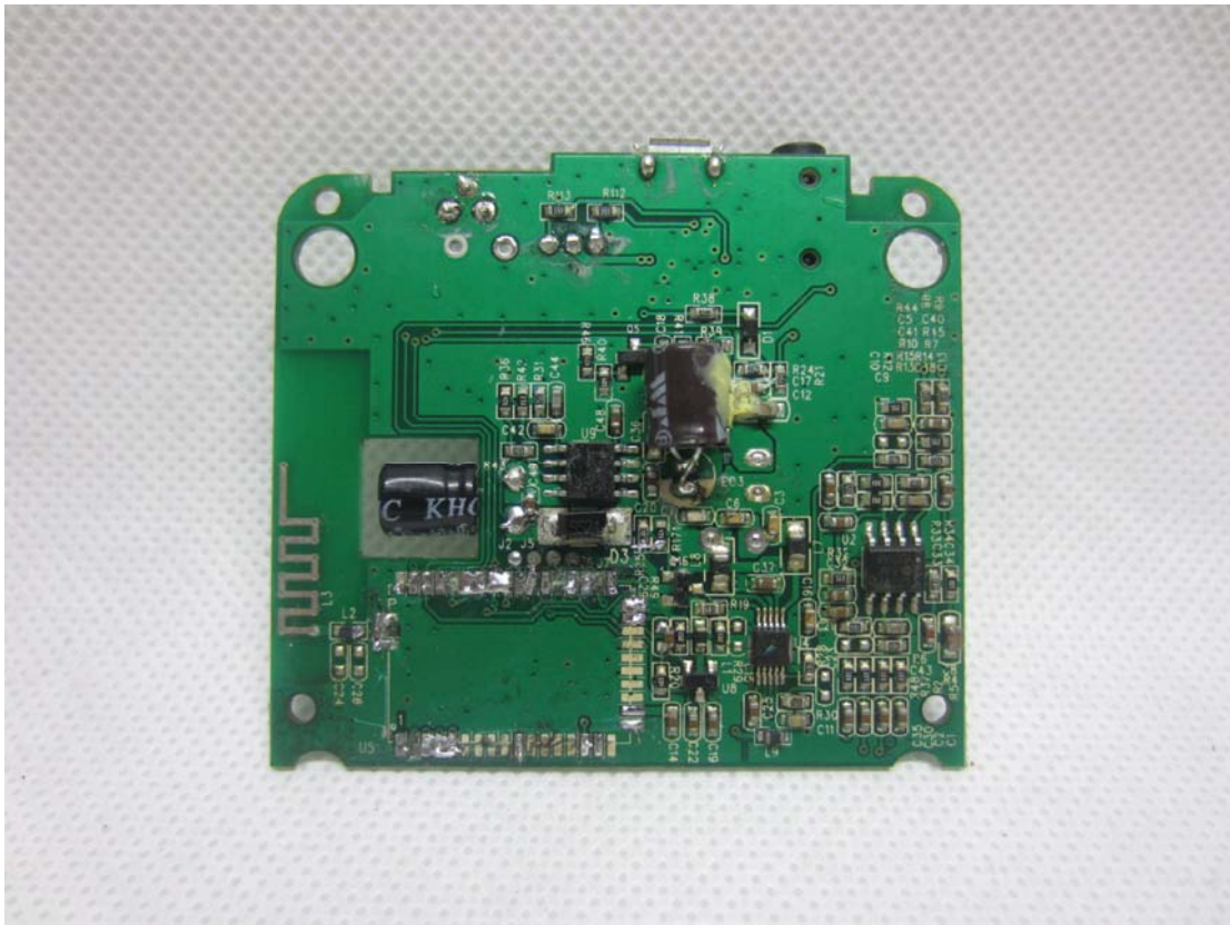
INTERNAL PHOTO OF SAMPLE - Speaker B - 7
