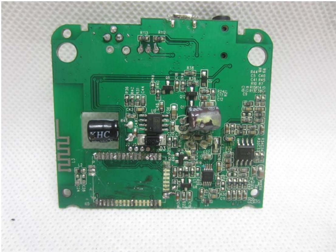
INTERNAL PHOTO OF SAMPLE - Speaker A - 7
