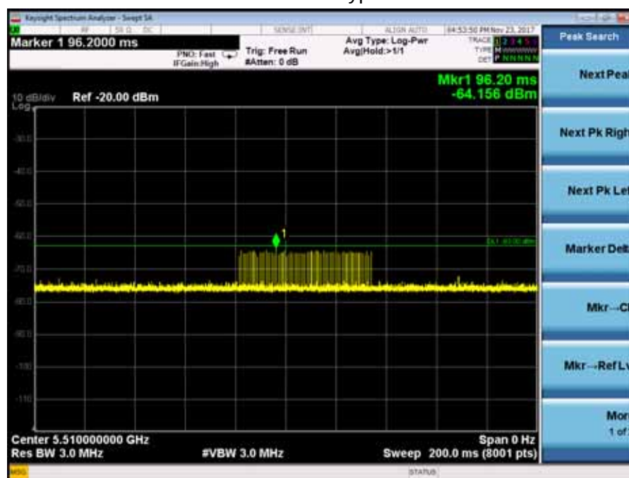
11ac40 CH102 5510MHz Radar Type 1A Calibration Plot
