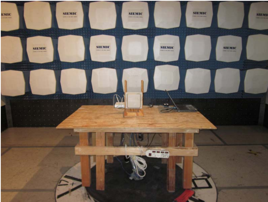
Radiated Emission Test Setup (Above 1GHz) - Front View
