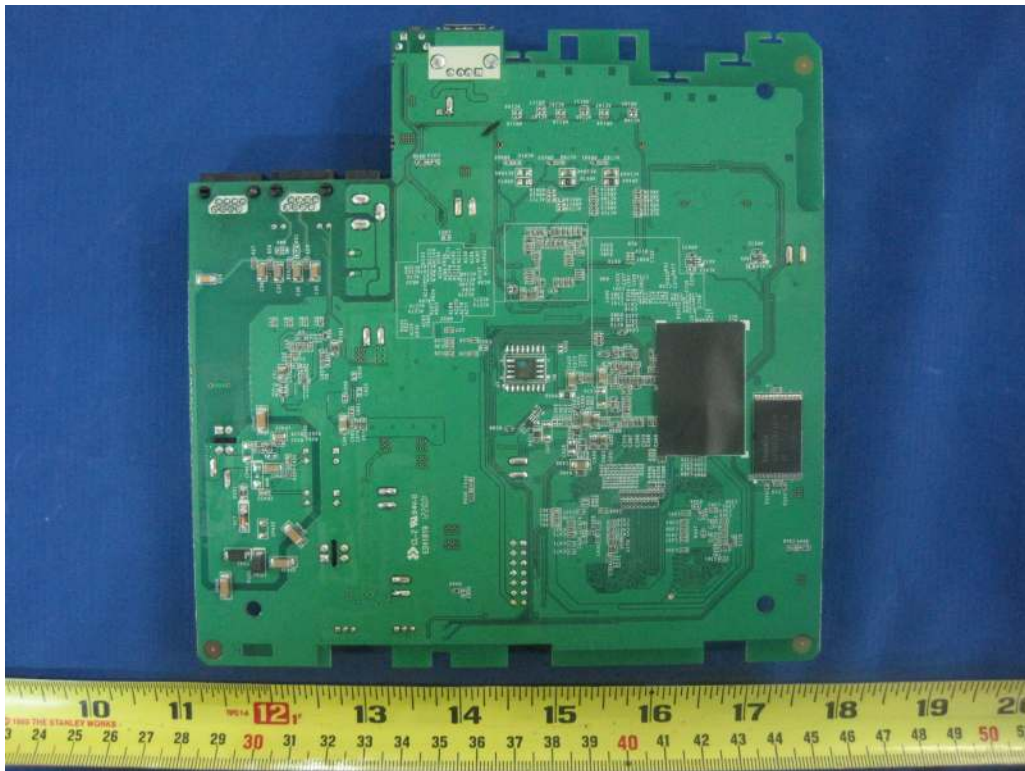
Radio Board with RF shield- Bottom View
