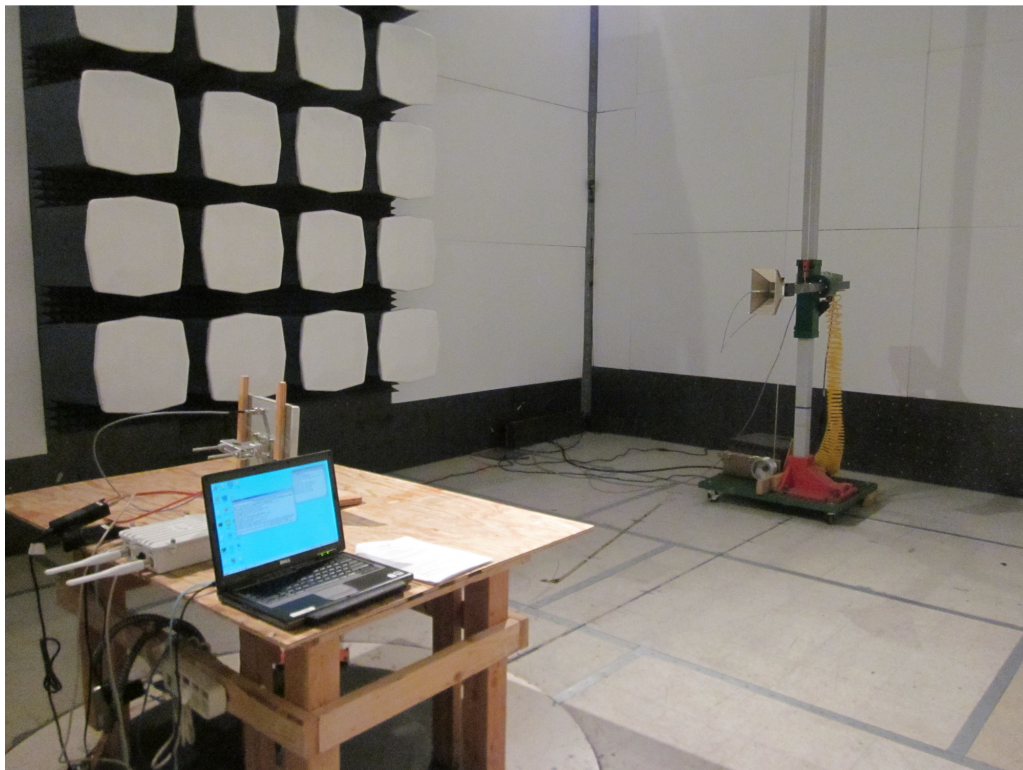
Radiated Emission Test Setup (above 1GHz) – Rear View
