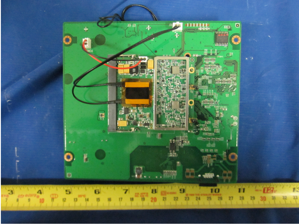
Radio Board without RF shield- Bottom View
