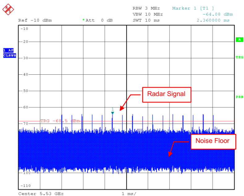
Radar Signal 2
