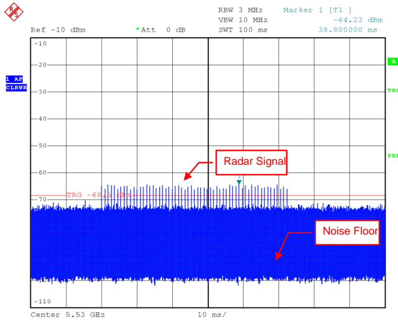
Radar Signal 1 (Test A)
