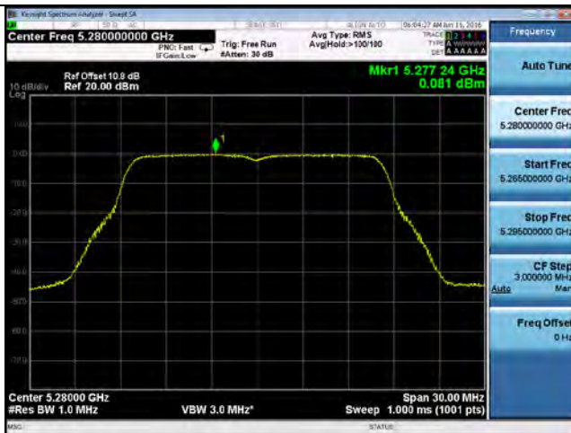
PSD-802.11a-5280M-chain2
