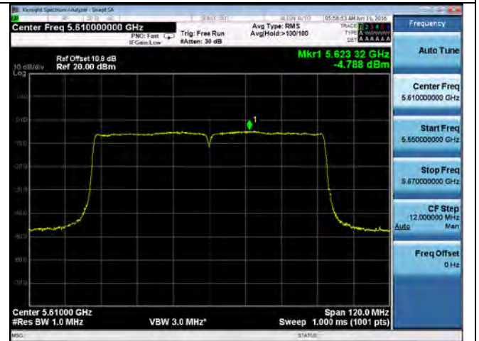
PSD-802.11ac-80-5610M-chain1
