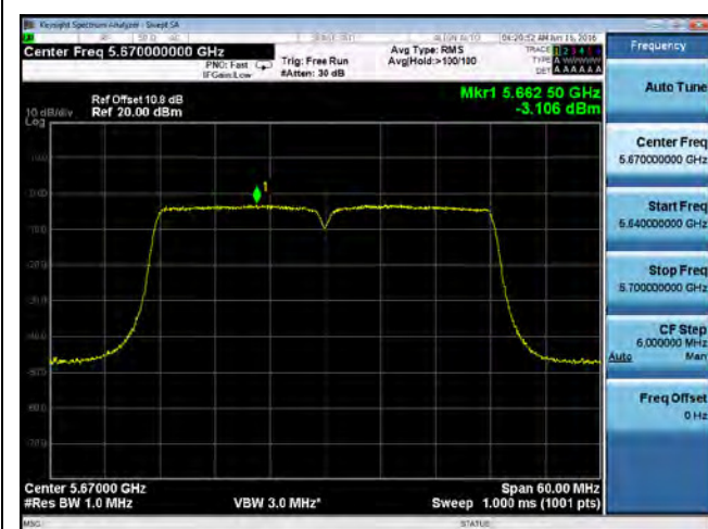
PSD-802.11n-40-5670M-chain2
