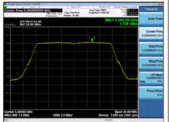
PSD-802.11n-20M -5260M-chain1
