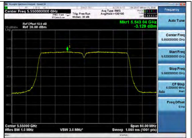
PSD-802.11n-40-5550M-chain2
