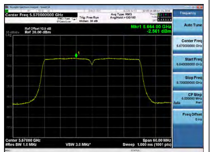
PSD-802.11n-40-5670M-chain3
