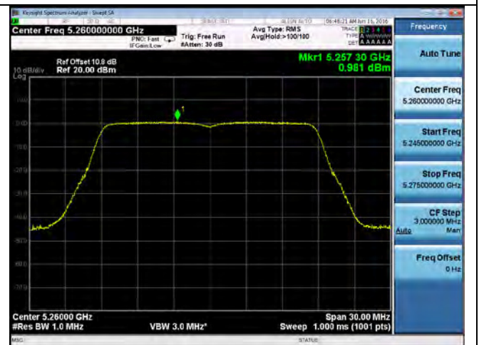
PSD-802.11n-20M -5260M-chain3
