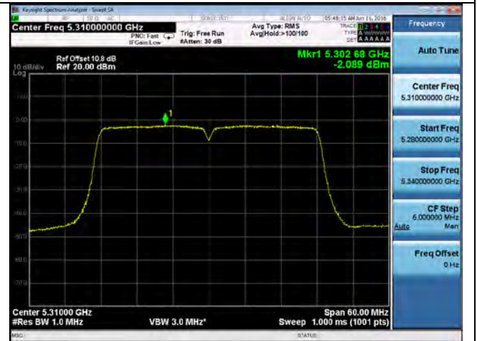
PSD-802.11n-40M-5310M-chain1
