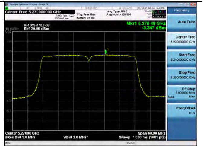
PSD-802.11n-40M-5270M-chain2
