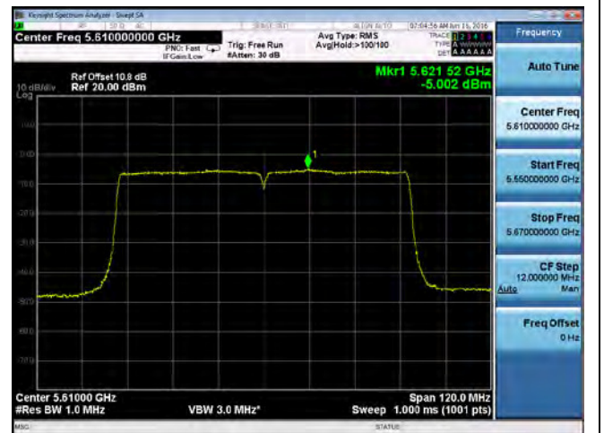
PSD-802.11ac-80-5610M-chain3
