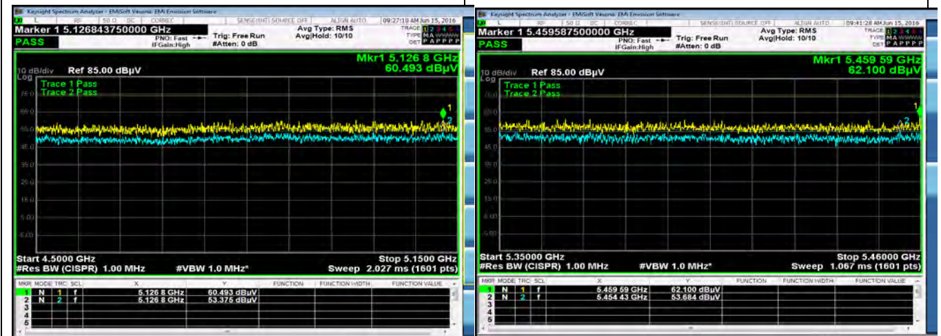
802.11n-HT40 5270M(4500-5150MHz)
