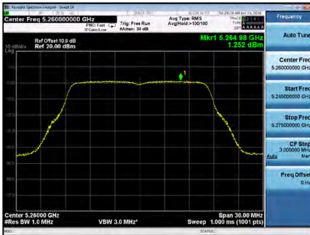
PSD-802.11a-5260M-chain3
