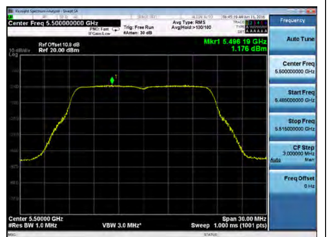
PSD-802.11a-5500M-chain3
