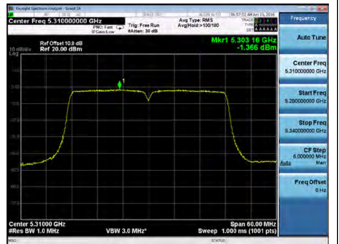
PSD-802.11n-40M-5310M-chain3
