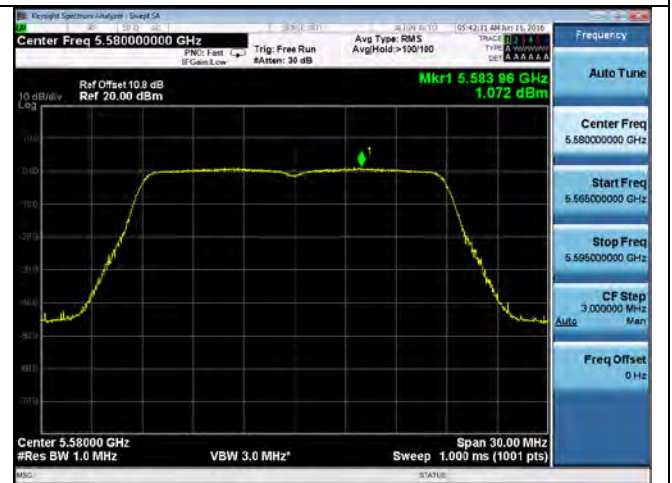
PSD-802.11n-20-5580M-chain1
