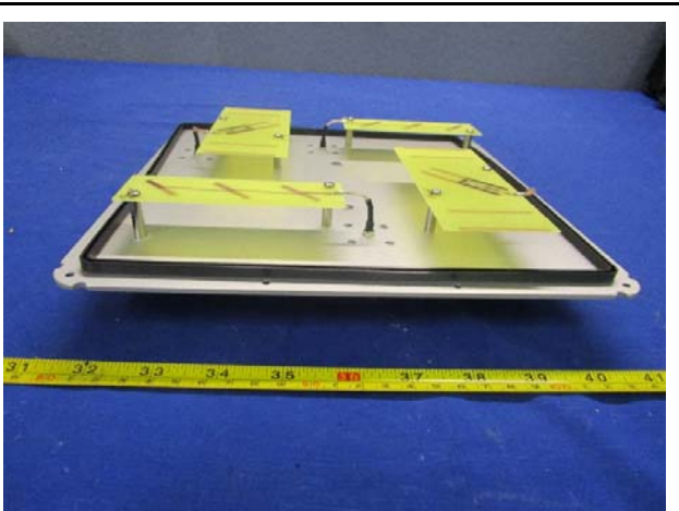
PCBA 1 Right Side View
