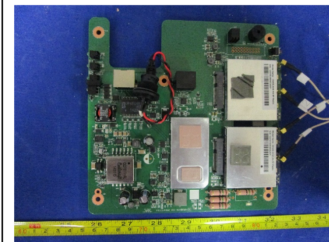
AP PCBA Top View
