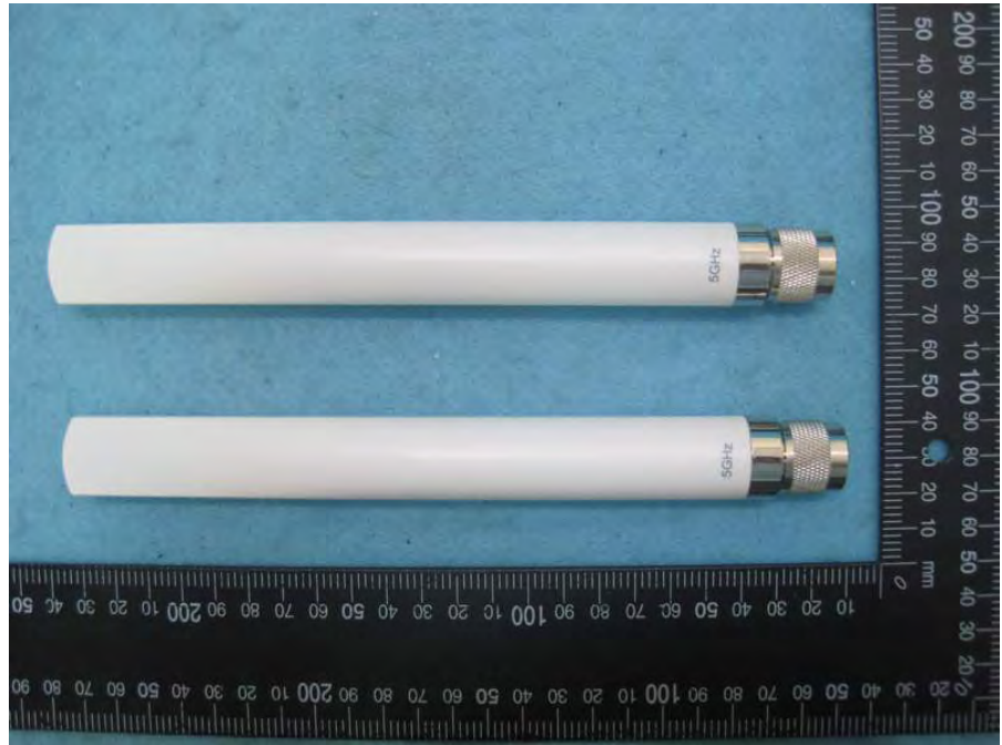
Dipole Antenna (5GHz)
