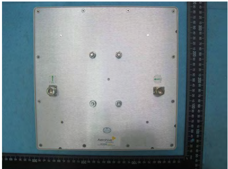
Panel Antenna (5GHz)
