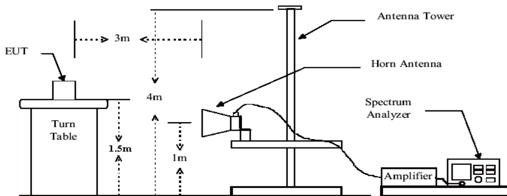
(F) Substituted Method Test Set-UP
