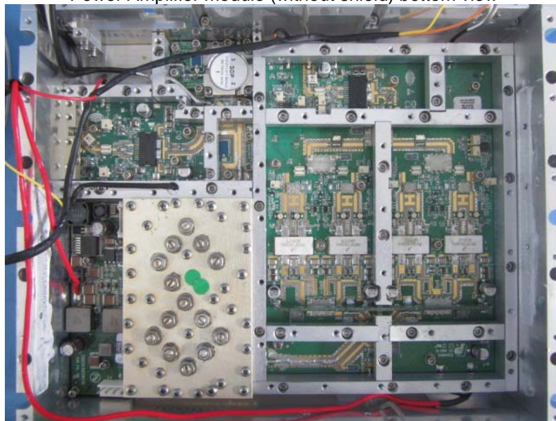
Power Amplifier module (without shield) bottom view
