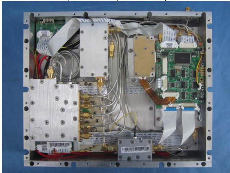
Power Amplifier module (without shield) front view
