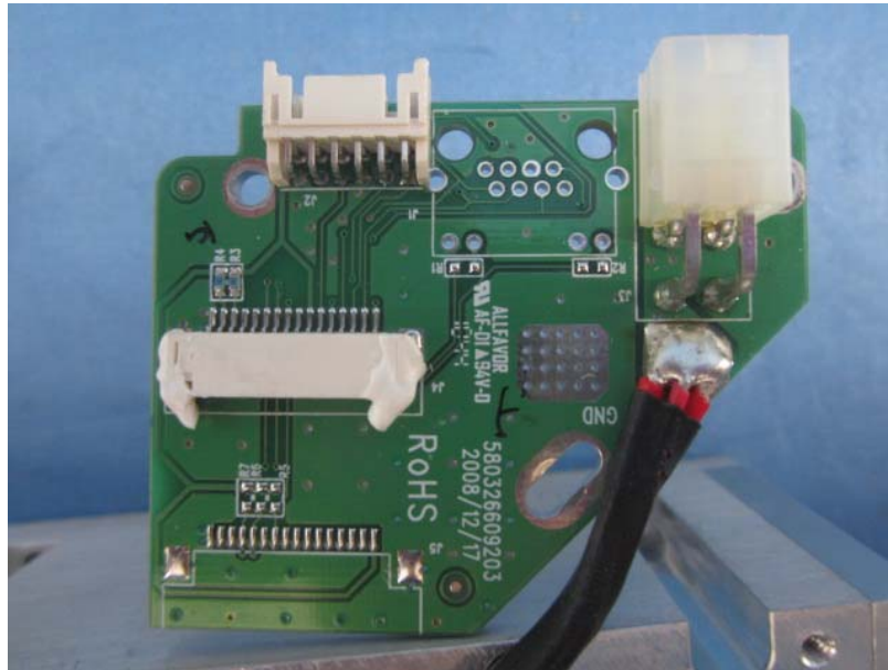
interface board front view
