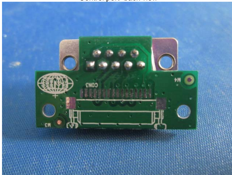
Control port back view
