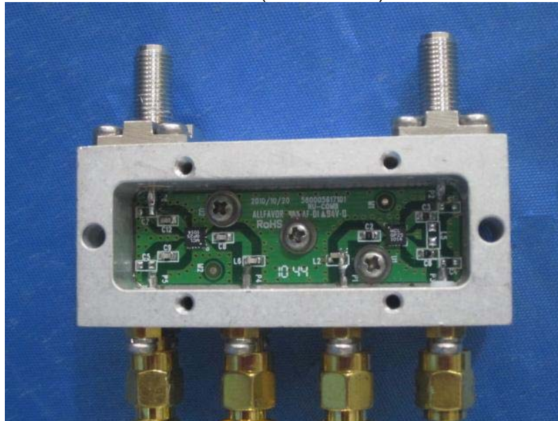
RU-COMB module (without shield) front view
