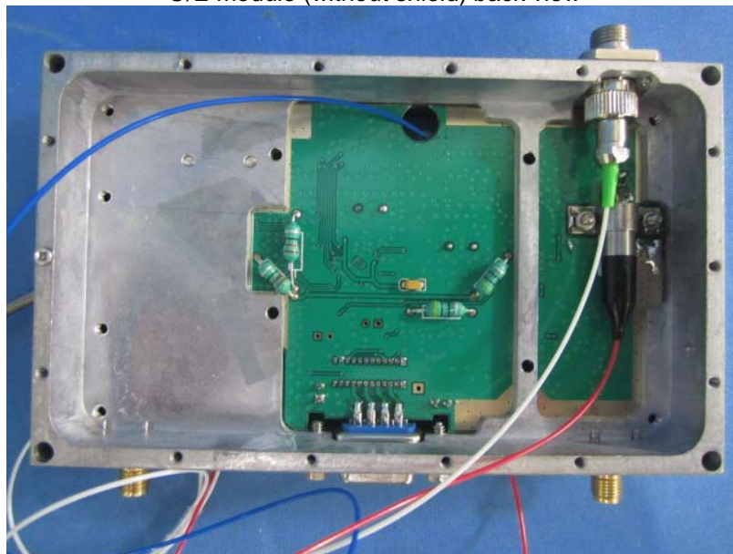
O/E module (without shield) back view
