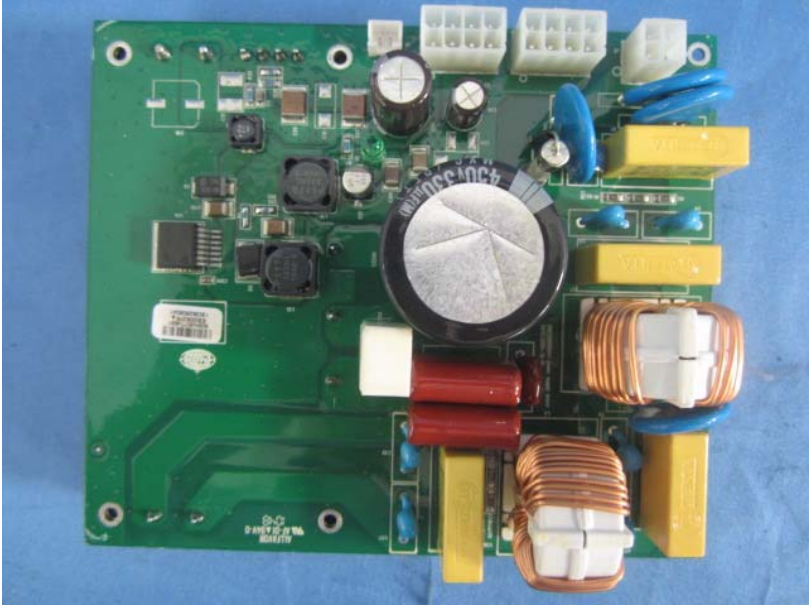
Power supply board (without shield) front view
