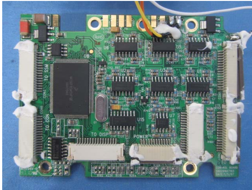
Main control board front view
