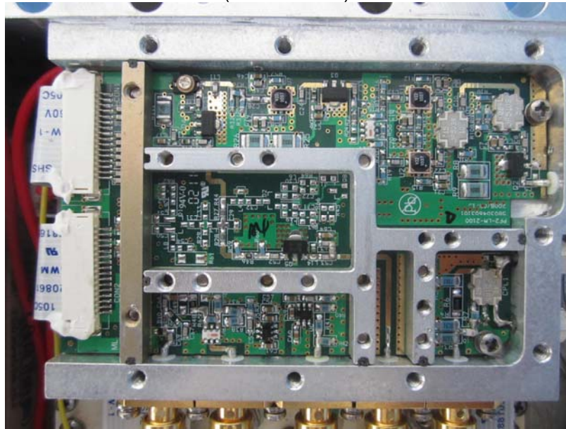
LMP view(without shield) front view
