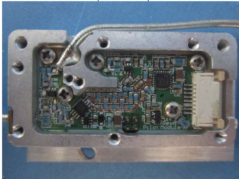
Pilot module (without shield) front view-1
