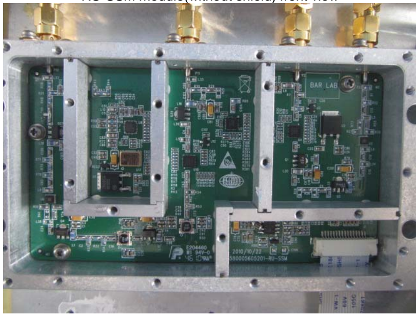
RU-SSM module(without shield) front view
