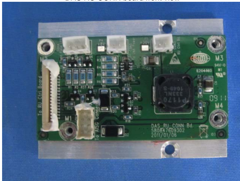
DAS RU CONN board front view
