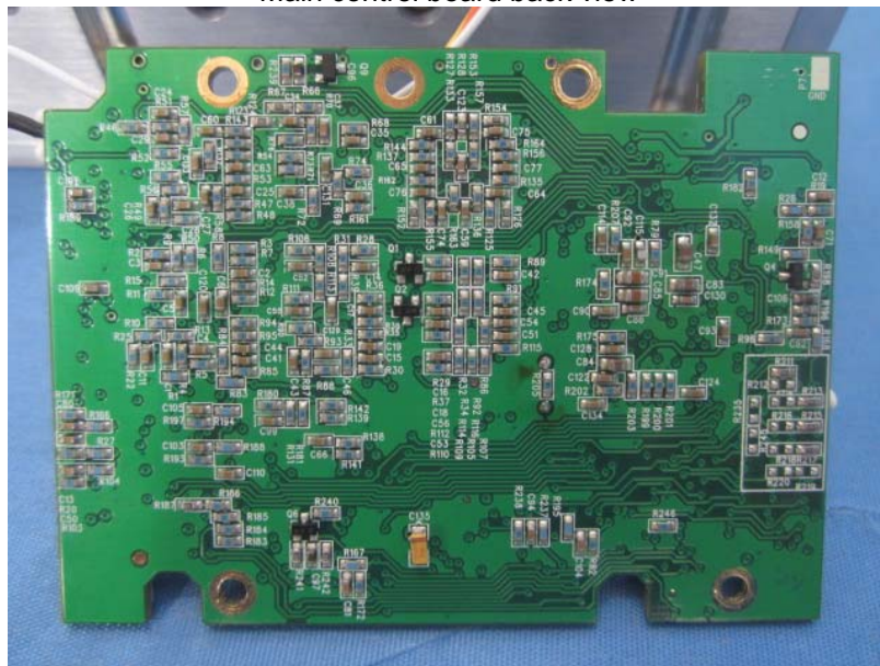
Main control board back view
