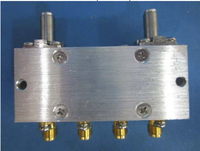
RU-COMB module (with shield) front view
