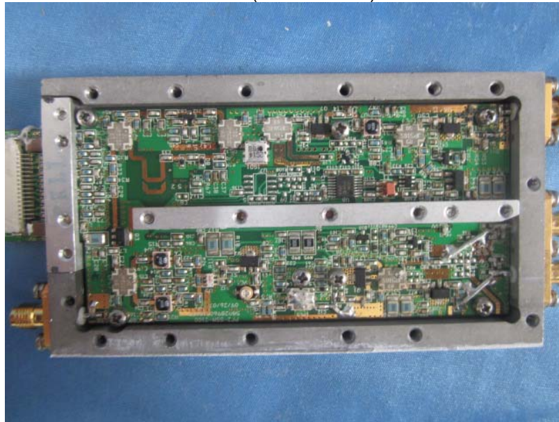
PA SSM module (without shield) front view
