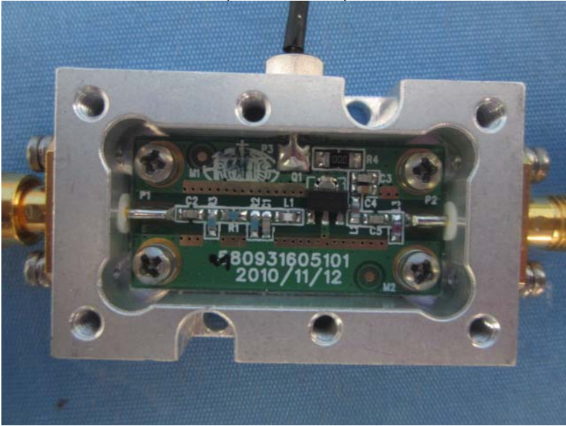
Pilot module (without shield) front view-2
