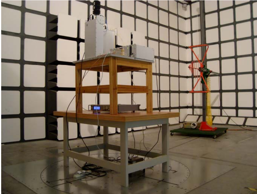
Below 1 GHz: Spurious Radiated Emissions - Front View (Downlink mode)
