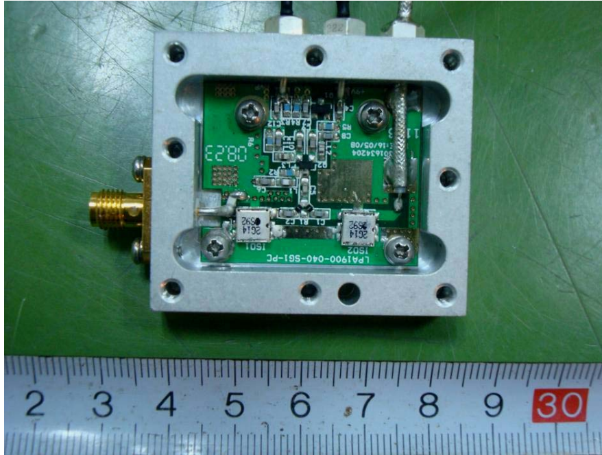
EUT – Pilot Module View
