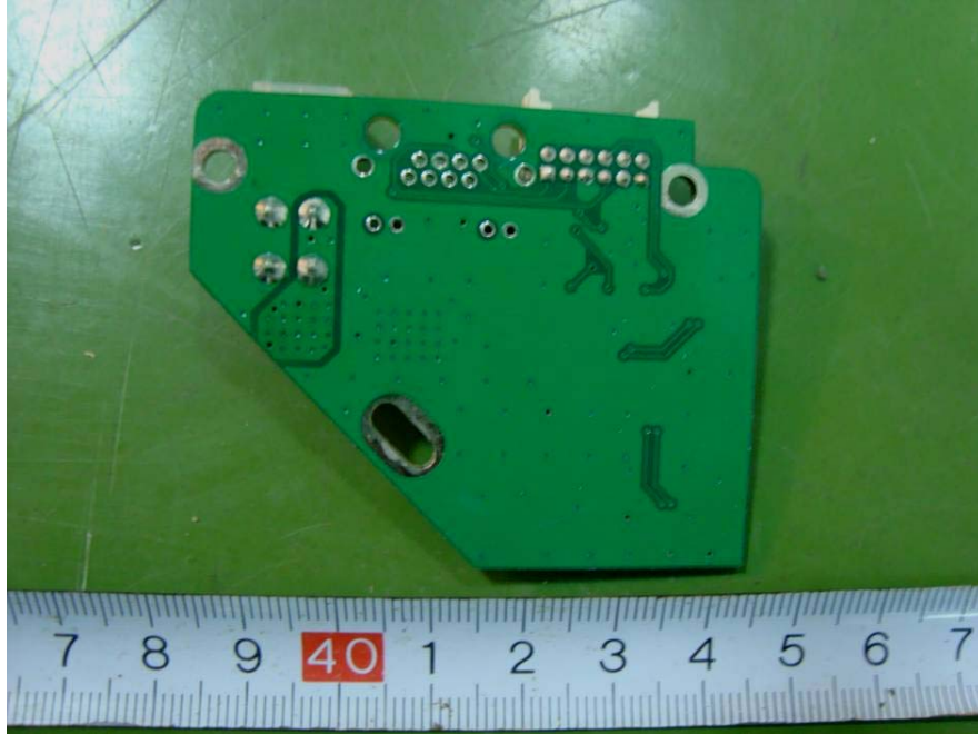
EUT – Linearization Module View
