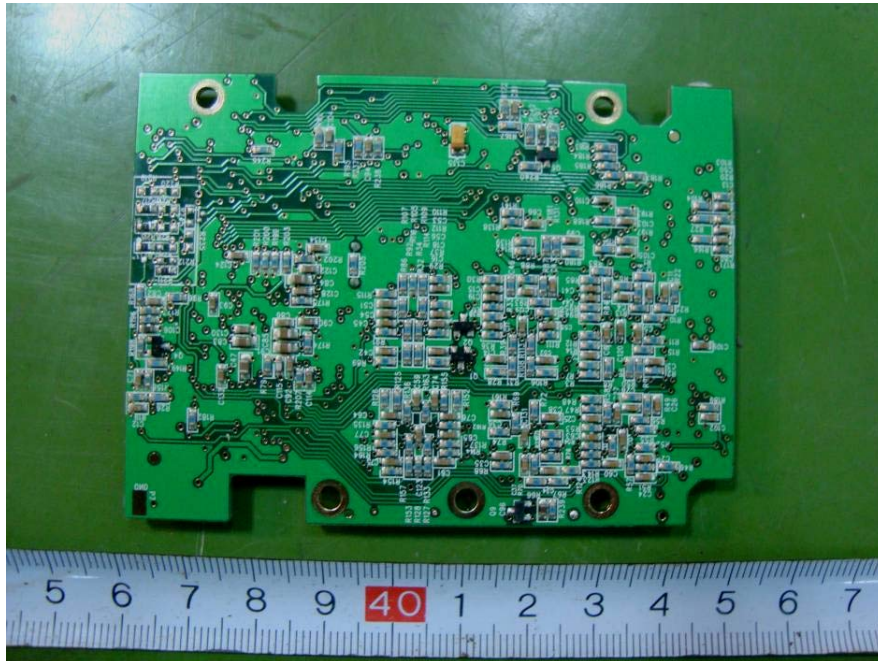
EUT – Phase Adjuster Module View
