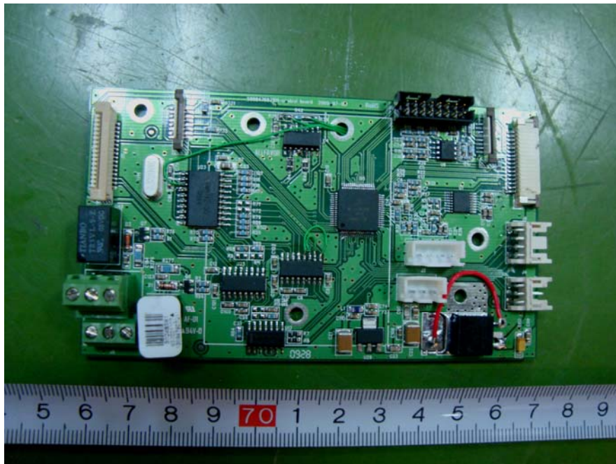
EUT – Host Unit Control Board Top View
