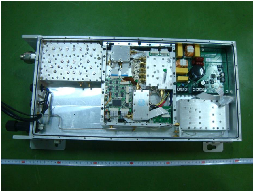
EUT –Without Cover View
