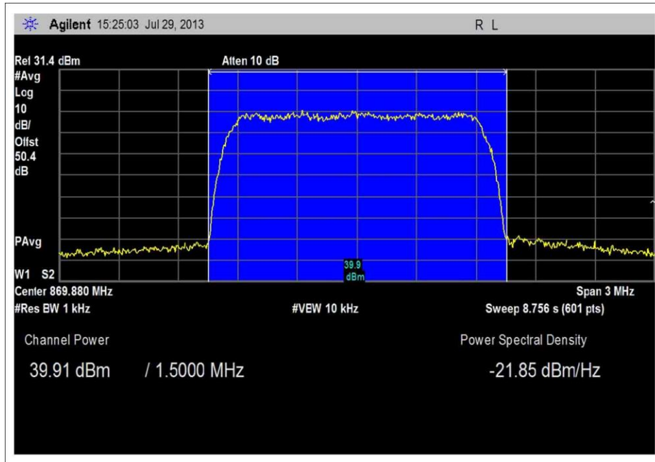
Band Power CDMA IS95A Low Channel 10W
