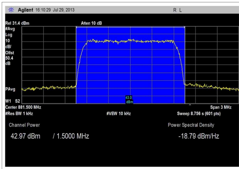
Band Power CDMA IS95A Middle Channel 20W
