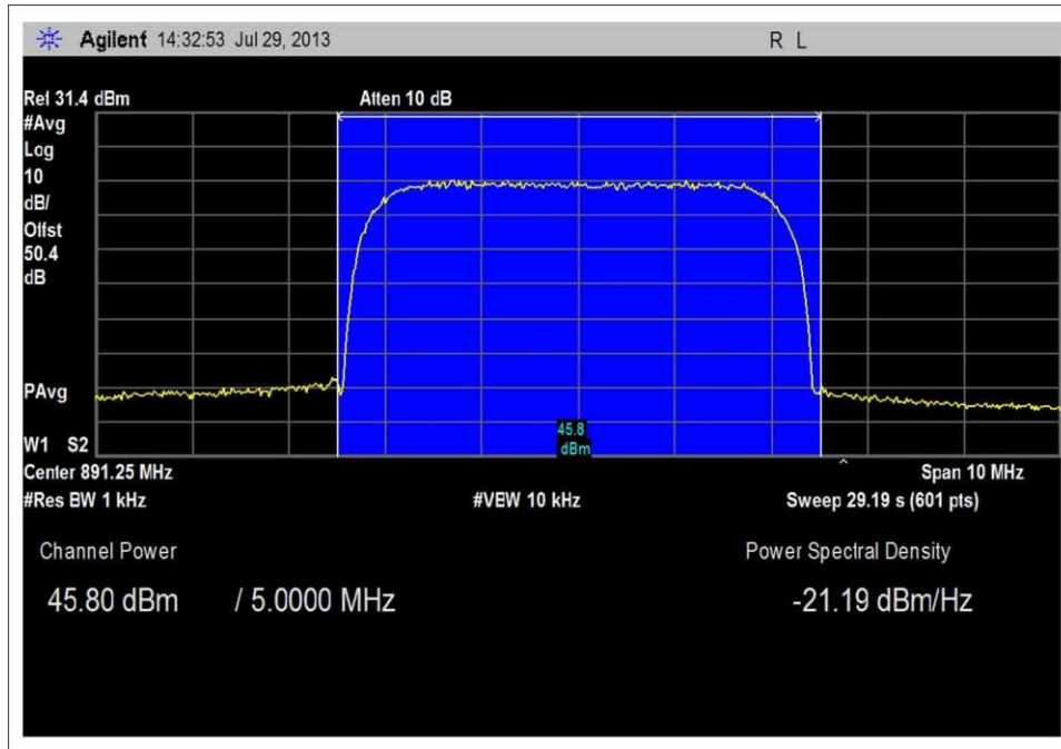
Band Power UMTS High Channel 40W
