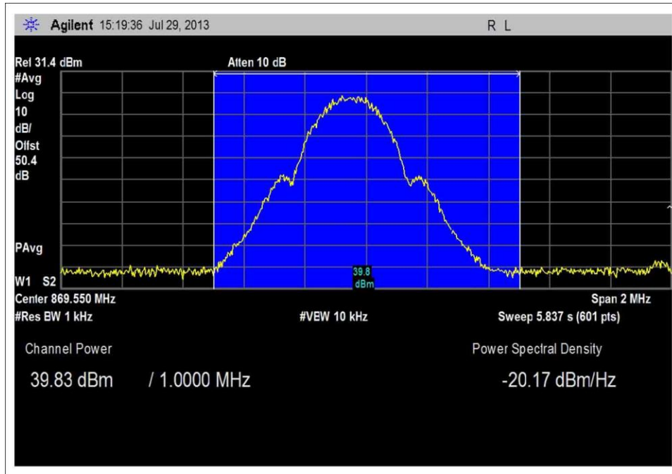
Band Power GSM Low Channel 10W
