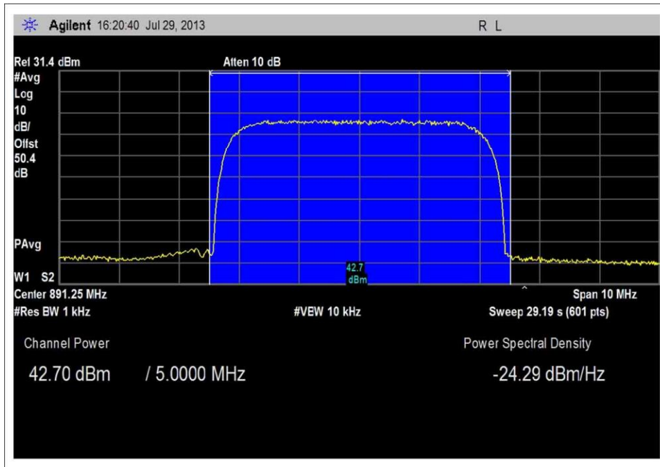
Band Power GSM High Channel 20W
