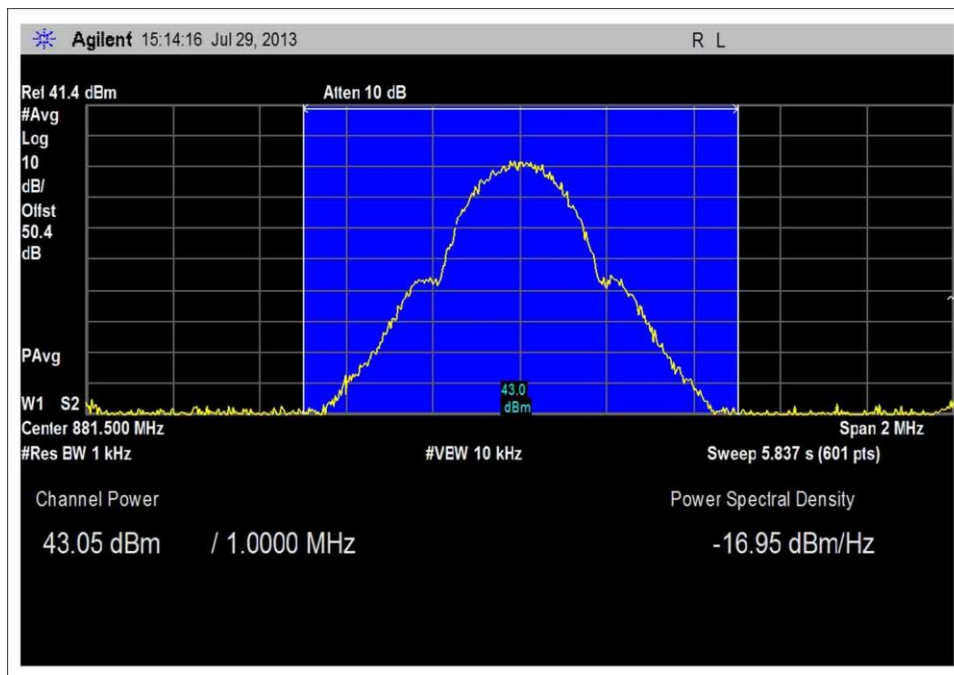
Band Power GSM Middle Channel 20W
