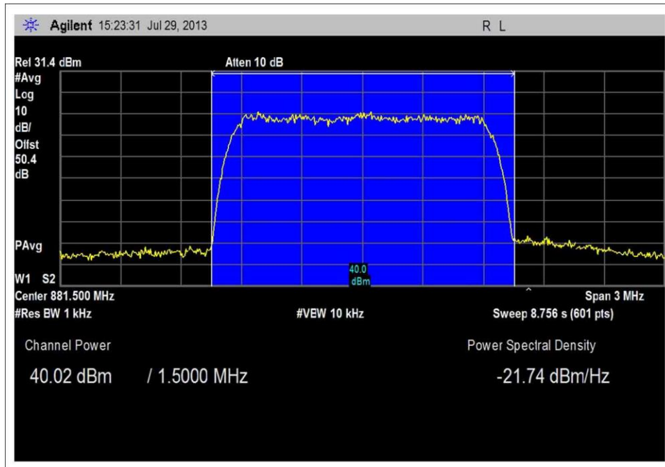
Band Power CDMA IS95A Middle Channel 10W
