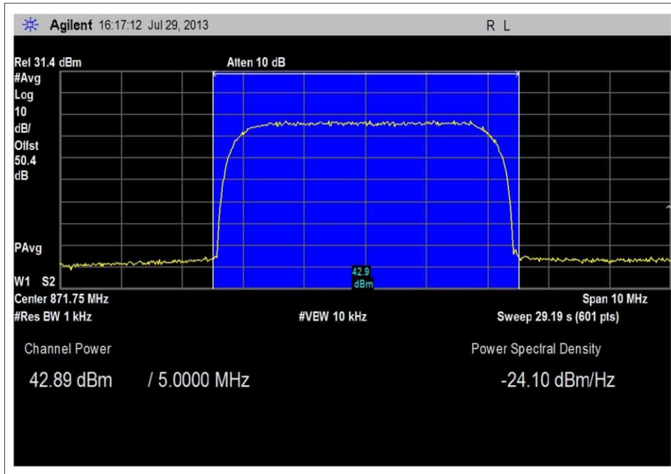
Band Power UMTS Low Channel 20W
