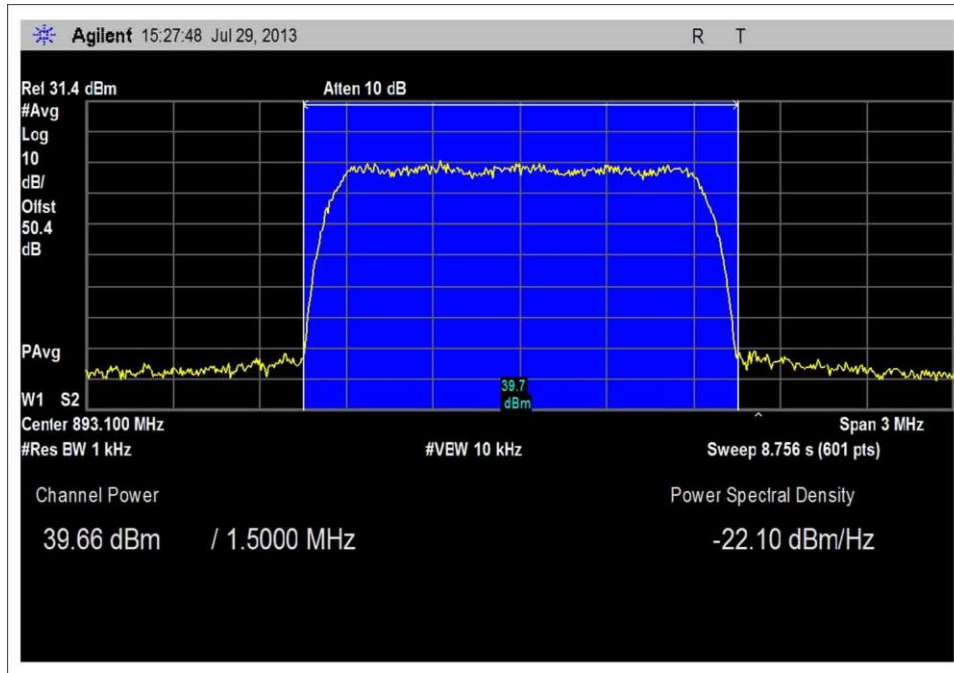
Band Power CDMA IS95A High Channel 10W
