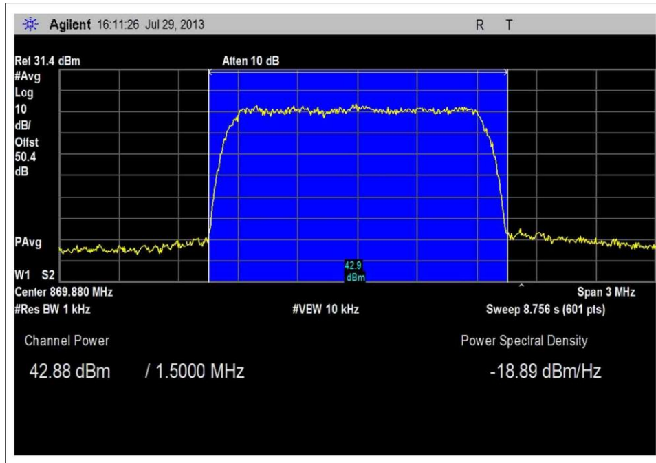
Band Power CDMA IS95A Low Channel 20W
