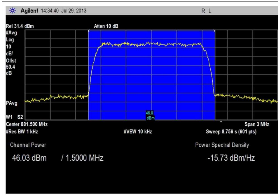
Band Power CMDA IS95A Middle Channel 40W
