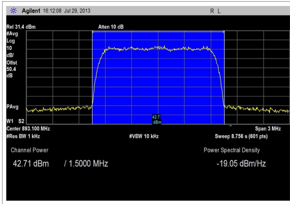
Band Power CDMA IS95A High Channel 20W
