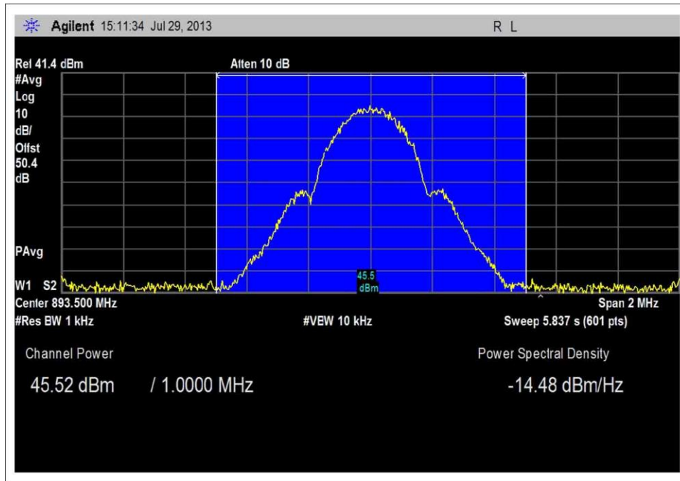
Band Power GSM High Channel 40W
