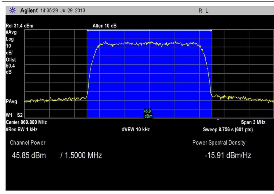
Band Power CMDA IS95A Low Channel 40W
