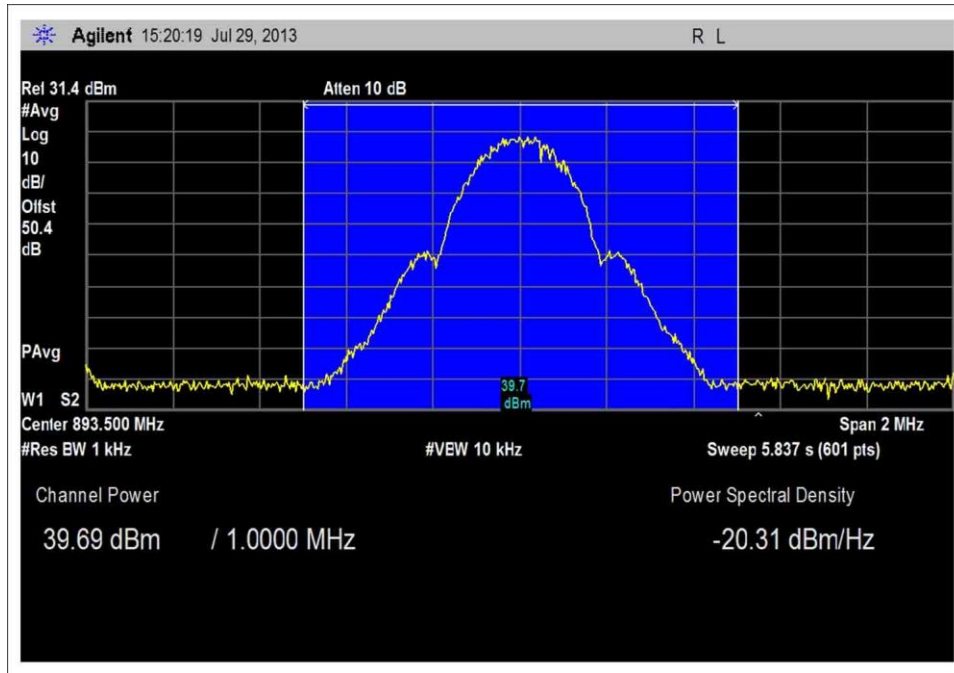
Band Power UMTS High Channel 10W
