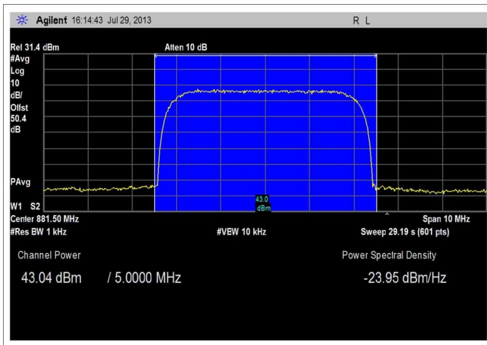
Band Power UMTS Middle Channel 20W
