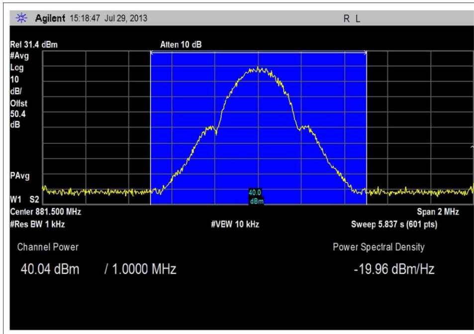
Band Power UMTS Middle Channel 10W
