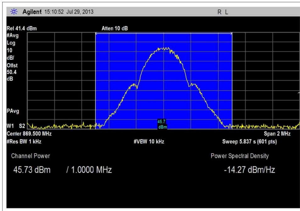
Band Power GSM Low Channel 40W
