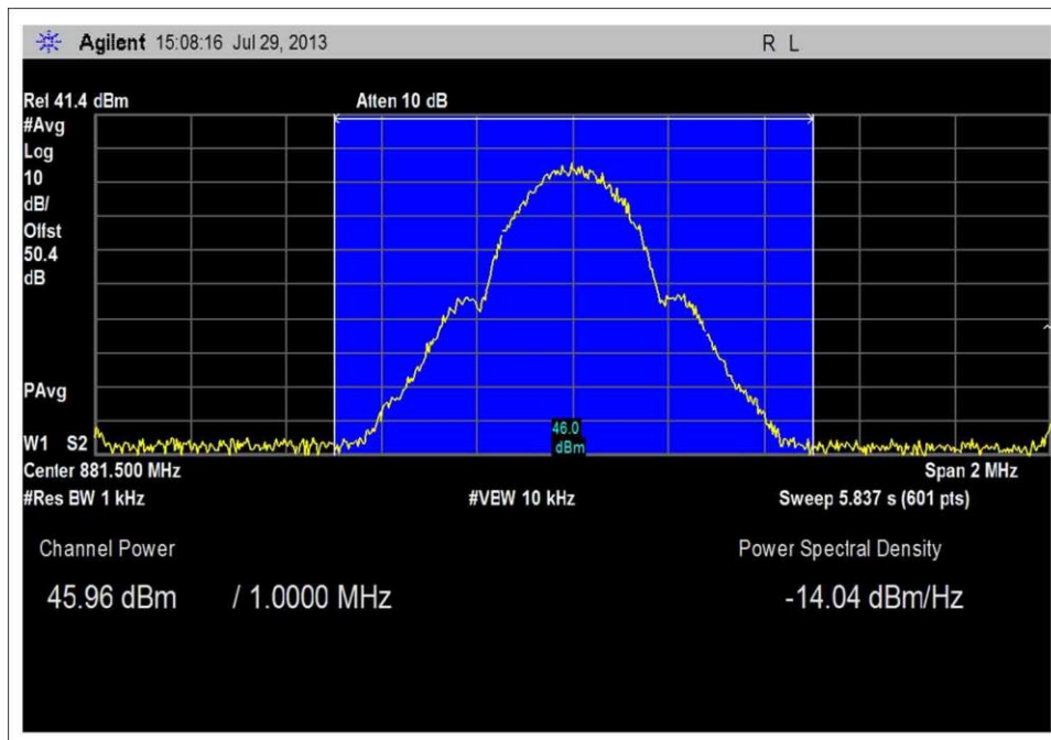
Band Power GSM Middle Channel 40W
