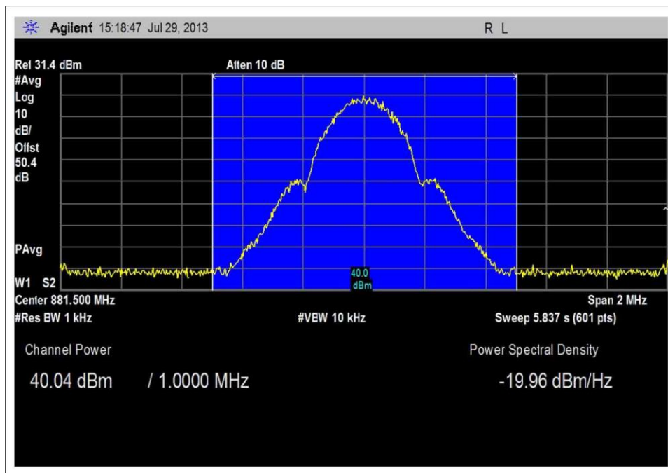
Band Power GSM Middle Channel 10W
