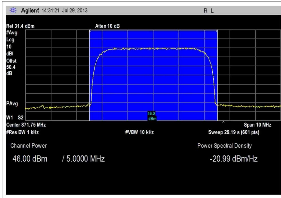
Band Power UMTS Low Channel 40W
