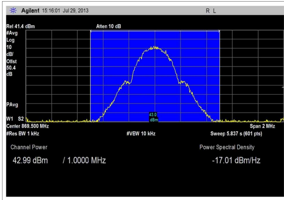
Band Power GSM Low Channel 20W
