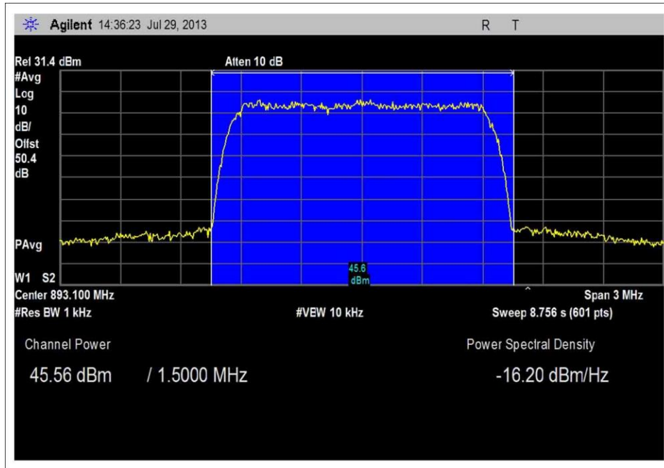
Band Power CMDA IS95A High Channel 40W
