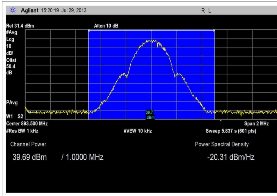
Band Power GSM High Channel 10W
