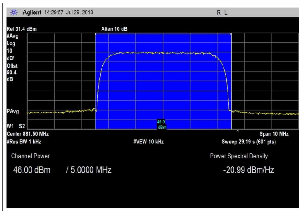
Band Power UMTS Middle Channel 40W
