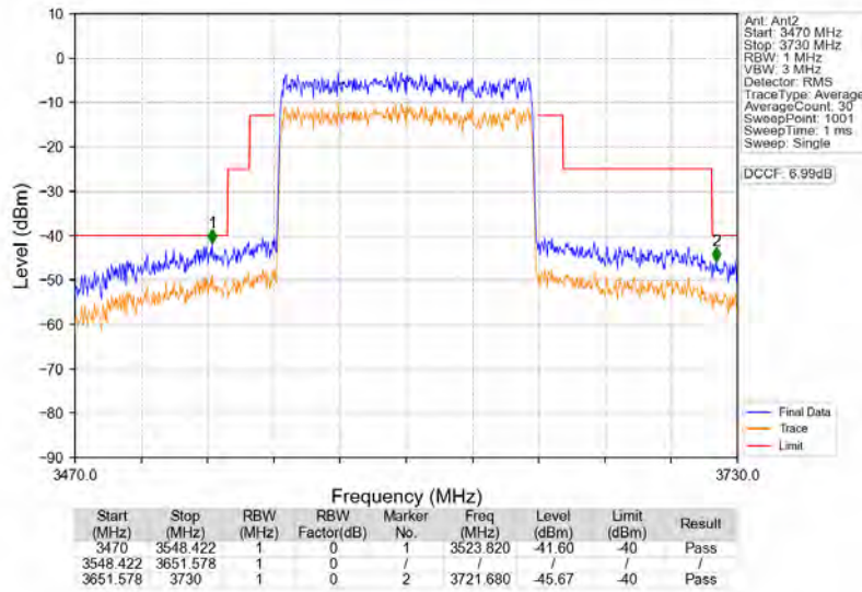
n78d_30kHz_MIMO_NTNV_100MHz_CP-OFDM QPSK_3600MHz_Outer_Full
