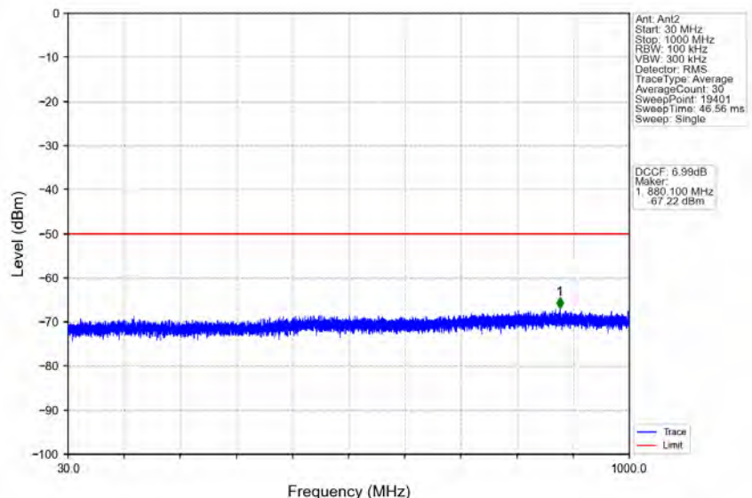
n78d_30kHz_MIMO_NTNV_90MHz_CP-OFDM QPSK_3654.99MHz_Edge_1RB_Right
