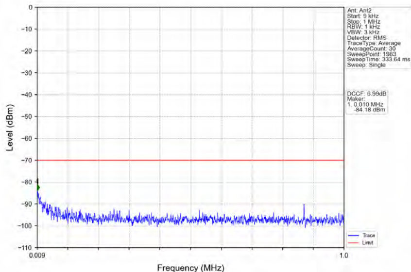
n78d_30kHz_MIMO_NTNV_100MHz_CP-OFDM QPSK_3649.98MHz_Outer_Full
