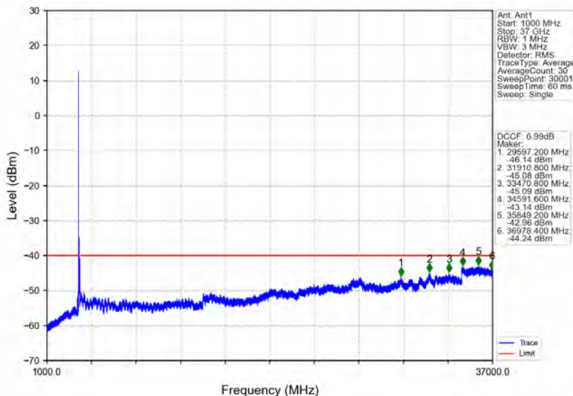
n78d_30kHz_MIMO_NTNV_100MHz_CP-OFDM QPSK_3600MHz_Edge_1RB_Left
