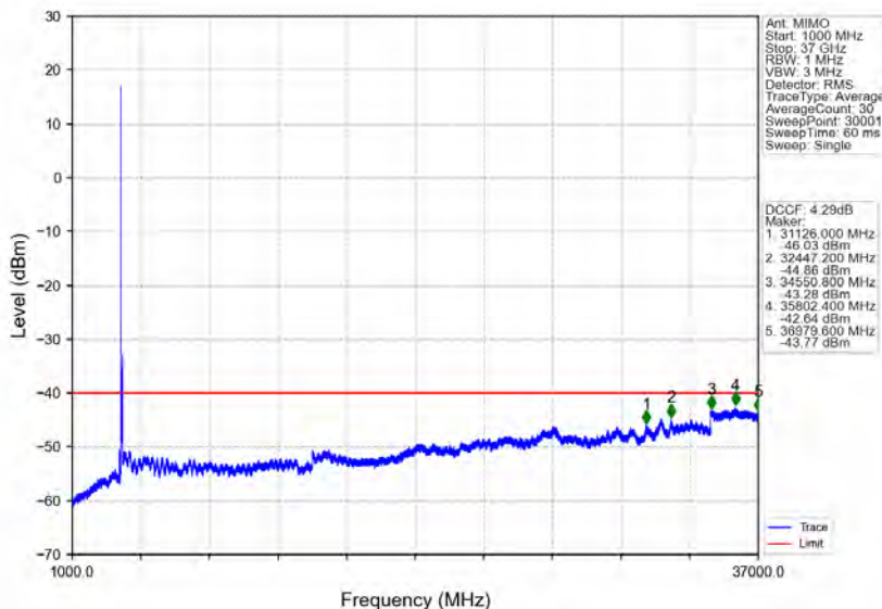
n78d_30kHz_MIMO_NTNV_90MHz_CP-OFDM QPSK_3654.99MHz_Edge_1RB_Right
