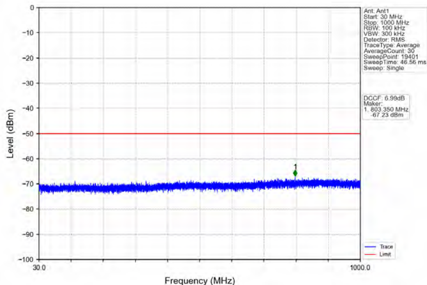
n78d_30kHz_MIMO_NTNV_100MHz_CP-OFDM QPSK_3649.98MHz_Inner_1RB_Right
