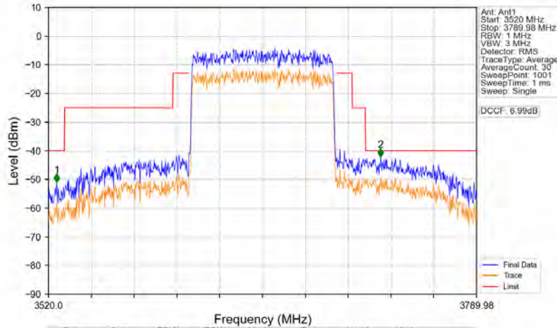
n78d_30kHz_MIMO_NTNV_90MHz_CP-OFDM_QPSK_3654.99MHz_Outer_Full
