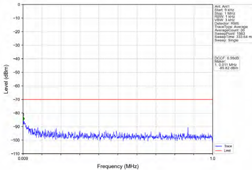
n78d_30kHz_MIMO_NTNV_100MHz_CP-OFDM QPSK_3649.98MHz_Outer_Full
