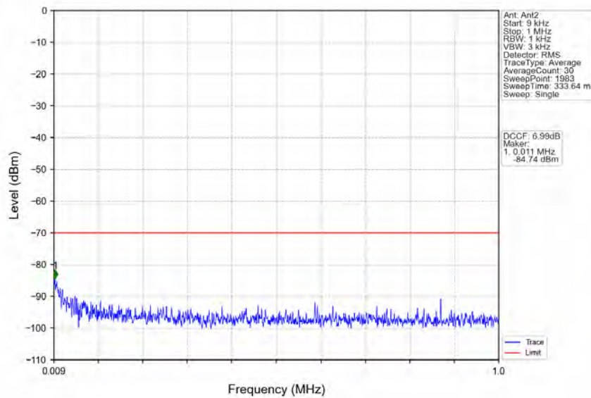
n78d_30kHz_MIMO_NTNV_100MHz_CP-OFDM QPSK_3600MHz_Outer_Full
