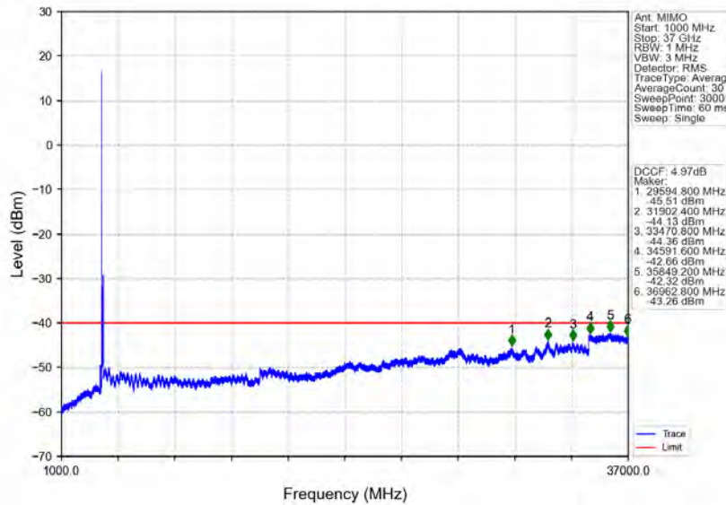
n78d_30kHz_MIMO_NTNV_100MHz_CP-OFDM QPSK_3600MHz_Outer_Full
