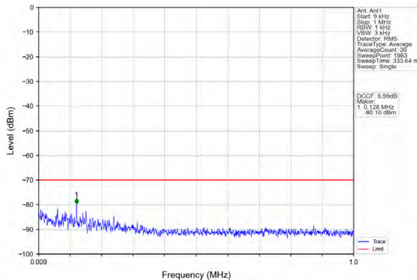
n78d_30kHz_MIMO_NTNV_90MHz_CP-OFDM_QPSK_3595.02MHz_Inner_1RB_Left
