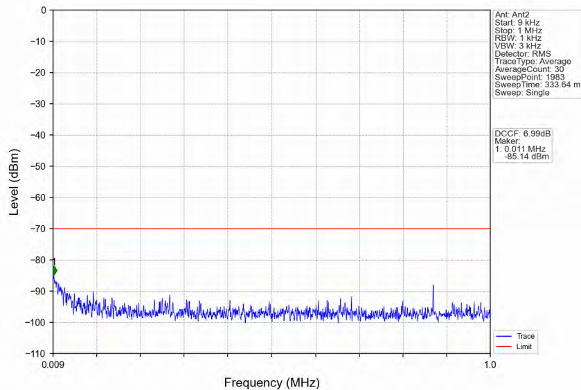
n78d_30kHz_MIMO_NTNV_90MHz_CP-OFDM_QPSK_3595.02MHz_Outer_Full
