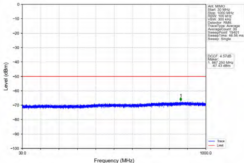
n78d_30kHz_MIMO_NTNV_100MHz_CP-OFDM QPSK_3649.98MHz_Edge_1RB_Right
