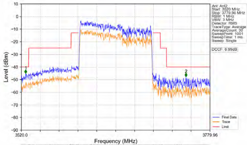
n78d_30kHz_MIMO_NTNV_100MHz_CP-OFDM_QPSK_3649.98MHz_Outer_Full
