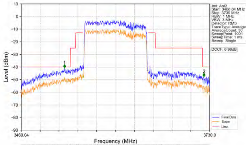
n78d_30kHz_MIMO_NTNV_90MHz_CP-OFDM_QPSK_3595.02MHz_Outer_Full
