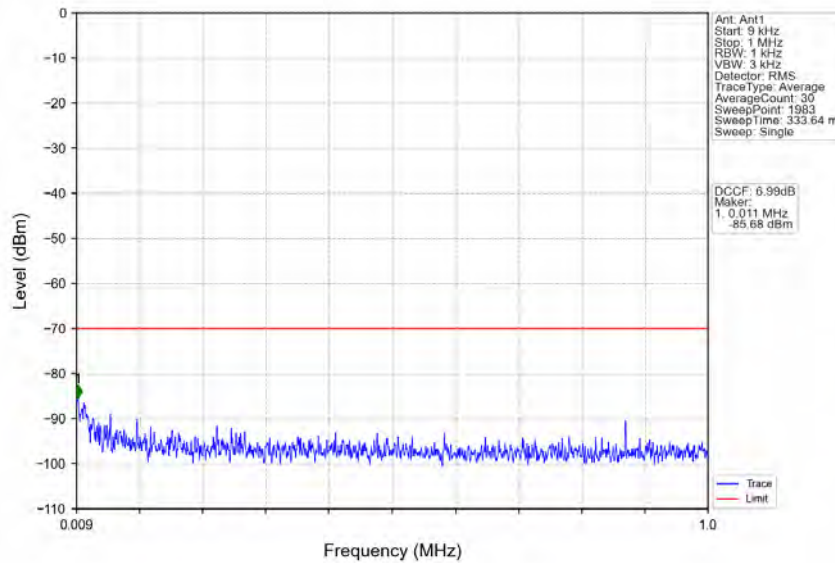
n78d_30kHz_MIMO_NTNV_90MHz_CP-OFDM_QPSK_3654.99MHz_Outer_Full
