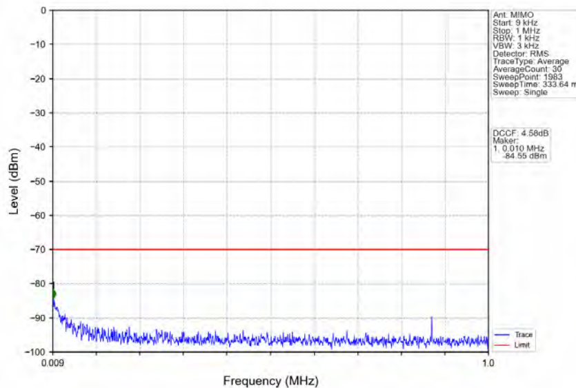
n78d_30kHz_MIMO_NTNV_100MHz_CP-OFDM_QPSK_3649.98MHz_Outer_Full
