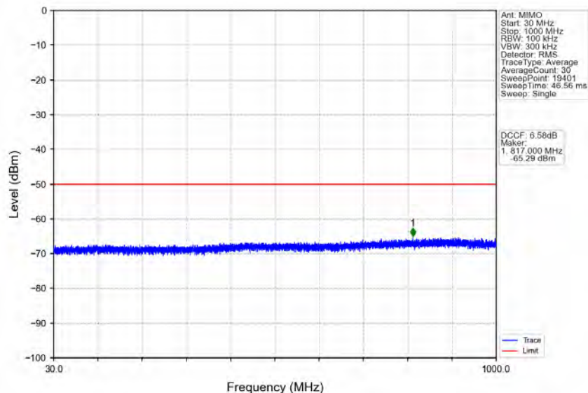
n78d_30kHz_MIMO_NTNV_90MHz_CP-OFDM QPSK_3654.99MHz_Edge_1RB_Right
