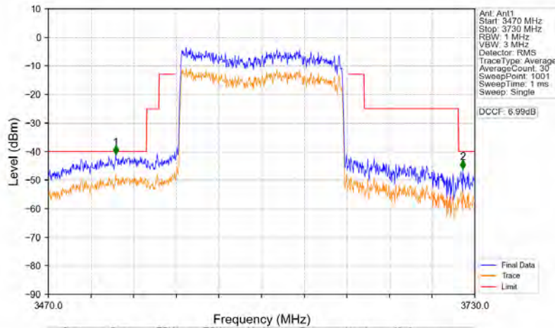
n78d_30kHz_MIMO_NTNV_100MHz_CP-OFDM QPSK_3600MHz_Outer_Full
