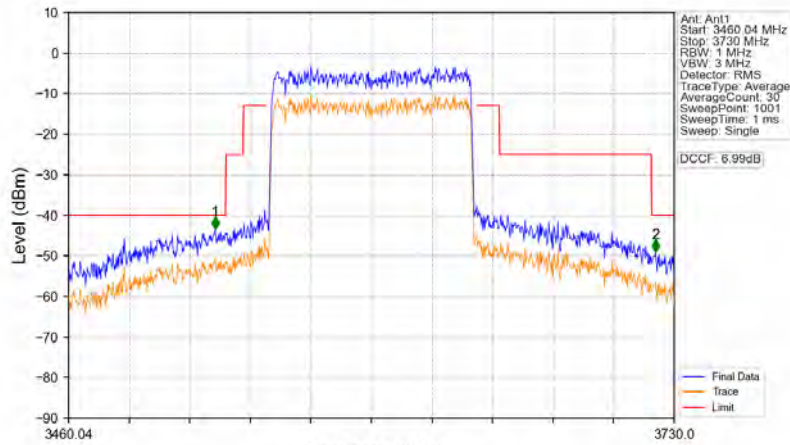
n78d_30kHz_MIMO_NTNV_90MHz_CP-OFDM QPSK_3595.02MHz_Outer_Full
