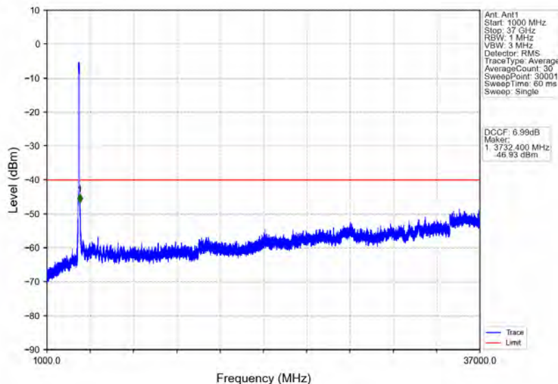
n78d_30kHz_MIMO_NTNV_90MHz_CP-OFDM_QPSK_3654.99MHz_Outer_Full
