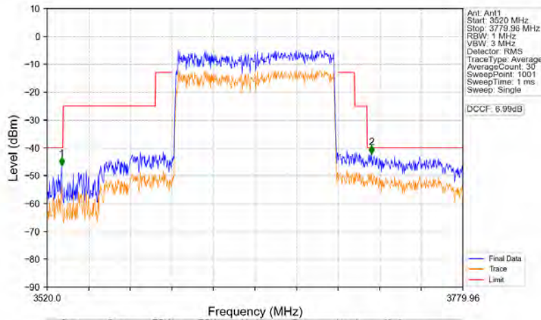
n78d_30kHz_MIMO_NTNV_100MHz_CP-OFDM QPSK_3649.98MHz_Outer_Full
