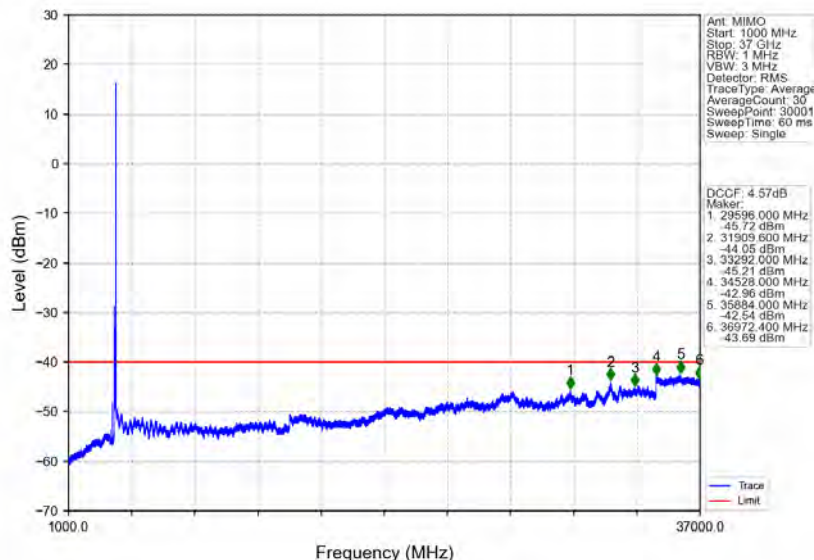
n78d_30kHz_MIMO_NTNV_100MHz_CP-OFDM QPSK_3649.98MHz_Edge_1RB_Right
