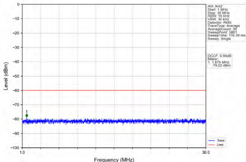
n78d_30kHz_MIMO_NTNV_90MHz_CP-OFDM QPSK_3595.02MHz_Inner_1RB_Left
