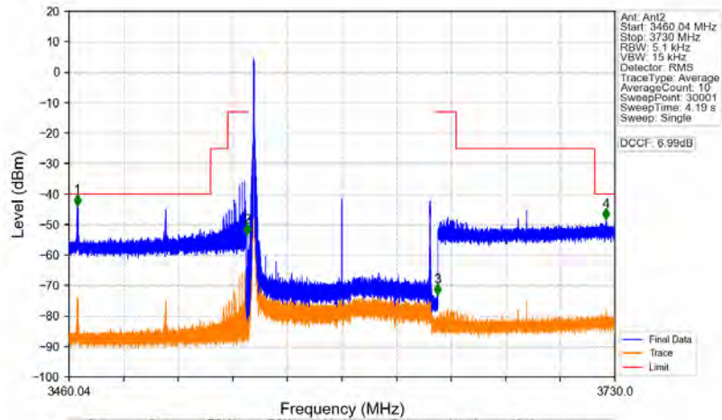
n78d_30kHz_MIMO_NTNV_90MHz_CP-OFDM QPSK_3595.02MHz_Inner_1RB_Left
