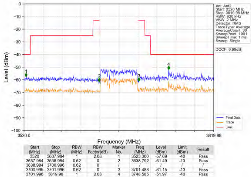
n78d_30kHz_MIMO_NTNV_60MHz_CP-OFDM_QPSK_3669.99MHz_Outer_Full
