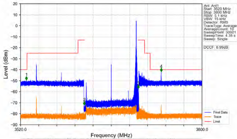
n78d_30kHz_MIMO_NTNV_80MHz_CP-OFDM QPSK_3660MHz_Inner_1RB_Right
