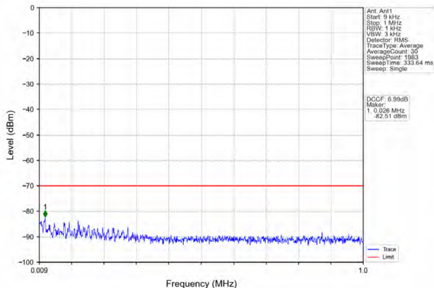
n78d_30kHz_MIMO_NTNV_80MHz_CP-OFDM QPSK_3660MHz_Inner_1RB_Right
