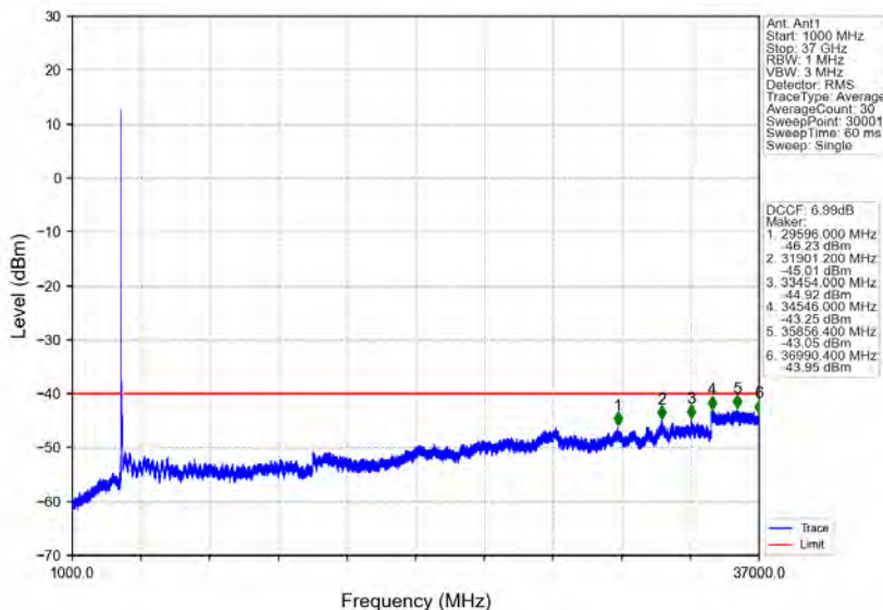
n78d_30kHz_MIMO_NTNV_80MHz_CP-OFDM_QPSK_3590.01MHz_Inner_1RB_Left
