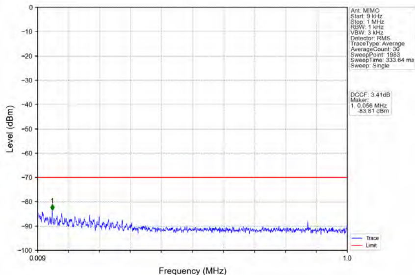
n78d_30kHz_MIMO_NTNV_70MHz_CP-OFDM QPSK_3664.98MHz_Edge_1RB_Right
