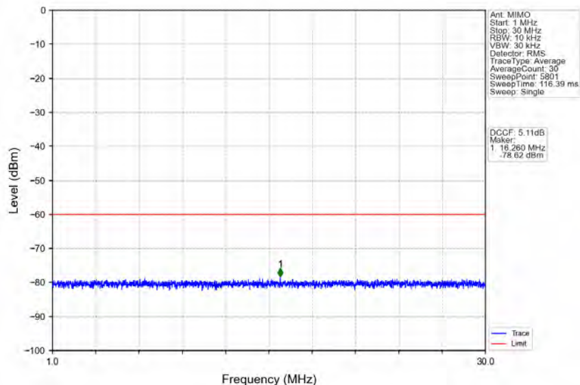
n78d_30kHz_MIMO_NTNV_80MHz_CP-OFDM QPSK_3590.01MHz_Edge_1RB_Left
