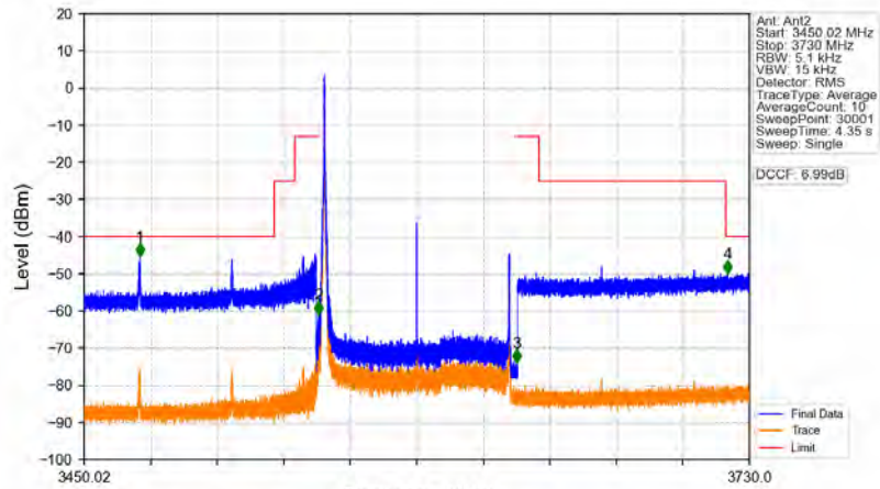
n78d_30kHz_MIMO_NTNV_80MHz_CP-OFDM_QPSK_3590.01MHz_Edge_1RB_Left
