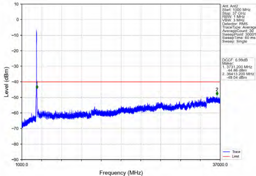
n78d_30kHz_MIMO_NTNV_70MHz_CP-OFDM QPSK_3664.98MHz_Outer_Full
