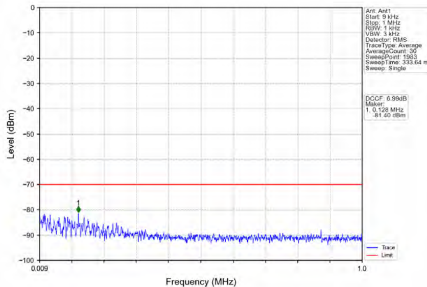
n78d_30kHz_MIMO_NTNV_80MHz_CP-OFDM_QPSK_3590.01MHz_Inner_1RB_Left
