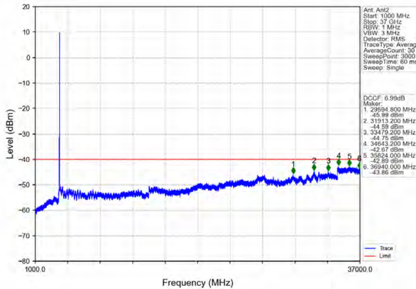
n78d_30kHz_MIMO_NTNV_60MHz_CP-OFDM_QPSK_3669.99MHz_Inner_1RB_Right
