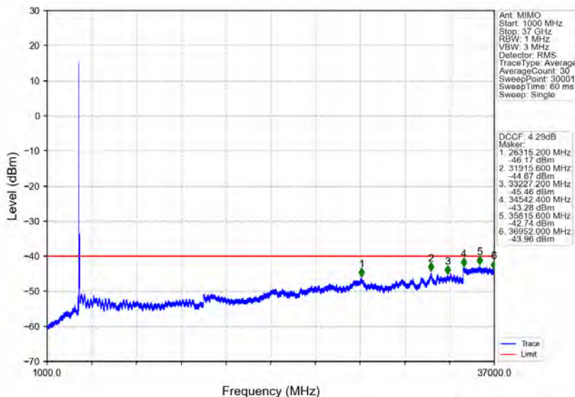
n78d_30kHz_MIMO_NTNV_70MHz_CP-OFDM QPSK_3664.98MHz_Edge_1RB_Right
