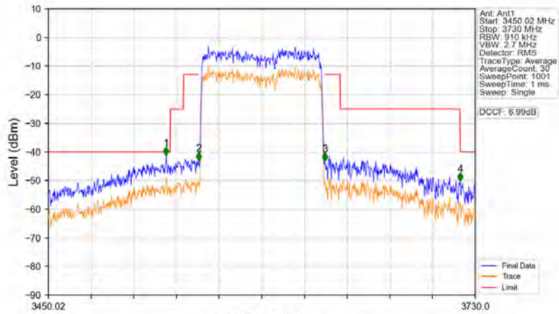
n78d_30kHz_MIMO_NTNV_80MHz_CP-OFDM QPSK_3590.01MHz_Outer_Full
