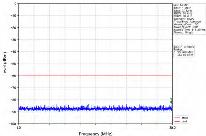
n78d_30kHz_MIMO_NTNV_70MHz_CP-OFDM QPSK_3664.98MHz_Outer_Full
