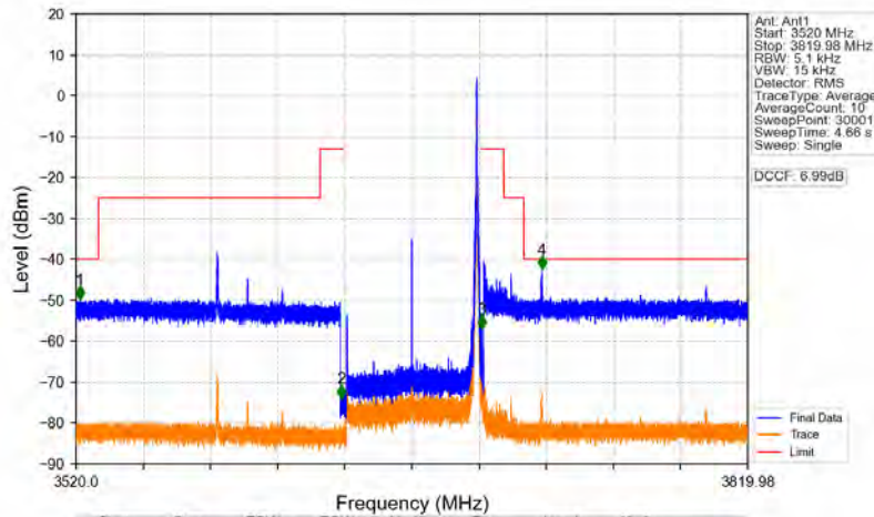
n78d_30kHz_MIMO_NTNV_60MHz_CP-OFDM QPSK_3669.99MHz_Edge_1RB_Right
