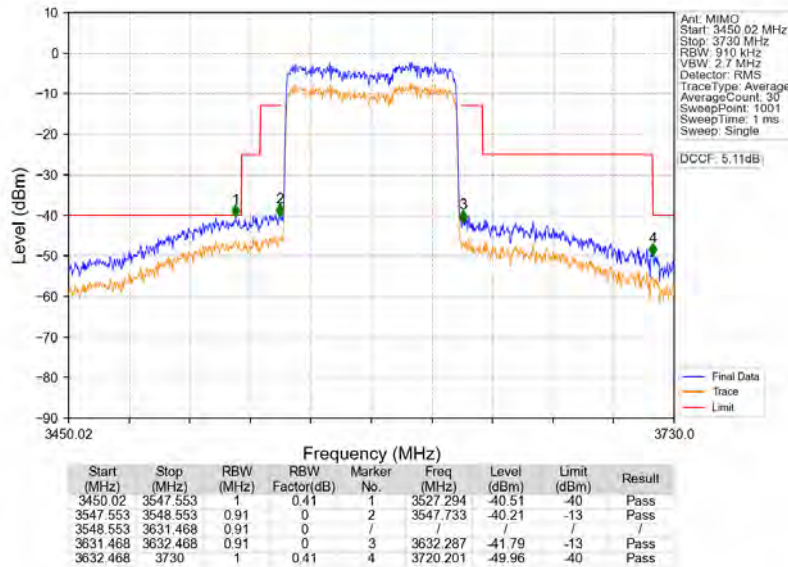
n78d_30kHz_MIMO_NTNV_80MHz_CP-OFDM_QPSK_3590.01MHz_Outer_Full
