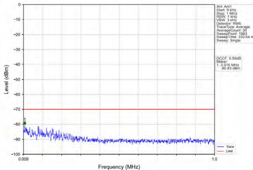
n78d_30kHz_MIMO_NTNV_70MHz_CP-OFDM QPSK_3585MHz_Inner_1RB_Left
