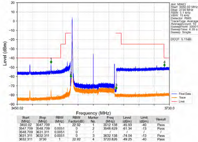
n78d_30kHz_MIMO_NTNV_80MHz_CP-OFDM_QPSK_3590.01MHz_Edge_1RB_Left
