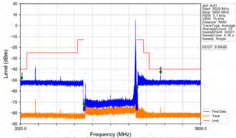
n78d_30kHz_MIMO_NTNV_80MHz_CP-OFDM QPSK_3660MHz_Edge_1RB_Right
