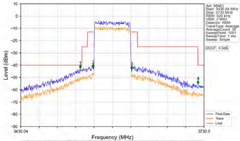
n78d_30kHz_MIMO_NTNV_60MHz_CP-OFDM_QPSK_3580.02MHz_Outer_Full
