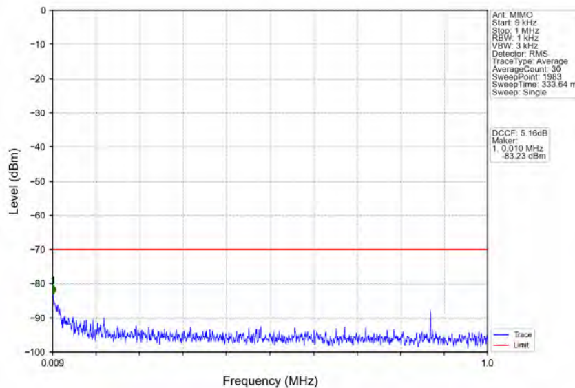
n78d_30kHz_MIMO_NTNV_60MHz_CP-OFDM_QPSK_3669.99MHz_Outer_Full
