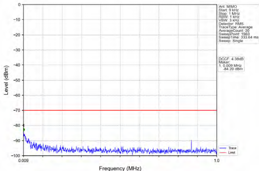
n78d_30kHz_MIMO_NTNV_70MHz_CP-OFDM QPSK_3585MHz_Outer_Full
