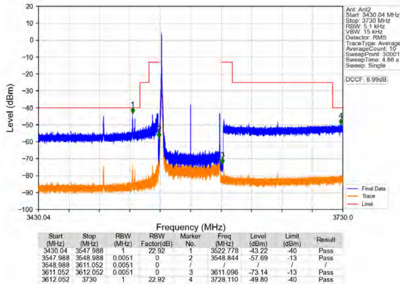
n78d_30kHz_MIMO_NTNV_60MHz_CP-OFDM_QPSK_3580.02MHz_Inner_1RB_Left
