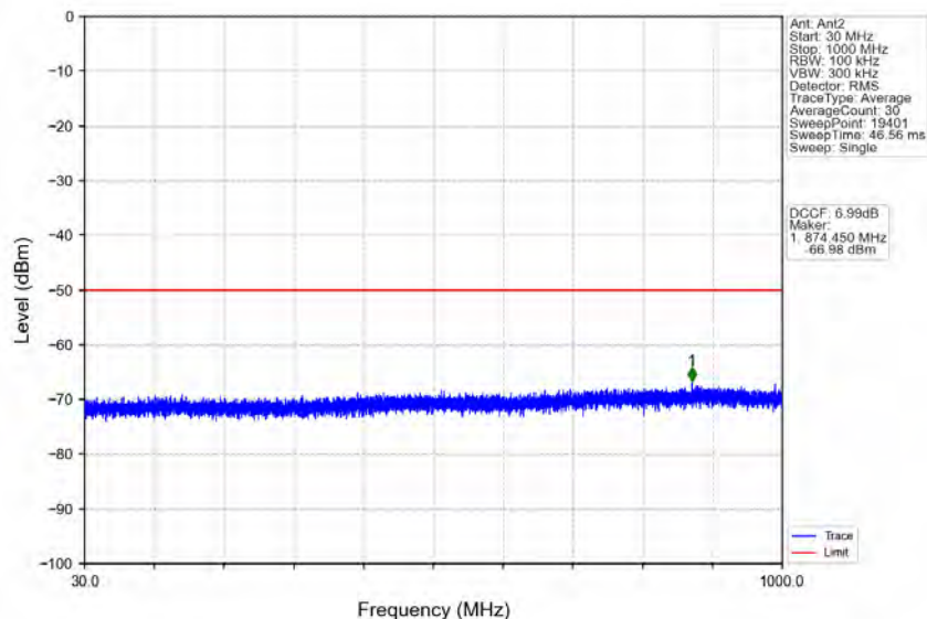
n78d_30kHz_MIMO_NTNV_80MHz_CP-OFDM QPSK_3590.01MHz_Inner_1RB_Left
