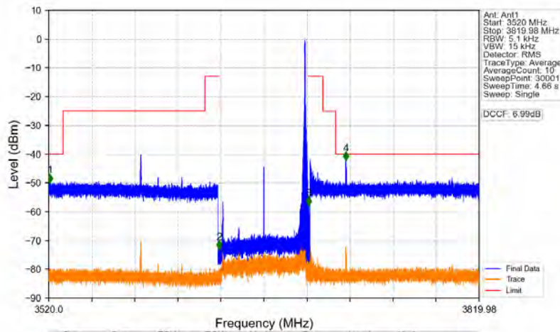
n78d_30kHz_MIMO_NTNV_60MHz_CP-OFDM QPSK_3669.99MHz_Inner_1RB_Right
