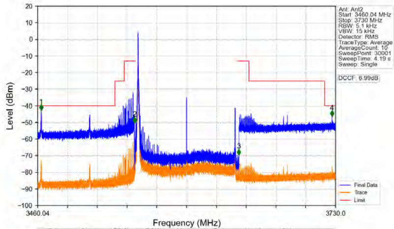
n78d_30kHz_MIMO_NTNV_90MHz_CP-OFDM_QPSK_3595.02MHz_Edge_1RB_Left
