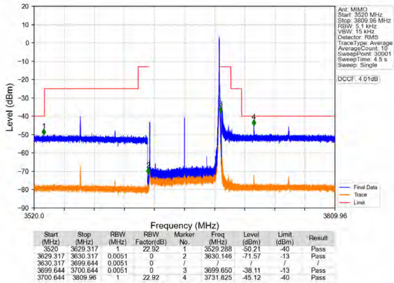
n78d_30kHz_MIMO_NTNV_70MHz_CP-OFDM_QPSK_3664.98MHz_Inner_1RB_Right
