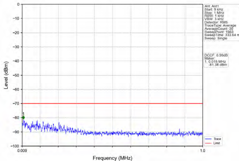
n78d_30kHz_MIMO_NTNV_60MHz_CP-OFDM_QPSK_3580.02MHz_Inner_1RB_Left
