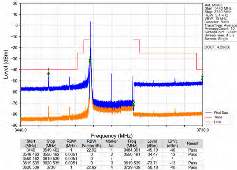
n78d_30kHz_MIMO_NTNV_70MHz_CP-OFDM QPSK_3585MHz_Inner_1RB_Left
