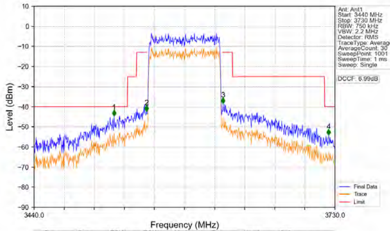
n78d_30kHz_MIMO_NTNV_70MHz_CP-OFDM QPSK_3585MHz_Outer_Full
