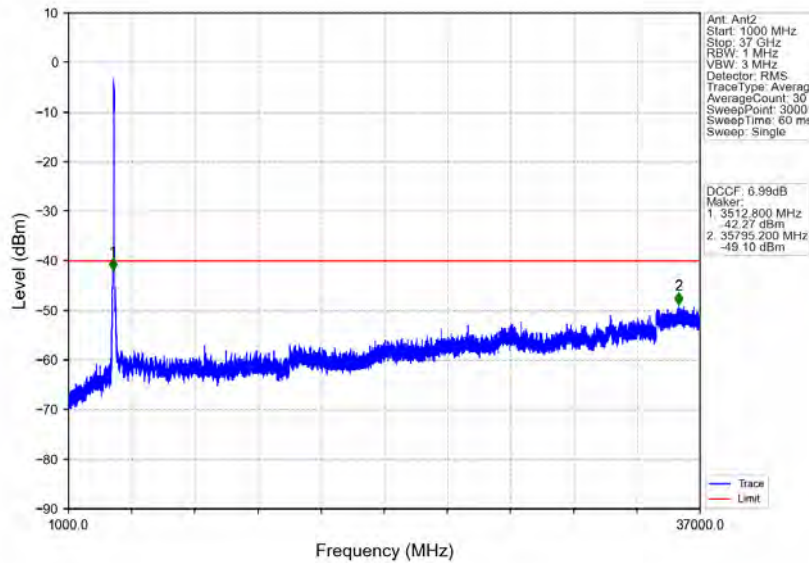
n78d_30kHz_MIMO_NTNV_80MHz_CP-OFDM_QPSK_3590.01MHz_Outer_Full
