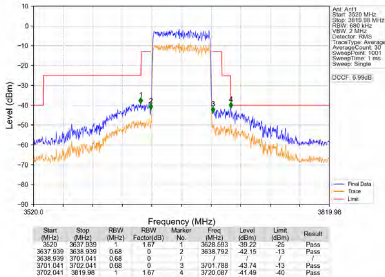
n78d_30kHz_MIMO_NTNV_60MHz_CP-OFDM_QPSK_3669.99MHz_Outer_Full
