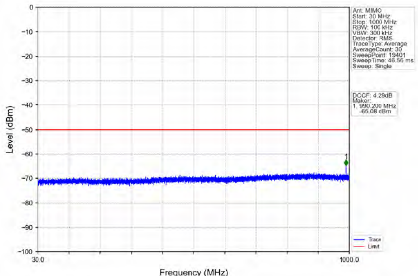
n78d_30kHz_MIMO_NTNV_70MHz_CP-OFDM QPSK_3585MHz_Inner_1RB_Left
