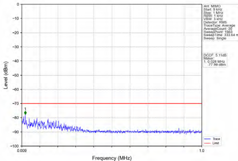
n78d_30kHz_MIMO_NTNV_80MHz_CP-OFDM_QPSK_3590.01MHz_Edge_1RB_Left
