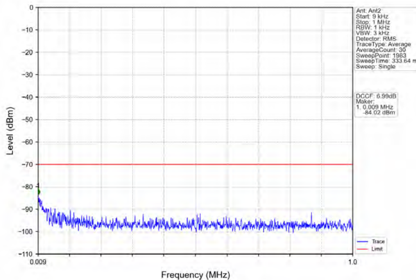
n78d_30kHz_MIMO_NTNV_70MHz_CP-OFDM QPSK_3585MHz_Outer_Full
