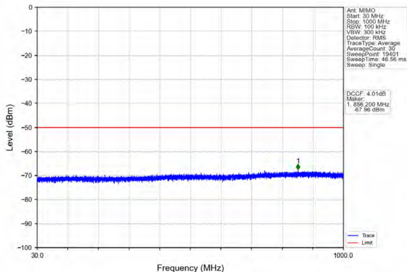
n78d_30kHz_MIMO_NTNV_70MHz_CP-OFDM QPSK_3664.98MHz_Inner_1RB_Right
