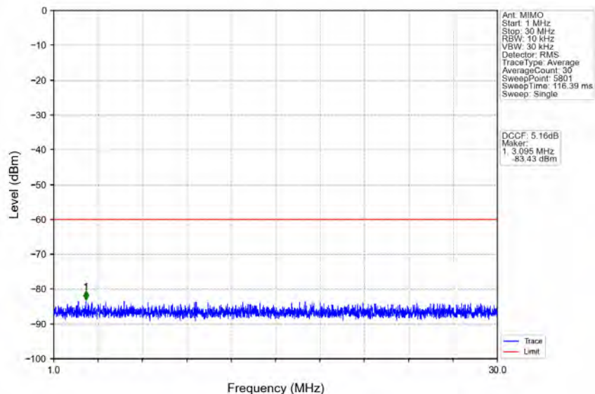
n78d_30kHz_MIMO_NTNV_60MHz_CP-OFDM QPSK_3669.99MHz_Outer_Full
