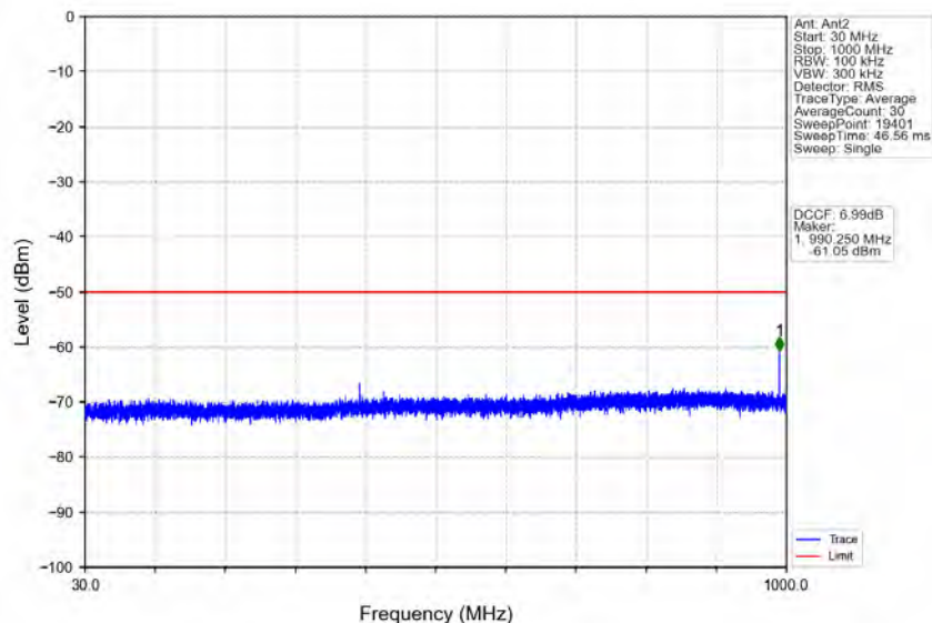
n78d_30kHz_MIMO_NTNV_30MHz_CP-OFDM QPSK_3565.02MHz_Inner_1RB_Left
