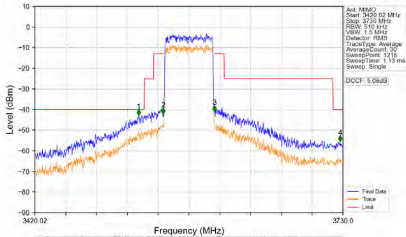
n78d_30kHz_MIMO_NTNV_50MHz_CP-OFDM_QPSK_3575.01MHz_Outer_Full
