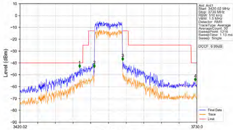
n78d_30kHz_MIMO_NTNV_50MHz_CP-OFDM QPSK_3575.01MHz_Outer_Full
