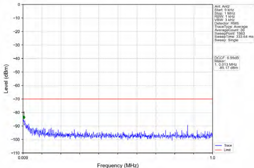
n78d_30kHz_MIMO_NTNV_50MHz_CP-OFDM QPSK_3675MHz_Outer_Full
