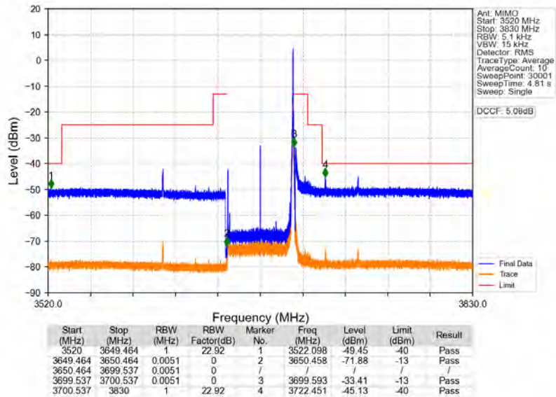
n78d_30kHz_MIMO_NTNV_50MHz_CP-OFDM QPSK_3675MHz_Edge_1RB_Right
