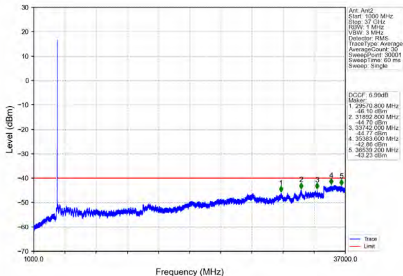
n78d_30kHz_MIMO_NTNV_30MHz_CP-OFDM_QPSK_3684.99MHz_Edge_1RB_Right
