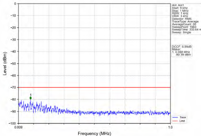
n78d_30kHz_MIMO_NTNV_30MHz_CP-OFDM_QPSK_3565.02MHz_Inner_1RB_Left
