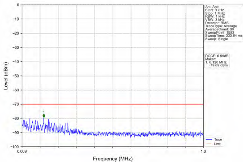
n78d_30kHz_MIMO_NTNV_40MHz_CP-OFDM_QPSK_3570MHz_Edge_1RB_Left
