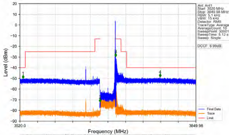
n78d_30kHz_MIMO_NTNV_30MHz_CP-OFDM QPSK_3684.99MHz_Edge_1RB_Right
