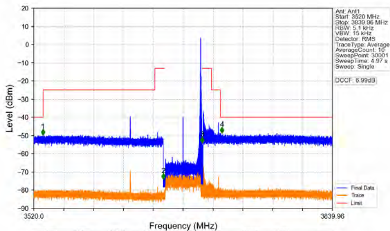
n78d_30kHz_MIMO_NTNV_40MHz_CP-OFDM QPSK_3679.98MHz_Edge_1RB_Right
