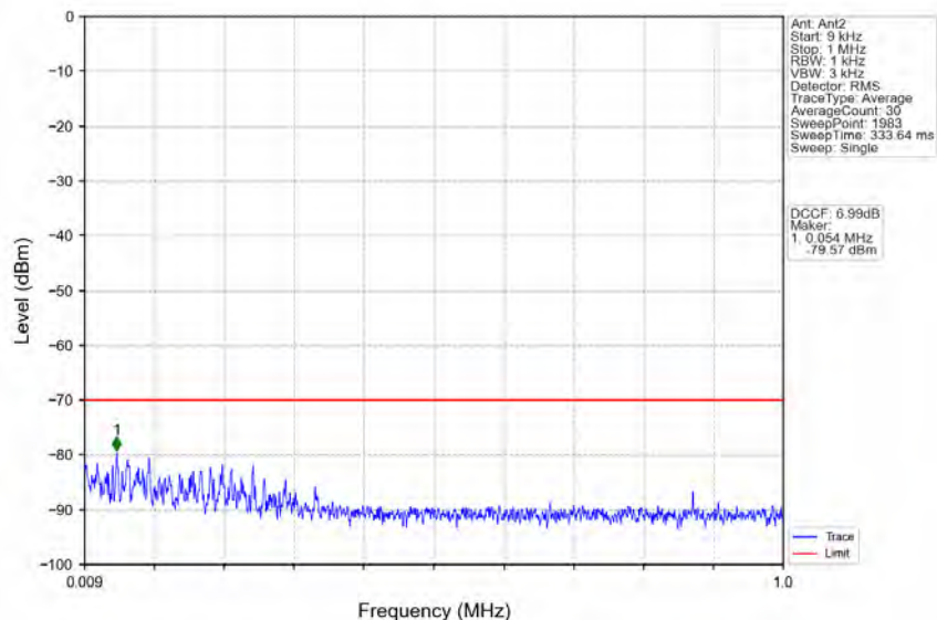
n78d_30kHz_MIMO_NTNV_50MHz_CP-OFDM QPSK_3575.01MHz_Inner_1RB_Left
