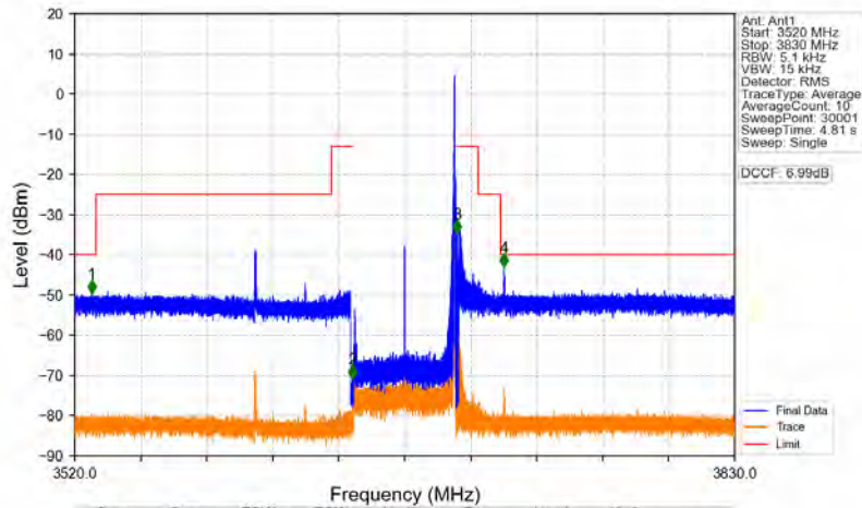
n78d_30kHz_MIMO_NTNV_50MHz_CP-OFDM QPSK_3675MHz_Inner_1RB_Right
