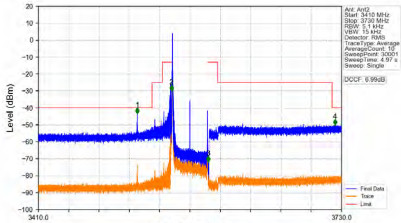
n78d_30kHz_MIMO_NTNV_40MHz_CP-OFDM_QPSK_3570MHz_Inner_1RB_Left
