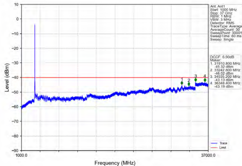
n78d_30kHz_MIMO_NTNV_40MHz_CP-OFDM QPSK_3570MHz_Outer_Full
