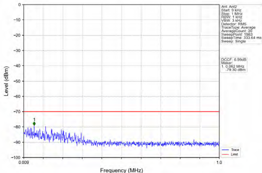
n78d_30kHz_MIMO_NTNV_50MHz_CP-OFDM QPSK_3575.01MHz_Edge_1RB_Left
