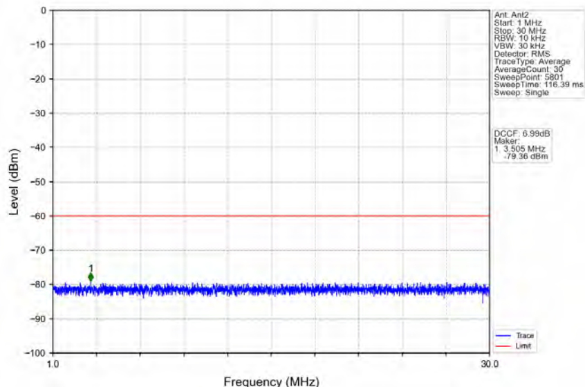
n78d_30kHz_MIMO_NTNV_60MHz_CP-OFDM QPSK_3580.02MHz_Edge_1RB_Left
