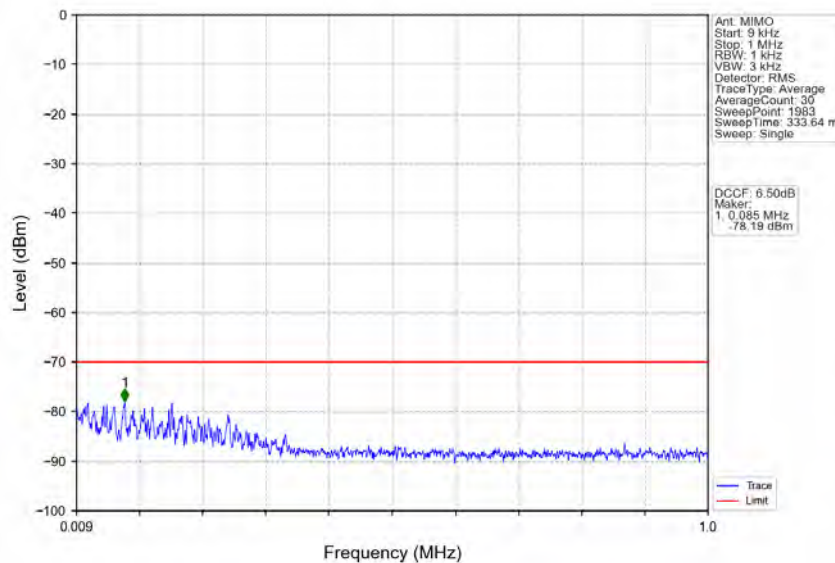
n78d_30kHz_MIMO_NTNV_40MHz_CP-OFDM QPSK_3570MHz_Edge_1RB_Left
