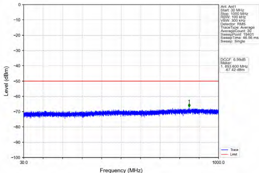
n78d_30kHz_MIMO_NTNV_40MHz_CP-OFDM_QPSK_3679.98MHz_Inner_1RB_Right
