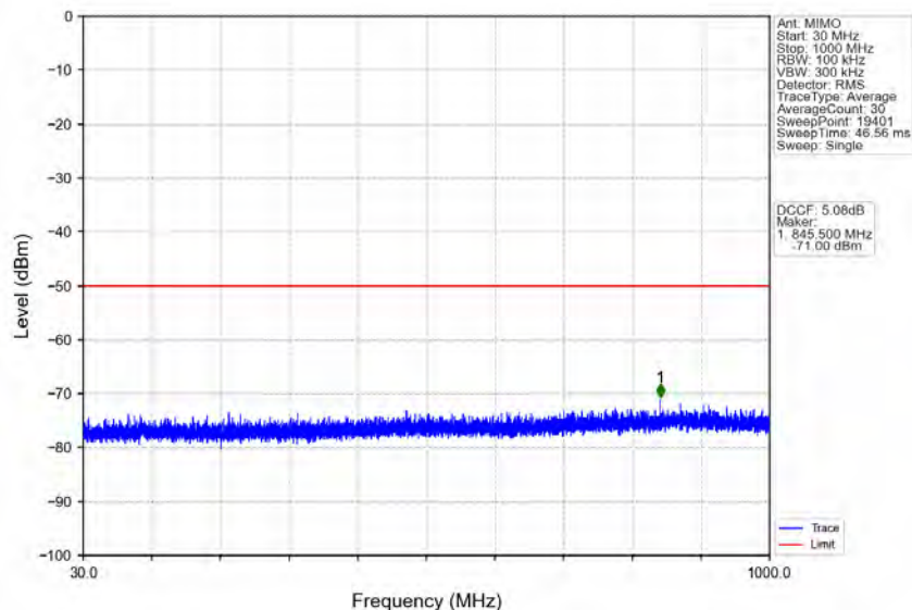
n78d_30kHz_MIMO_NTNV_50MHz_CP-OFDM QPSK_3575.01MHz_Outer_Full
