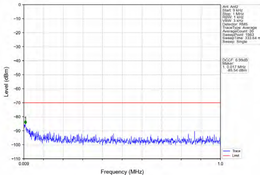
n78d_30kHz_MIMO_NTNV_50MHz_CP-OFDM_QPSK_3575.01MHz_Outer_Full
