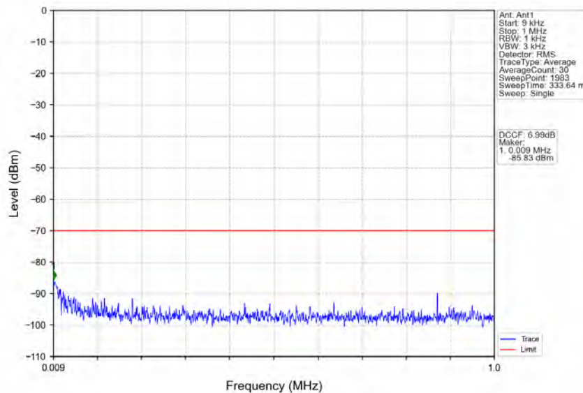
n78d_30kHz_MIMO_NTNV_40MHz_CP-OFDM_QPSK_3679.98MHz_Outer_Full
