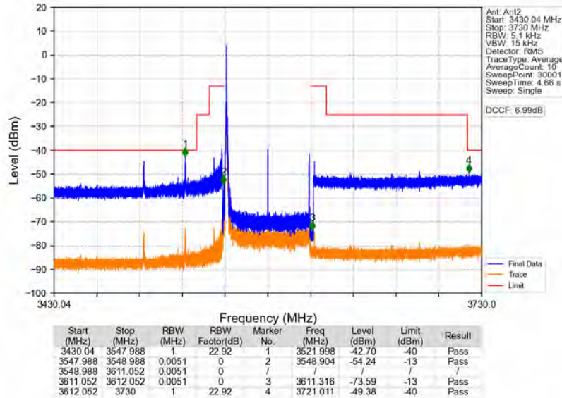
n78d_30kHz_MIMO_NTNV_60MHz_CP-OFDM_QPSK_3580.02MHz_Edge_1RB_Left
