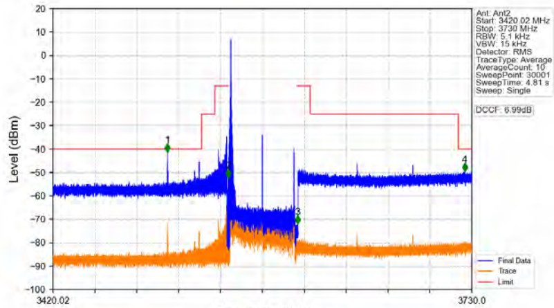
n78d_30kHz_MIMO_NTNV_50MHz_CP-OFDM_QPSK_3575.01MHz_Inner_1RB_Left
