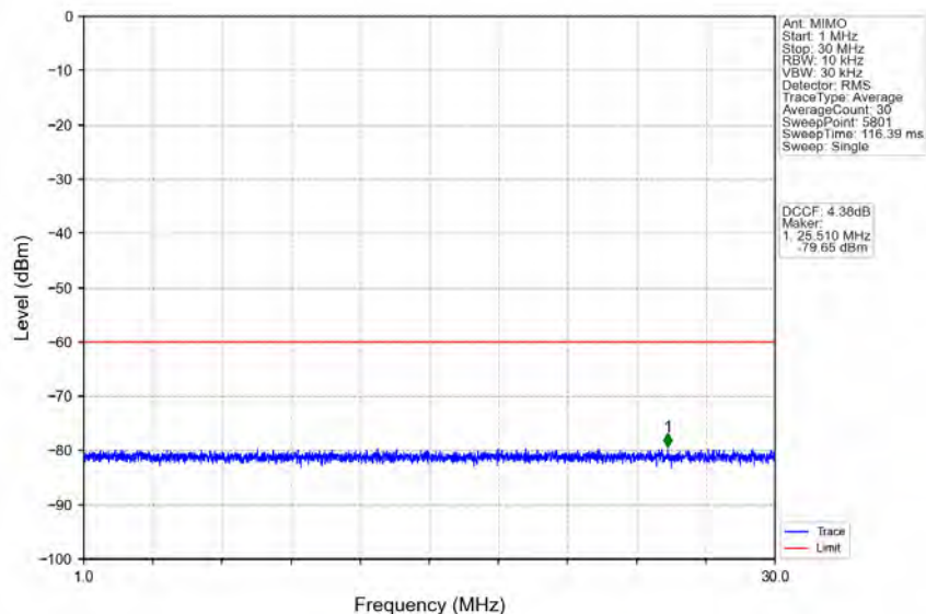
n78d_30kHz_MIMO_NTNV_30MHz_CP-OFDM QPSK_3565.02MHz_Inner_1RB_Left
