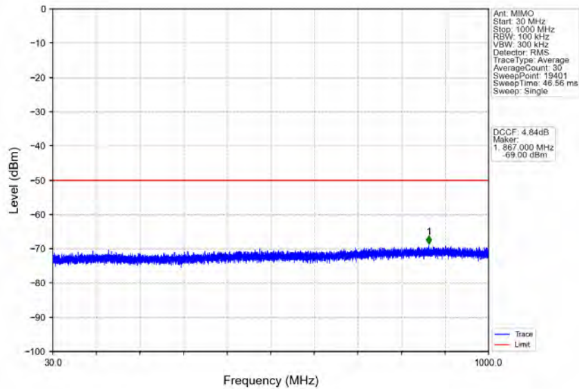
n78d_30kHz_MIMO_NTNV_40MHz_CP-OFDM QPSK_3570MHz_Outer_Full
