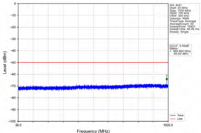
n78d_30kHz_MIMO_NTNV_40MHz_CP-OFDM QPSK_3570MHz_Edge_1RB_Left
