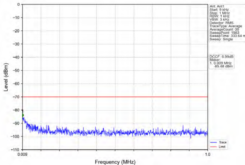
n78d_30kHz_MIMO_NTNV_30MHz_CP-OFDM_QPSK_3684.99MHz_Outer_Full
