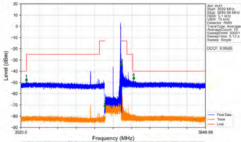
n78d_30kHz_MIMO_NTNV_30MHz_CP-OFDM QPSK_3684.99MHz_Inner_1RB_Right
