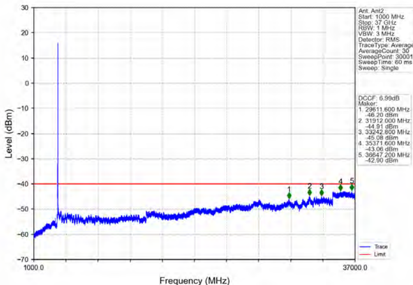
n78d_30kHz_MIMO_NTNV_40MHz_CP-OFDM_QPSK_3679.98MHz_Inner_1RB_Right
