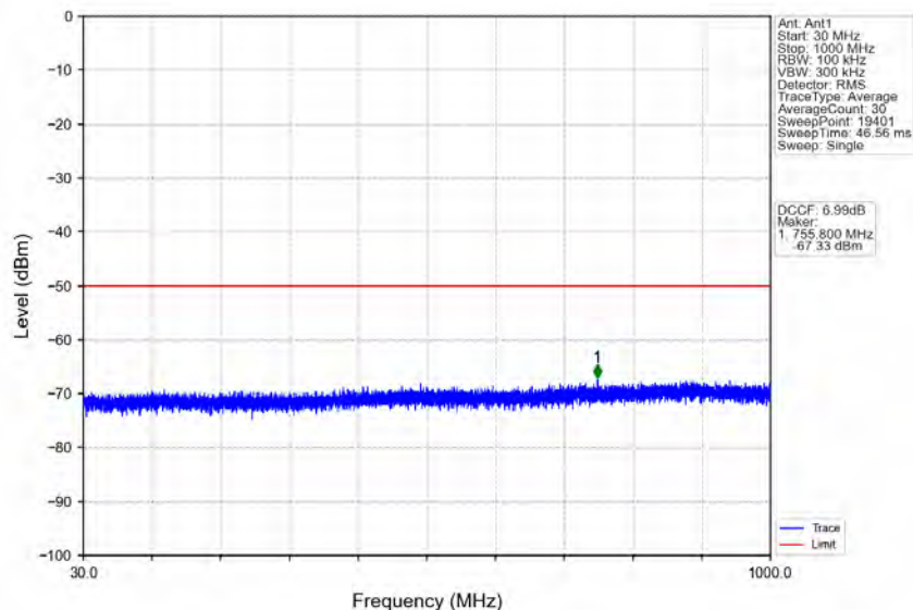
n78d_30kHz_MIMO_NTNV_50MHz_CP-OFDM QPSK_3675MHz_Inner_1RB_Right
