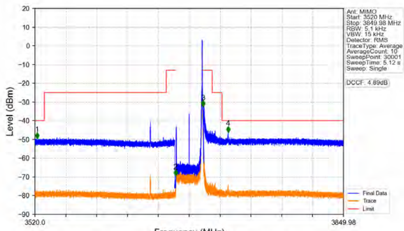
n78d_30kHz_MIMO_NTNV_30MHz_CP-OFDM_QPSK_3684.99MHz_Edge_1RB_Right
