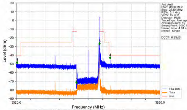
n78d_30kHz_MIMO_NTNV_50MHz_CP-OFDM QPSK_3675MHz_Edge_1RB_Right
