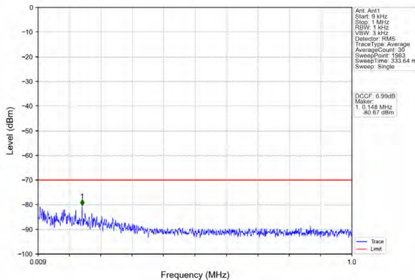
n78d_30kHz_MIMO_NTNV_40MHz_CP-OFDM QPSK_3570MHz_Inner_1RB_Left
