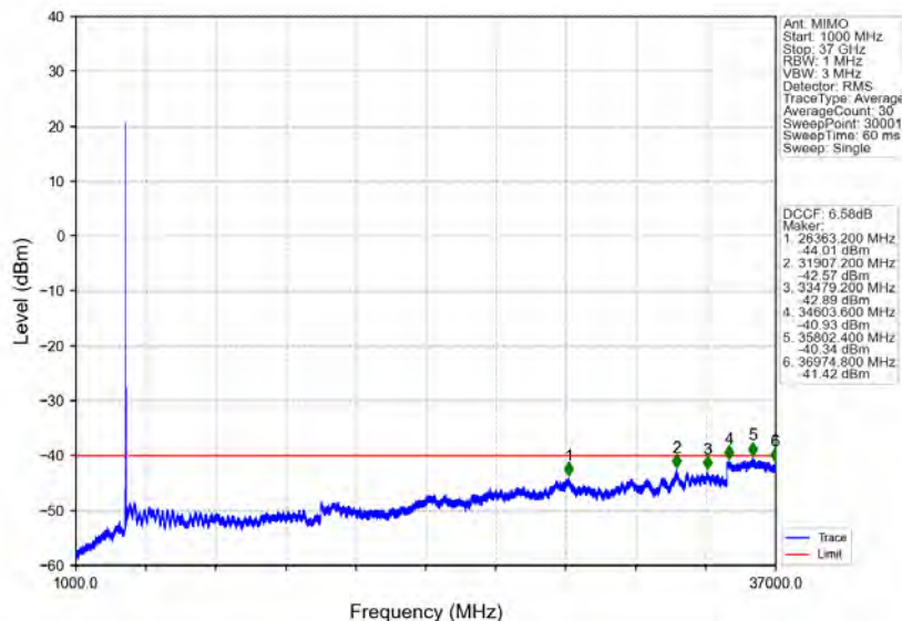
n78d_30kHz_MIMO_NTNV_40MHz_CP-OFDM QPSK_3679.98MHz_Edge_1RB_Right
