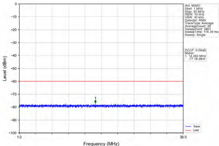
n78d_30kHz_MIMO_NTNV_40MHz_CP-OFDM QPSK_3570MHz_Inner_1RB_Left
