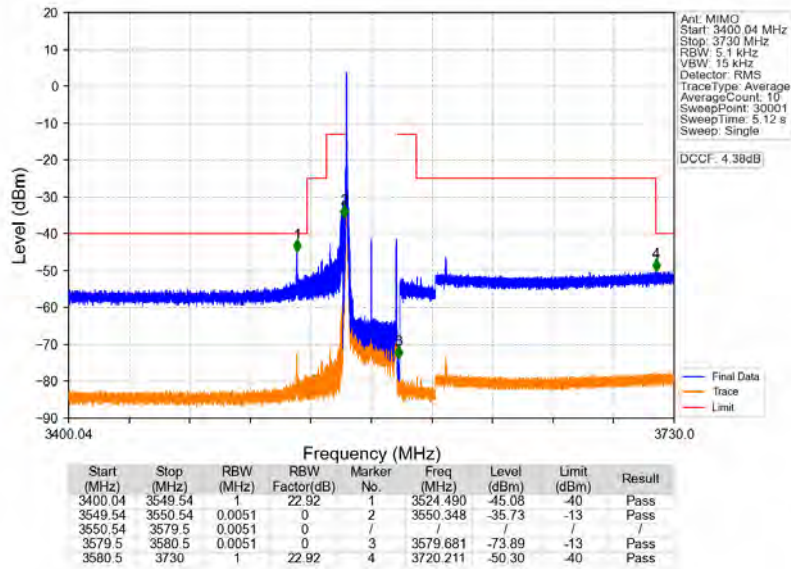
n78d_30kHz_MIMO_NTNV_30MHz_CP-OFDM_QPSK_3565.02MHz_Inner_1RB_Left
