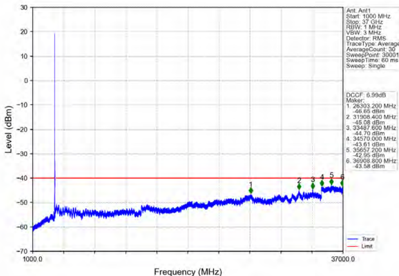
n78d_30kHz_MIMO_NTNV_20MHz_CP-OFDM QPSK_3560.01MHz_Inner_1RB_Left
