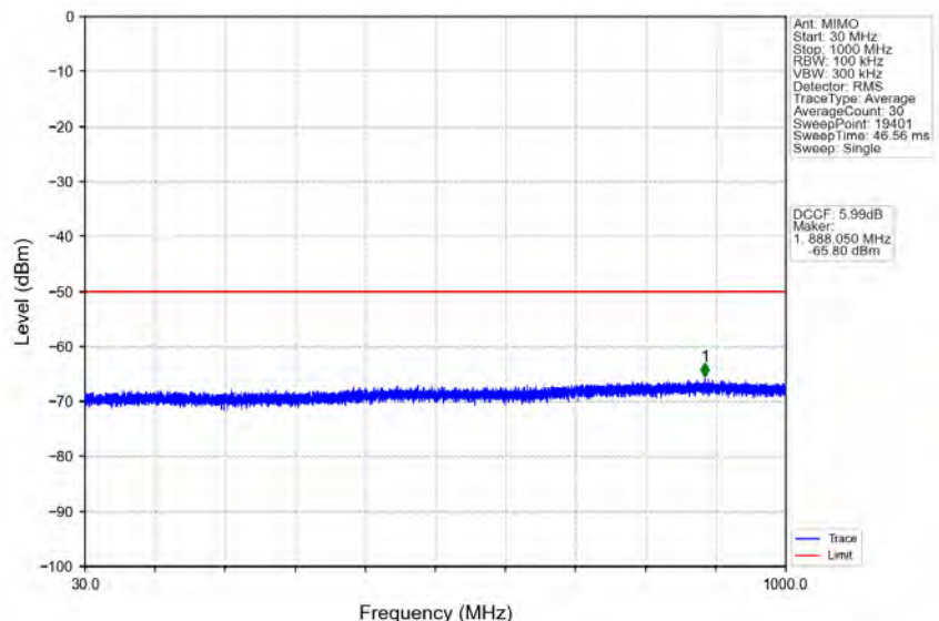
n78d_30kHz_MIMO_NTNV_20MHz_CP-OFDM QPSK_3690MHz_Outer_Full
