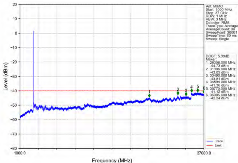
n78d_30kHz_MIMO_NTNV_20MHz_CP-OFDM QPSK_3690MHz_Inner_1RB_Right
