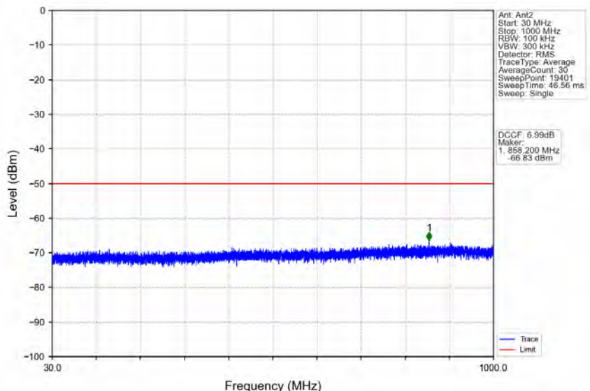
n78d_30kHz_MIMO_NTNV_20MHz_CP-OFDM_QPSK_3560.01MHz_Outer_Full
