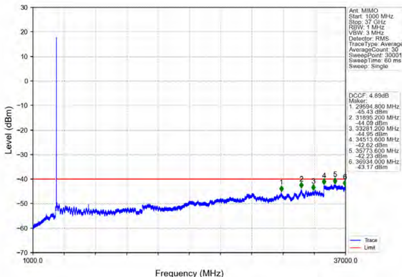
n78d_30kHz_MIMO_NTNV_10MHz_CP-OFDM QPSK_3694.98MHz_Edge_1RB_Right
