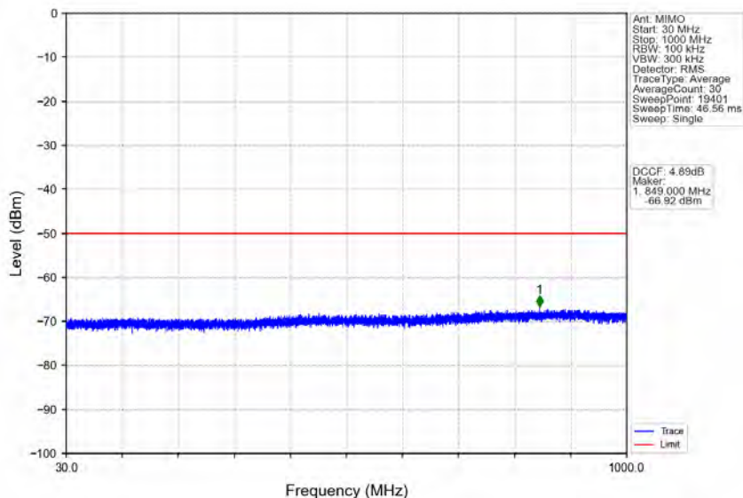
n78d_30kHz_MIMO_NTNV_10MHz_CP-OFDM QPSK_3694.98MHz_Edge_1RB_Right
