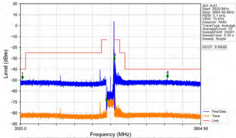
n78d_30kHz_MIMO_NTNV_15MHz_CP-OFDM QPSK_3692.49MHz_Edge_1RB_Right
