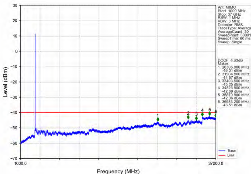
n78d_30kHz_MIMO_NTNV_10MHz_CP-OFDM QPSK_3694.98MHz_Inner_1RB_Right
