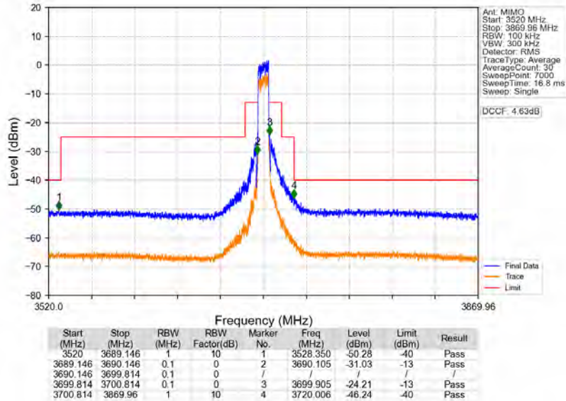
n78d_30kHz_MIMO_NTNV_10MHz_CP-OFDM QPSK_3694.98MHz_Outer_Full
