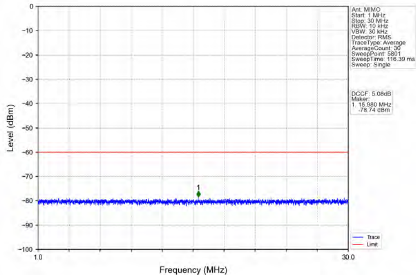
n78d_30kHz_MIMO_NTNV_15MHz_CP-OFDM QPSK_3692.49MHz_Edge_1RB_Right
