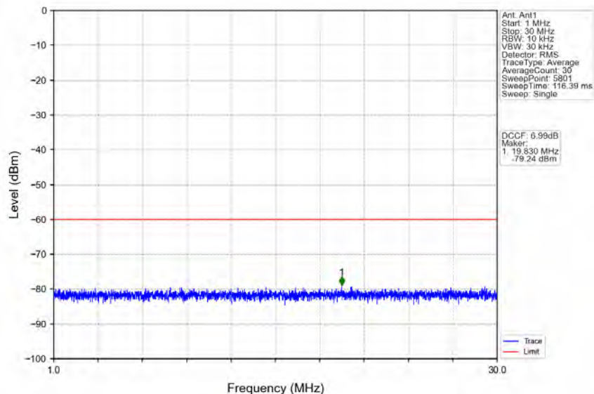
n78d_30kHz_MIMO_NTNV_15MHz_CP-OFDM QPSK_3557.52MHz_Edge_1RB_Left
