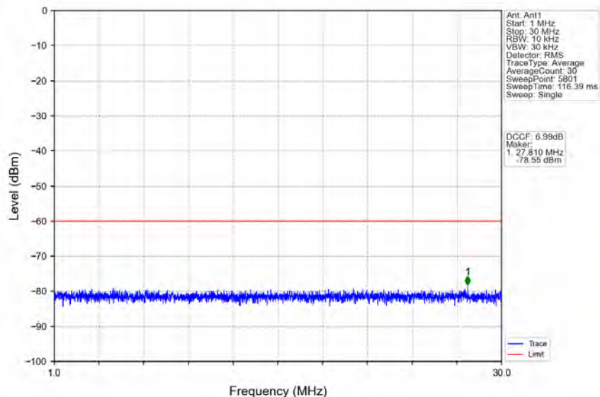
n78d_30kHz_MIMO_NTNV_15MHz_CP-OFDM_QPSK_3692.49MHz_Outer_Full
