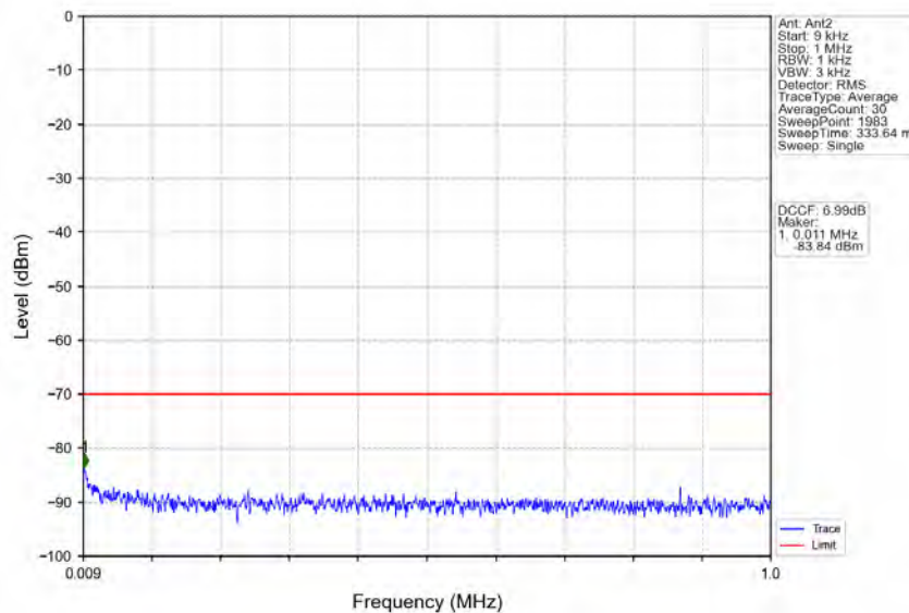
n78d_30kHz_MIMO_NTNV_20MHz_CP-OFDM_QPSK_3560.01MHz_Outer_Full
