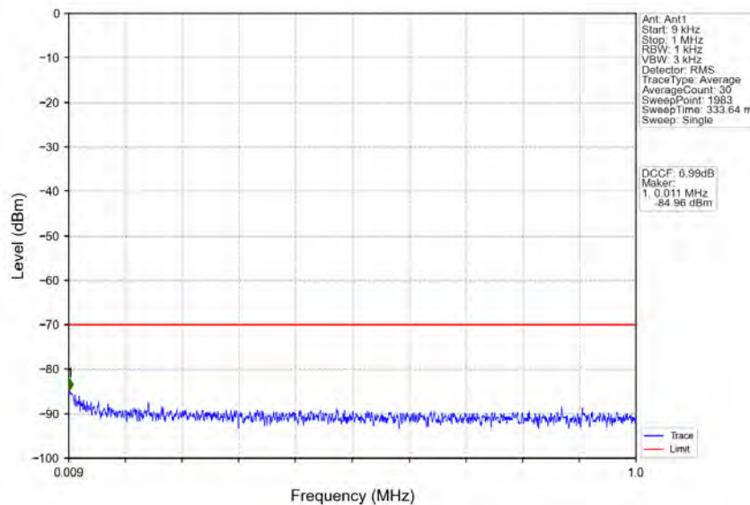
n78d_30kHz_MIMO_NTNV_15MHz_CP-OFDM_QPSK_3692.49MHz_Outer_Full
