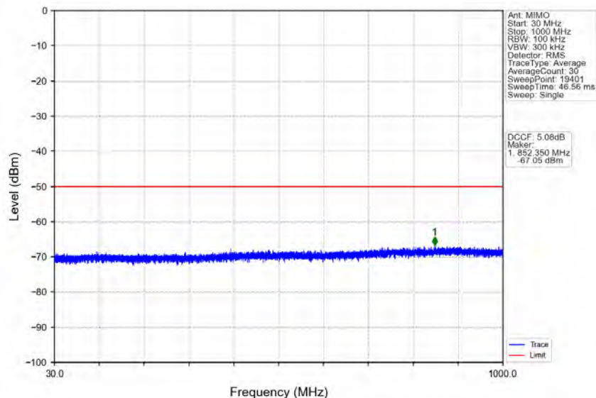
n78d_30kHz_MIMO_NTNV_15MHz_CP-OFDM QPSK_3692.49MHz_Edge_1RB_Right
