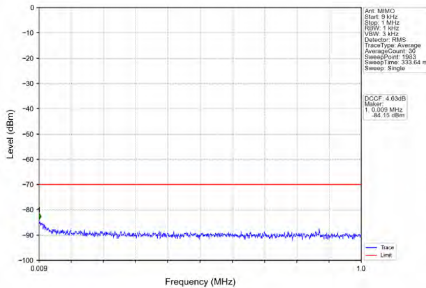
n78d_30kHz_MIMO_NTNV_10MHz_CP-OFDM QPSK_3694.98MHz_Outer_Full
