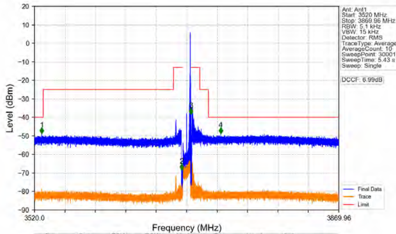
n78d_30kHz_MIMO_NTNV_10MHz_CP-OFDM QPSK_3694.98MHz_Edge_1RB_Right
