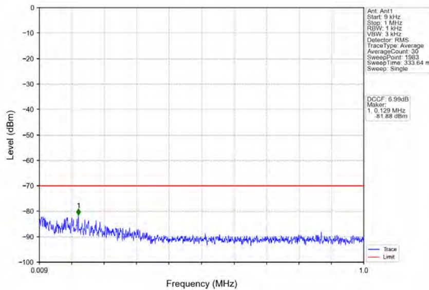
n78d_30kHz_MIMO_NTNV_15MHz_CP-OFDM QPSK_3557.52MHz_Inner_1RB_Left
