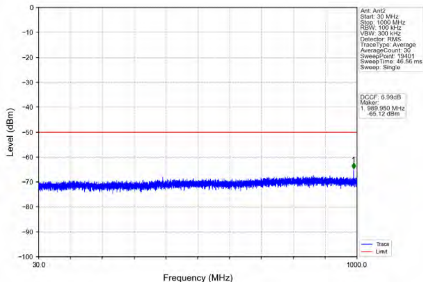
n78d_30kHz_MIMO_NTNV_15MHz_CP-OFDM QPSK_3557.52MHz_Inner_1RB_Left
