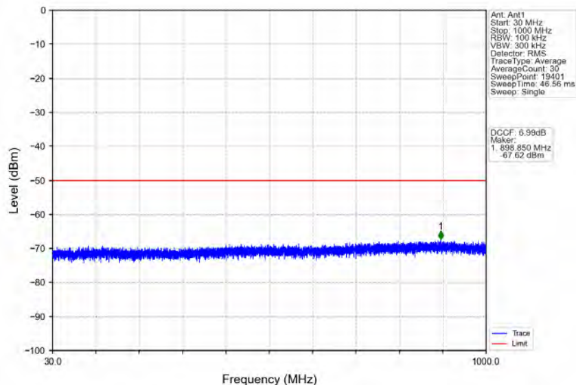
n78d_30kHz_MIMO_NTNV_10MHz_CP-OFDM QPSK_3694.98MHz_Inner_1RB_Right
