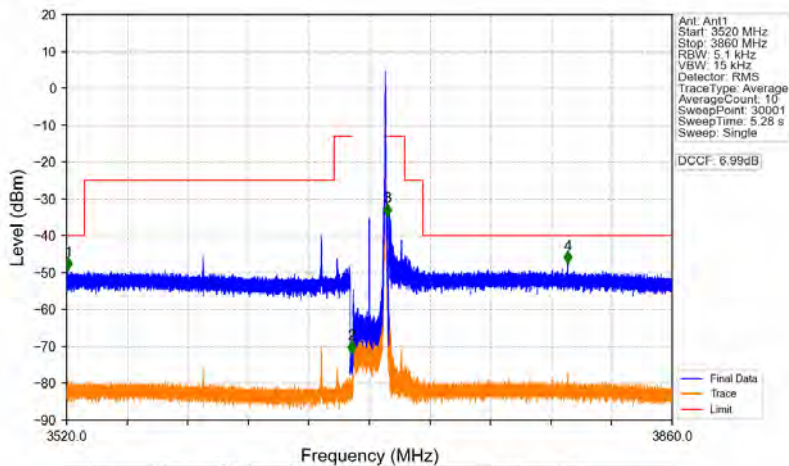
n78d_30kHz_MIMO_NTNV_20MHz_CP-OFDM QPSK_3690MHz_Edge_1RB_Right
