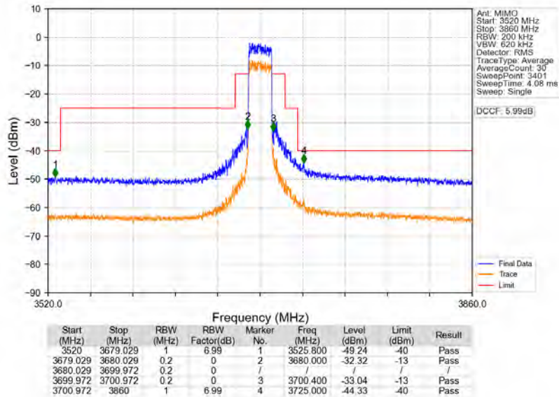
n78d_30kHz_MIMO_NTV_20MHz_CP-OFDM QPSK_3690MHz_Outer_Full
