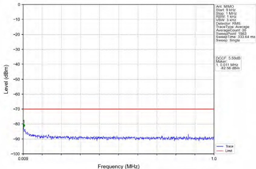
n78d_30kHz_MIMO_NTNV_30MHz_CP-OFDM QPSK_3565.02MHz_Outer_Full
