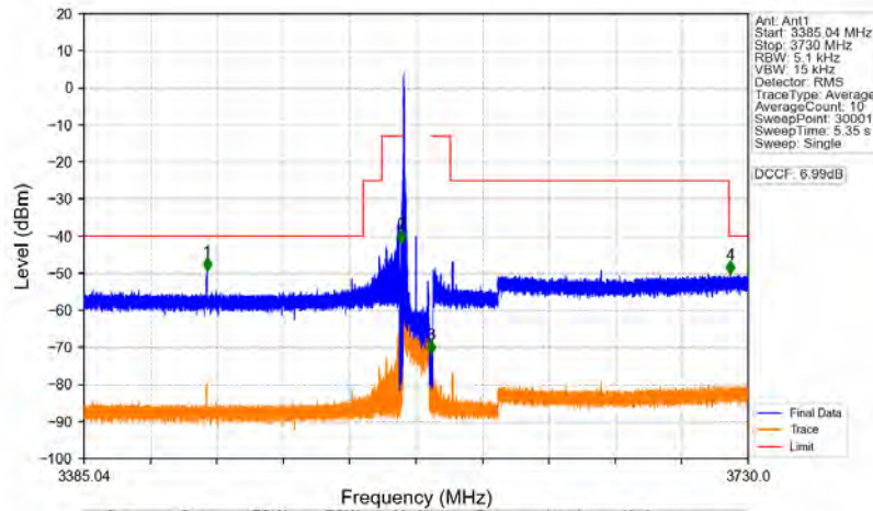
n78d_30kHz_MIMO_NTNV_15MHz_CP-OFDM QPSK_3557.52MHz_Inner_1RB_Left
