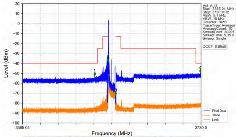
n78d_30kHz_MIMO_NTNV_15MHz_CP-OFDM_QPSK_3557.52MHz_Inner_1RB_Left
