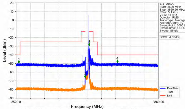
n78d_30kHz_MIMO_NTNV_10MHz_CP-OFDM_QPSK_3694.98MHz_Edge_1RB_Right
