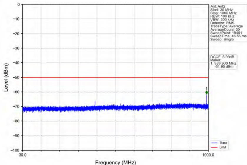
n78d_30kHz_MIMO_NTNV_30MHz_CP-OFDM QPSK_3565.02MHz_Edge_1RB_Left
