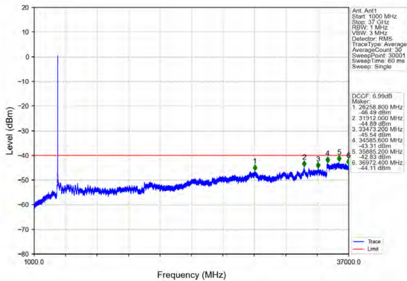
n78d_30kHz_MIMO_NTV_20MHz_CP-OFDM QPSK_3690MHz_Outer_Full
