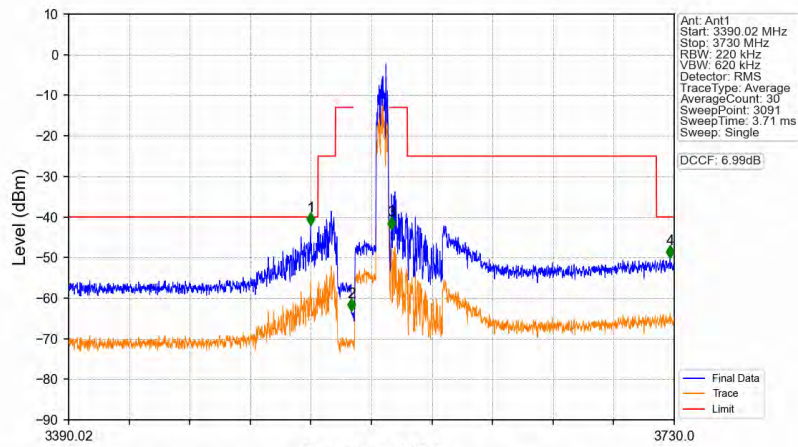
n78d_30kHz_MIMO_NTNV_20MHz_CP-OFDM QPSK_3560.01MHz_Outer_Full
