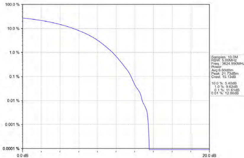
n78d_30kHz_MIMO_NTNV_90MHz_CP-OFDM_QPSK_3624.99MHz_Outer_Full
