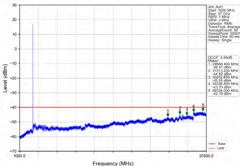
n78d_30kHz_MIMO_NTNV_10MHz_CP-OFDM_QPSK_3555MHz_Inner_1RB_Left
