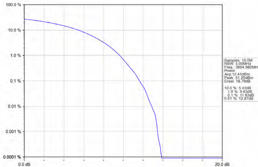
n78d_30kHz_MIMO_NTNV_10MHz_CP-OFDM 256 QAM_3694.98MHz_Outer_Full
