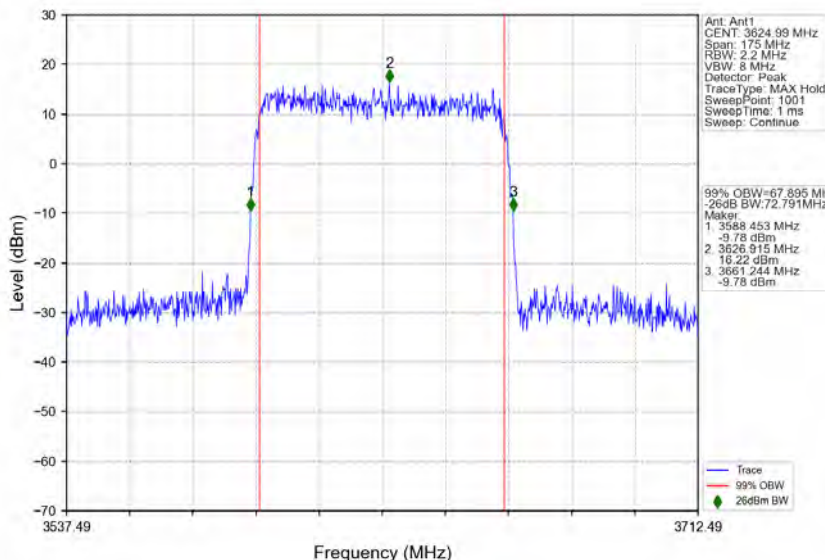
n78d_30kHz_MIMO_NTNV_70MHz_CP-OFDM_256_QAM_3624.99MHz_Outer_Full
