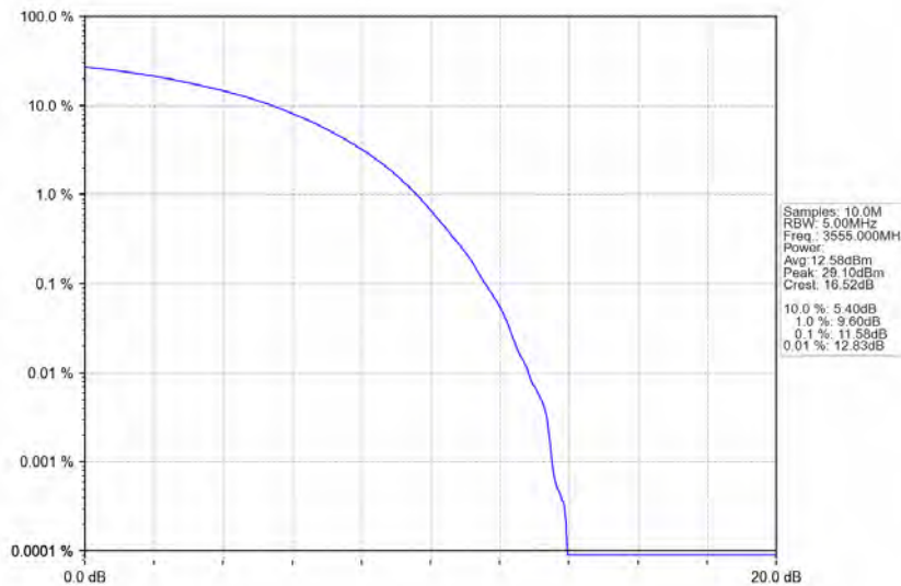
n78d_30kHz_MIMO_NTNV_10MHz_CP-OFDM_256_QAM_3555MHz_Outer_Full
