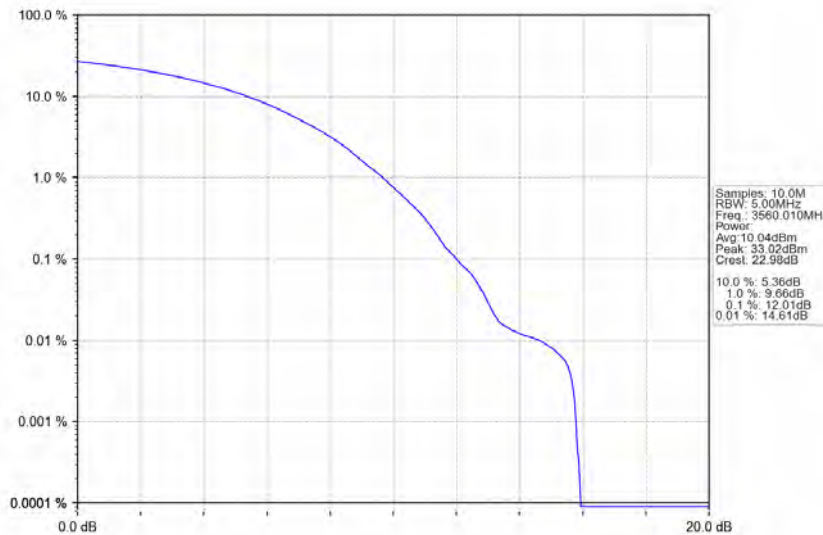
n78d_30kHz_MIMO_NTNV_20MHz_CP-OFDM 256 QAM_3560.01MHz_Outer_Full
