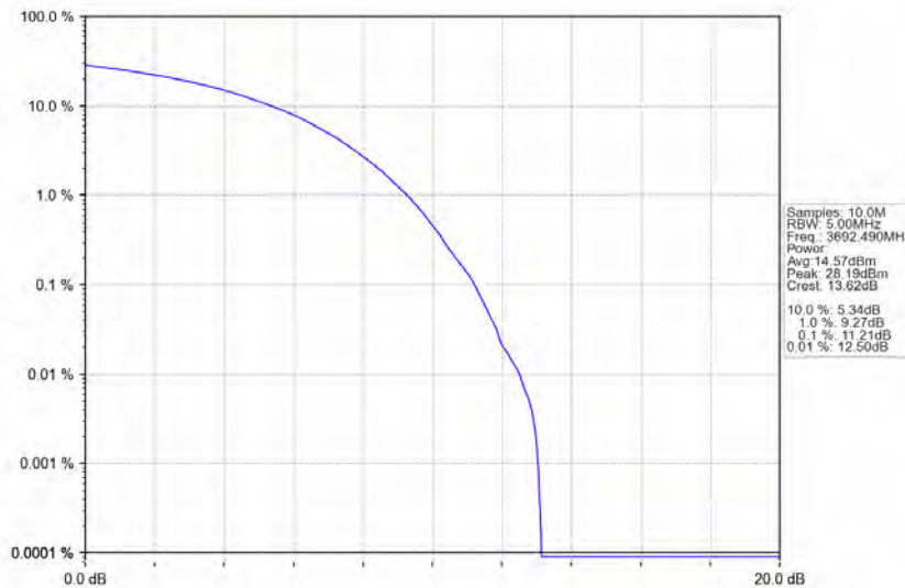
n78d_30kHz_MIMO_NTNV_15MHz_CP-OFDM QPSK_3692.49MHz_Outer_Full
