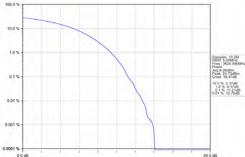
n78d_30kHz_MIMO_NTNV_60MHz_CP-OFDM 64 QAM_3624.99MHz_Outer_Full
