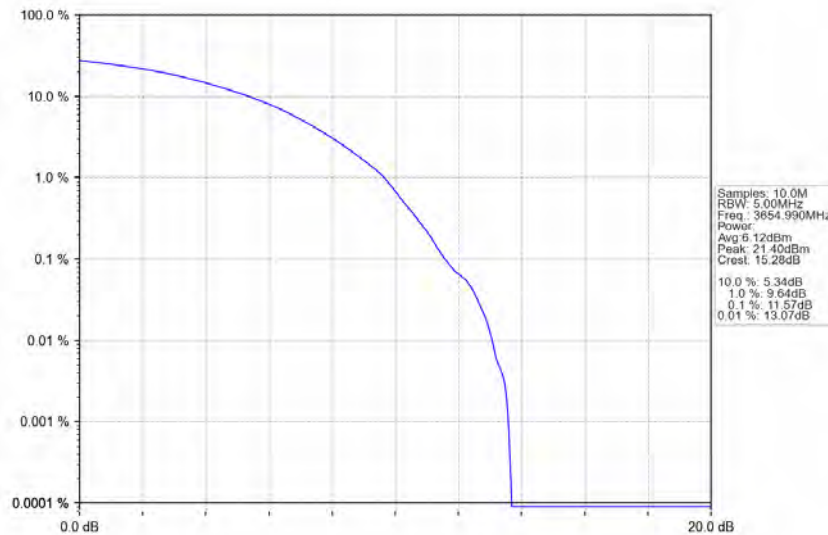
n78d_30kHz_MIMO_NTNV_90MHz_CP-OFDM 16 QAM_3654.99MHz_Outer_Full
