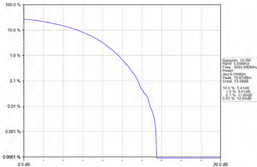
n78d_30kHz_MIMO_NTNV_90MHz_CP-OFDM_QPSK_3654.99MHz_Outer_Full
