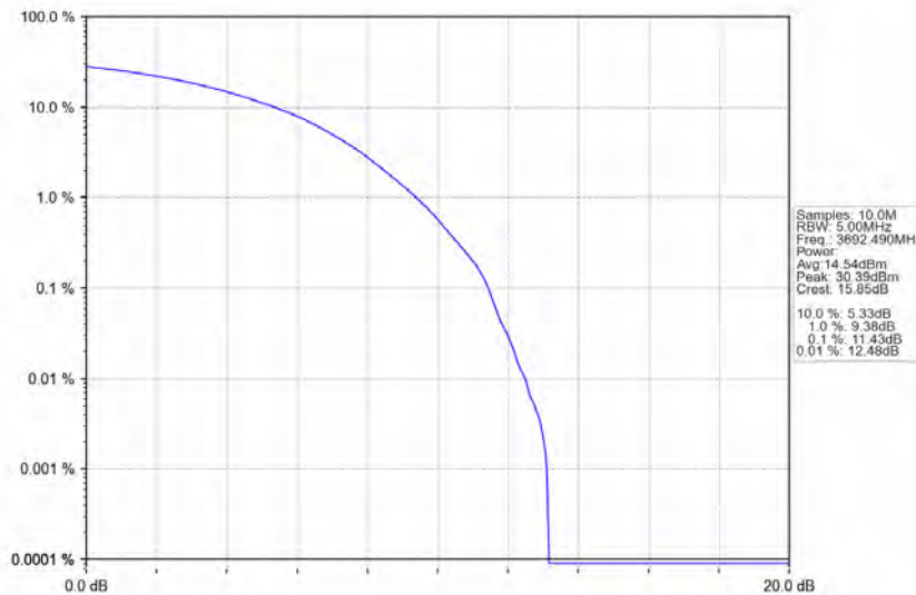
n78d_30kHz_MIMO_NTNV_15MHz_CP-OFDM 16 QAM_3692.49MHz_Outer_Full
