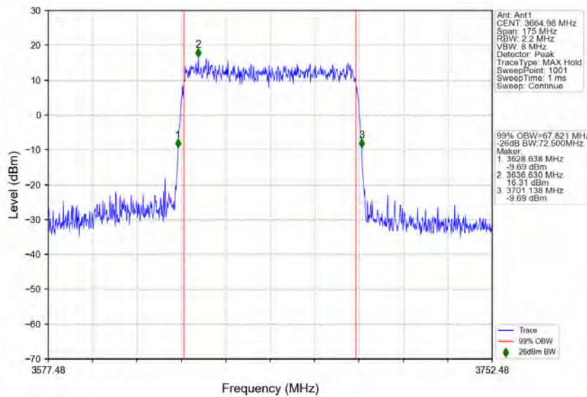
n78d_30kHz_MIMO_NTNV_70MHz_CP-OFDM 256 QAM_3664.98MHz_Outer_Full
