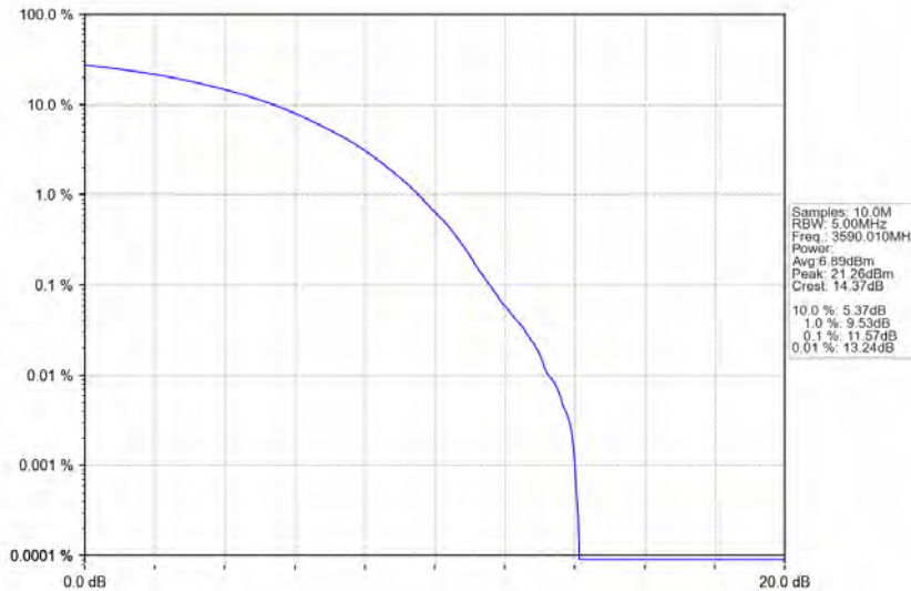
n78d_30kHz_MIMO_NTNV_80MHz_CP-OFDM_16_QAM_3590.01MHz_Outer_Full
