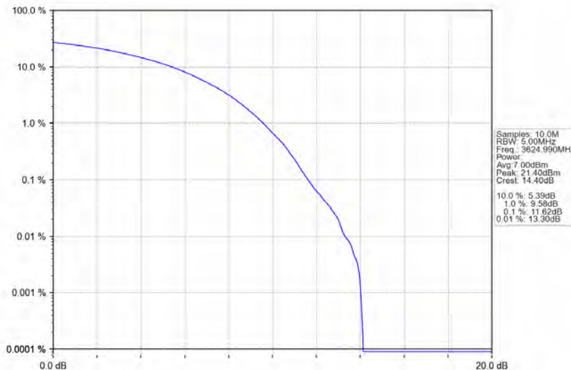
n78d_30kHz_MIMO_NTNV_80MHz_CP-OFDM_16_QAM_3624.99MHz_Outer_Full
