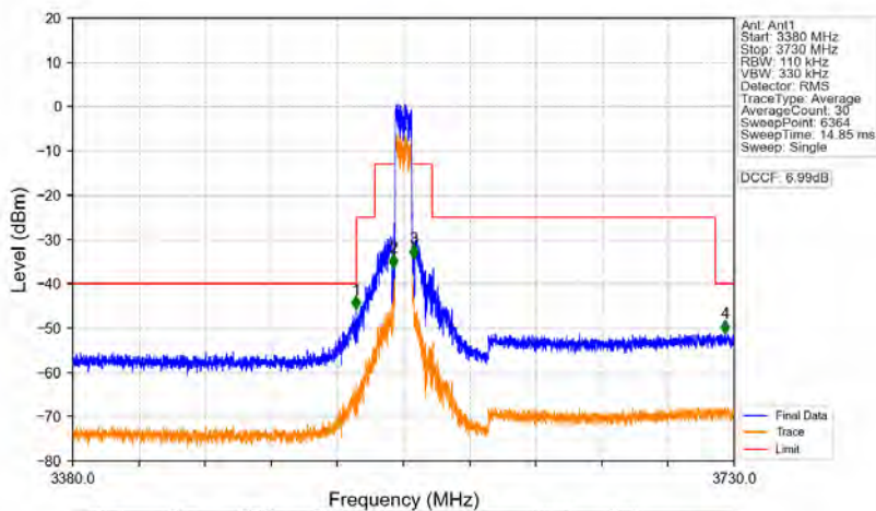
n78d_30kHz_MIMO_NTNV_10MHz_CP-OFDM QPSK_3555MHz_Outer_Full
