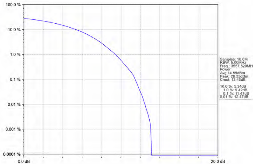
n78d_30kHz_MIMO_NTNV_15MHz_CP-OFDM_16_QAM_3557.52MHz_Outer_Full
