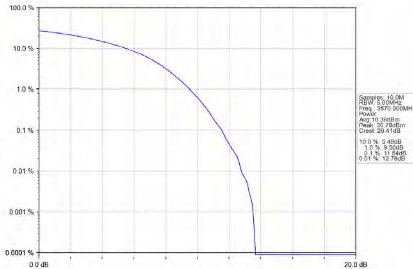
n78d_30kHz_MIMO_NTNV_40MHz_CP-OFDM_16_QAM_3570MHz_Outer_Full
