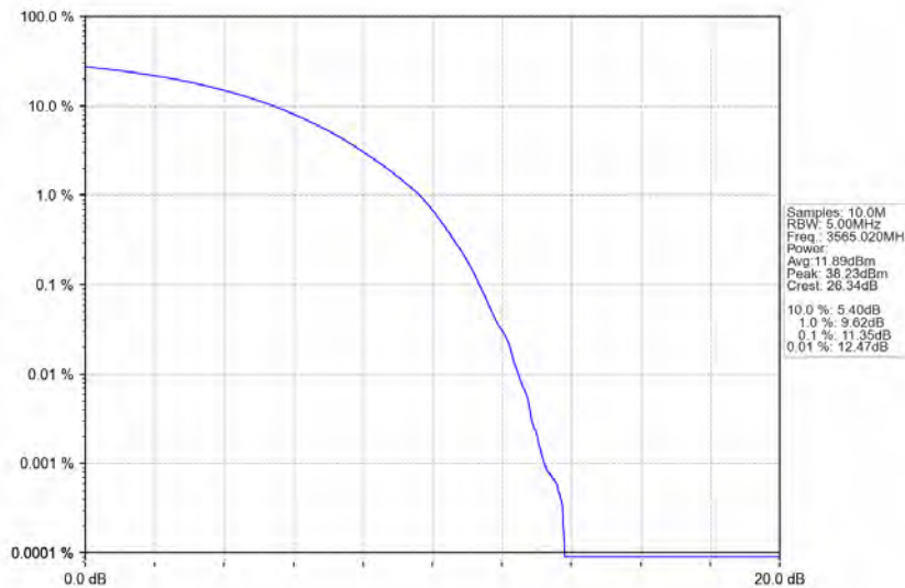
n78d_30kHz_MIMO_NTNV_30MHz_CP-OFDM_16_QAM_3565.02MHz_Outer_Full
