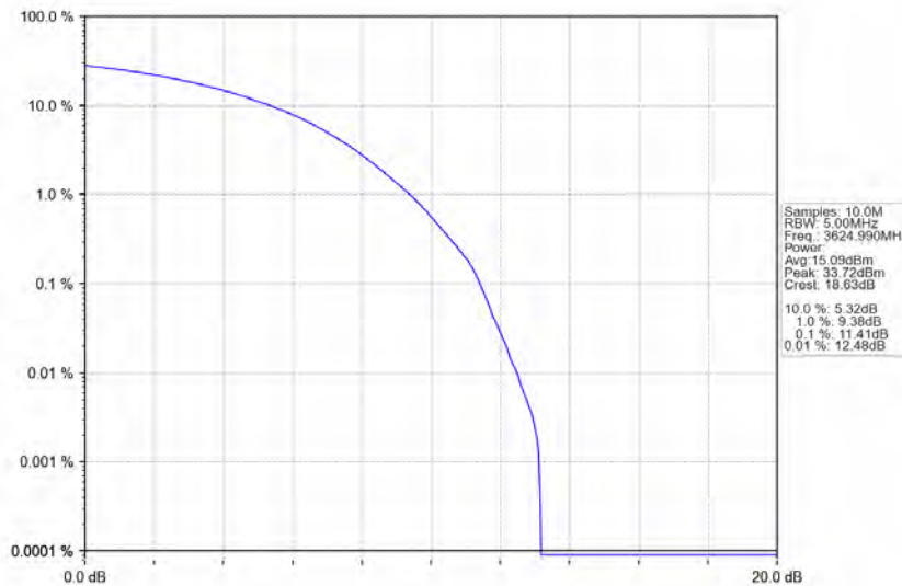
n78d_30kHz_MIMO_NTNV_15MHz_CP-OFDM_16_QAM_3624.99MHz_Outer_Full
