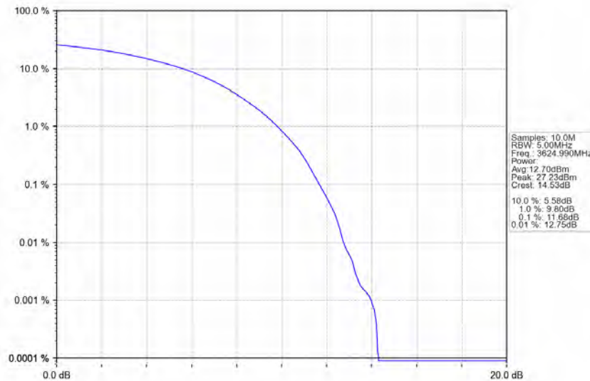
n78d_30kHz_MIMO_NTNV_20MHz_CP-OFDM 64 QAM_3624.99MHz_Outer_Full
