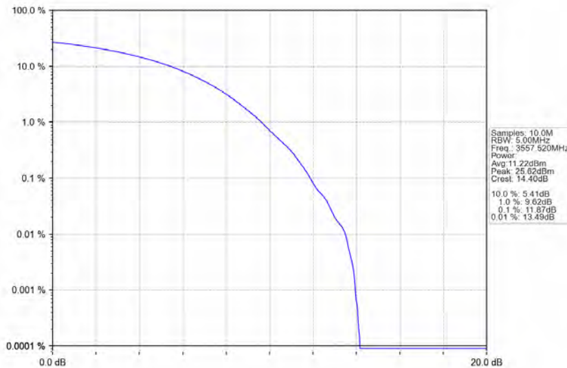
n78d_30kHz_MIMO_NTNV_15MHz_CP-OFDM 256 QAM_3557.52MHz_Outer_Full
