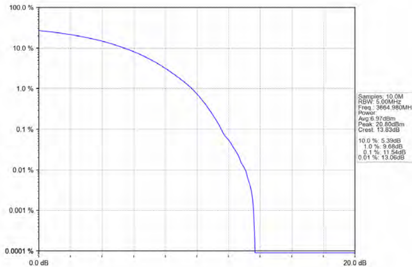
n78d_30kHz_MIMO_NTNV_70MHz_CP-OFDM 16 QAM_3664.98MHz_Outer_Full
