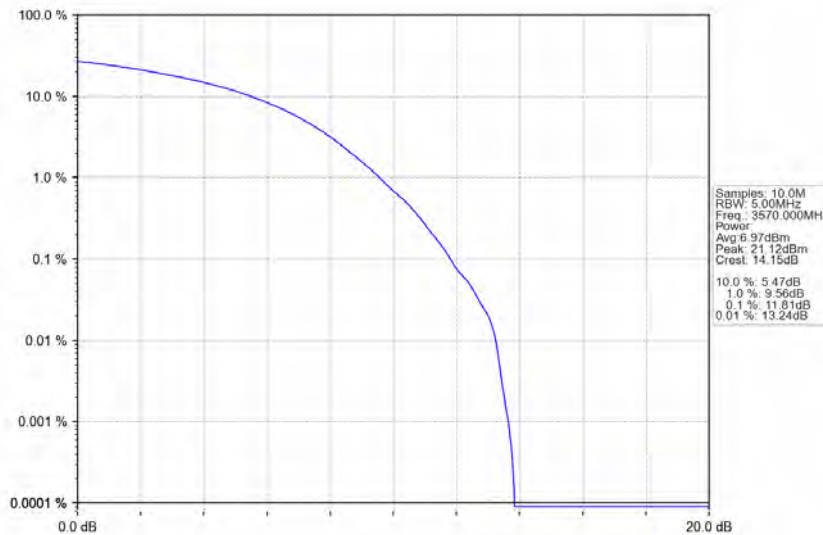
n78d_30kHz_MIMO_NTNV_40MHz_CP-OFDM_256_QAM_3570MHz_Outer_Full
