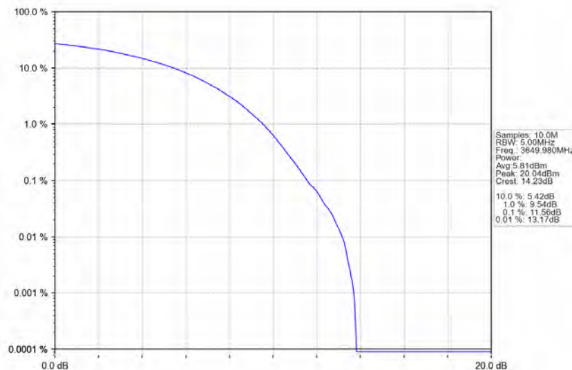
n78d_30kHz_MIMO_NTNV_100MHz_CP-OFDM QPSK_3649.98MHz_Outer_Full
