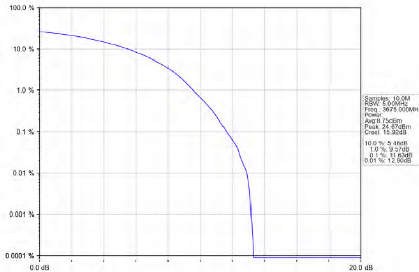
n78d_30kHz_MIMO_NTNV_50MHz_CP-OFDM 16 QAM_3675MHz_Outer_Full
