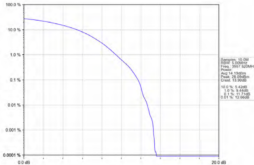
n78d_30kHz_MIMO_NTNV_15MHz_CP-OFDM 64 QAM_3557.52MHz_Outer_Full
