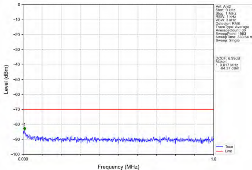
n78d_30kHz_MIMO_NTNV_10MHz_CP-OFDM QPSK_3555MHz_Outer_Full
