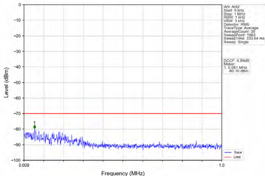
n78d_30kHz_MIMO_NTNV_10MHz_CP-OFDM QPSK_3555MHz_Edge_1RB_Left
