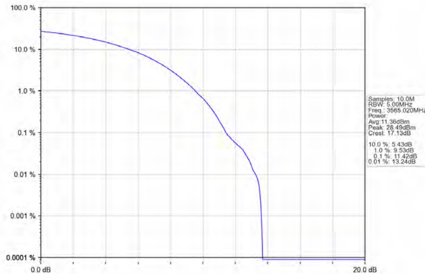
n78d_30kHz_MIMO_NTNV_30MHz_CP-OFDM 64 QAM_3565.02MHz_Outer_Full
