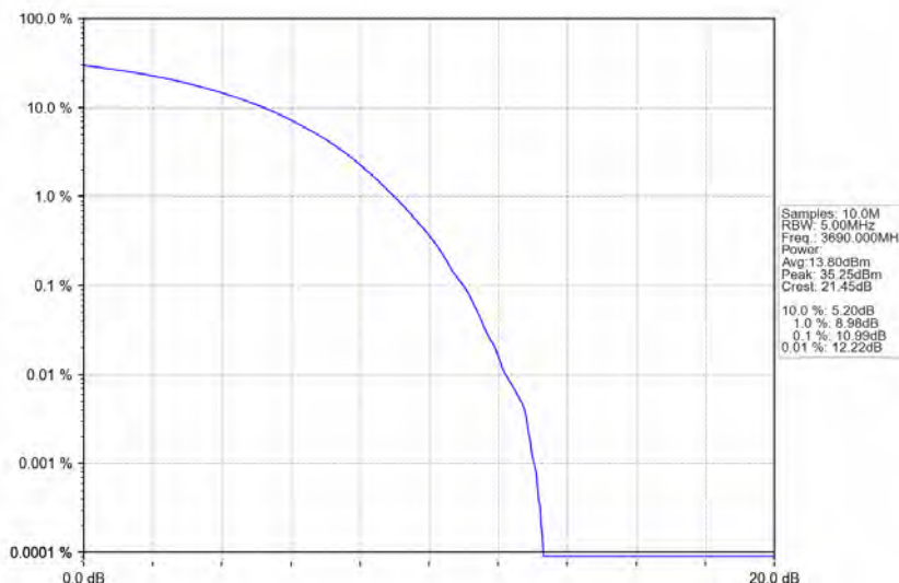
n78d_30kHz_MIMO_NTNV_20MHz_CP-OFDM 16 QAM_3690MHz_Outer_Full
