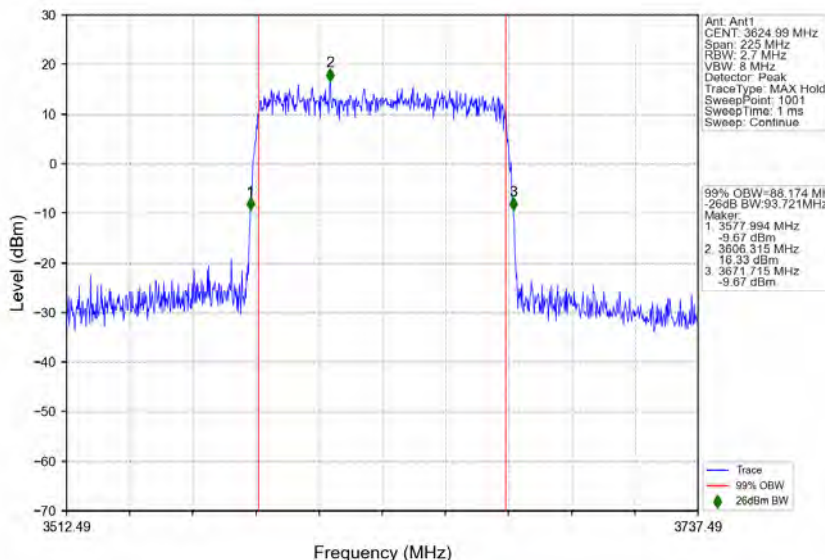
n78d_30kHz_MIMO_NTNV_90MHz_CP-OFDM_256_QAM_3624.99MHz_Outer_Full
