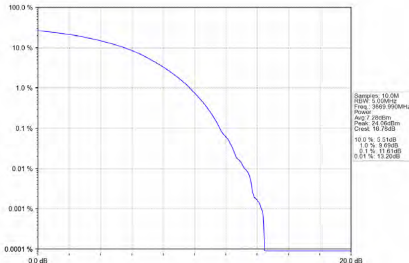
n78d_30kHz_MIMO_NTNV_60MHz_CP-OFDM 64 QAM_3669.99MHz_Outer_Full
