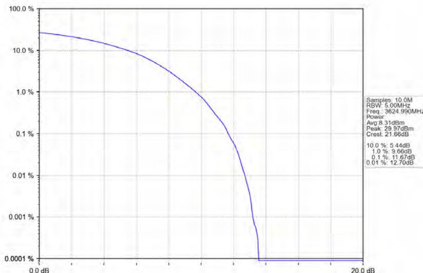
n78d_30kHz_MIMO_NTNV_30MHz_CP-OFDM 256 QAM_3624.99MHz_Outer_Full
