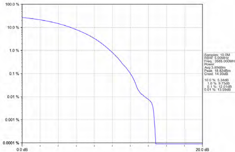
n78d_30kHz_MIMO_NTNV_70MHz_CP-OFDM_256_QAM_3585MHz_Outer_Full
