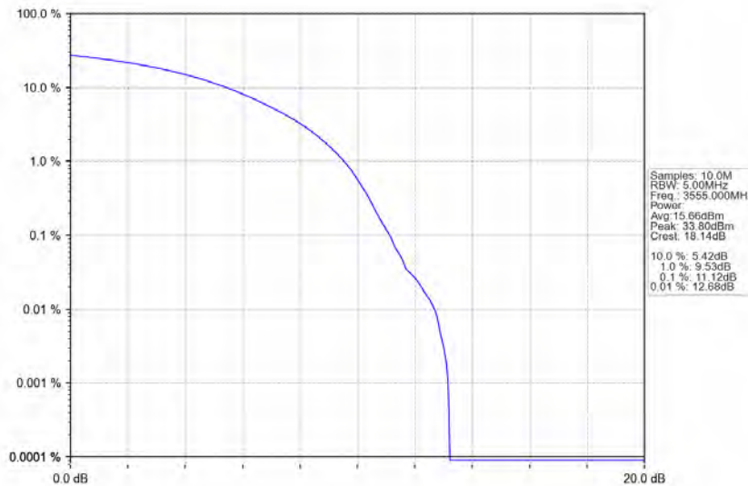
n78d_30kHz_MIMO_NTNV_10MHz_CP-OFDM 64 QAM_3555MHz_Outer_Full
