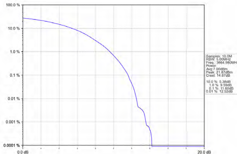
n78d_30kHz_MIMO_NTNV_70MHz_CP-OFDM QPSK_3664.98MHz_Outer_Full
