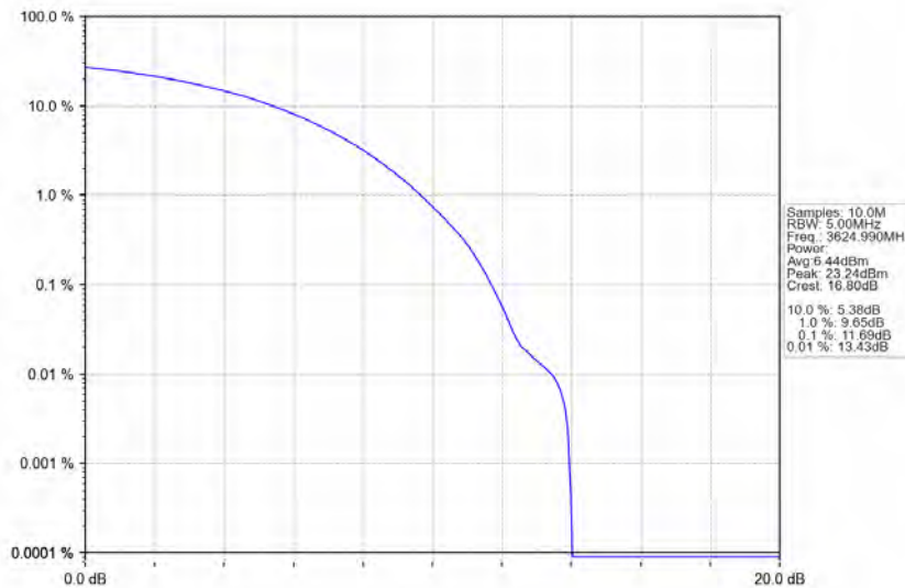
n78d_30kHz_MIMO_NTNV_80MHz_CP-OFDM 64 QAM_3624.99MHz_Outer_Full
