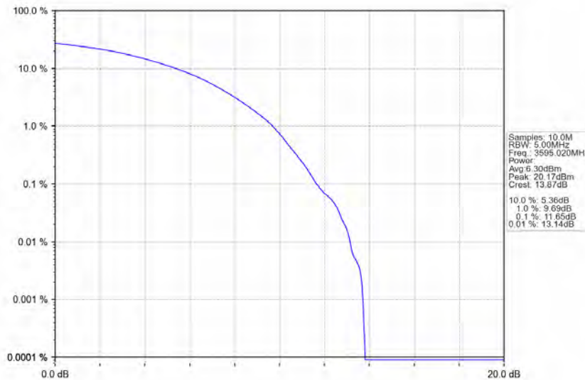
n78d_30kHz_MIMO_NTNV_90MHz_CP-OFDM_16_QAM_3595.02MHz_Outer_Full
