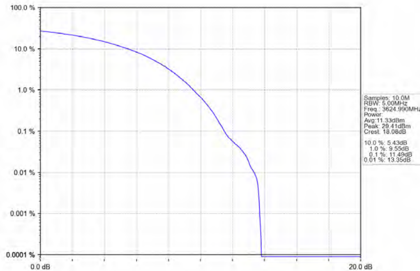
n78d_30kHz_MIMO_NTNV_30MHz_CP-OFDM 64 QAM_3624.99MHz_Outer_Full
