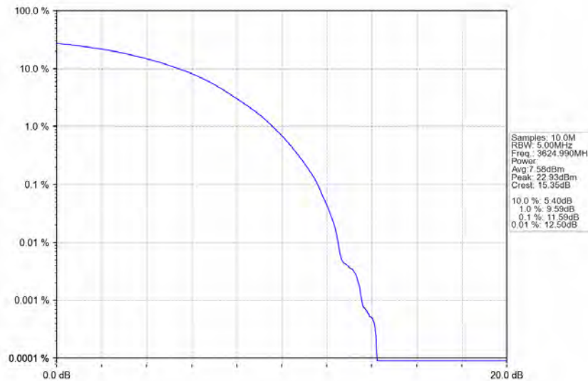
n78d_30kHz_MIMO_NTNV_70MHz_CP-OFDM QPSK_3624.99MHz_Outer_Full
