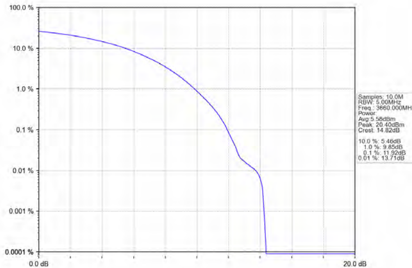
n78d_30kHz_MIMO_NTNV_80MHz_CP-OFDM 64 QAM_3660MHz_Outer_Full
