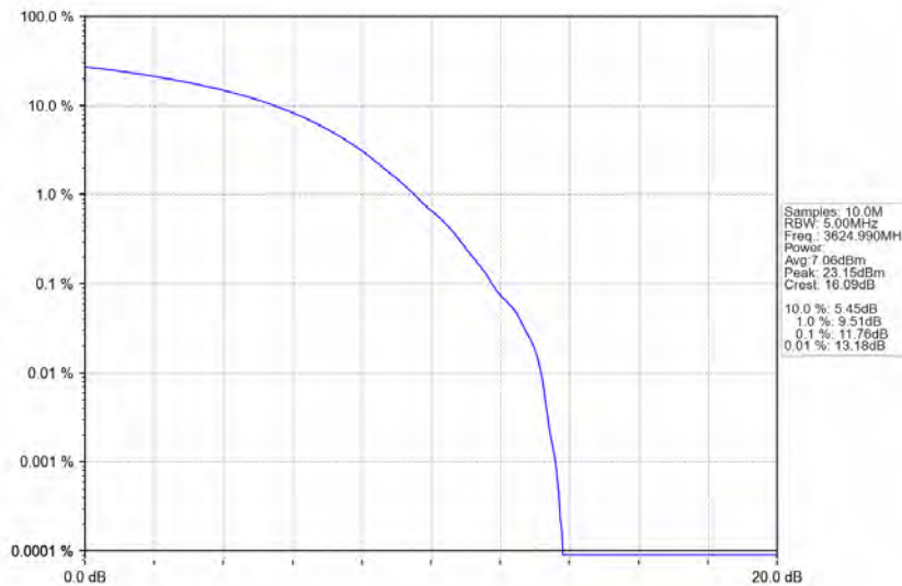
n78d_30kHz_MIMO_NTNV_40MHz_CP-OFDM_256_QAM_3624.99MHz_Outer_Full
