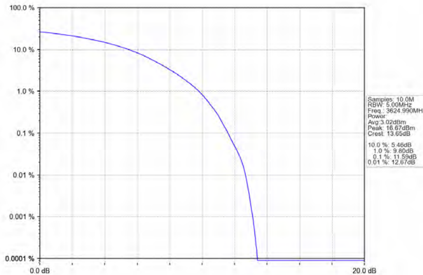
n78d_30kHz_MIMO_NTNV_90MHz_CP-OFDM 256 QAM_3624.99MHz_Outer_Full
