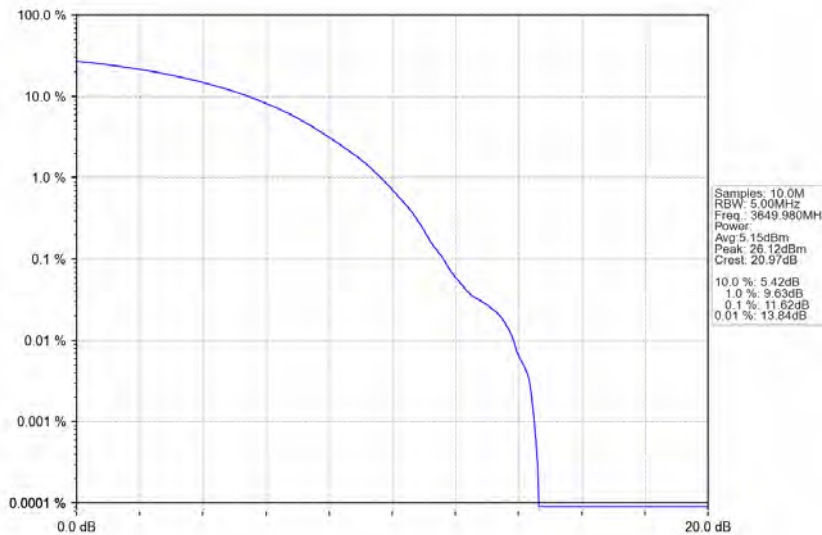
n78d_30kHz_MIMO_NTNV_100MHz_CP-OFDM 64 QAM_3649.98MHz_Outer_Full
