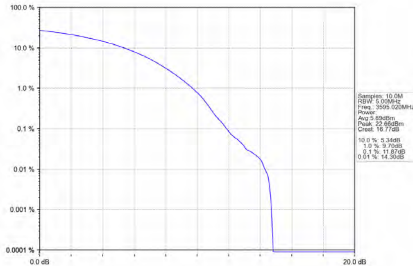
n78d_30kHz_MIMO_NTNV_90MHz_CP-OFDM 64 QAM_3595.02MHz_Outer_Full
