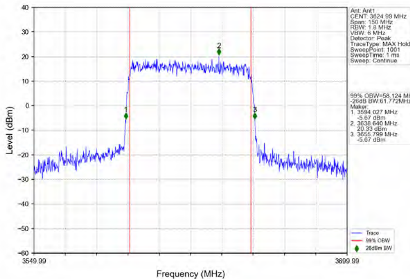
n78d_30kHz_MIMO_NTNV_60MHz_CP-OFDM 16 QAM_3624.99MHz_Outer_Full
