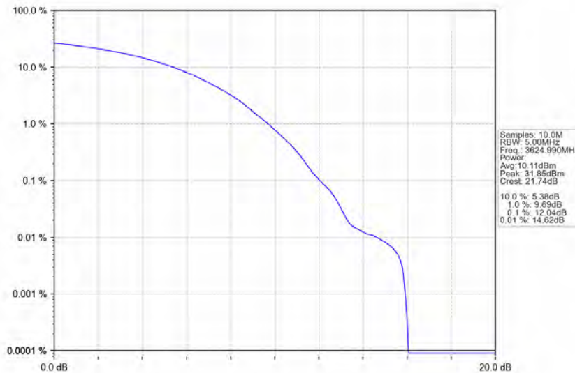
n78d_30kHz_MIMO_NTNV_20MHz_CP-OFDM 256 QAM_3624.99MHz_Outer_Full
