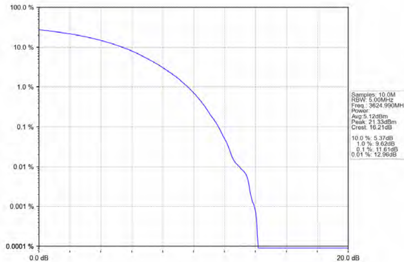
n78d_30kHz_MIMO_NTNV_60MHz_CP-OFDM_256_QAM_3624.99MHz_Outer_Full
