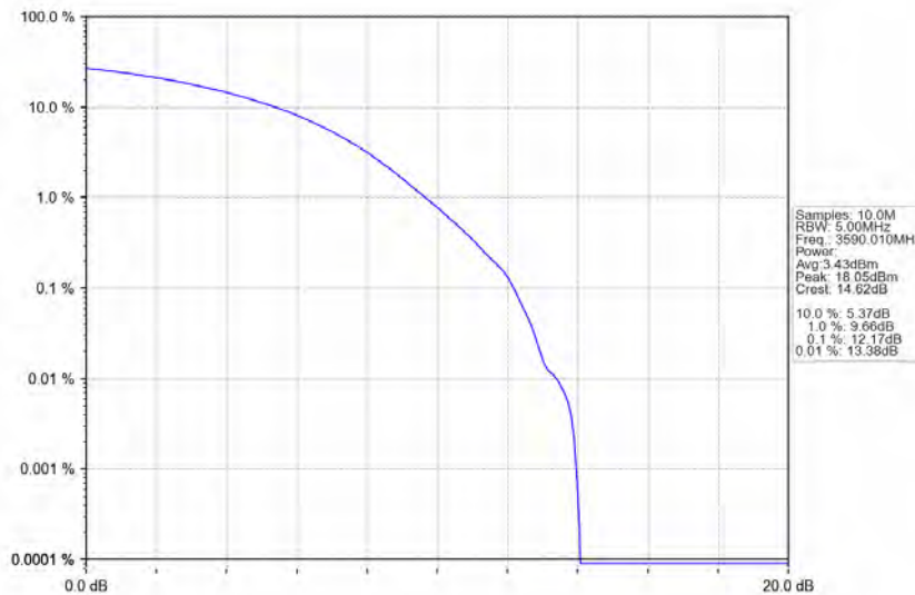
n78d_30kHz_MIMO_NTNV_80MHz_CP-OFDM_256_QAM_3590.01MHz_Outer_Full
