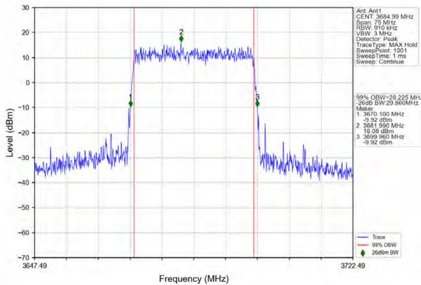
n78d_30kHz_MIMO_NTNV_30MHz_CP-OFDM 256 QAM_3684.99MHz_Outer_Full
