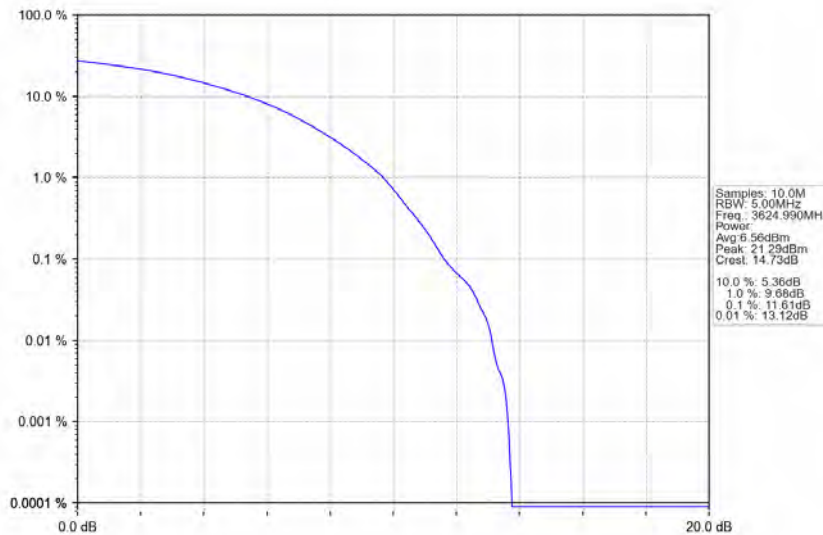
n78d_30kHz_MIMO_NTNV_90MHz_CP-OFDM_16_QAM_3624.99MHz_Outer_Full
