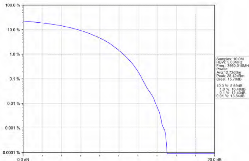
n78d_30kHz_MIMO_NTNV_20MHz_CP-OFDM 64 QAM_3560.01MHz_Outer_Full
