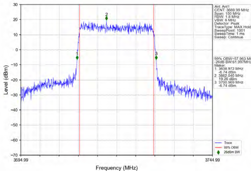
n78d_30kHz_MIMO_NTNV_60MHz_CP-OFDM QPSK_3669.99MHz_Outer_Full
