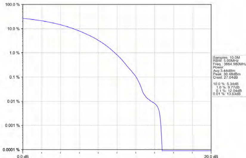
n78d_30kHz_MIMO_NTNV_70MHz_CP-OFDM 256 QAM_3664.98MHz_Outer_Full
