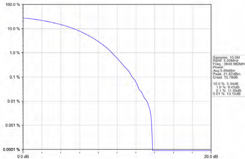
n78d_30kHz_MIMO_NTNV_100MHz_CP-OFDM 16 QAM_3649.98MHz_Outer_Full
