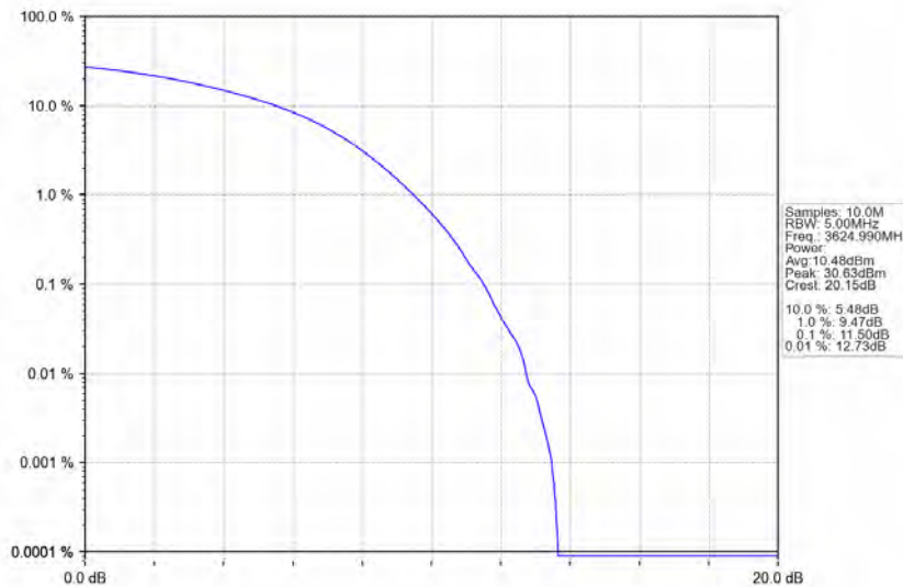
n78d_30kHz_MIMO_NTNV_40MHz_CP-OFDM_16_QAM_3624.99MHz_Outer_Full
