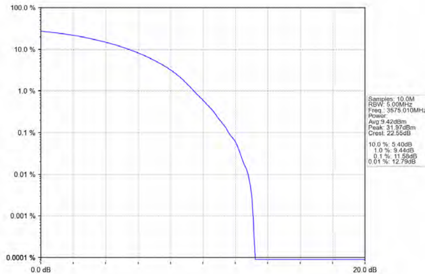
n78d_30kHz_MIMO_NTNV_50MHz_CP-OFDM_16_QAM_3575.01MHz_Outer_Full
