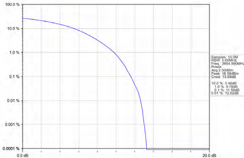
n78d_30kHz_MIMO_NTNV_90MHz_CP-OFDM 256 QAM_3654.99MHz_Outer_Full
