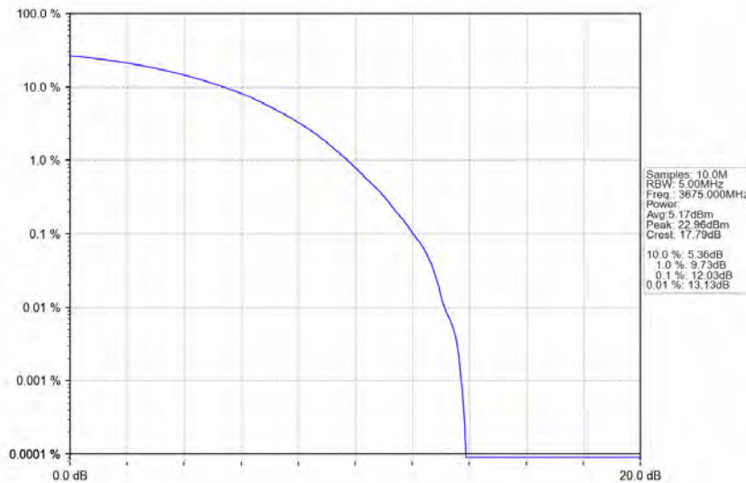
n78d_30kHz_MIMO_NTNV_50MHz_CP-OFDM_256_QAM_3675MHz_Outer_Full
