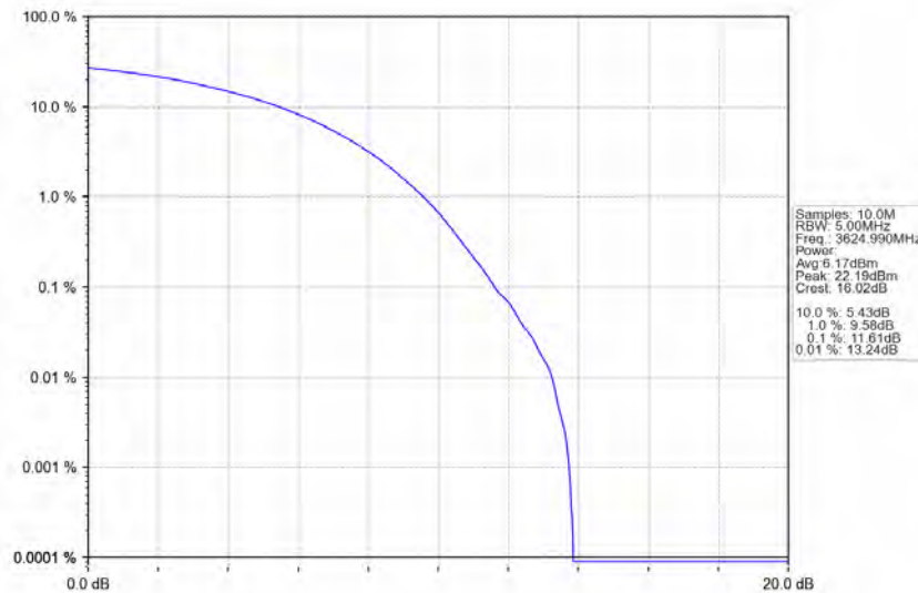
n78d_30kHz_MIMO_NTNV_100MHz_CP-OFDM QPSK_3624.99MHz_Outer_Full
