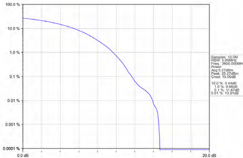
n78d_30kHz_MIMO_NTNV_100MHz_CP-OFDM 64 QAM_3600MHz_Outer_Full
