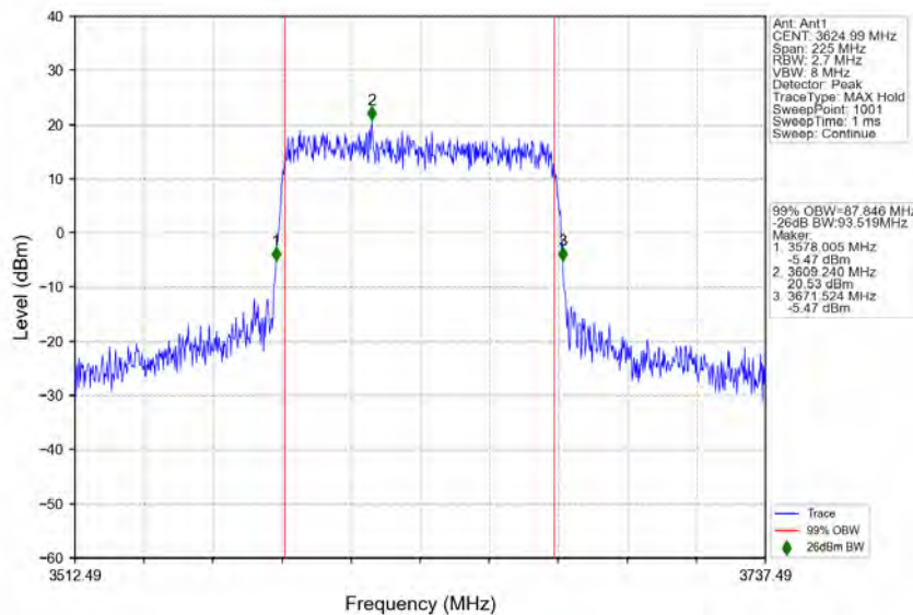
n78d_30kHz_MIMO_NTNV_90MHz_CP-OFDM 16 QAM_3624.99MHz_Outer_Full
