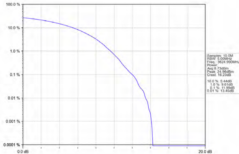
n78d_30kHz_MIMO_NTNV_50MHz_CP-OFDM 64 QAM_3624.99MHz_Outer_Full
