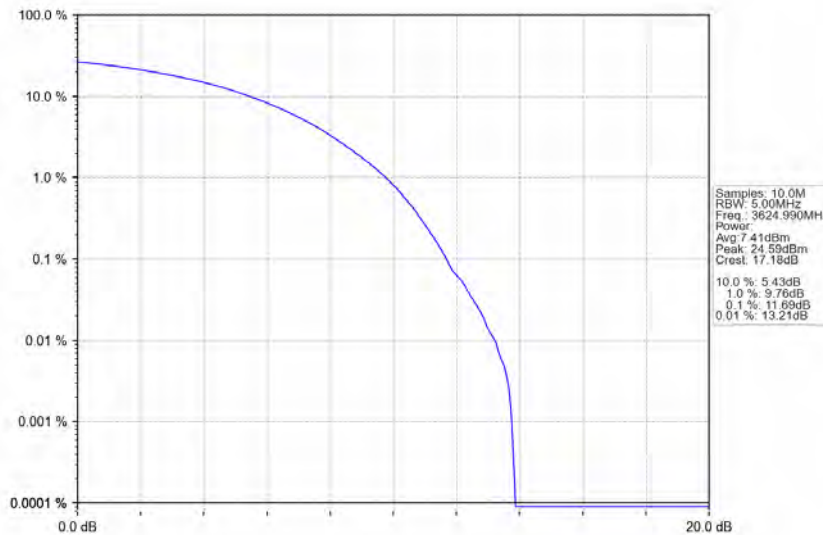
n78d_30kHz_MIMO_NTNV_70MHz_CP-OFDM 16 QAM_3624.99MHz_Outer_Full
