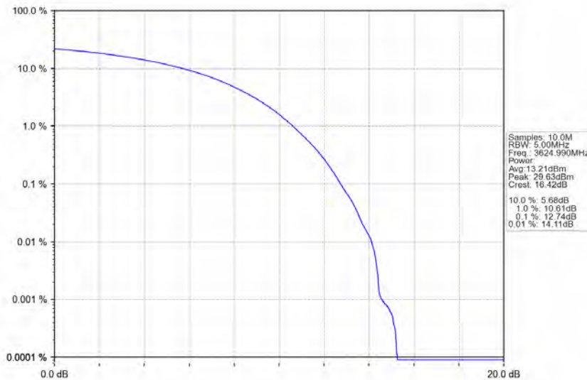
n78d_30kHz_MIMO_NTNV_20MHz_CP-OFDM 16 QAM_3624.99MHz_Outer_Full
