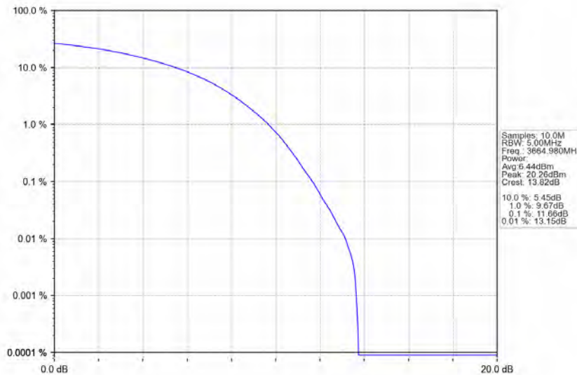
n78d_30kHz_MIMO_NTNV_70MHz_CP-OFDM_64_QAM_3664.98MHz_Outer_Full
