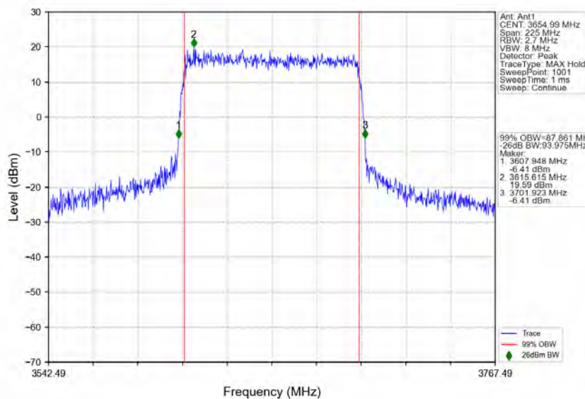
n78d_30kHz_MIMO_NTNV_90MHz_CP-OFDM_QPSK_3654.99MHz_Outer_Full
