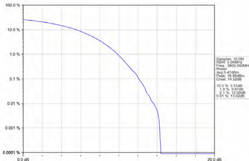
n78d_30kHz_MIMO_NTNV_100MHz_CP-OFDM_16 QAM_3600MHz_Outer_Full
