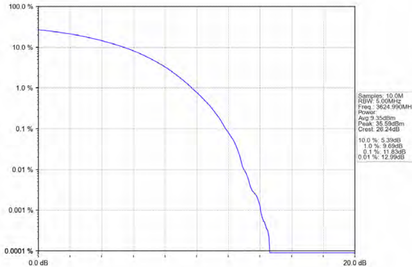
n78d_30kHz_MIMO_NTNV_50MHz_CP-OFDM QPSK_3624.99MHz_Outer_Full
