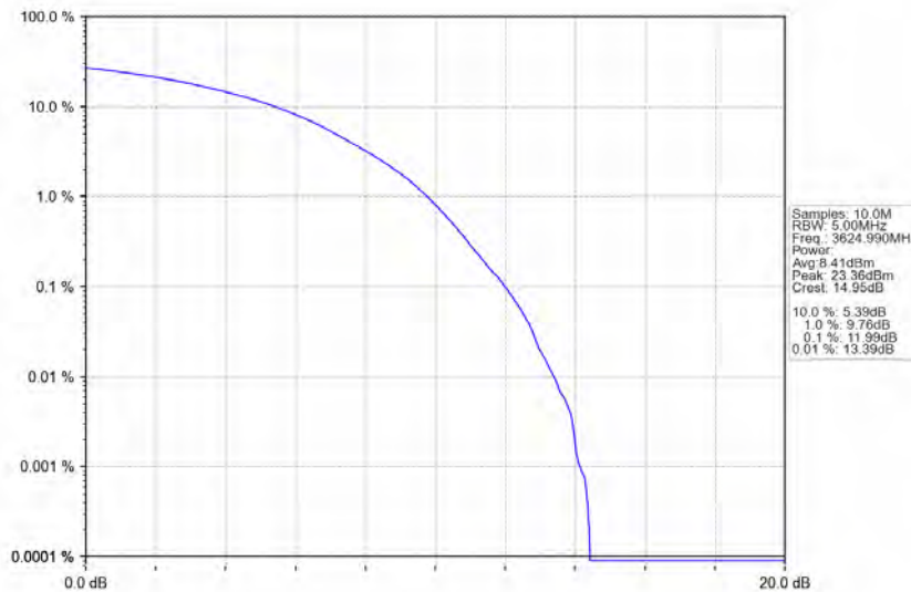
n78d_30kHz_MIMO_NTNV_60MHz_CP-OFDM_16_QAM_3624.99MHz_Outer_Full
