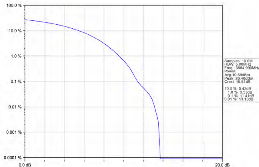
n78d_30kHz_MIMO_NTNV_30MHz_CP-OFDM 64 QAM_3684.99MHz_Outer_Full
