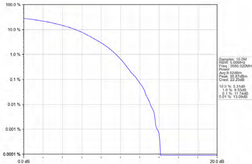
n78d_30kHz_MIMO_NTNV_60MHz_CP-OFDM_16_QAM_3580.02MHz_Outer_Full
