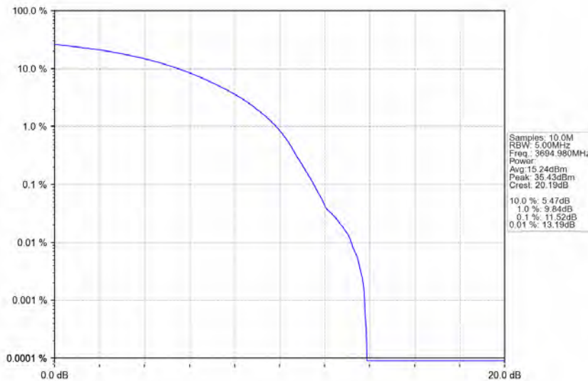
n78d_30kHz_MIMO_NTNV_10MHz_CP-OFDM 64 QAM_3694.98MHz_Outer_Full
