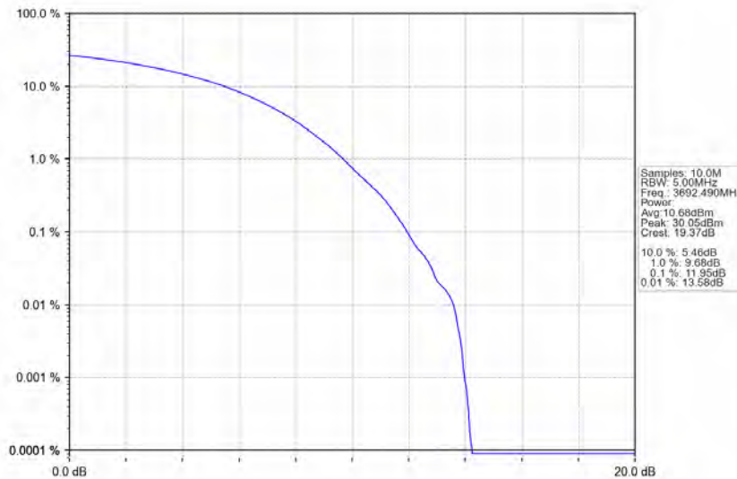
n78d_30kHz_MIMO_NTNV_15MHz_CP-OFDM 256 QAM_3692.49MHz_Outer_Full
