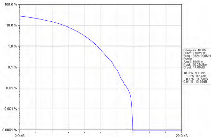
n78d_30kHz_MIMO_NTNV_100MHz_CP-OFDM_16 QAM_3624.99MHz_Outer_Full
