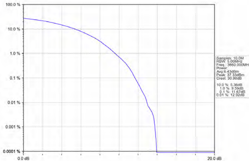
n78d_30kHz_MIMO_NTNV_80MHz_CP-OFDM QPSK_3660MHz_Outer_Full
