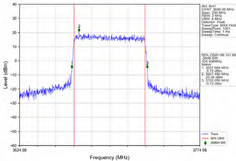
n78d_30kHz_MIMO_NTNV_100MHz_CP-OFDM QPSK_3649.98MHz_Outer_Full
