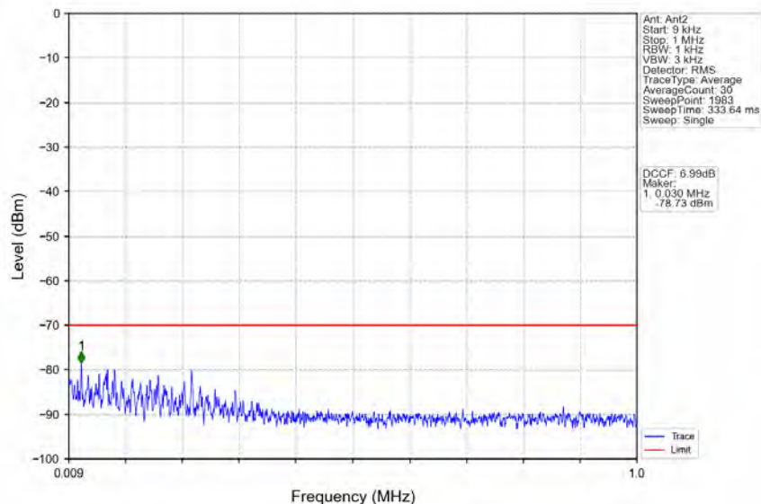
n78d_30kHz_MIMO_NTNV_10MHz_CP-OFDM QPSK_3555MHz_Inner_1RB_Left
