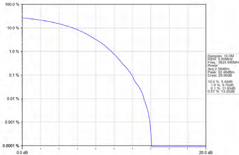
n78d_30kHz_MIMO_NTNV_100MHz_CP-OFDM_256_QAM_3624.99MHz_Outer_Full
