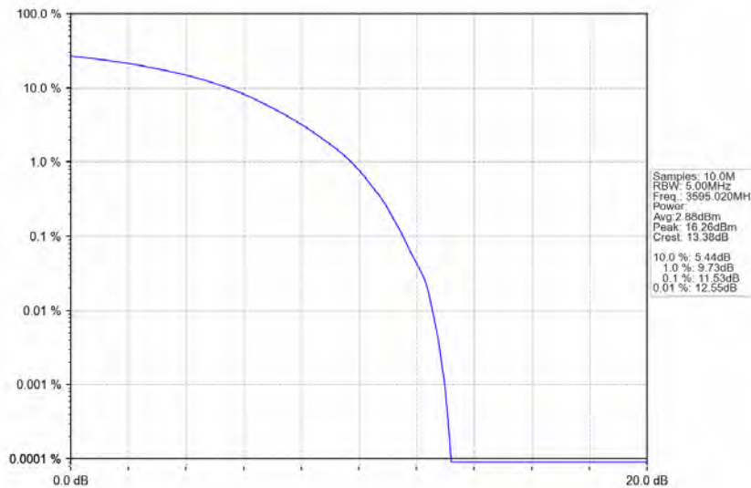
n78d_30kHz_MIMO_NTNV_90MHz_CP-OFDM 256 QAM_3595.02MHz_Outer_Full
