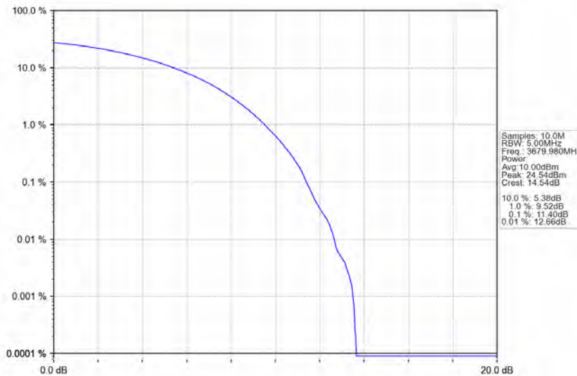
n78d_30kHz_MIMO_NTNV_40MHz_CP-OFDM_QPSK_3679.98MHz_Outer_Full
