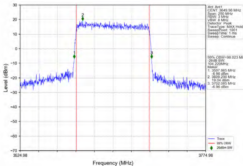
n78d_30kHz_MIMO_NTNV_100MHz_CP-OFDM 64 QAM_3649.98MHz_Outer_Full
