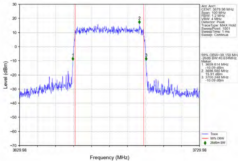
n78d_30kHz_MIMO_NTNV_40MHz_CP-OFDM 256 QAM_3679.98MHz_Outer_Full
