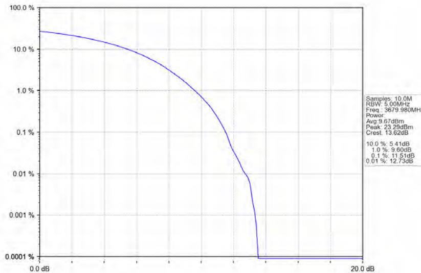
n78d_30kHz_MIMO_NTNV_40MHz_CP-OFDM 64 QAM_3679.98MHz_Outer_Full
