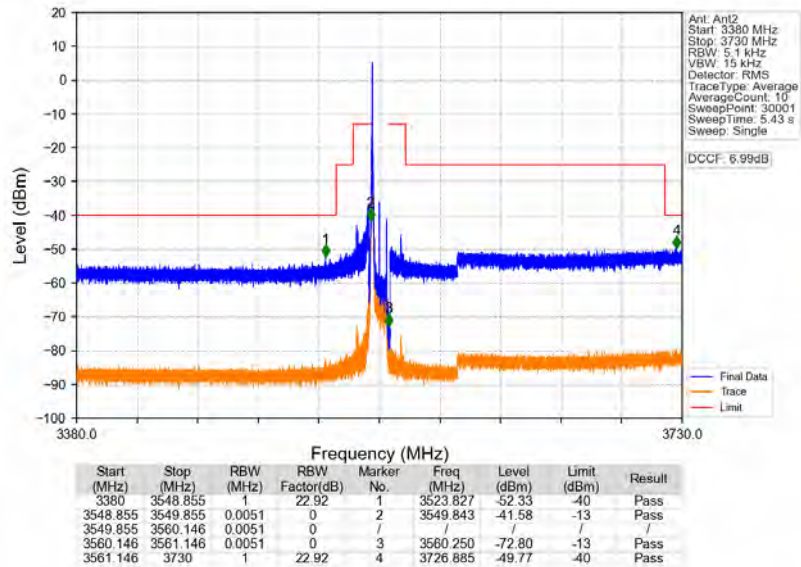
n78d_30kHz_MIMO_NTNV_10MHz_CP-OFDM QPSK_3555MHz_Edge_1RB_Left
