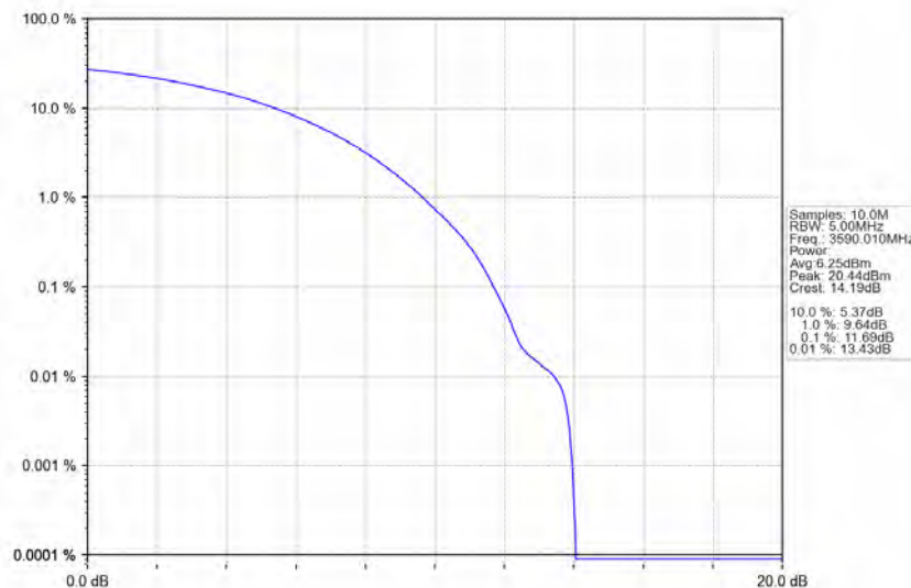
n78d_30kHz_MIMO_NTNV_80MHz_CP-OFDM 64 QAM_3590.01MHz_Outer_Full
