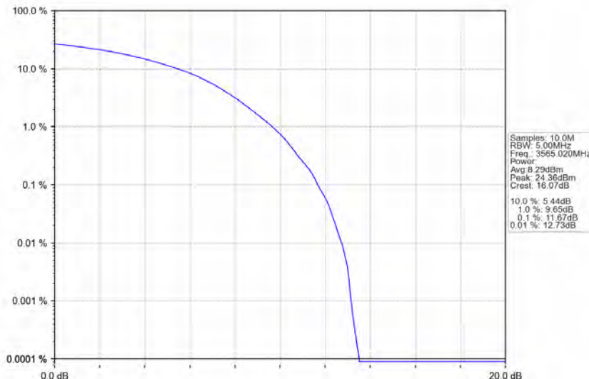
n78d_30kHz_MIMO_NTNV_30MHz_CP-OFDM 256 QAM_3565.02MHz_Outer_Full
