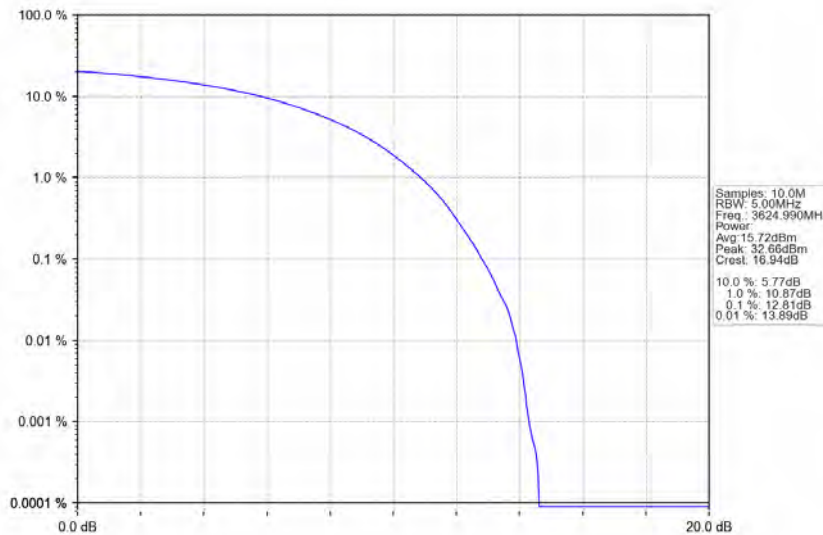
n78d_30kHz_MIMO_NTNV_10MHz_CP-OFDM QPSK_3624.99MHz_Outer_Full
