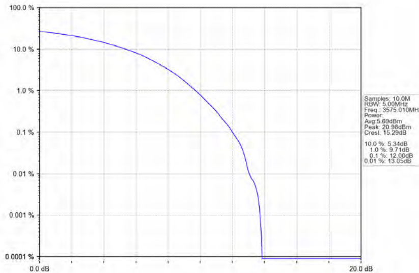
n78d_30kHz_MIMO_NTNV_50MHz_CP-OFDM 256 QAM_3575.01MHz_Outer_Full
