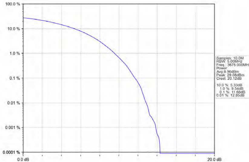
n78d_30kHz_MIMO_NTNV_50MHz_CP-OFDM QPSK_3675MHz_Outer_Full
