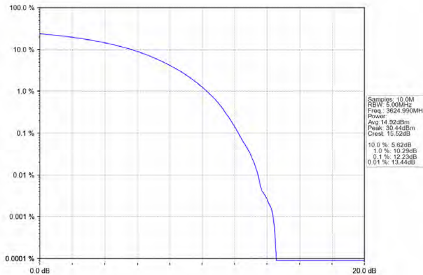
n78d_30kHz_MIMO_NTNV_15MHz_CP-OFDM QPSK_3624.99MHz_Outer_Full
