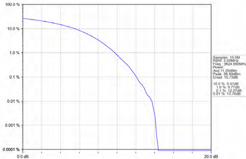
n78d_30kHz_MIMO_NTNV_15MHz_CP-OFDM 256 QAM_3624.99MHz_Outer_Full
