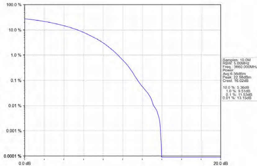
n78d_30kHz_MIMO_NTNV_80MHz_CP-OFDM 16 QAM_3660MHz_Outer_Full
