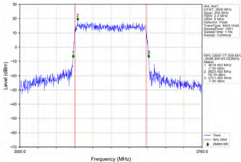
n78d_30kHz_MIMO_NTNV_80MHz_CP-OFDM 64 QAM_3660MHz_Outer_Full
