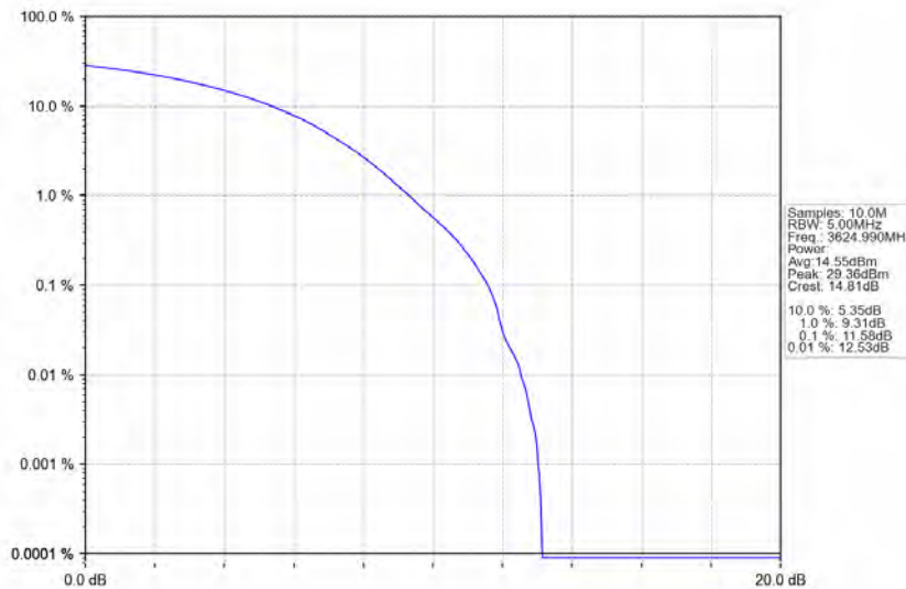
n78d_30kHz_MIMO_NTNV_15MHz_CP-OFDM 64 QAM_3624.99MHz_Outer_Full
