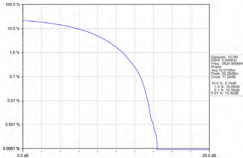
n78d_30kHz_MIMO_NTNV_10MHz_CP-OFDM 16 QAM_3624.99MHz_Outer_Full
