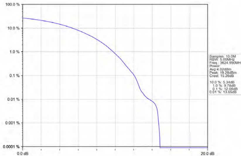
n78d_30kHz_MIMO_NTNV_70MHz_CP-OFDM_256_QAM_3624.99MHz_Outer_Full
