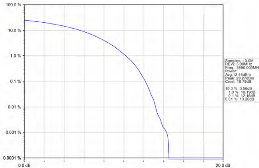
n78d_30kHz_MIMO_NTNV_20MHz_CP-OFDM QPSK_3690MHz_Outer_Full
