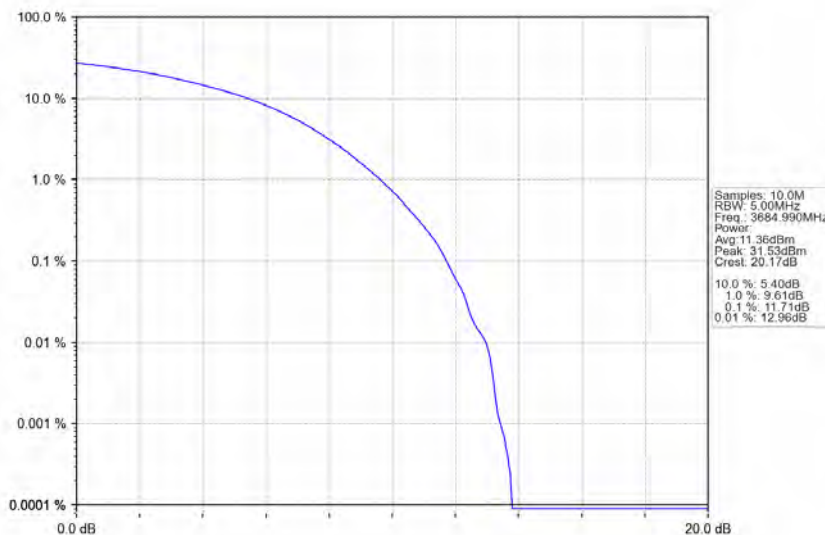
n78d_30kHz_MIMO_NTNV_30MHz_CP-OFDM QPSK_3684.99MHz_Outer_Full
