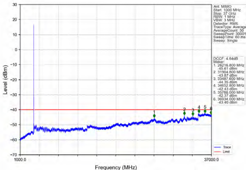
n78d_30kHz_MIMO_NTNV_10MHz_CP-OFDM QPSK_3555MHz_Outer_Full
