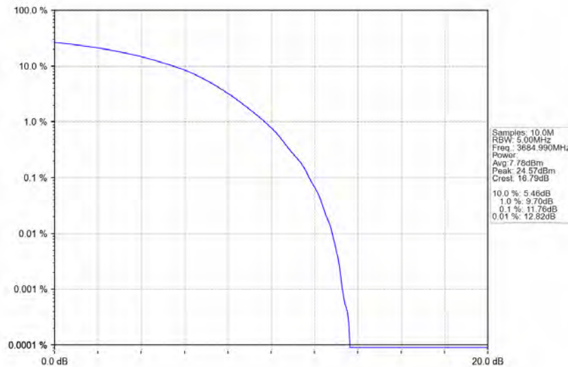
n78d_30kHz_MIMO_NTNV_30MHz_CP-OFDM 256 QAM_3684.99MHz_Outer_Full
