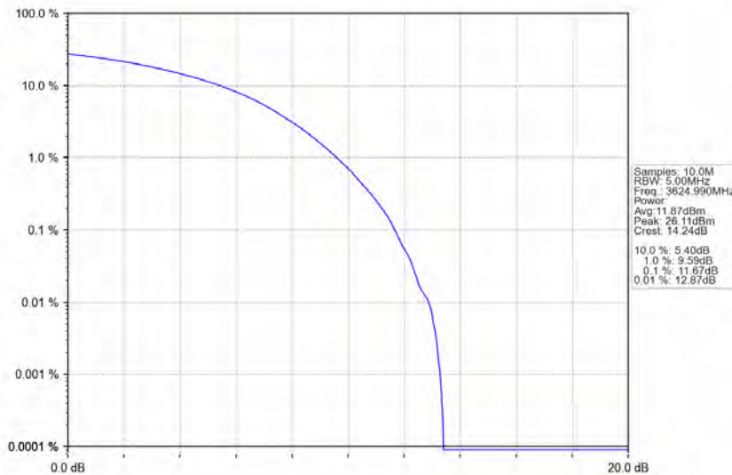
n78d_30kHz_MIMO_NTNV_30MHz_CP-OFDM QPSK_3624.99MHz_Outer_Full
