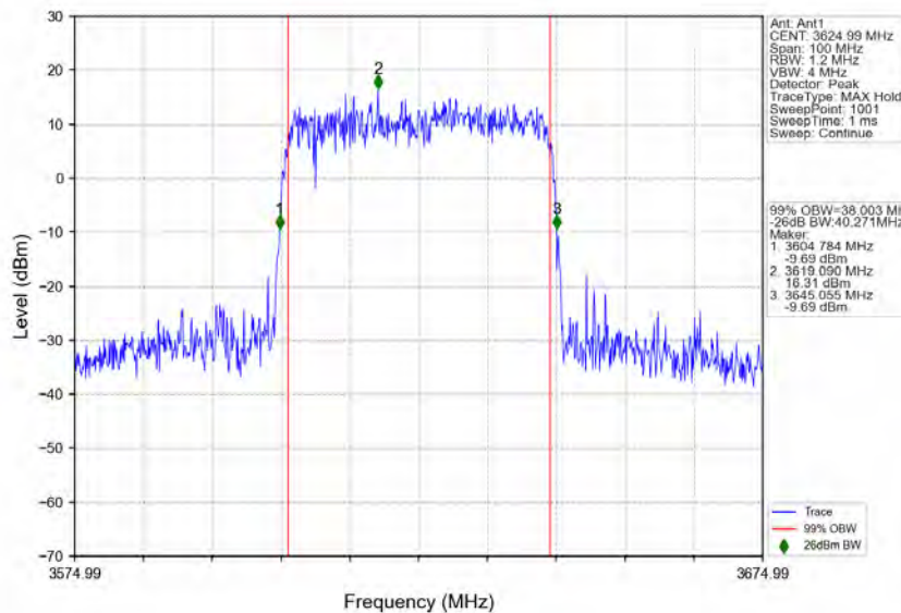
n78d_30kHz_MIMO_NTNV_40MHz_CP-OFDM 256 QAM_3624.99MHz_Outer_Full
