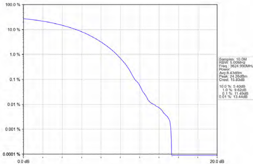
n78d_30kHz_MIMO_NTNV_60MHz_CP-OFDM QPSK_3624.99MHz_Outer_Full
