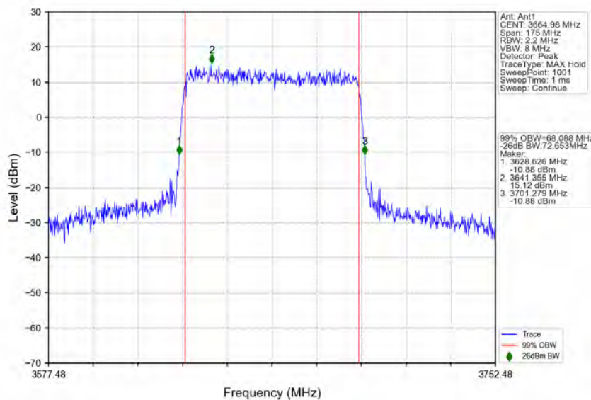
n78d_30kHz_MIMO_NTNV_70MHz_CP-OFDM QPSK_3664.98MHz_Outer_Full
