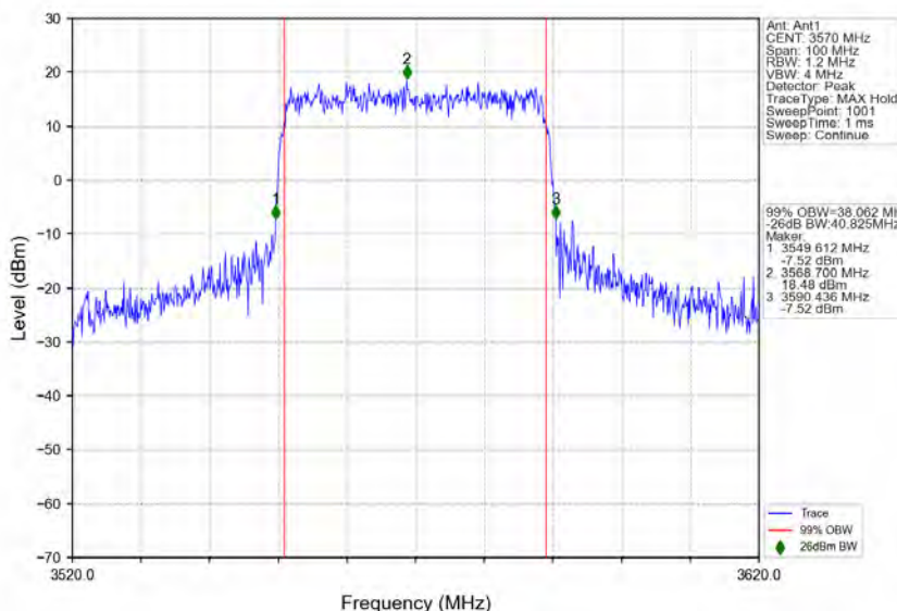
n78d_30kHz_MIMO_NTNV_40MHz_CP-OFDM 64 QAM_3570MHz_Outer_Full
