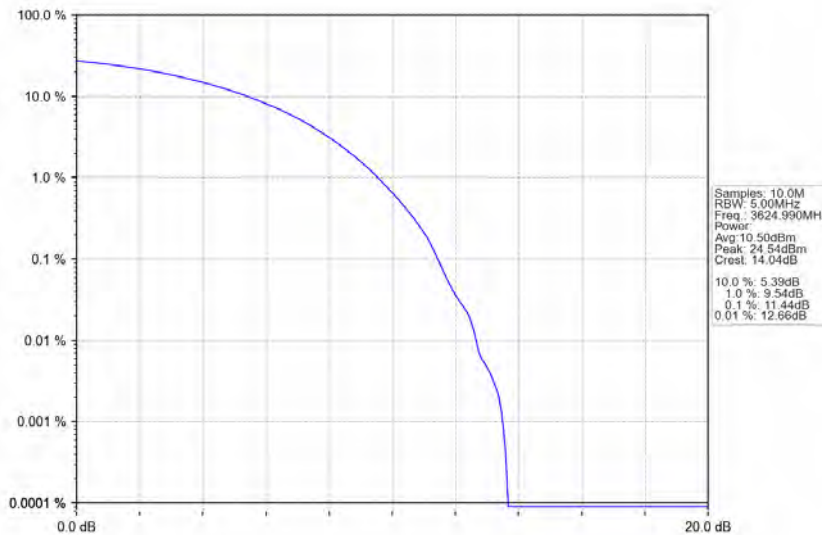
n78d_30kHz_MIMO_NTNV_40MHz_CP-OFDM_QPSK_3624.99MHz_Outer_Full
