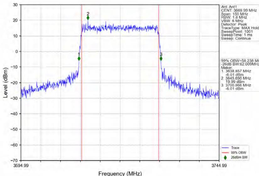
n78d_30kHz_MIMO_NTNV_60MHz_CP-OFDM_64_QAM_3669.99MHz_Outer_Full
