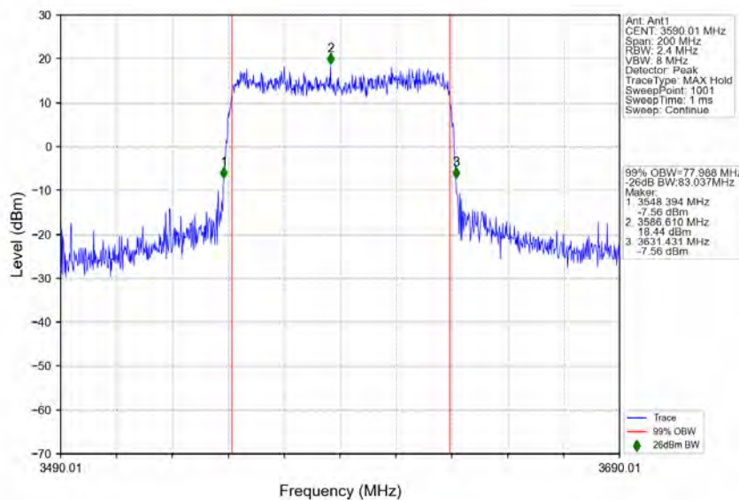
n78d_30kHz_MIMO_NTNV_80MHz_CP-OFDM 64 QAM_3590.01MHz_Outer_Full
