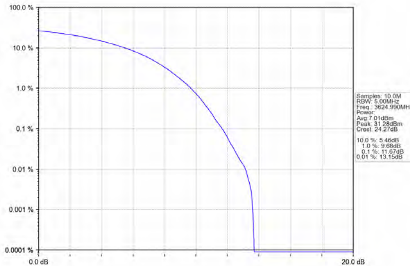
n78d_30kHz_MIMO_NTNV_70MHz_CP-OFDM_64_QAM_3624.99MHz_Outer_Full
