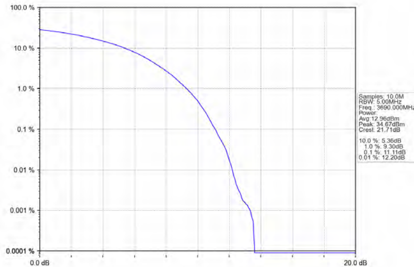
n78d_30kHz_MIMO_NTNV_20MHz_CP-OFDM 64 QAM_3690MHz_Outer_Full
