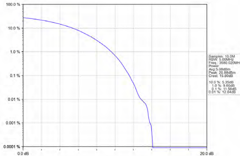
n78d_30kHz_MIMO_NTNV_60MHz_CP-OFDM_256_QAM_3580.02MHz_Outer_Full
