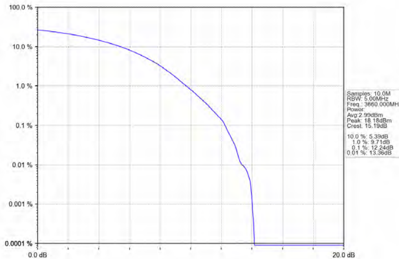
n78d_30kHz_MIMO_NTNV_80MHz_CP-OFDM_256_QAM_3660MHz_Outer_Full
