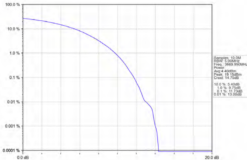
n78d_30kHz_MIMO_NTNV_60MHz_CP-OFDM 256 QAM_3669.99MHz_Outer_Full
