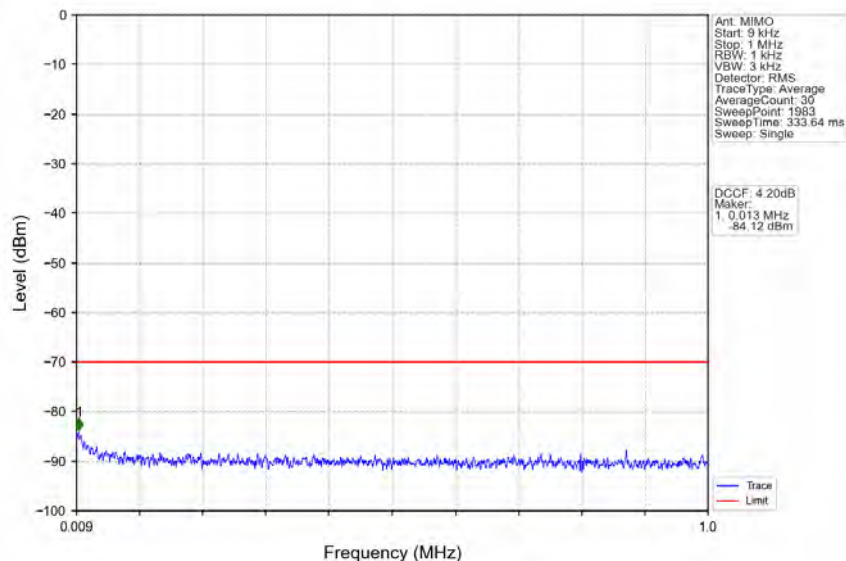
n78d_30kHz_MIMO_NTNV_10MHz_CP-OFDM QPSK_3555MHz_Outer_Full
