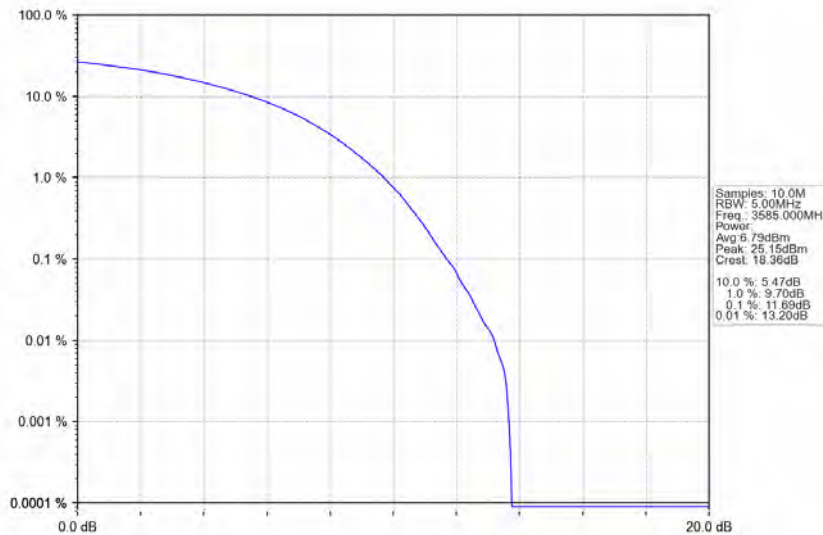
n78d_30kHz_MIMO_NTNV_70MHz_CP-OFDM 64 QAM_3585MHz_Outer_Full
