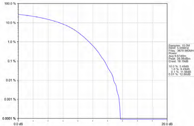
n78d_30kHz_MIMO_NTNV_40MHz_CP-OFDM 16 QAM_3679.98MHz_Outer_Full
