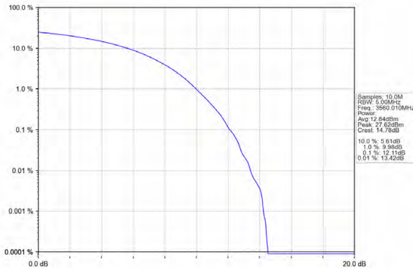
n78d_30kHz_MIMO_NTNV_20MHz_CP-OFDM 16 QAM_3560.01MHz_Outer_Full
