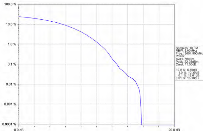
n78d_30kHz_MIMO_NTNV_90MHz_CP-OFDM_64_QAM_3654.99MHz_Outer_Full
