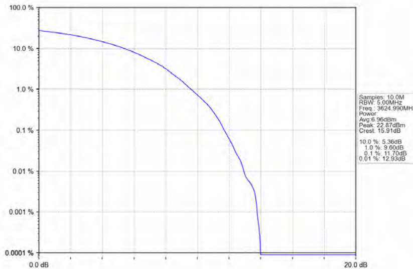
n78d_30kHz_MIMO_NTNV_80MHz_CP-OFDM QPSK_3624.99MHz_Outer_Full
