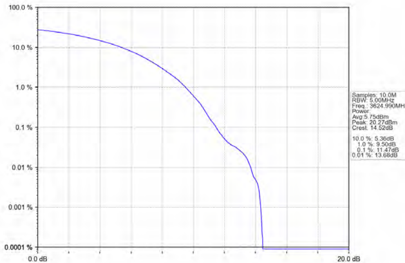
n78d_30kHz_MIMO_NTNV_100MHz_CP-OFDM 64 QAM_3624.99MHz_Outer_Full
