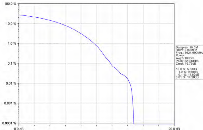
n78d_30kHz_MIMO_NTNV_90MHz_CP-OFDM_64_QAM_3624.99MHz_Outer_Full
