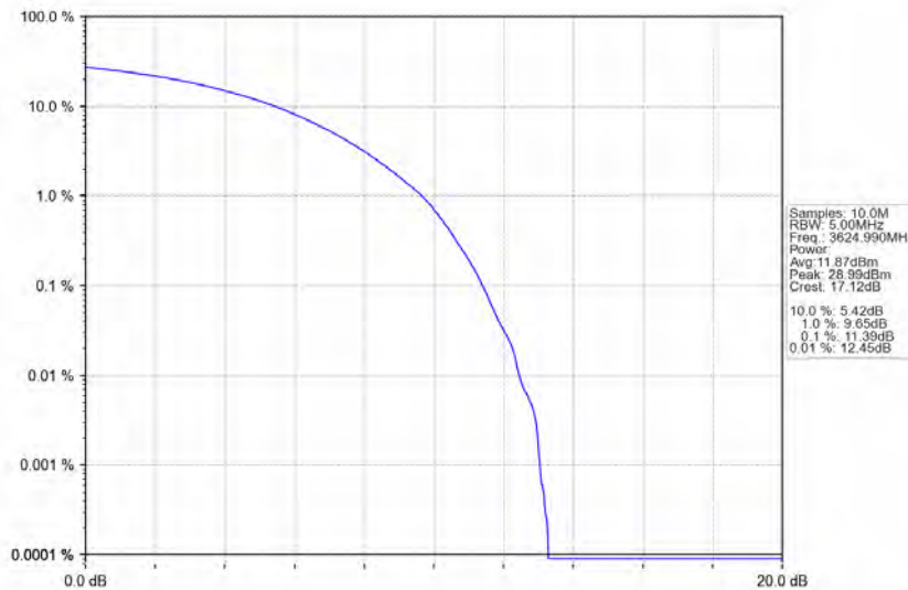
n78d_30kHz_MIMO_NTNV_30MHz_CP-OFDM_16_QAM_3624.99MHz_Outer_Full
