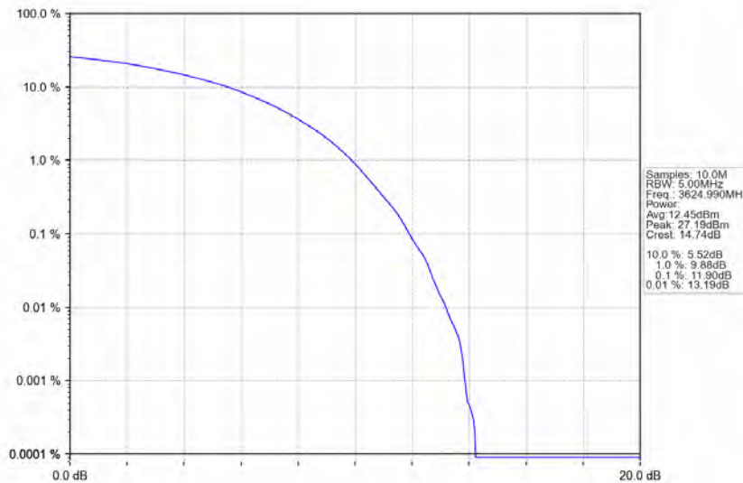
n78d_30kHz_MIMO_NTNV_10MHz_CP-OFDM_256_QAM_3624.99MHz_Outer_Full
