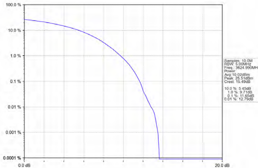
n78d_30kHz_MIMO_NTNV_40MHz_CP-OFDM 64 QAM_3624.99MHz_Outer_Full
