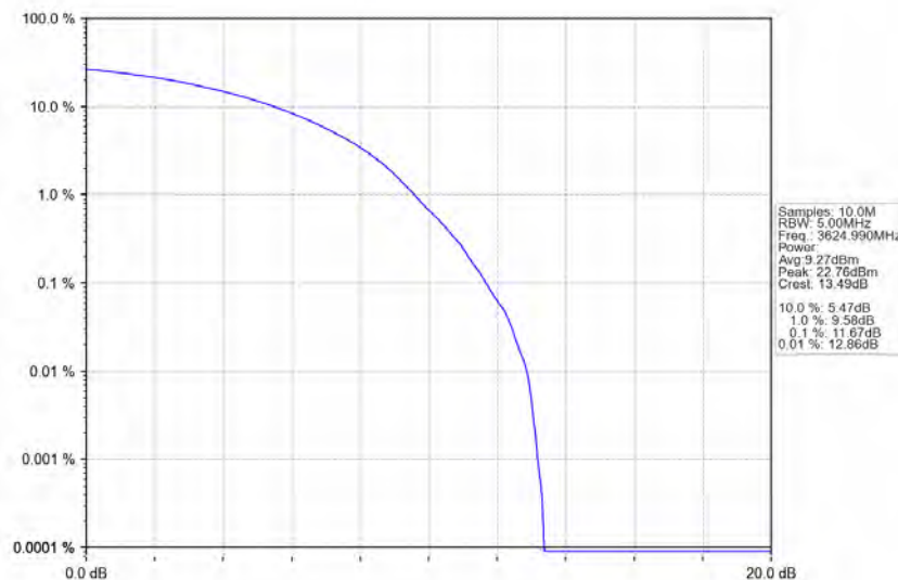
n78d_30kHz_MIMO_NTNV_50MHz_CP-OFDM_16_QAM_3624.99MHz_Outer_Full
