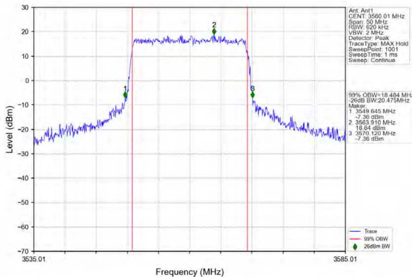
n78d_30kHz_MIMO_NTNV_20MHz_CP-OFDM 64 QAM_3560.01MHz_Outer_Full
