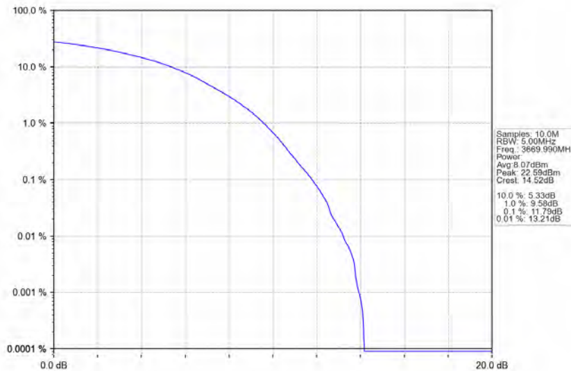
n78d_30kHz_MIMO_NTNV_60MHz_CP-OFDM 16 QAM_3669.99MHz_Outer_Full
