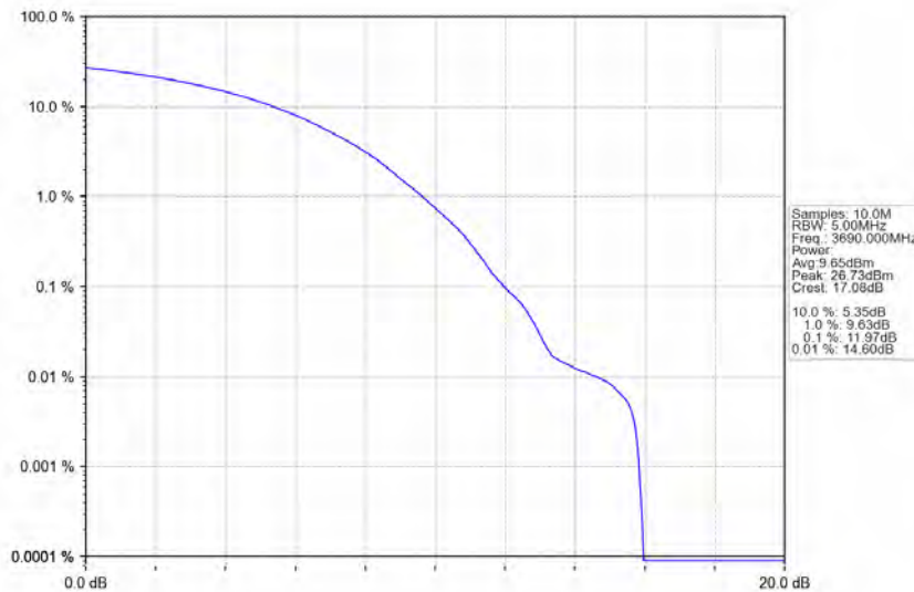
n78d_30kHz_MIMO_NTNV_20MHz_CP-OFDM_256_QAM_3690MHz_Outer_Full
