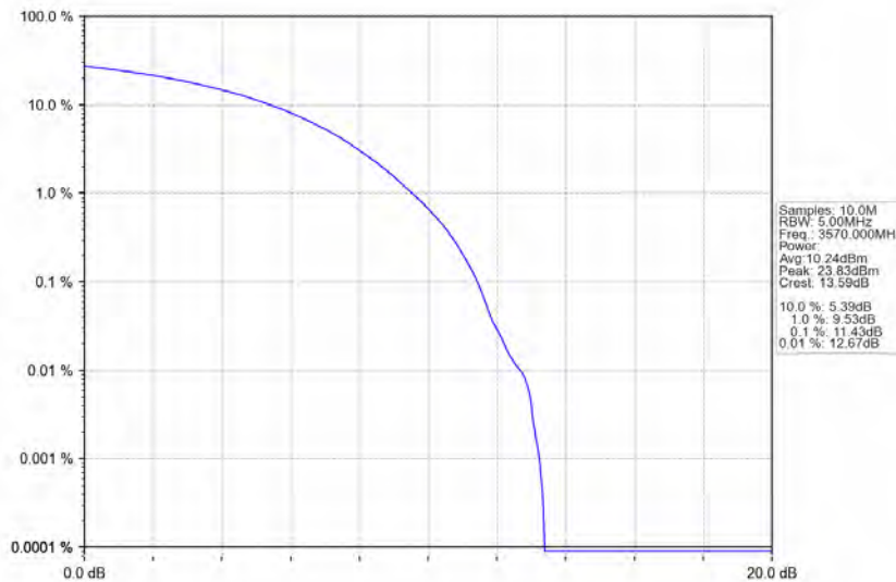
n78d_30kHz_MIMO_NTNV_40MHz_CP-OFDM 64 QAM_3570MHz_Outer_Full
