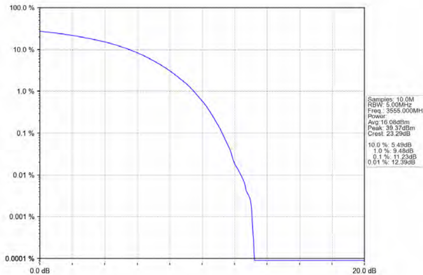
n78d_30kHz_MIMO_NTNV_10MHz_CP-OFDM 16 QAM_3555MHz_Outer_Full
