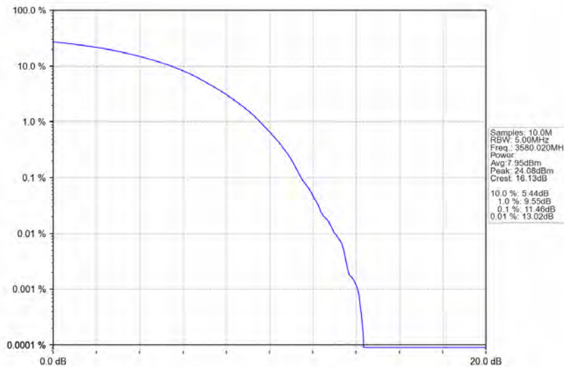
n78d_30kHz_MIMO_NTNV_60MHz_CP-OFDM 64 QAM_3580.02MHz_Outer_Full
