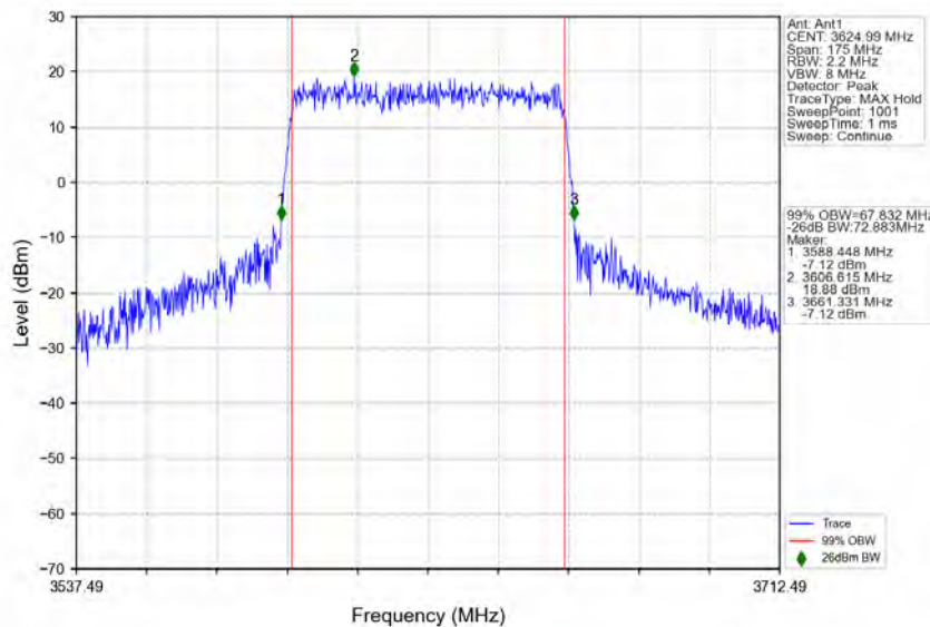
n78d_30kHz_MIMO_NTNV_70MHz_CP-OFDM 16 QAM_3624.99MHz_Outer_Full
