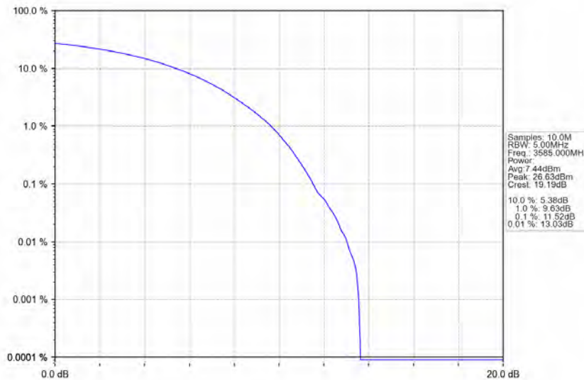
n78d_30kHz_MIMO_NTNV_70MHz_CP-OFDM 16 QAM_3585MHz_Outer_Full
