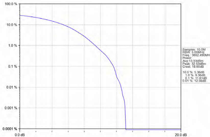
n78d_30kHz_MIMO_NTNV_15MHz_CP-OFDM 64 QAM_3692.49MHz_Outer_Full
