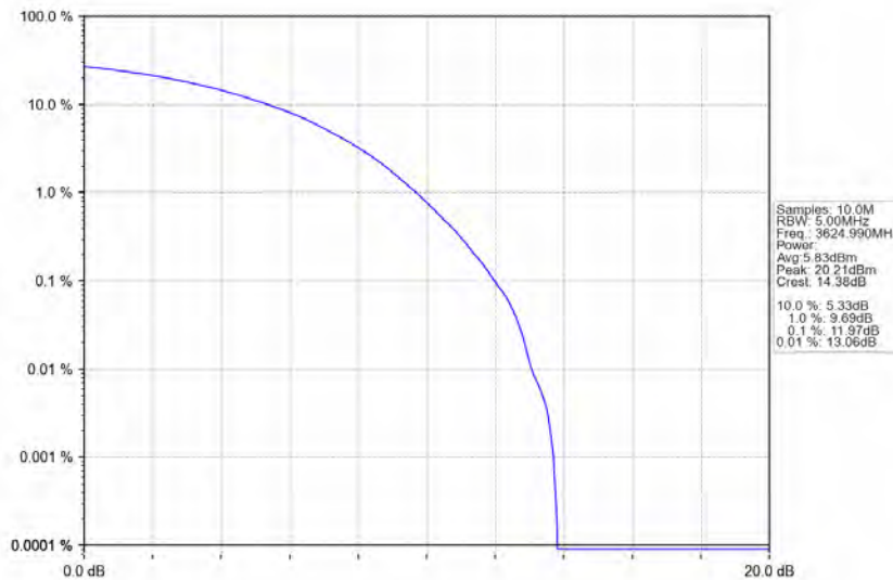
n78d_30kHz_MIMO_NTNV_50MHz_CP-OFDM 256 QAM_3624.99MHz_Outer_Full
