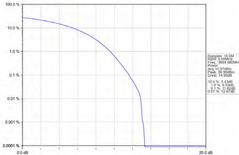
n78d_30kHz_MIMO_NTNV_10MHz_CP-OFDM QPSK_3694.98MHz_Outer_Full
