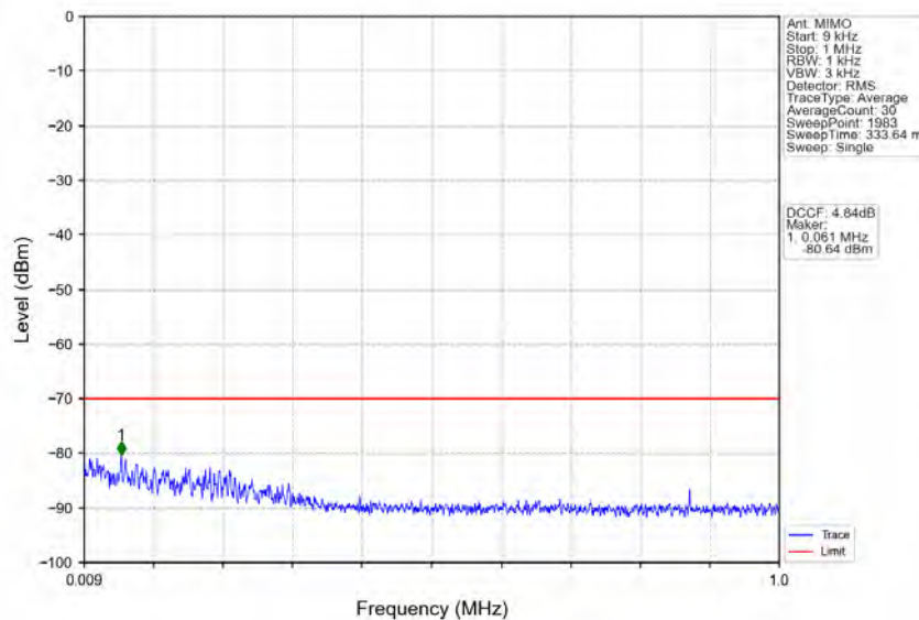
n78d_30kHz_MIMO_NTNV_10MHz_CP-OFDM QPSK_3555MHz_Edge_1RB_Left
