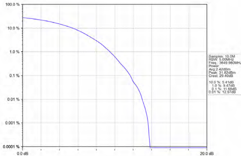
n78d_30kHz_MIMO_NTNV_100MHz_CP-OFDM_256_QAM_3649.98MHz_Outer_Full
