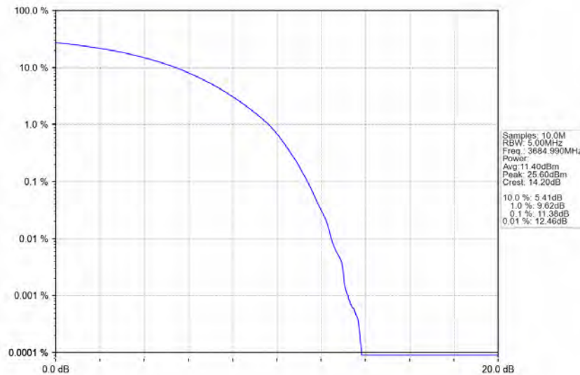
n78d_30kHz_MIMO_NTNV_30MHz_CP-OFDM 16 QAM_3684.99MHz_Outer_Full
