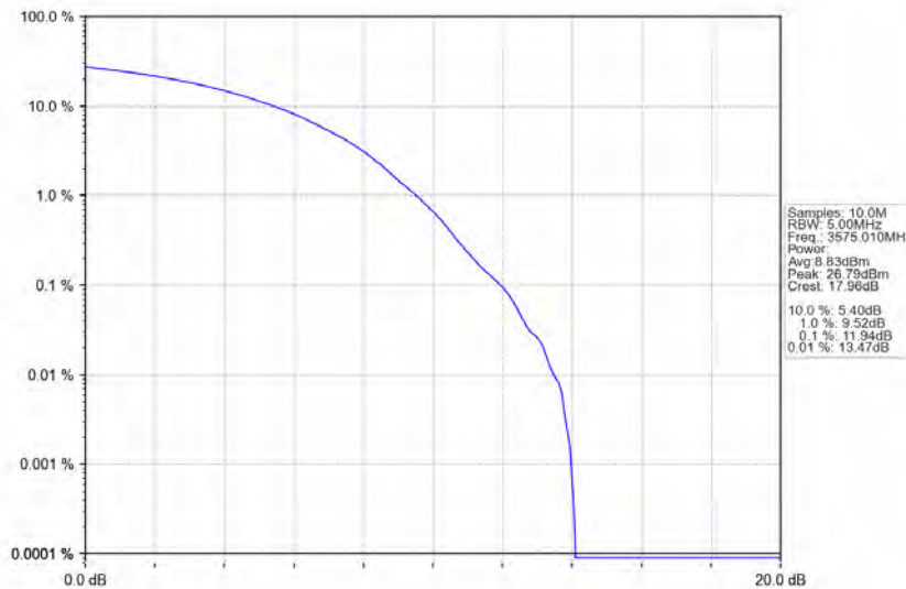
n78d_30kHz_MIMO_NTNV_50MHz_CP-OFDM 64 QAM_3575.01MHz_Outer_Full
