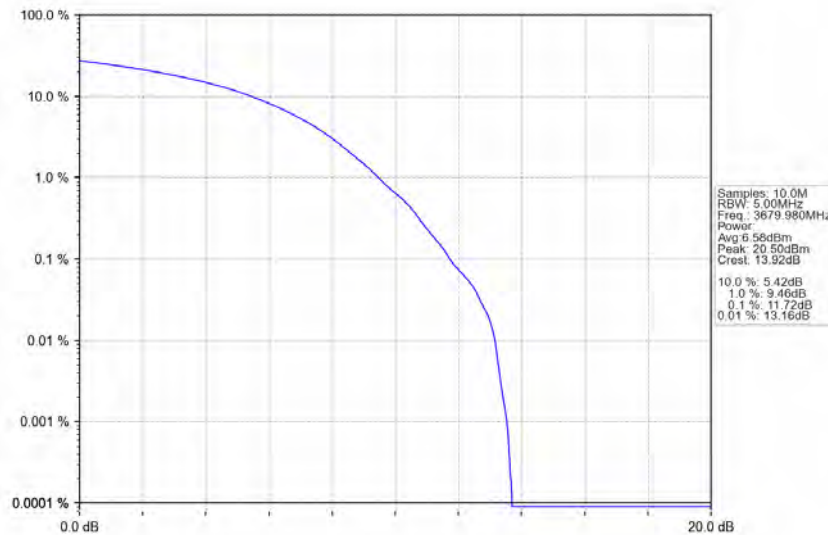
n78d_30kHz_MIMO_NTNV_40MHz_CP-OFDM 256 QAM_3679.98MHz_Outer_Full
