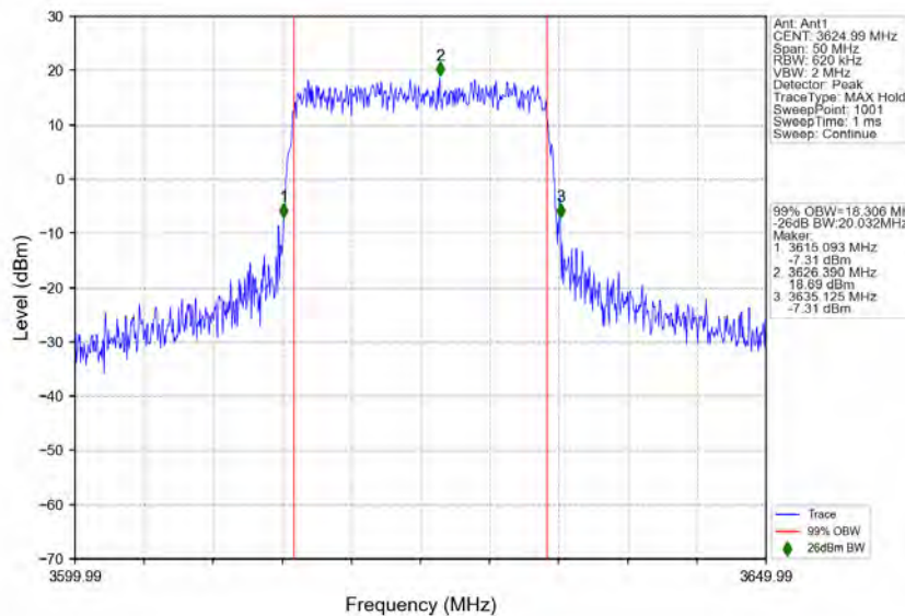
n78d_30kHz_MIMO_NTNV_20MHz_CP-OFDM_16_QAM_3624.99MHz_Outer_Full
