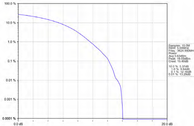
n78d_30kHz_MIMO_NTNV_80MHz_CP-OFDM_256_QAM_3624.99MHz_Outer_Full
