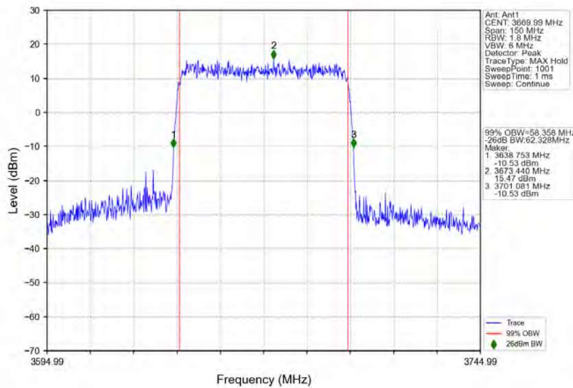
n78d_30kHz_MIMO_NTNV_60MHz_CP-OFDM 256 QAM_3669.99MHz_Outer_Full
