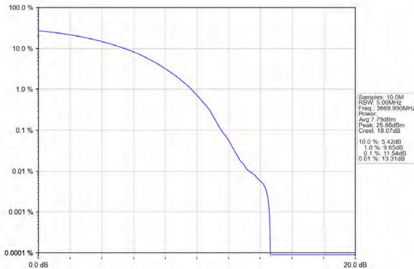
n78d_30kHz_MIMO_NTNV_60MHz_CP-OFDM QPSK_3669.99MHz_Outer_Full
