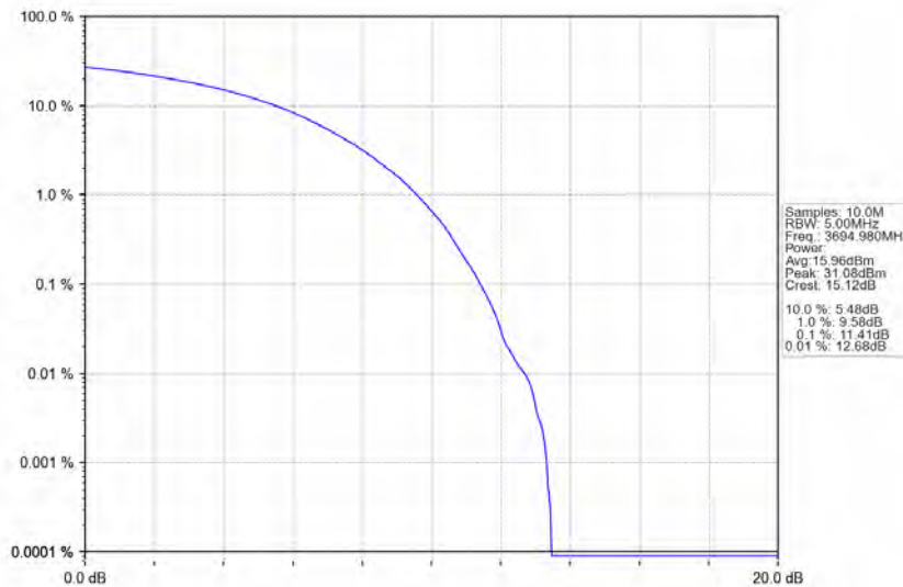
n78d_30kHz_MIMO_NTNV_10MHz_CP-OFDM 16 QAM_3694.98MHz_Outer_Full
