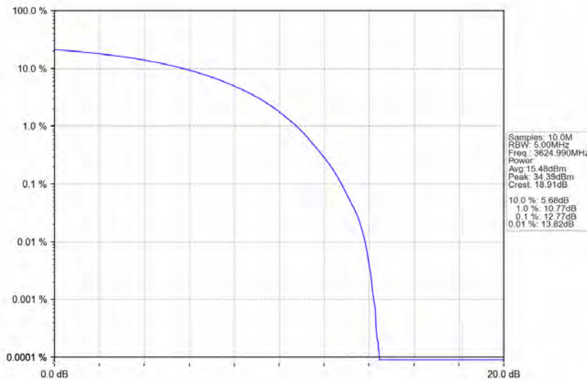
n78d_30kHz_MIMO_NTNV_10MHz_CP-OFDM 64 QAM_3624.99MHz_Outer_Full
