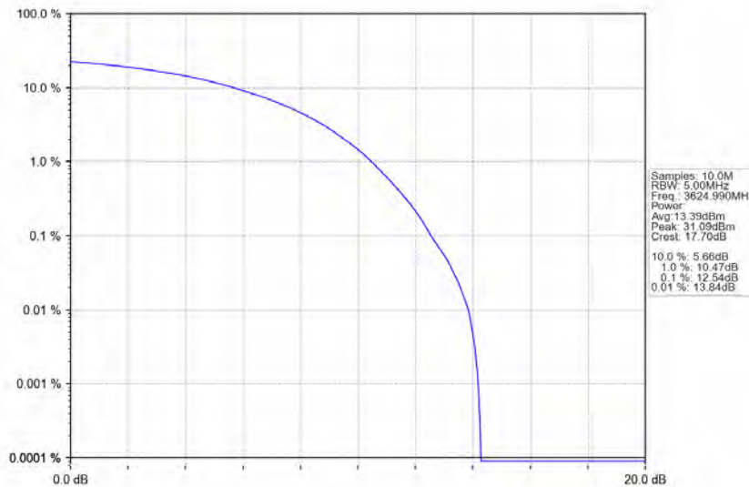
n78d_30kHz_MIMO_NTNV_20MHz_CP-OFDM QPSK_3624.99MHz_Outer_Full
