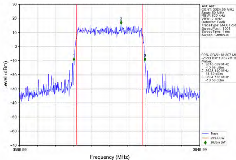
n78d_30kHz_MIMO_NTNV_20MHz_CP-OFDM 256 QAM_3624.99MHz_Outer_Full
