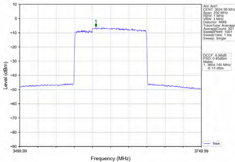
n78d_30kHz_MIMO_NTNV_100MHz_CP-OFDM 256 QAM_3624.99MHz_Inner_Full
