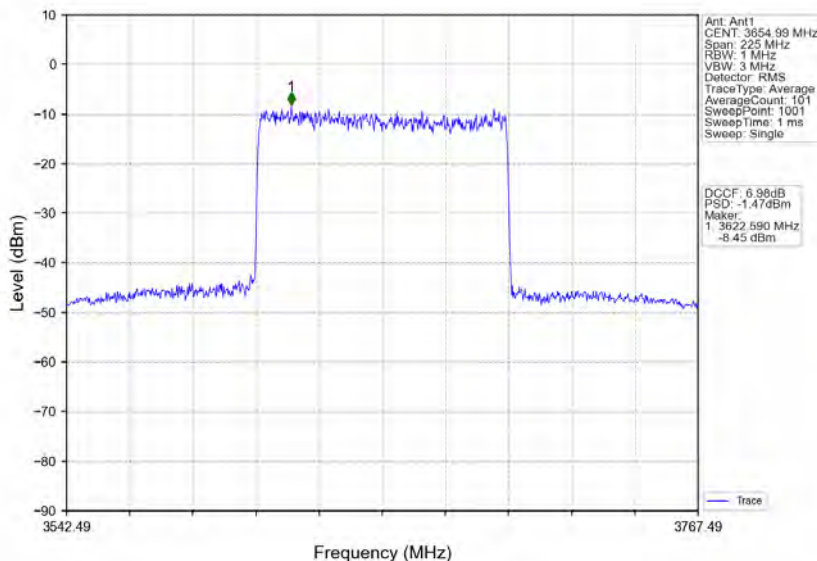
n78d_30kHz_MIMO_NTNV_90MHz_CP-OFDM_QPSK_3654.99MHz_Inner_Full
