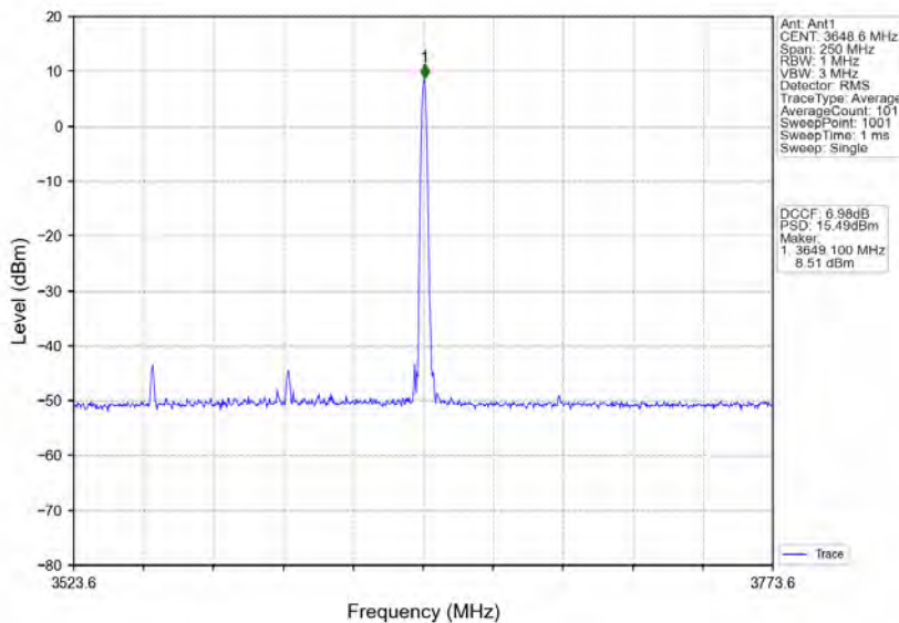
n78d_30kHz_MIMO_NTNV_100MHz_CP-OFDM 16 QAM_3600MHz_Inner_1RB_Right
