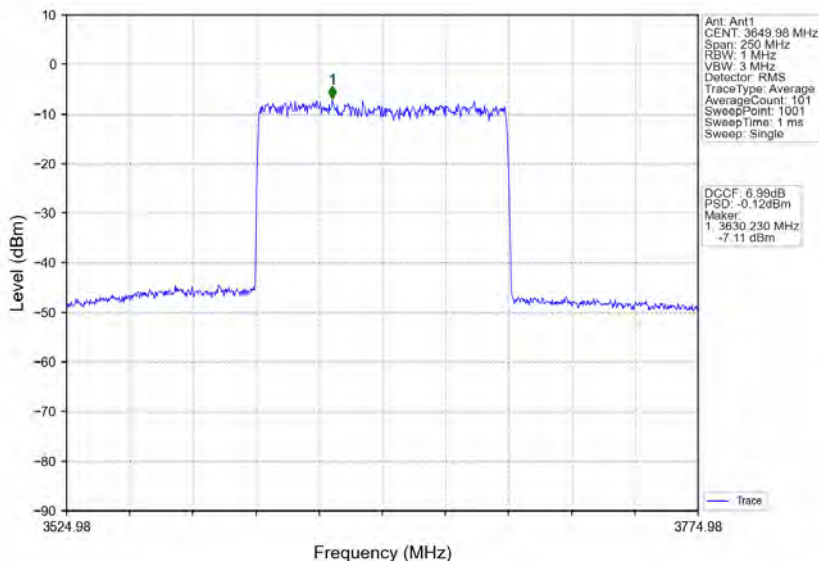
n78d_30kHz_MIMO_NTNV_100MHz_CP-OFDM 256 QAM_3649.98MHz_Inner_Full
