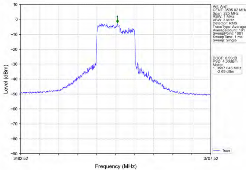
n78d_30kHz_MIMO_NTNV_90MHz_CP-OFDM 16 QAM_3595.02MHz_Inner_Full
