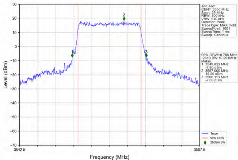
n78d_30kHz_MIMO_NTNV_10MHz_CP-OFDM 64 QAM_3555MHz_Outer_Full
