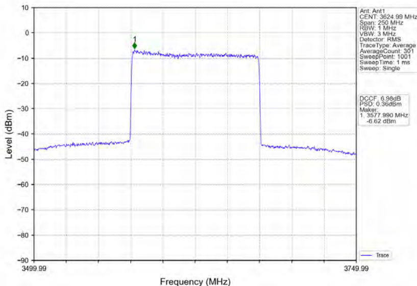
n78d_30kHz_MIMO_NTNV_100MHz_CP-OFDM 16 QAM_3624.99MHz_Inner_Full
