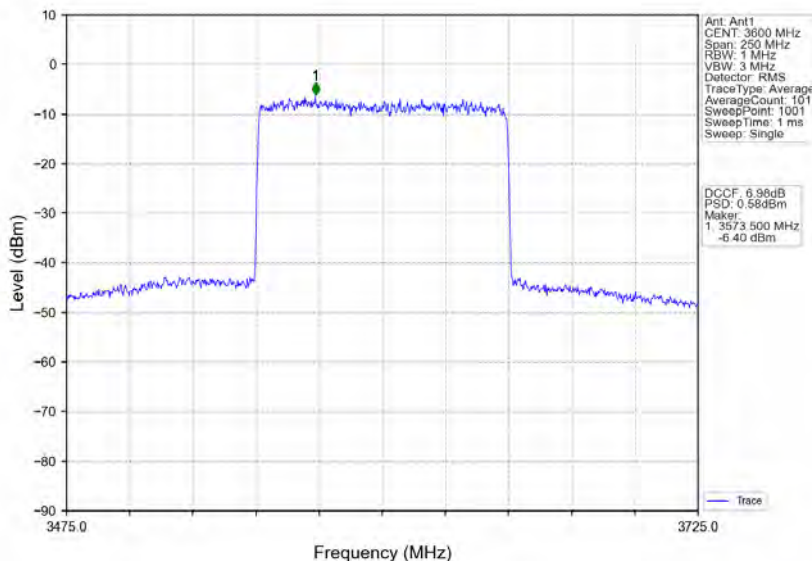
n78d_30kHz_MIMO_NTNV_100MHz_CP-OFDM 16 QAM_3600MHz_Inner_Full
