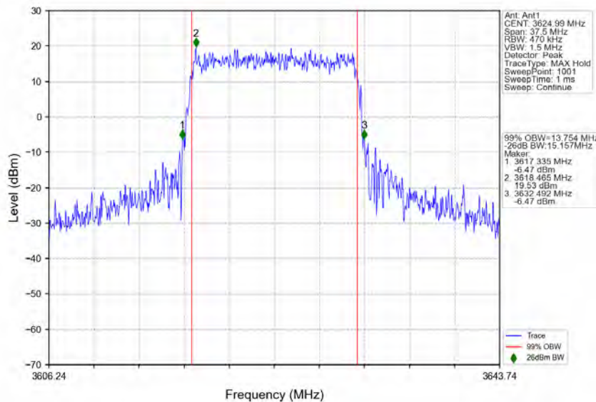
n78d_30kHz_MIMO_NTNV_15MHz_CP-OFDM_16_QAM_3624.99MHz_Outer_Full
