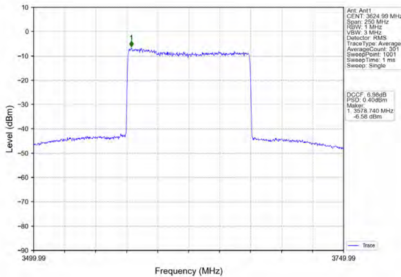
n78d_30kHz_MIMO_NTNV_100MHz_CP-OFDM QPSK_3624.99MHz_Inner_Full
