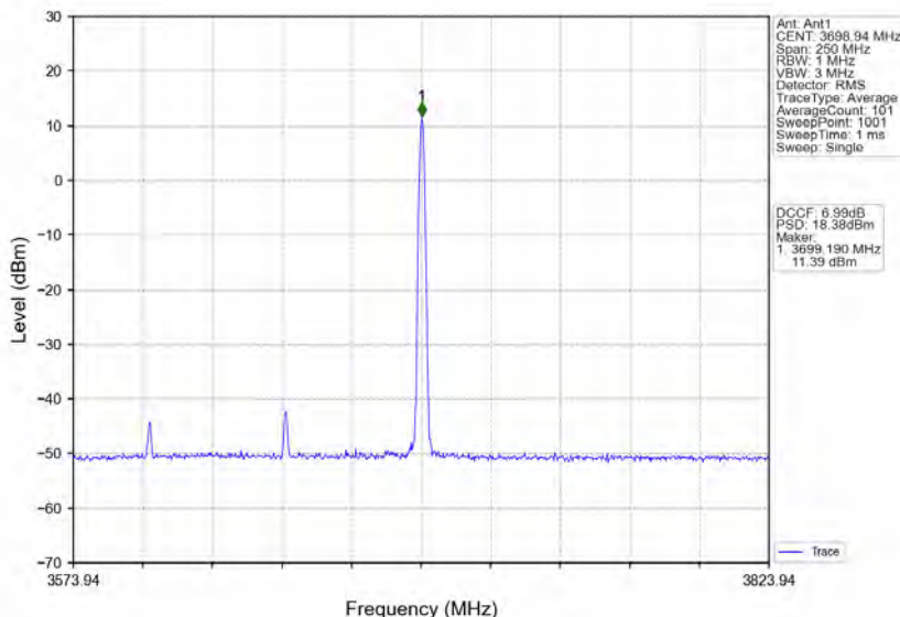
n78d_30kHz_MIMO_NTNV_100MHz_CP-OFDM 16 QAM_3649.98MHz_Edge_1RB_Right
