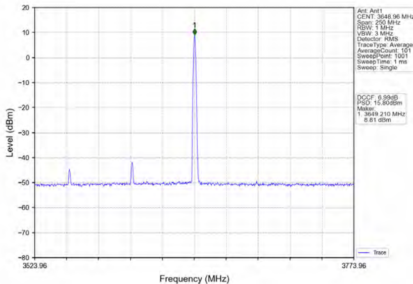
n78d_30kHz_MIMO_NTNV_100MHz_CP-OFDM 256 QAM_3600MHz_Edge_1RB_Right
