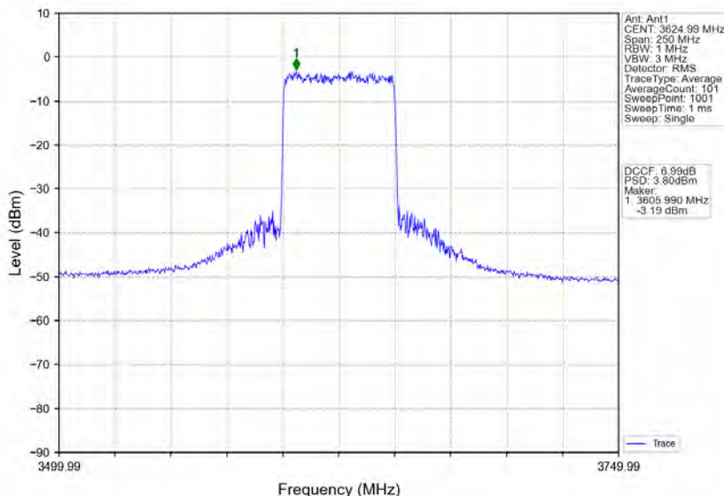
n78d_30kHz_MIMO_NTNV_100MHz_CP-OFDM 64 QAM_3624.99MHz_Inner_Full
