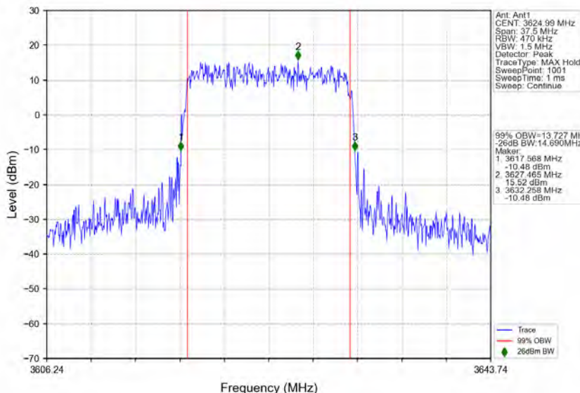
n78d_30kHz_MIMO_NTNV_15MHz_CP-OFDM_256_QAM_3624.99MHz_Outer_Full
