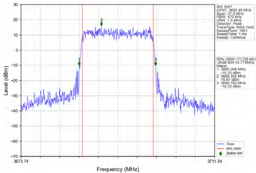
n78d_30kHz_MIMO_NTNV_15MHz_CP-OFDM 256 QAM_3692.49MHz_Outer_Full
