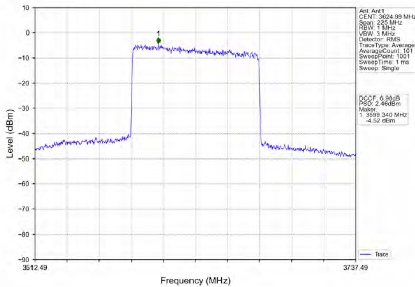
n78d_30kHz_MIMO_NTNV_90MHz_CP-OFDM 16 QAM_3624.99MHz_Inner_Full
