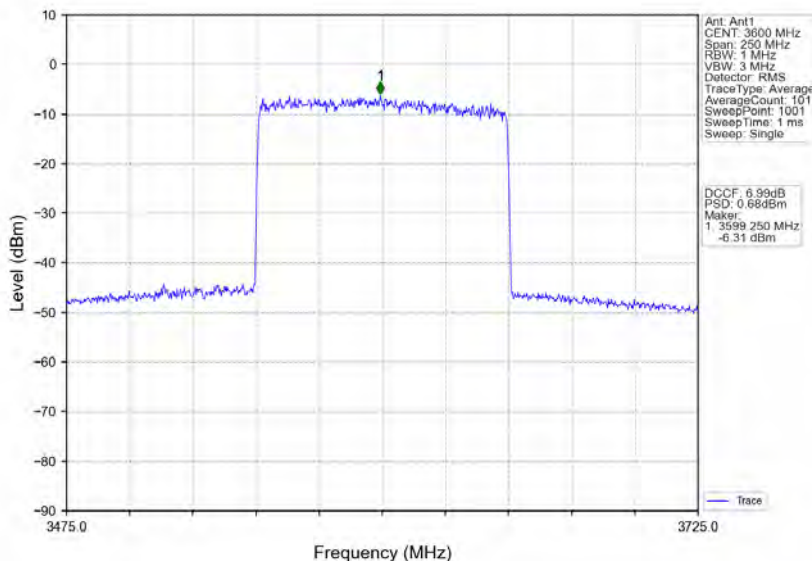
n78d_30kHz_MIMO_NTNV_100MHz_CP-OFDM_256_QAM_3600MHz_Inner_Full
