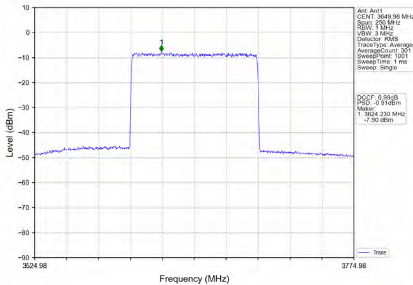
n78d_30kHz_MIMO_NTNV_100MHz_CP-OFDM 256 QAM_3649.98MHz_Inner_Full
