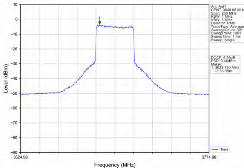
n78d_30kHz_MIMO_NTNV_100MHz_CP-OFDM QPSK_3649.98MHz_Inner_Full
