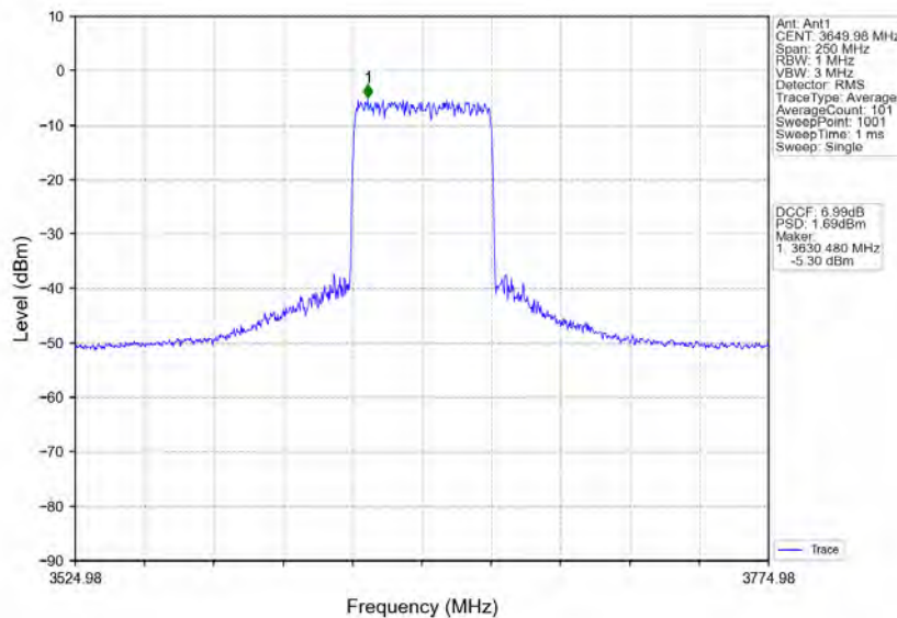
n78d_30kHz_MIMO_NTNV_100MHz_CP-OFDM 16 QAM_3649.98MHz_Inner_Full
