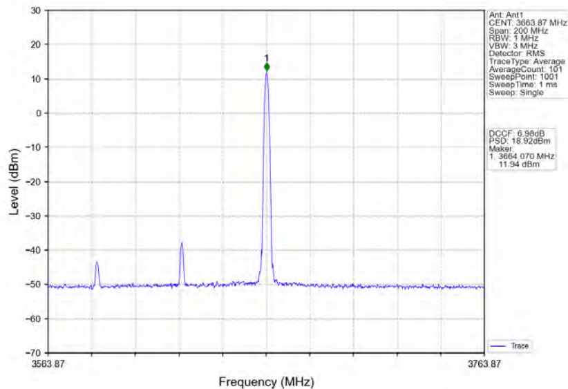
n78d_30kHz_MIMO_NTNV_80MHz_CP-OFDM 256 QAM_3624.99MHz_Edge_1RB_Right
