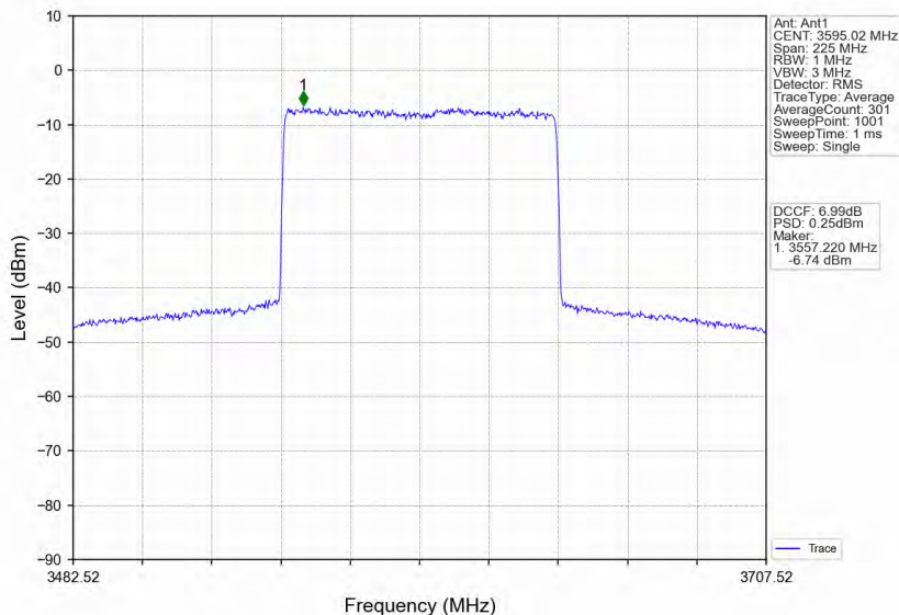
n78d_30kHz_MIMO_NTNV_90MHz_CP-OFDM 16 QAM_3595.02MHz_Inner_Full
