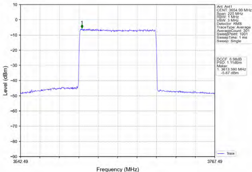
n78d_30kHz_MIMO_NTNV_90MHz_CP-OFDM 256 QAM_3654.99MHz_Inner_Full
