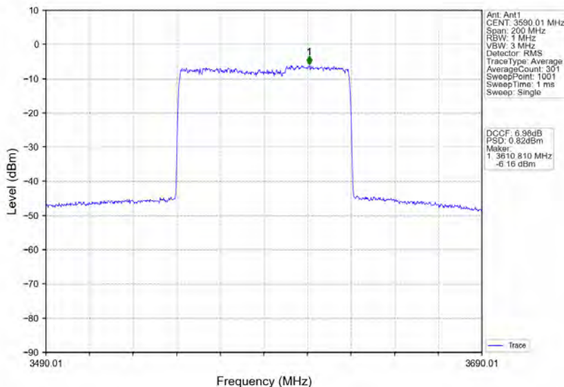
n78d_30kHz_MIMO_NTNV_80MHz_CP-OFDM_256_QAM_3590.01MHz_Inner_Full
