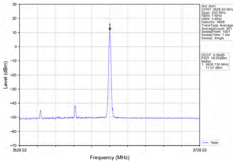
n78d_30kHz_MIMO_NTNV_80MHz_CP-OFDM QPSK_3590.01MHz_Inner_1RB_Right
