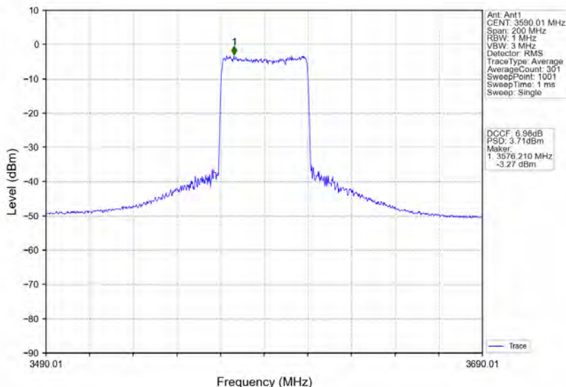
n78d_30kHz_MIMO_NTNV_80MHz_CP-OFDM 64 QAM_3590.01MHz_Inner_Full
