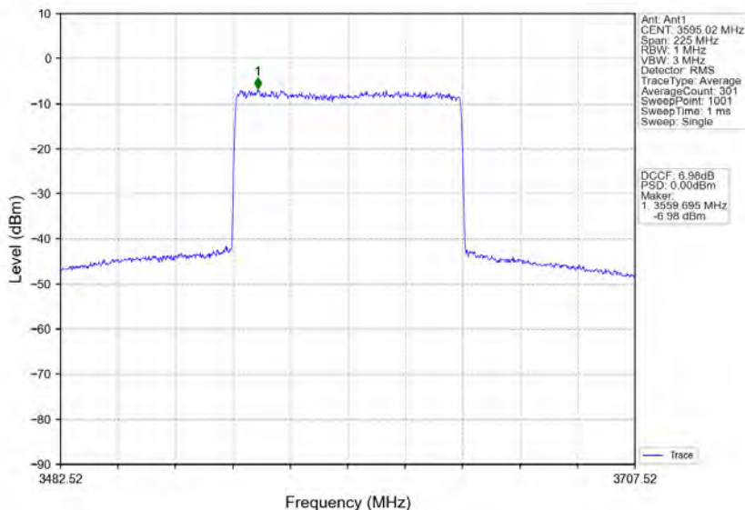
n78d_30kHz_MIMO_NTNV_90MHz_CP-OFDM 64 QAM_3595.02MHz_Inner_Full
