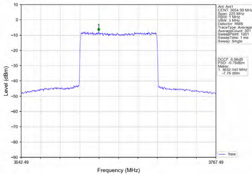
n78d_30kHz_MIMO_NTNV_90MHz_CP-OFDM 16 QAM_3654.99MHz_Inner_Full
