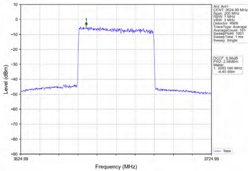
n78d_30kHz_MIMO_NTNV_80MHz_CP-OFDM_256_QAM_3624.99MHz_Inner_Full
