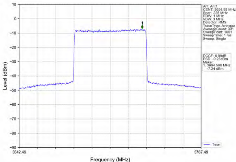
n78d_30kHz_MIMO_NTNV_90MHz_CP-OFDM 64 QAM_3654.99MHz_Inner_Full
