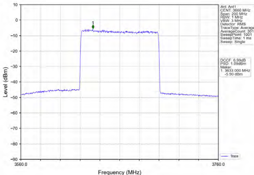
n78d_30kHz_MIMO_NTNV_80MHz_CP-OFDM_256_QAM_3660MHz_Inner_Full
