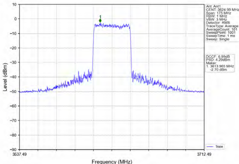
n78d_30kHz_MIMO_NTNV_70MHz_CP-OFDM 64 QAM_3624.99MHz_Inner_Full
