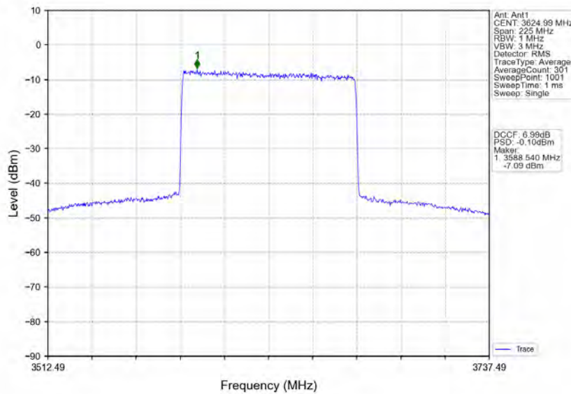
n78d_30kHz_MIMO_NTNV_90MHz_CP-OFDM QPSK_3624.99MHz_Inner_Full
