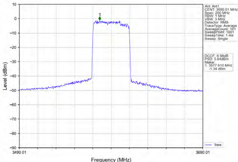
n78d_30kHz_MIMO_NTNV_80MHz_CP-OFDM_256_QAM_3590.01MHz_Inner_Full
