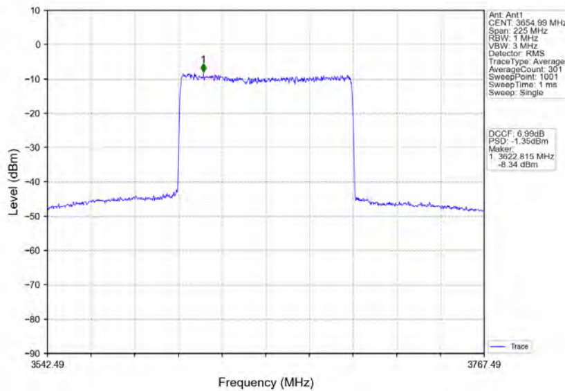
n78d_30kHz_MIMO_NTNV_90MHz_CP-OFDM QPSK_3654.99MHz_Inner_Full
