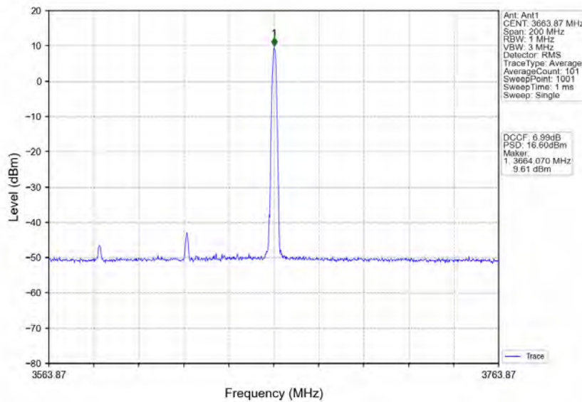
n78d_30kHz_MIMO_NTNV_80MHz_CP-OFDM QPSK_3624.99MHz_Edge_1RB_Right
