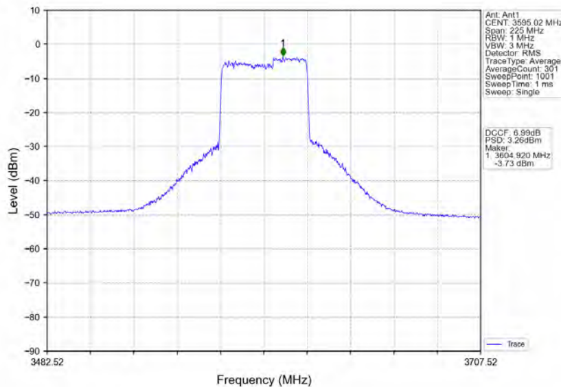
n78d_30kHz_MIMO_NTNV_90MHz_CP-OFDM QPSK_3595.02MHz_Inner_Full
