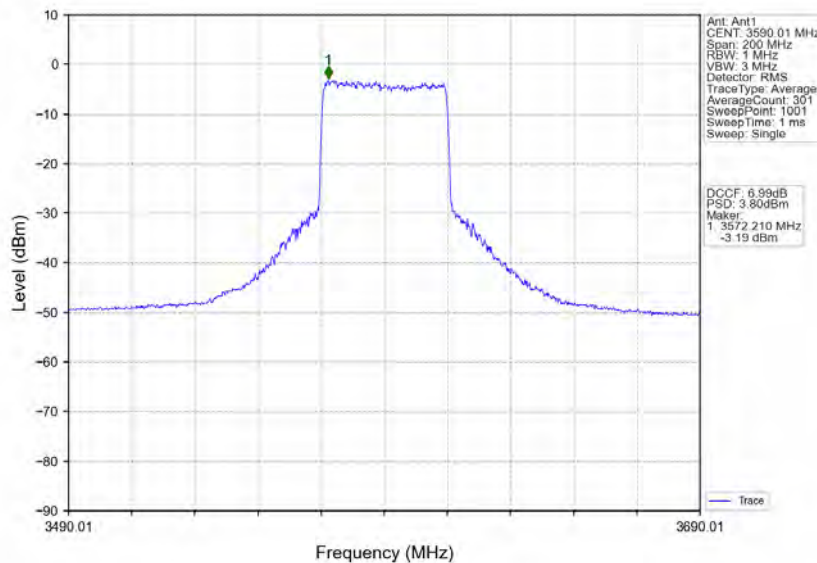
n78d_30kHz_MIMO_NTNV_80MHz_CP-OFDM QPSK_3590.01MHz_Inner_Full
