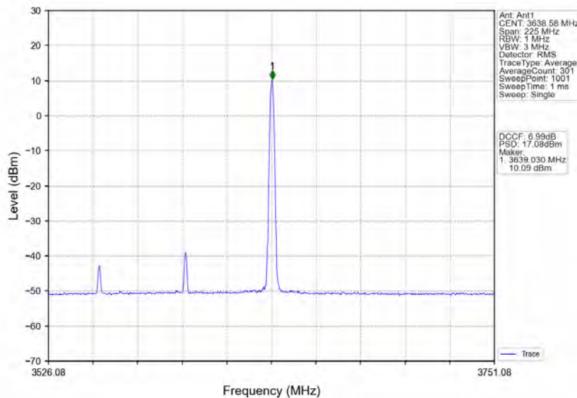
n78d_30kHz_MIMO_NTNV_90MHz_CP-OFDM 256 QAM_3595.02MHz_Inner_1RB_Right
