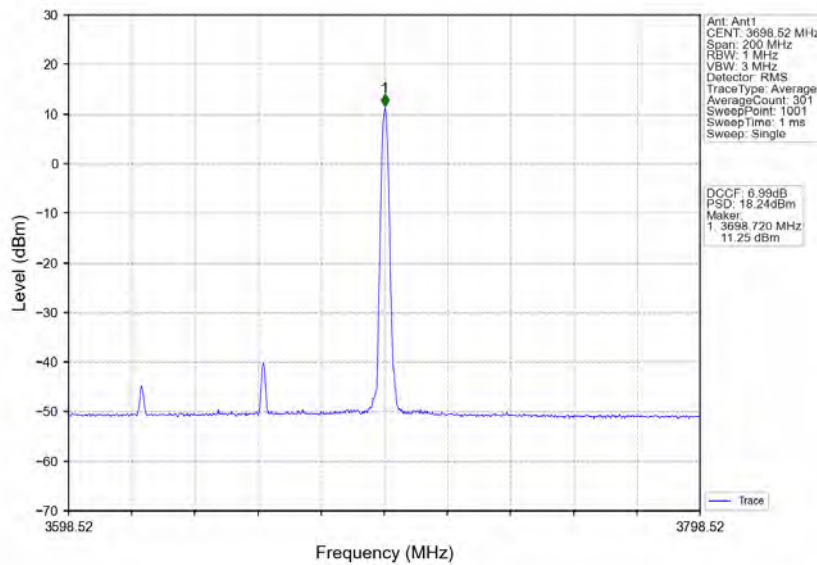
n78d_30kHz_MIMO_NTNV_80MHz_CP-OFDM 64 QAM_3660MHz_Inner_1RB_Right
