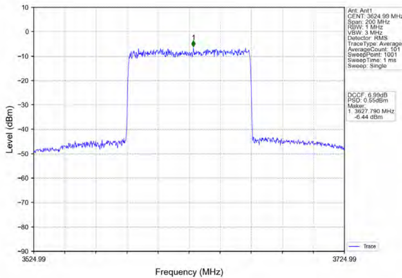
n78d_30kHz_MIMO_NTNV_80MHz_CP-OFDM_QPSK_3624.99MHz_Inner_Full
