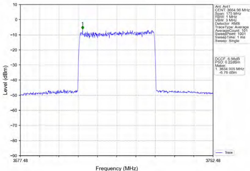
n78d_30kHz_MIMO_NTNV_70MHz_CP-OFDM 256 QAM_3664.98MHz_Inner_Full
