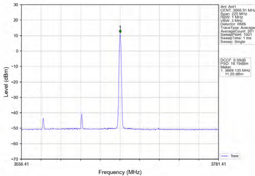
n78d_30kHz_MIMO_NTNV_90MHz_CP-OFDM 64 QAM_3624.99MHz_Edge_1RB_Right
