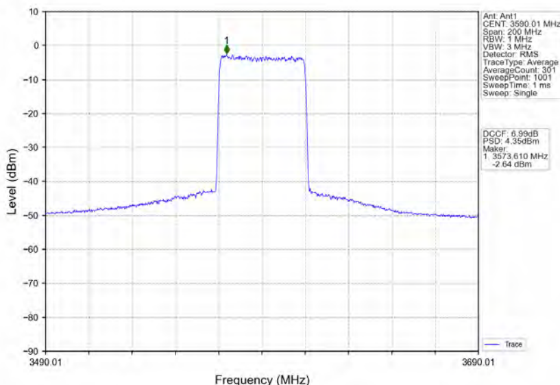
n78d_30kHz_MIMO_NTNV_80MHz_CP-OFDM_256_QAM_3590.01MHz_Inner_Full
