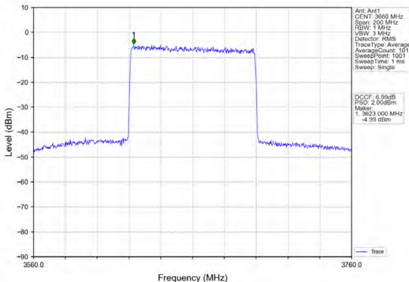
n78d_30kHz_MIMO_NTNV_80MHz_CP-OFDM QPSK_3660MHz_Inner_Full
