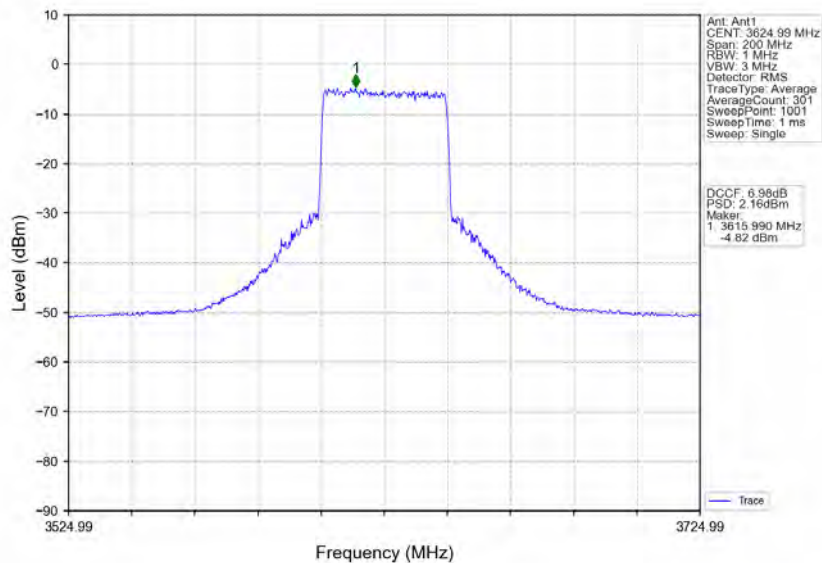
n78d_30kHz_MIMO_NTNV_80MHz_CP-OFDM QPSK_3624.99MHz_Inner_Full
