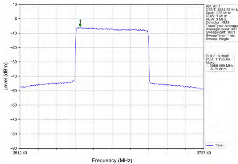
n78d_30kHz_MIMO_NTNV_90MHz_CP-OFDM 64 QAM_3624.99MHz_Inner_Full
