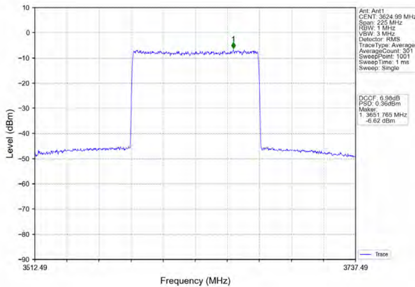
n78d_30kHz_MIMO_NTNV_90MHz_CP-OFDM 256 QAM_3624.99MHz_Inner_Full
