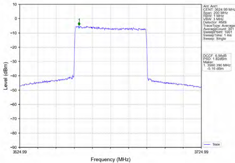
n78d_30kHz_MIMO_NTNV_80MHz_CP-OFDM 64 QAM_3624.99MHz_Inner_Full
