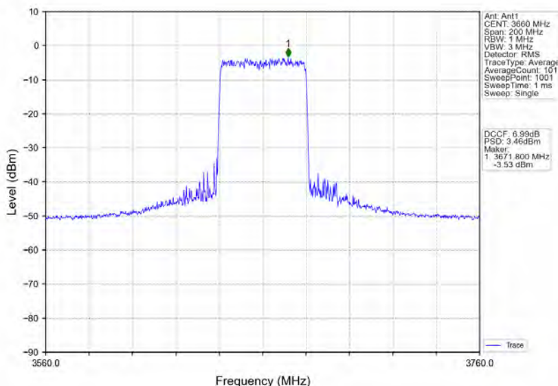
n78d_30kHz_MIMO_NTNV_80MHz_CP-OFDM 64 QAM_3660MHz_Inner_Full
