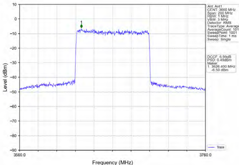
n78d_30kHz_MIMO_NTNV_80MHz_CP-OFDM 64 QAM_3660MHz_Inner_Full
