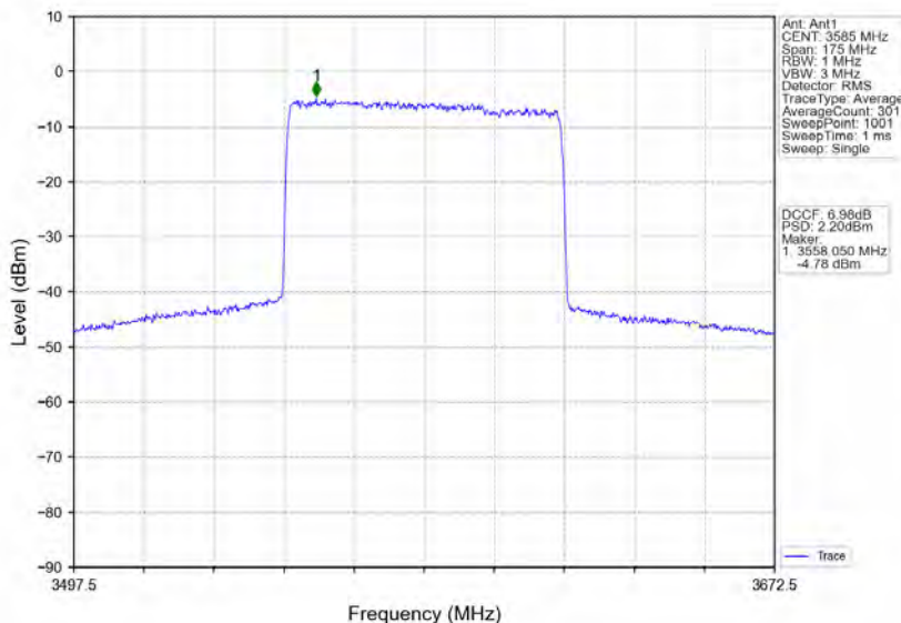
n78d_30kHz_MIMO_NTNV_70MHz_CP-OFDM QPSK_3585MHz_Inner_Full
