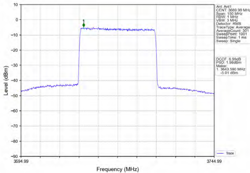
n78d_30kHz_MIMO_NTNV_60MHz_CP-OFDM QPSK_3669.99MHz_Inner_Full
