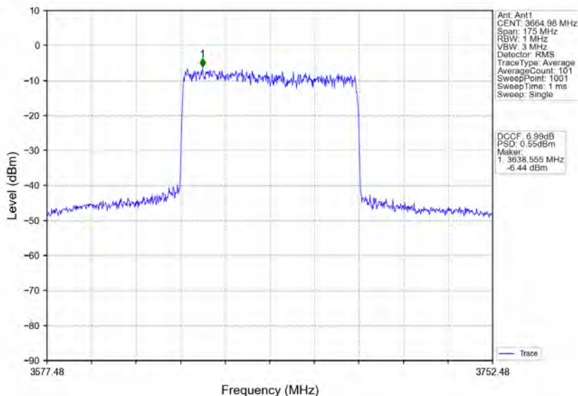
n78d_30kHz_MIMO_NTNV_70MHz_CP-OFDM 16 QAM_3664.98MHz_Inner_Full
