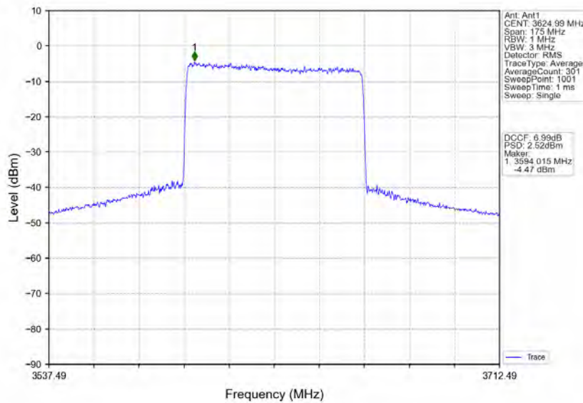
n78d_30kHz_MIMO_NTNV_70MHz_CP-OFDM 64 QAM_3624.99MHz_Inner_Full
