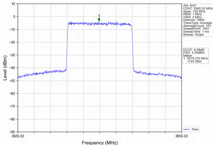
n78d_30kHz_MIMO_NTNV_60MHz_CP-OFDM QPSK_3580.02MHz_Inner_Full
