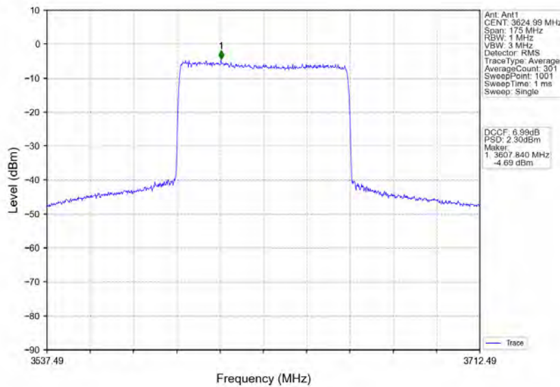
n78d_30kHz_MIMO_NTNV_70MHz_CP-OFDM 16 QAM_3624.99MHz_Inner_Full
