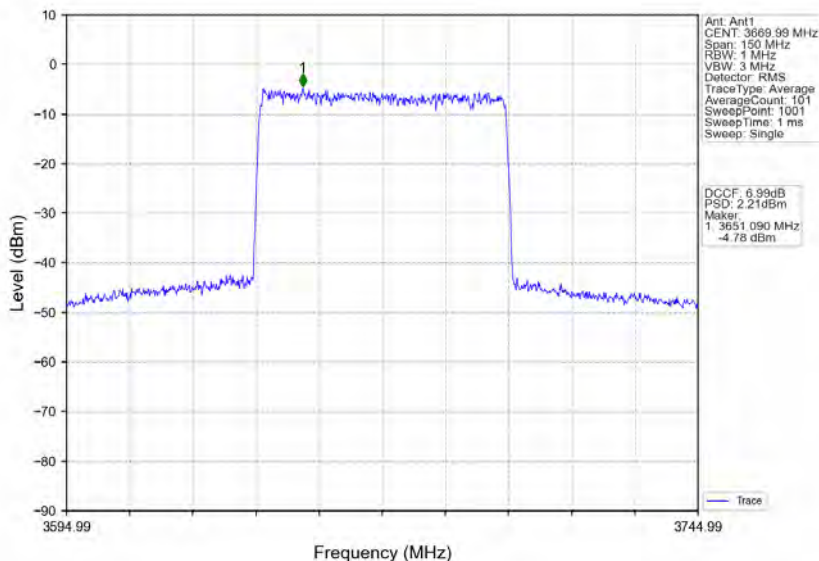
n78d_30kHz_MIMO_NTNV_60MHz_CP-OFDM 64 QAM_3669.99MHz_Inner_Full
