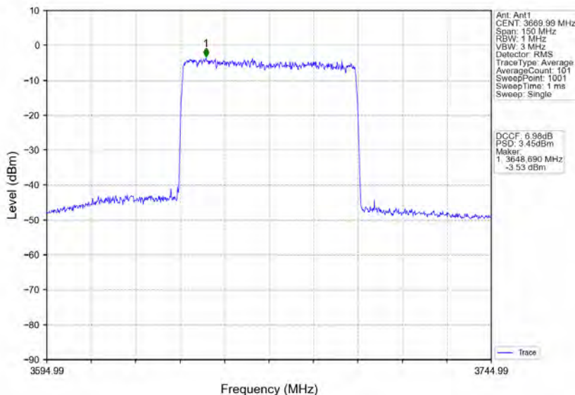
n78d_30kHz_MIMO_NTNV_60MHz_CP-OFDM 256 QAM_3669.99MHz_Inner_Full
