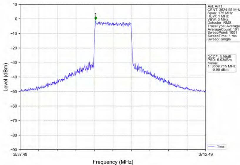
n78d_30kHz_MIMO_NTNV_70MHz_CP-OFDM QPSK_3624.99MHz_Inner_Full
