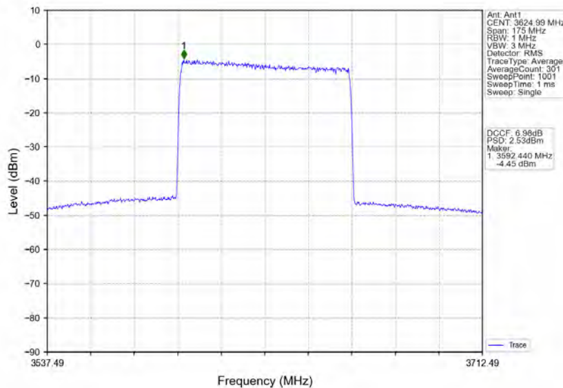
n78d_30kHz_MIMO_NTNV_70MHz_CP-OFDM 256 QAM_3624.99MHz_Inner_Full
