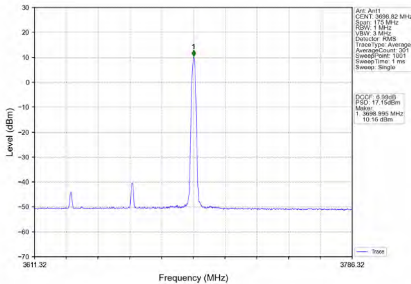
n78d_30kHz_MIMO_NTNV_70MHz_CP-OFDM 64 QAM_3664.98MHz_Edge_1RB_Right
