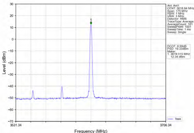
n78d_30kHz_MIMO_NTNV_70MHz_CP-OFDM 16 QAM_3585MHz_Edge_1RB_Right
