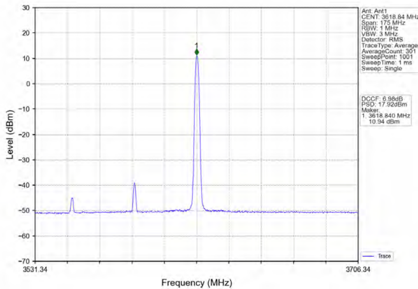
n78d_30kHz_MIMO_NTNV_70MHz_CP-OFDM 256 QAM_3585MHz_Edge_1RB_Right
