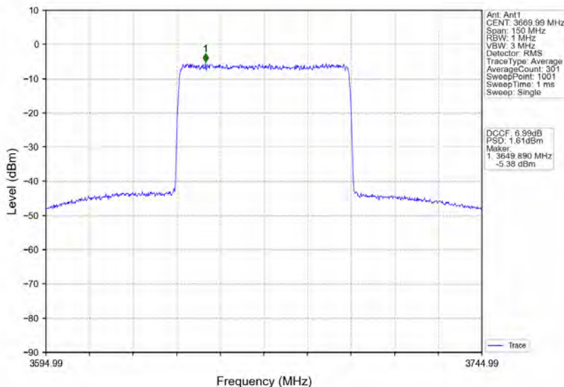
n78d_30kHz_MIMO_NTNV_60MHz_CP-OFDM 16 QAM_3669.99MHz_Inner_Full
