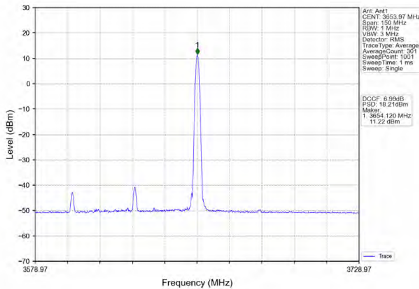
n78d_30kHz_MIMO_NTNV_60MHz_CP-OFDM QPSK_3624.99MHz_Edge_1RB_Right
