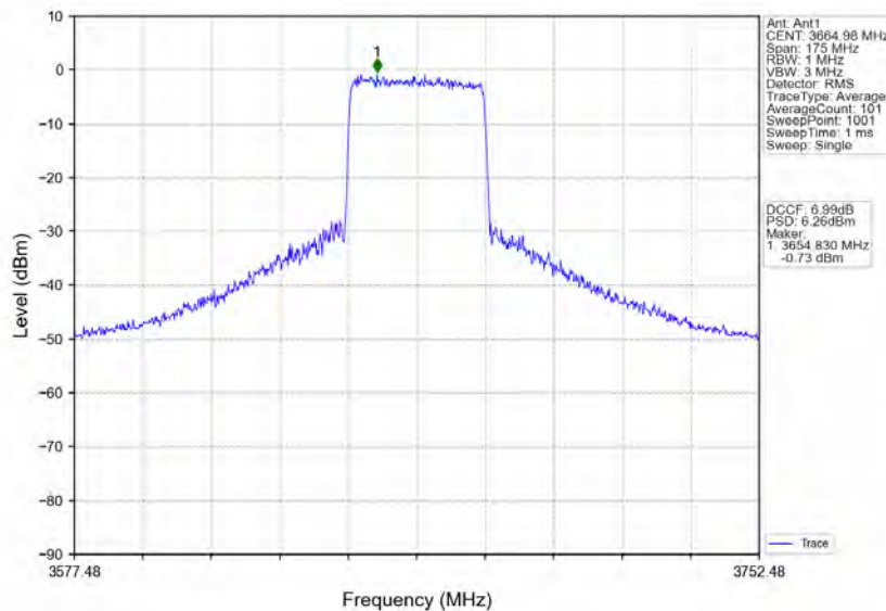
n78d_30kHz_MIMO_NTNV_70MHz_CP-OFDM QPSK_3664.98MHz_Inner_Full
