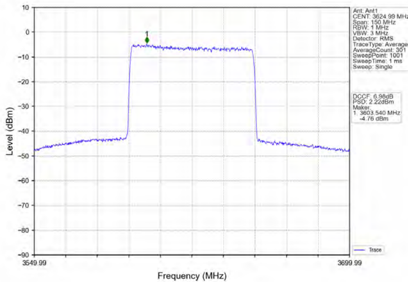
n78d_30kHz_MIMO_NTNV_60MHz_CP-OFDM 16 QAM_3624.99MHz_Inner_Full
