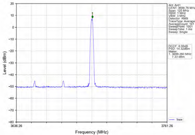
n78d_30kHz_MIMO_NTNV_50MHz_CP-OFDM 64 QAM_3675MHz_Edge_1RB_Right
