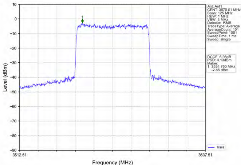
n78d_30kHz_MIMO_NTNV_50MHz_CP-OFDM 64 QAM_3575.01MHz_Inner_Full
