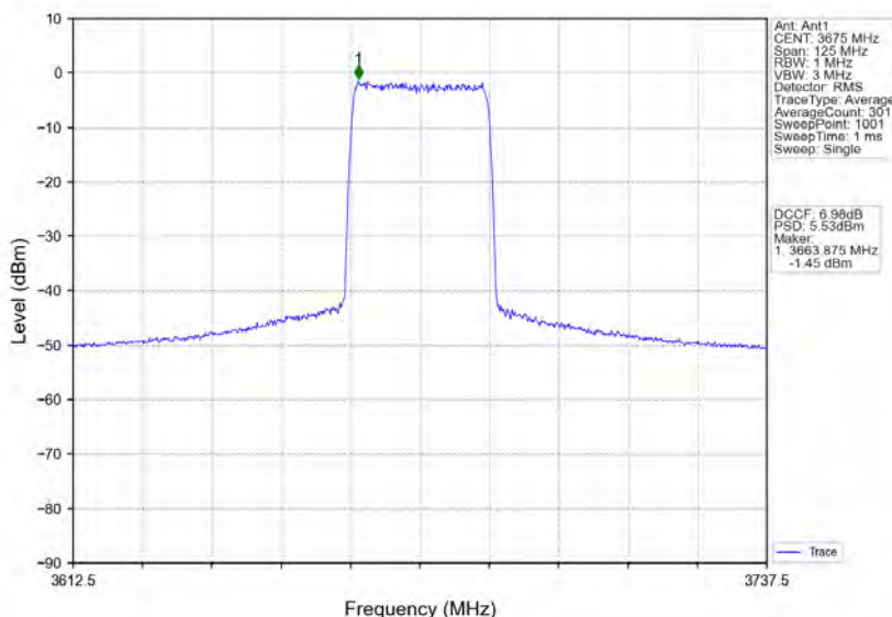
n78d_30kHz_MIMO_NTNV_50MHz_CP-OFDM_256_QAM_3675MHz_Inner_Full
