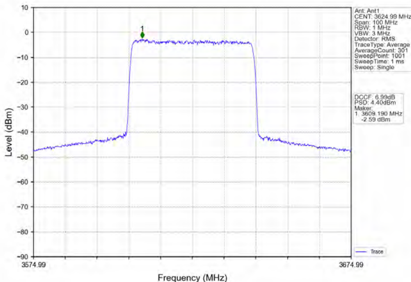
n78d_30kHz_MIMO_NTNV_40MHz_CP-OFDM 64 QAM_3624.99MHz_Inner_Full
