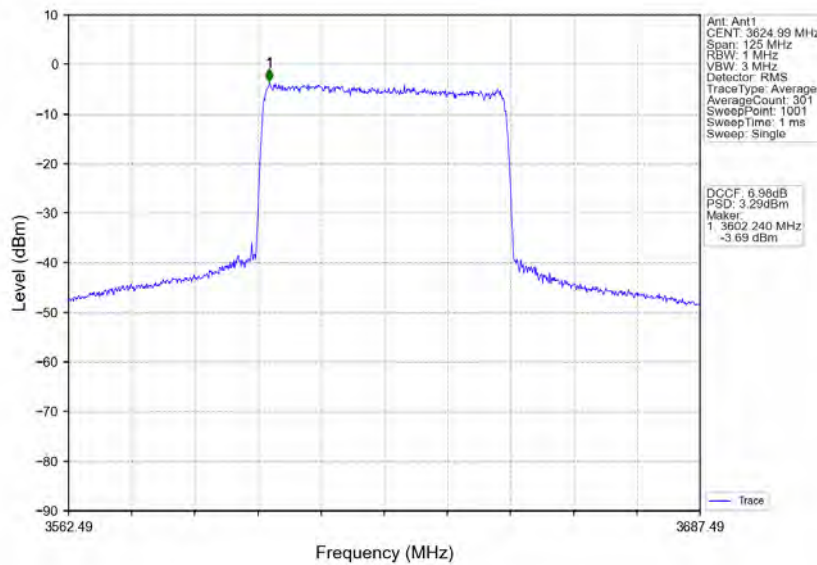
n78d_30kHz_MIMO_NTNV_50MHz_CP-OFDM 64 QAM_3624.99MHz_Inner_Full
