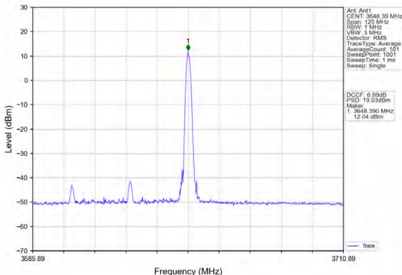
n78d_30kHz_MIMO_NTNV_50MHz_CP-OFDM QPSK_3624.99MHz_Inner_1RB_Right
