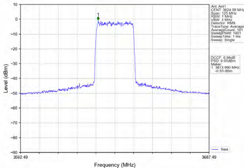
n78d_30kHz_MIMO_NTNV_50MHz_CP-OFDM 256 QAM_3624.99MHz_Inner_Full
