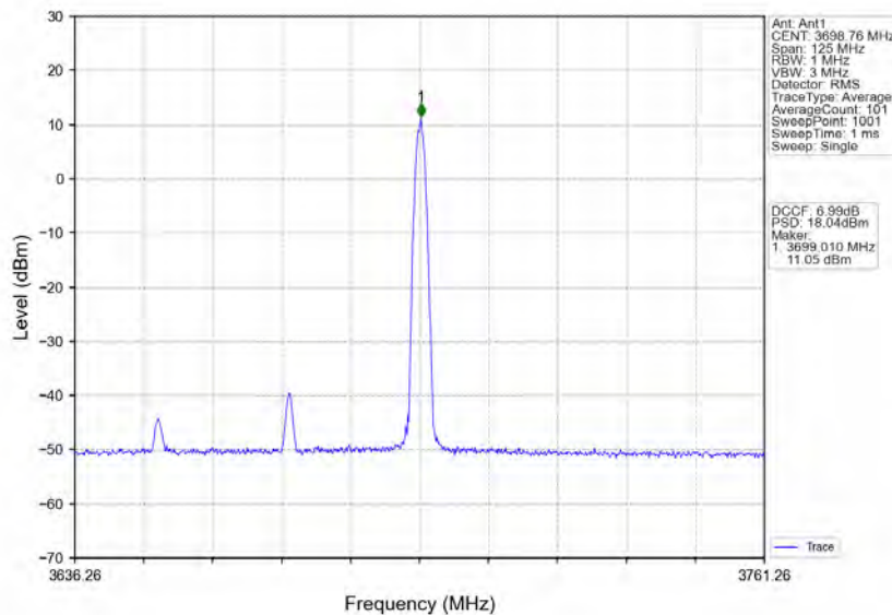
n78d_30kHz_MIMO_NTNV_50MHz_CP-OFDM 256 QAM_3675MHz_Edge_1RB_Right
