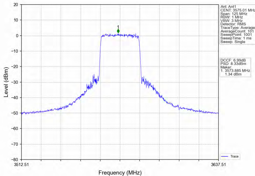
n78d_30kHz_MIMO_NTNV_50MHz_CP-OFDM 16 QAM_3575.01MHz_Inner_Full
