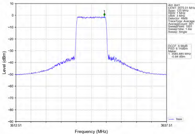
n78d_30kHz_MIMO_NTNV_50MHz_CP-OFDM 64 QAM_3575.01MHz_Inner_Full
