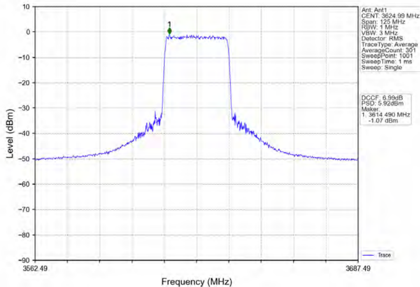
n78d_30kHz_MIMO_NTNV_50MHz_CP-OFDM 16 QAM_3624.99MHz_Inner_Full
