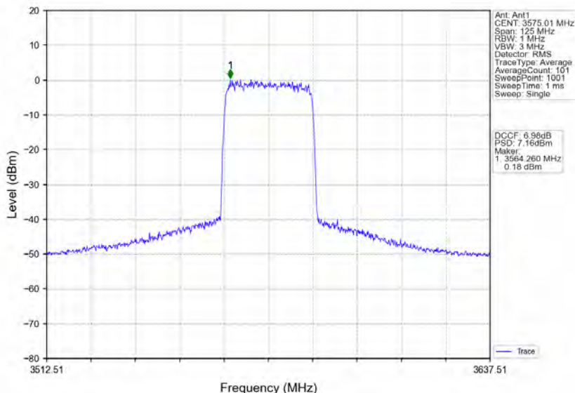
n78d_30kHz_MIMO_NTNV_50MHz_CP-OFDM 256 QAM_3575.01MHz_Inner_Full
