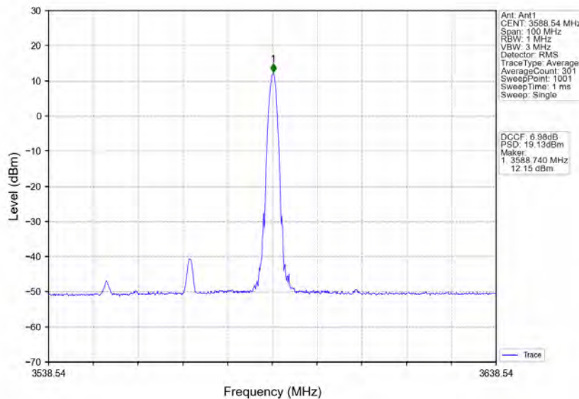
n78d_30kHz_MIMO_NTNV_40MHz_CP-OFDM_16 QAM_3570MHz_Inner_1RB_Right
