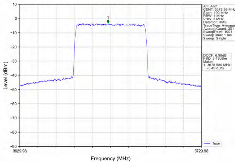
n78d_30kHz_MIMO_NTNV_40MHz_CP-OFDM 64 QAM_3679.98MHz_Inner_Full
