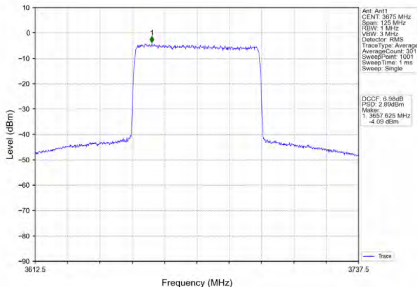
n78d_30kHz_MIMO_NTNV_50MHz_CP-OFDM QPSK_3675MHz_Inner_Full
