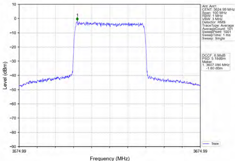
n78d_30kHz_MIMO_NTNV_40MHz_CP-OFDM 16 QAM_3624.99MHz_Inner_Full
