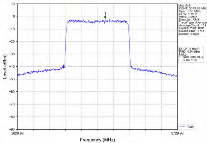
n78d_30kHz_MIMO_NTNV_40MHz_CP-OFDM QPSK_3679.98MHz_Inner_Full
