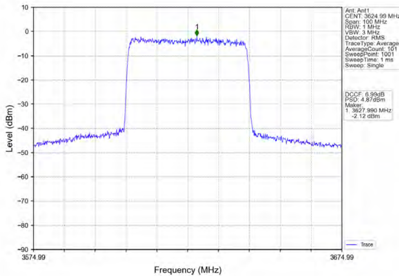
n78d_30kHz_MIMO_NTNV_40MHz_CP-OFDM QPSK_3624.99MHz_Inner_Full
