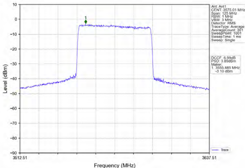
n78d_30kHz_MIMO_NTNV_50MHz_CP-OFDM 64 QAM_3575.01MHz_Inner_Full
