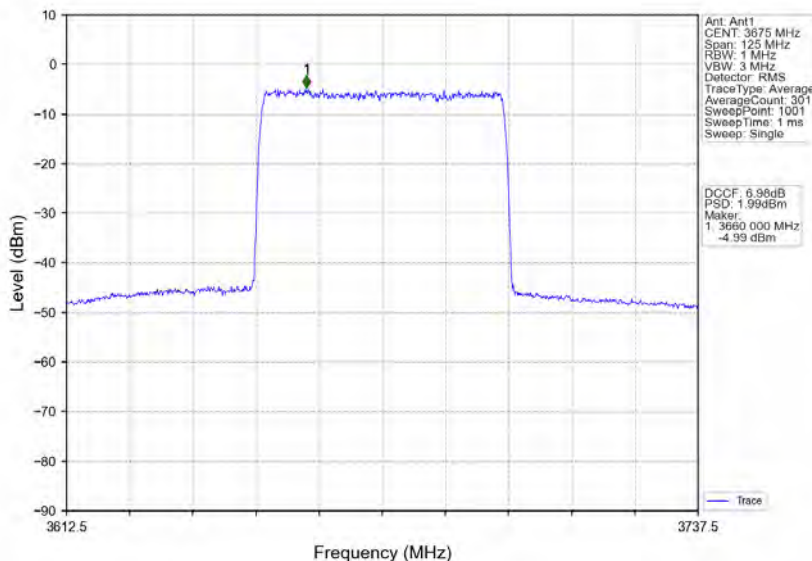
n78d_30kHz_MIMO_NTNV_50MHz_CP-OFDM_256_QAM_3675MHz_Inner_Full
