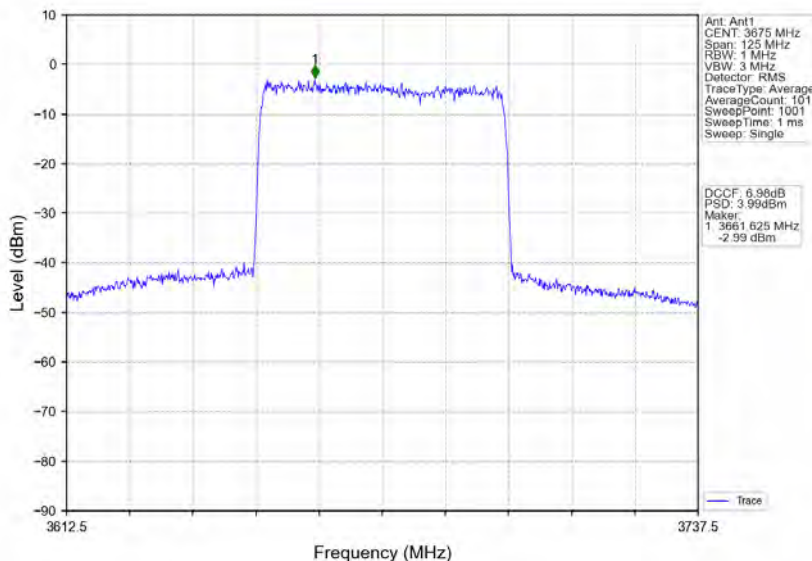
n78d_30kHz_MIMO_NTNV_50MHz_CP-OFDM QPSK_3675MHz_Inner_Full
