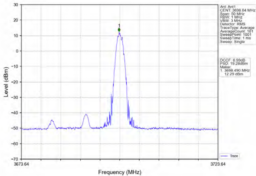
n78d_30kHz_MIMO_NTNV_20MHz_CP-OFDM 256 QAM_3690MHz_Inner_1RB_Right
