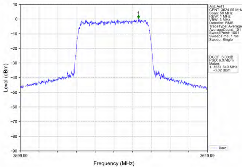
n78d_30kHz_MIMO_NTNV_20MHz_CP-OFDM QPSK_3624.99MHz_Inner_Full
