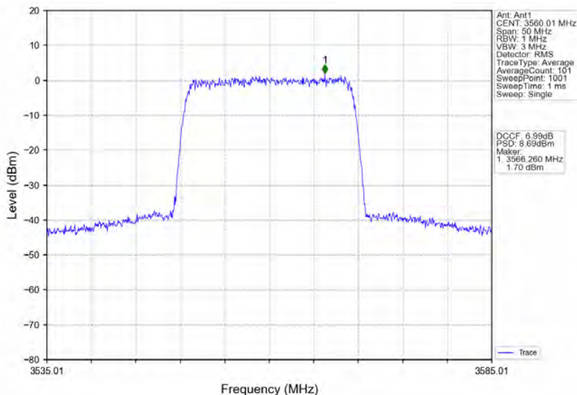
n78d_30kHz_MIMO_NTNV_20MHz_CP-OFDM 256 QAM_3560.01MHz_Inner_Full
