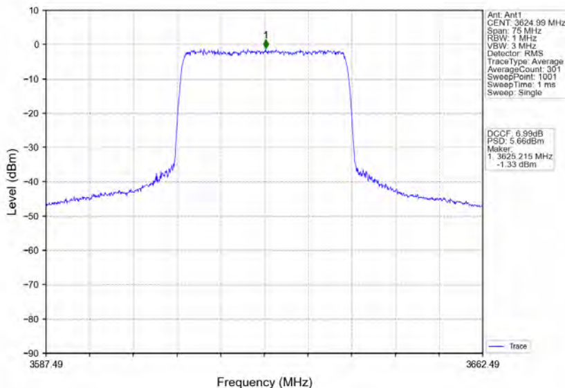
n78d_30kHz_MIMO_NTNV_30MHz_CP-OFDM 16 QAM_3624.99MHz_Inner_Full
