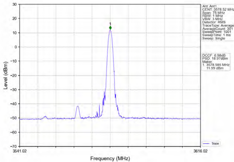
n78d_30kHz_MIMO_NTNV_30MHz_CP-OFDM QPSK_3565.02MHz_Inner_1RB_Right
