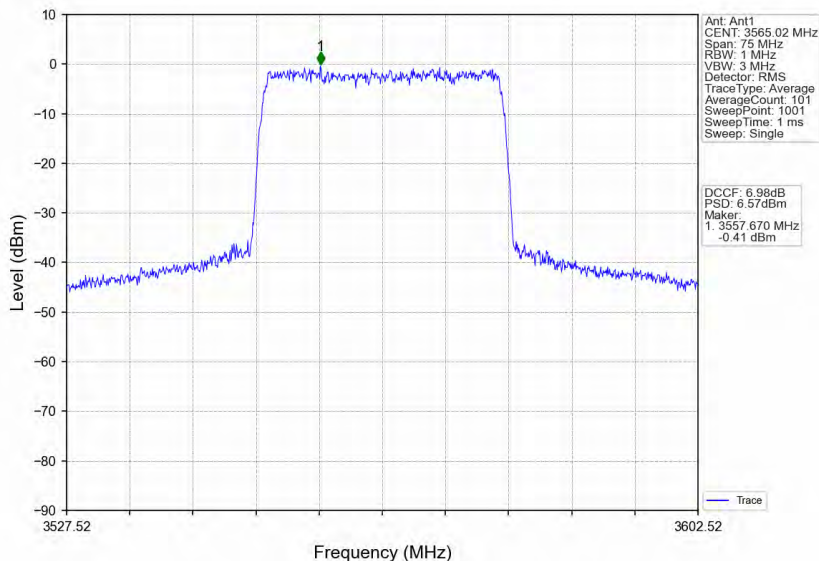
n78d_30kHz_MIMO_NTNV_30MHz_CP-OFDM 16 QAM_3565.02MHz_Inner_Full
