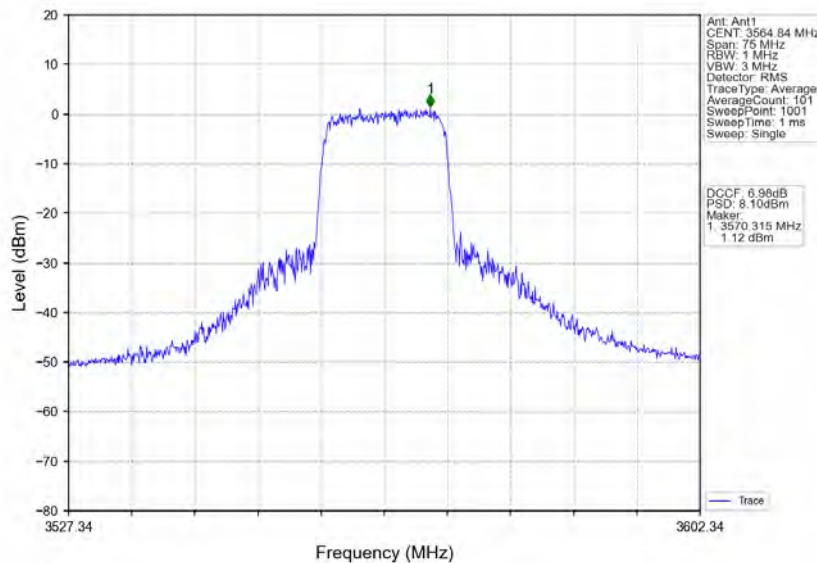
n78d_30kHz_MIMO_NTNV_30MHz_CP-OFDM QPSK_3565.02MHz_Inner_Full
