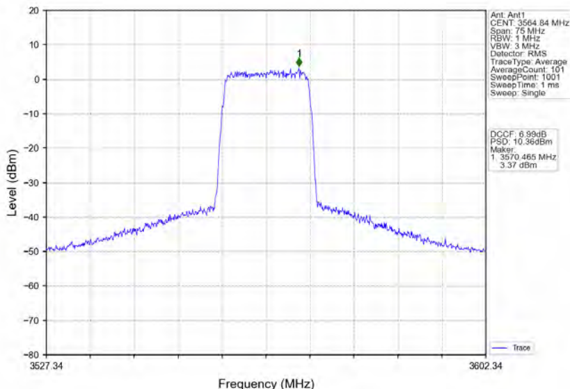
n78d_30kHz_MIMO_NTNV_30MHz_CP-OFDM 256 QAM_3565.02MHz_Inner_Full
