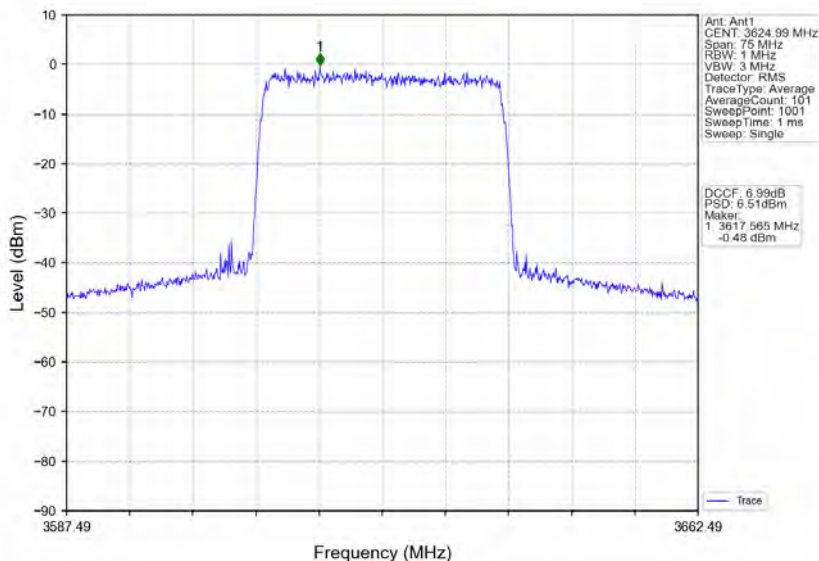
n78d_30kHz_MIMO_NTNV_30MHz_CP-OFDM 64 QAM_3624.99MHz_Inner_Full
