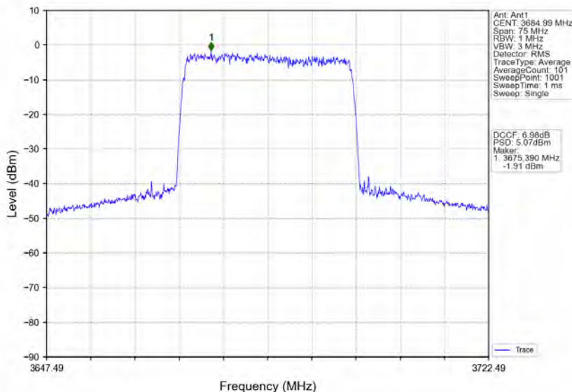
n78d_30kHz_MIMO_NTNV_30MHz_CP-OFDM 64 QAM_3684.99MHz_Inner_Full
