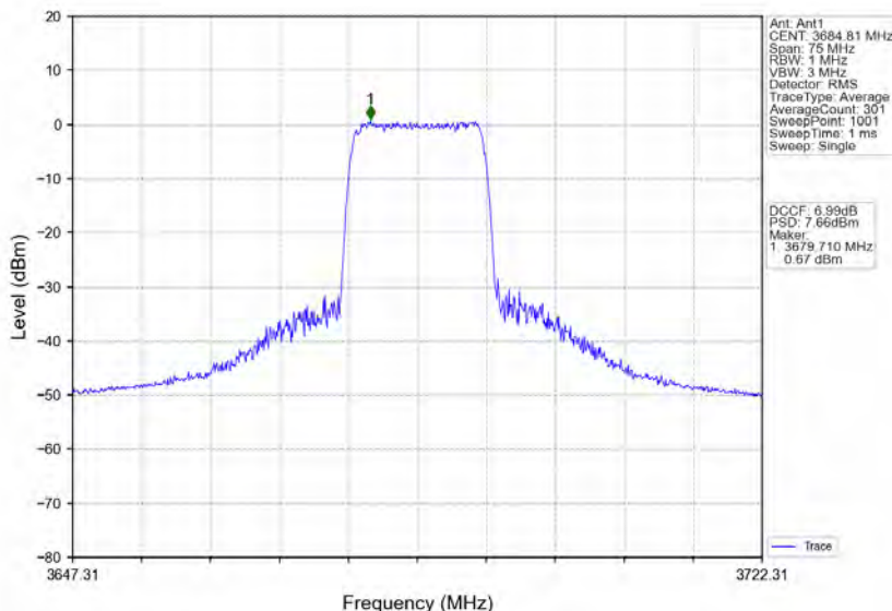
n78d_30kHz_MIMO_NTNV_30MHz_CP-OFDM 16 QAM_3684.99MHz_Inner_Full
