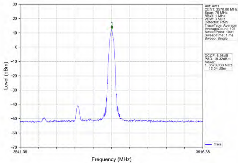
n78d_30kHz_MIMO_NTNV_30MHz_CP-OFDM 16 QAM_3565.02MHz_Edge_1RB_Right
