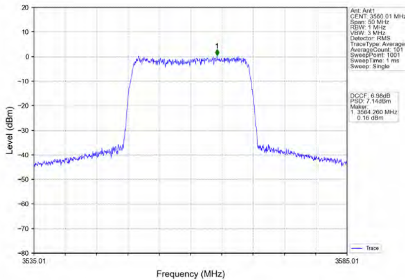
n78d_30kHz_MIMO_NTNV_20MHz_CP-OFDM QPSK_3560.01MHz_Inner_Full
