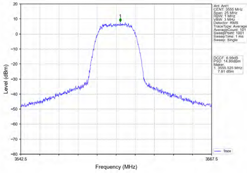
n78d_30kHz_MIMO_NTNV_10MHz_CP-OFDM_256_QAM_3555MHz_Inner_Full
