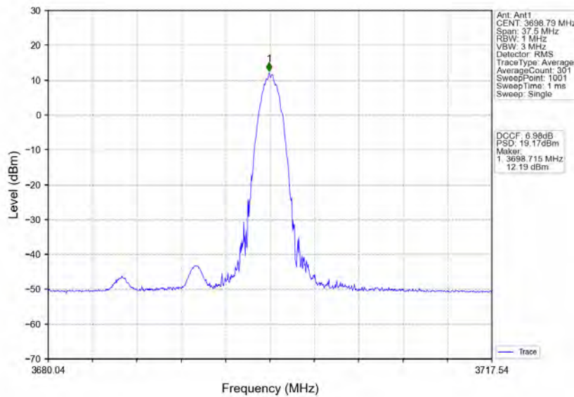
n78d_30kHz_MIMO_NTNV_15MHz_CP-OFDM_16 QAM_3692.49MHz_Inner_1RB_Right
