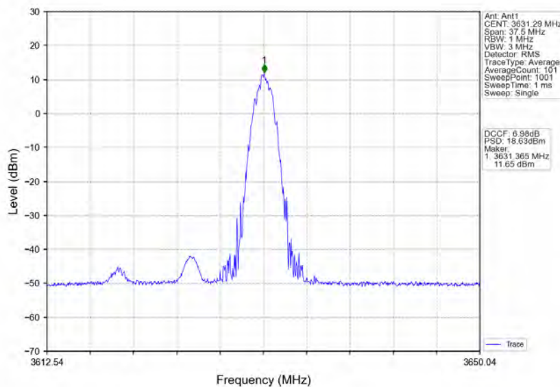
n78d_30kHz_MIMO_NTNV_15MHz_CP-OFDM 256 QAM_3624.99MHz_Inner_1RB_Right
