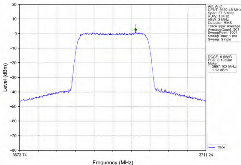
n78d_30kHz_MIMO_NTNV_15MHz_CP-OFDM 64 QAM_3692.49MHz_Inner_Full
