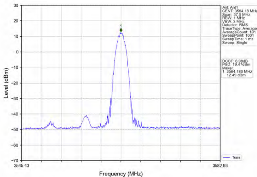
n78d_30kHz_MIMO_NTNV_15MHz_CP-OFDM 256 QAM_3557.52MHz_Edge_1RB_Right
