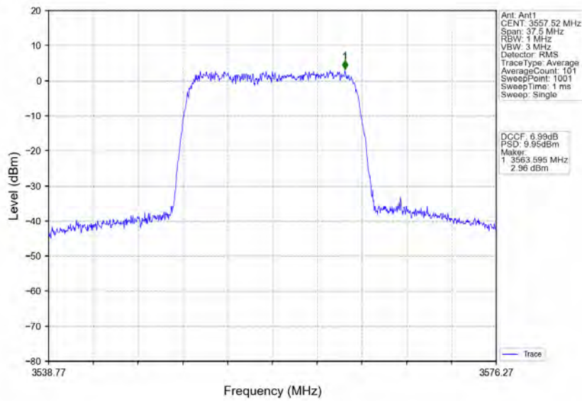
n78d_30kHz_MIMO_NTNV_15MHz_CP-OFDM 256 QAM_3557.52MHz_Inner_Full
