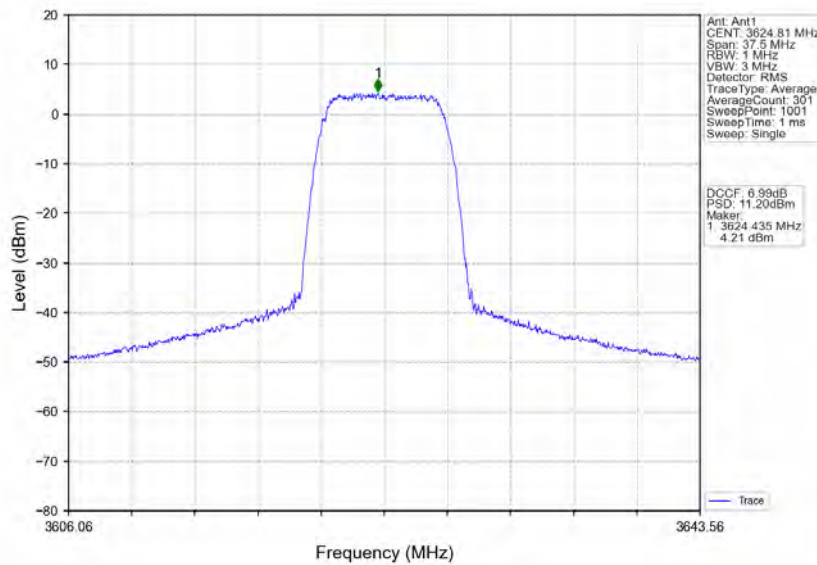
n78d_30kHz_MIMO_NTNV_15MHz_CP-OFDM 256 QAM_3624.99MHz_Inner_Full
