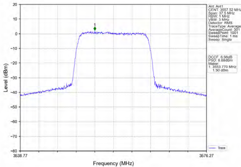
n78d_30kHz_MIMO_NTNV_15MHz_CP-OFDM 64 QAM_3557.52MHz_Inner_Full
