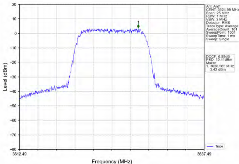
n78d_30kHz_MIMO_NTNV_10MHz_CP-OFDM 64 QAM_3624.99MHz_Inner_Full
