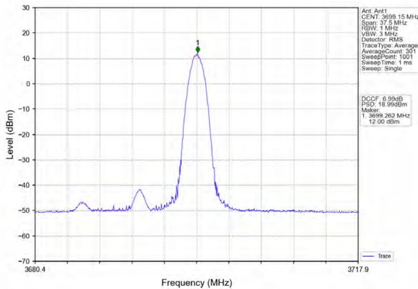
n78d_30kHz_MIMO_NTNV_15MHz_CP-OFDM 16 QAM_3692.49MHz_Edge_1RB_Right
