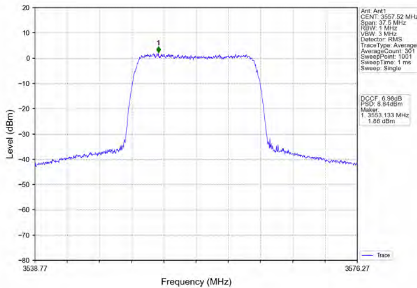
n78d_30kHz_MIMO_NTNV_15MHz_CP-OFDM 16 QAM_3557.52MHz_Inner_Full
