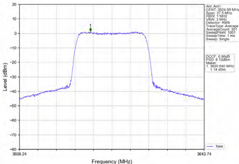
n78d_30kHz_MIMO_NTNV_15MHz_CP-OFDM 16 QAM_3624.99MHz_Inner_Full
