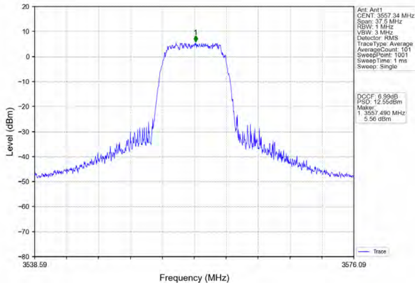
n78d_30kHz_MIMO_NTNV_15MHz_CP-OFDM 64 QAM_3557.52MHz_Inner_Full
