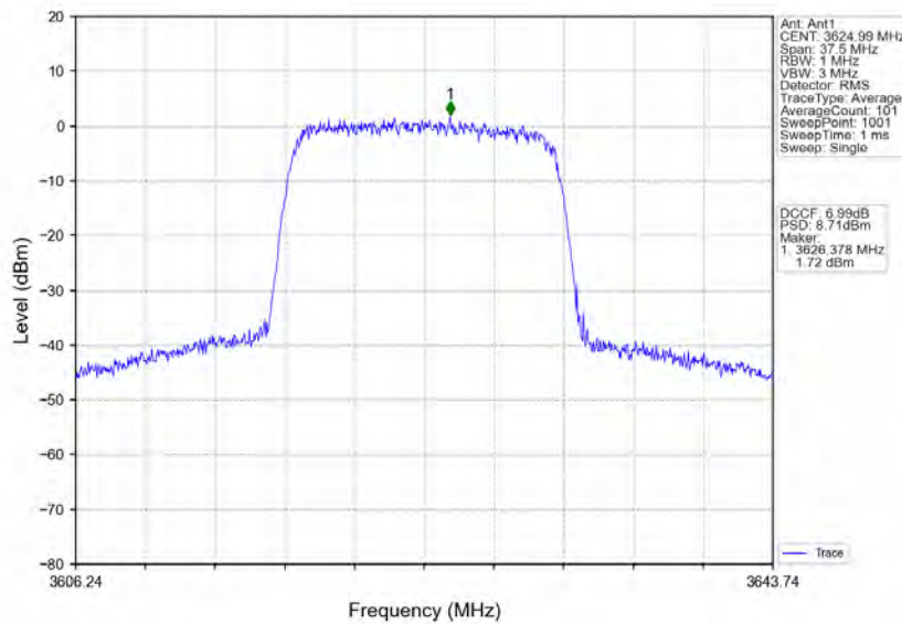
n78d_30kHz_MIMO_NTNV_15MHz_CP-OFDM QPSK_3624.99MHz_Inner_Full
