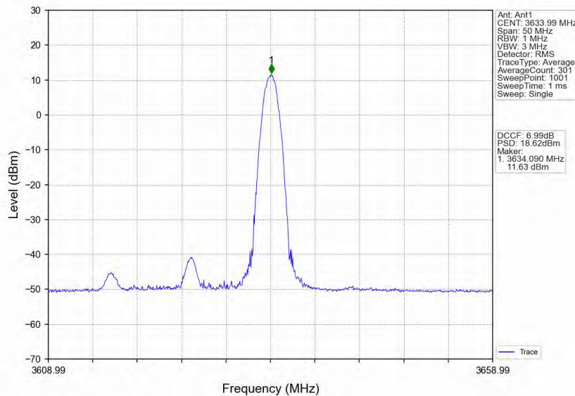
n78d_30kHz_MIMO_NTNV_20MHz_CP-OFDM 16 QAM_3624.99MHz_Edge_1RB_Right
