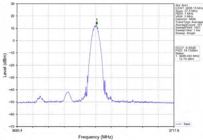
n78d_30kHz_MIMO_NTNV_15MHz_CP-OFDM 64 QAM_3692.49MHz_Edge_1RB_Right
