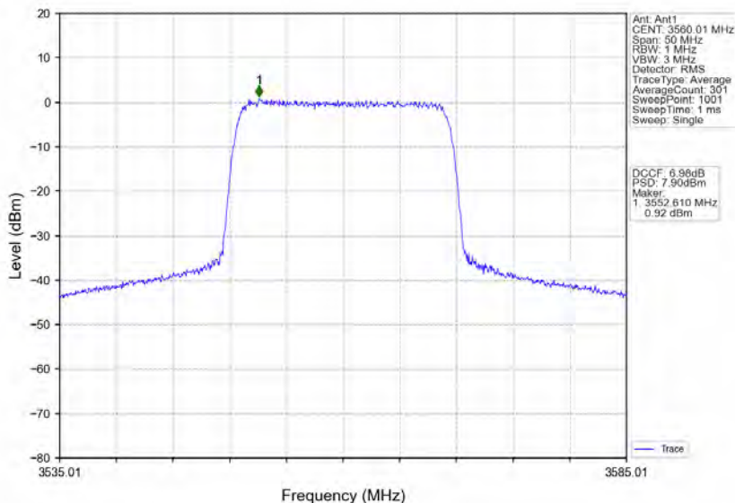
n78d_30kHz_MIMO_NTNV_20MHz_CP-OFDM 16 QAM_3560.01MHz_Inner_Full
