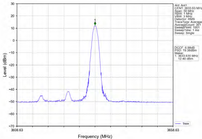
n78d_30kHz_MIMO_NTNV_20MHz_CP-OFDM 16 QAM_3624.99MHz_Inner_1RB_Right
