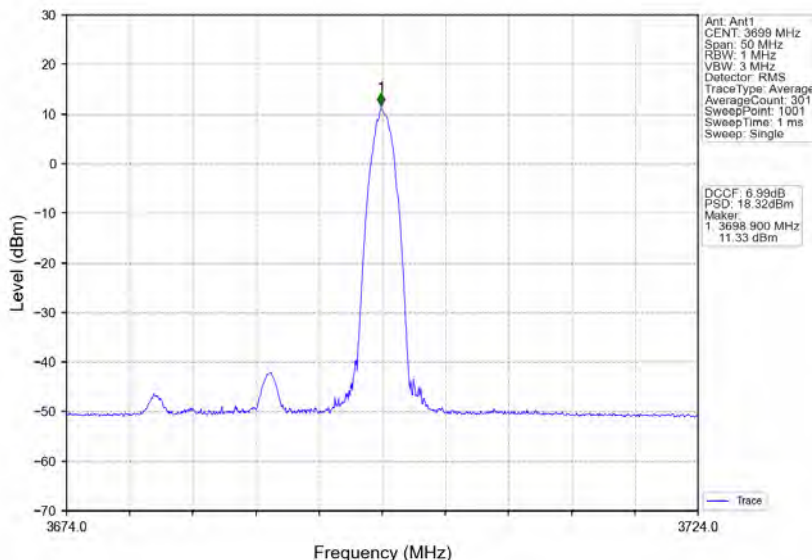
n78d_30kHz_MIMO_NTNV_20MHz_CP-OFDM QPSK_3690MHz_Edge_1RB_Right
