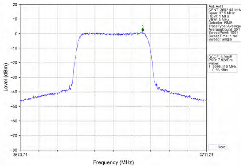
n78d_30kHz_MIMO_NTNV_15MHz_CP-OFDM 16 QAM_3692.49MHz_Inner_Full
