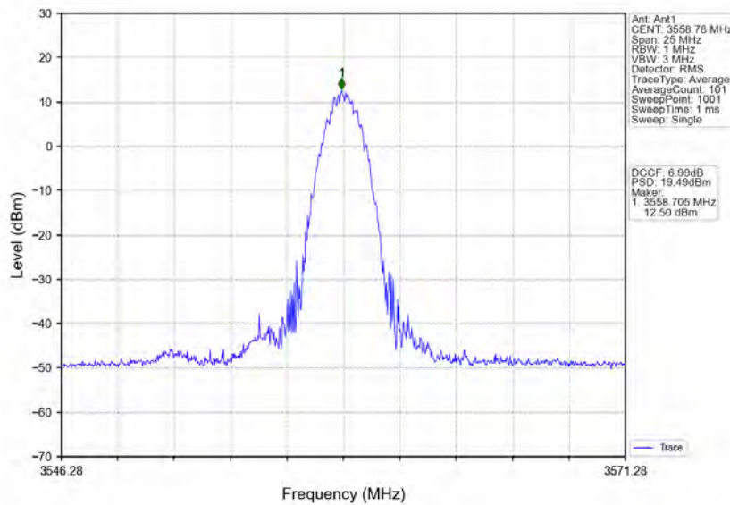
n78d_30kHz_MIMO_NTNV_10MHz_CP-OFDM QPSK_3558MHz_Inner_1RB_Right
