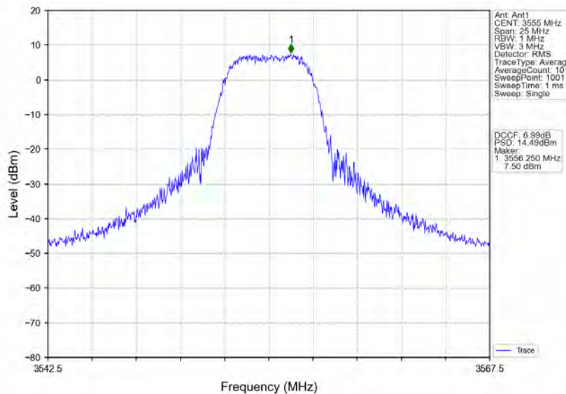
n78d_30kHz_MIMO_NTNV_10MHz_CP-OFDM 16 QAM_3555MHz_Inner_Full
