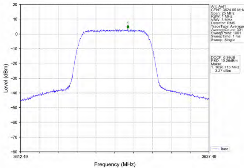
n78d_30kHz_MIMO_NTNV_10MHz_CP-OFDM QPSK_3624.99MHz_Inner_Full
