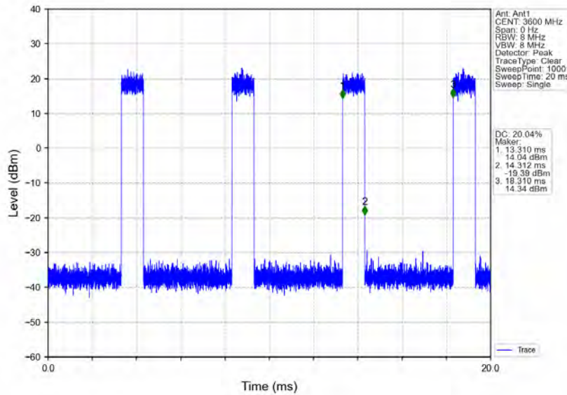
n78d_30kHz_MIMO_NTNV_100MHz_CP-OFDM 16 QAM_3600MHz_Inner_Full
