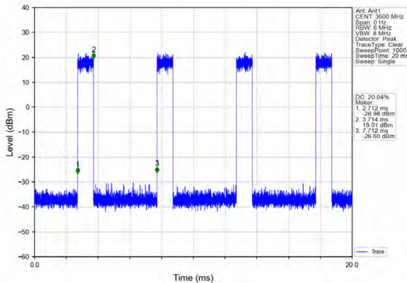
n78d_30kHz_MIMO_NTNV_100MHz_CP-OFDM_256_QAM_3600MHz_Inner_Full
