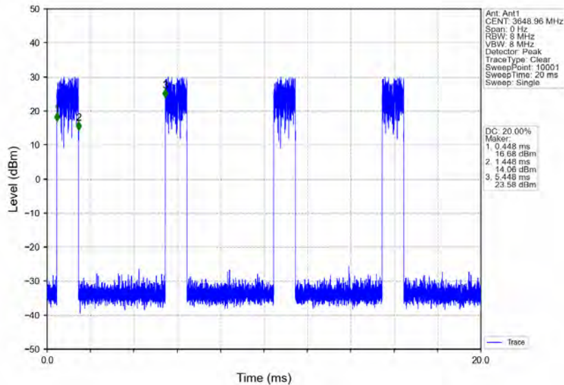
n78d_30kHz_MIMO_NTNV_100MHz_CP-OFDM 64 QAM_3600MHz_Edge_1RB_Right
