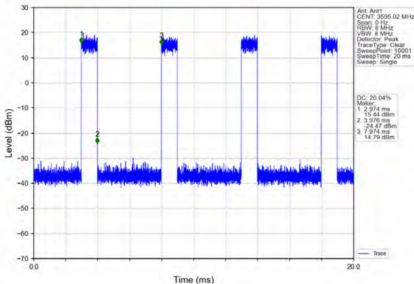
n78d_30kHz_MIMO_NTNV_90MHz_CP-OFDM 256 QAM_3595.02MHz_Inner_Full
