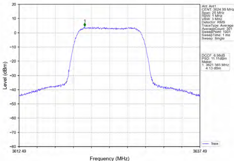
n78d_30kHz_MIMO_NTNV_10MHz_CP-OFDM 16 QAM_3624.99MHz_Inner_Full
