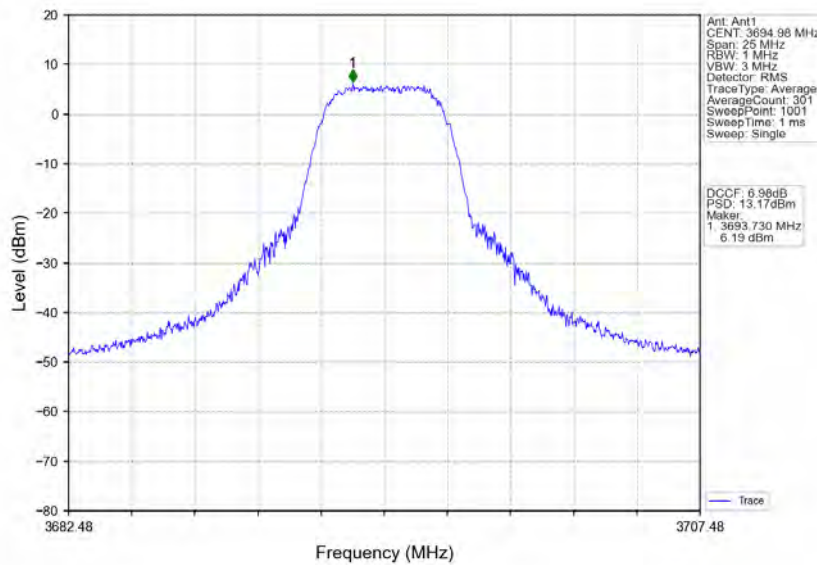
n78d_30kHz_MIMO_NTNV_10MHz_CP-OFDM_QPSK_3694.98MHz_Inner_Full
