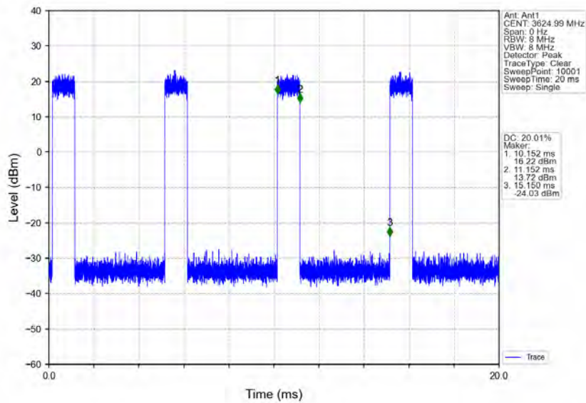
n78d_30kHz_MIMO_NTNV_100MHz_CP-OFDM_16 QAM_3624.99MHz_Inner_Full
