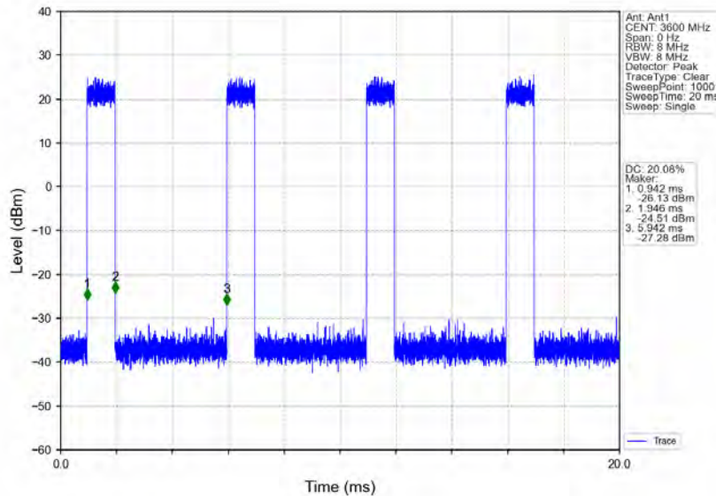
n78d_30kHz_MIMO_NTNV_100MHz_CP-OFDM 16 QAM_3600MHz_Inner_Full
