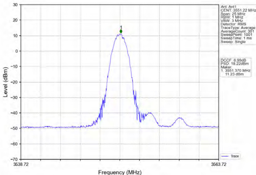
n78d_30kHz_MIMO_NTNV_10MHz_CP-OFDM 256 QAM_3555MHz_Inner_1RB_Right
