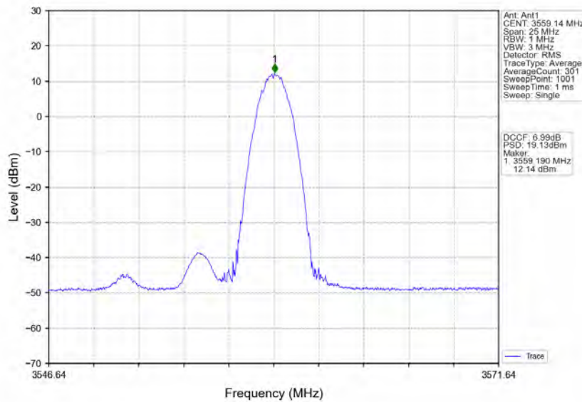
n78d_30kHz_MIMO_NTNV_10MHz_CP-OFDM 256 QAM_3555MHz_Edge_1RB_Right
