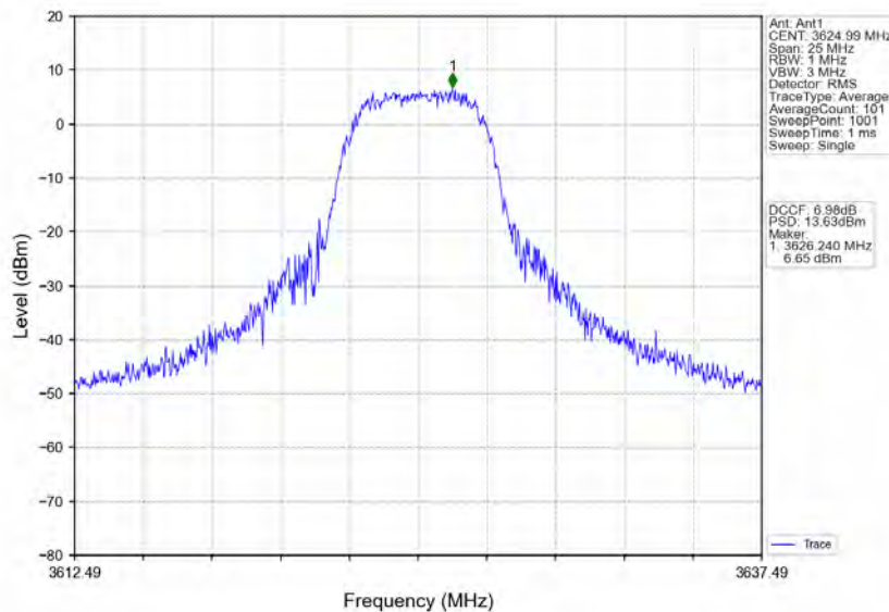
n78d_30kHz_MIMO_NTNV_10MHz_CP-OFDM 16 QAM_3624.99MHz_Inner_Full
