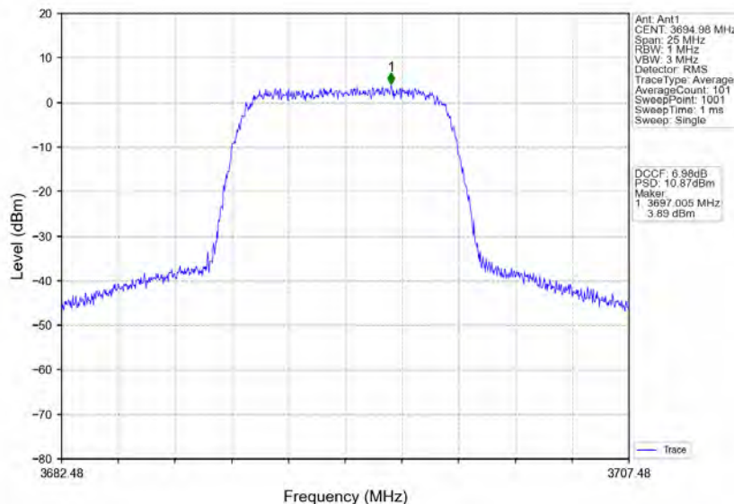
n78d_30kHz_MIMO_NTNV_10MHz_CP-OFDM_QPSK_3694.98MHz_Inner_Full
