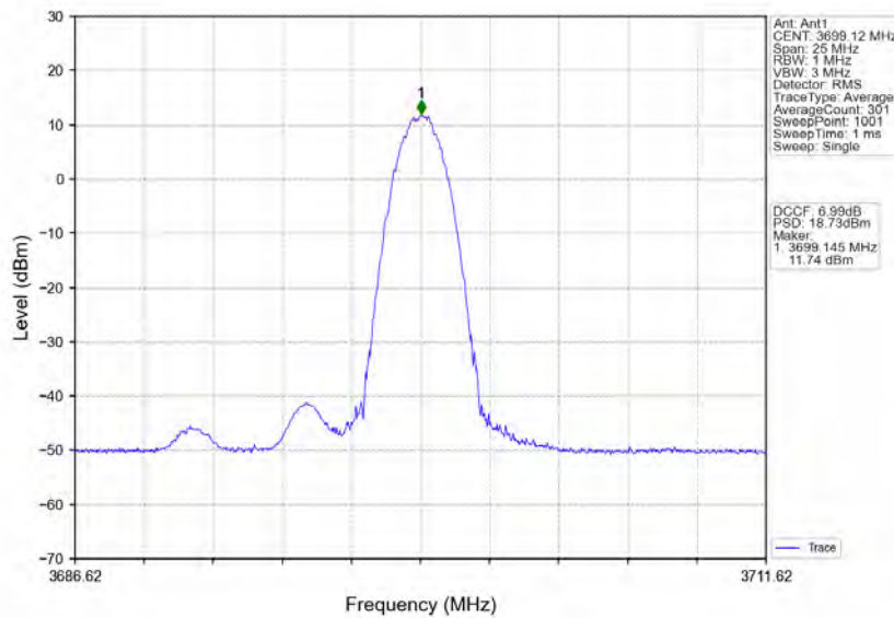
n78d_30kHz_MIMO_NTNV_10MHz_CP-OFDM 64 QAM_3694.98MHz_Edge_1RB_Right
