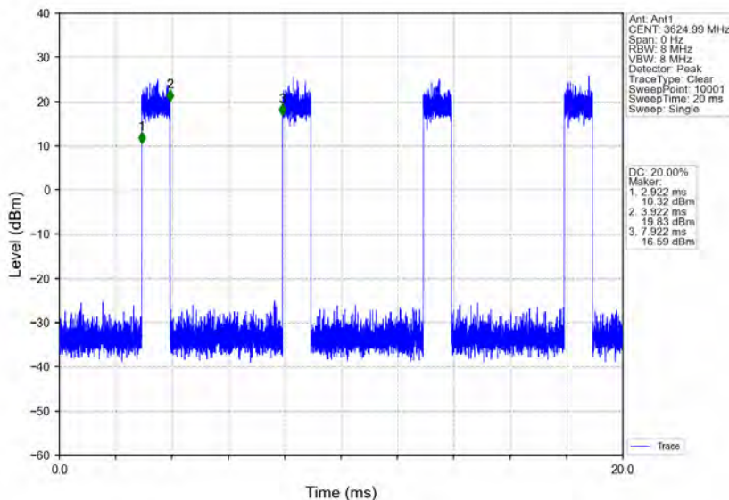
n78d_30kHz_MIMO_NTNV_90MHz_CP-OFDM_16_QAM_3624.99MHz_Inner_Full
