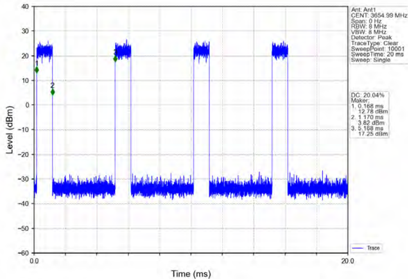
n78d_30kHz_MIMO_NTNV_90MHz_CP-OFDM_16_QAM_3654.99MHz_Inner_Full
