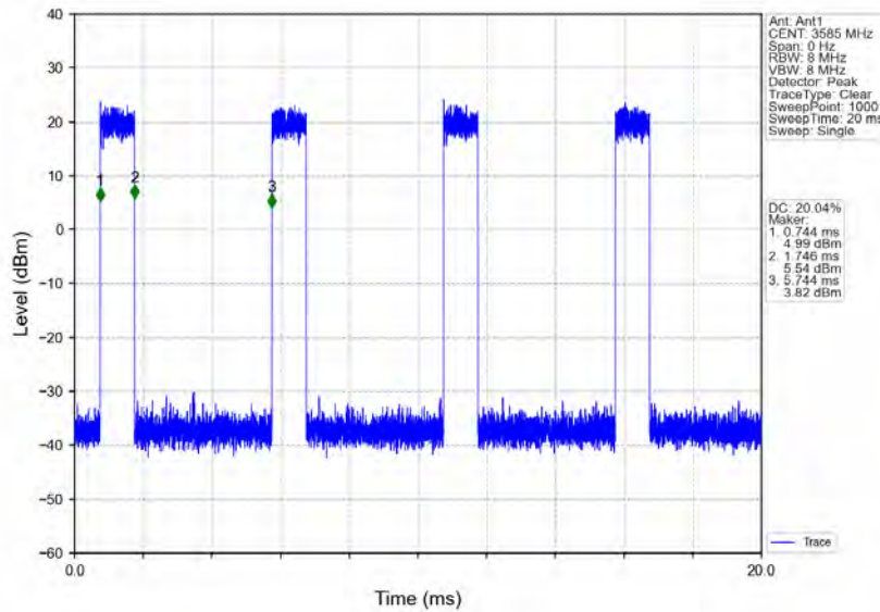
n78d_30kHz_MIMO_NTNV_70MHz_CP-OFDM 16 QAM_3585MHz_Inner_Full
