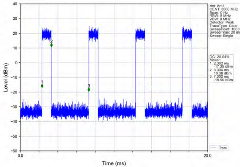
n78d_30kHz_MIMO_NTNV_80MHz_CP-OFDM QPSK_3660MHz_Inner_Full
