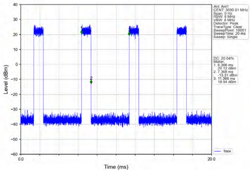
n78d_30kHz_MIMO_NTNV_80MHz_CP-OFDM 16 QAM_3590.01MHz_Inner_Full
