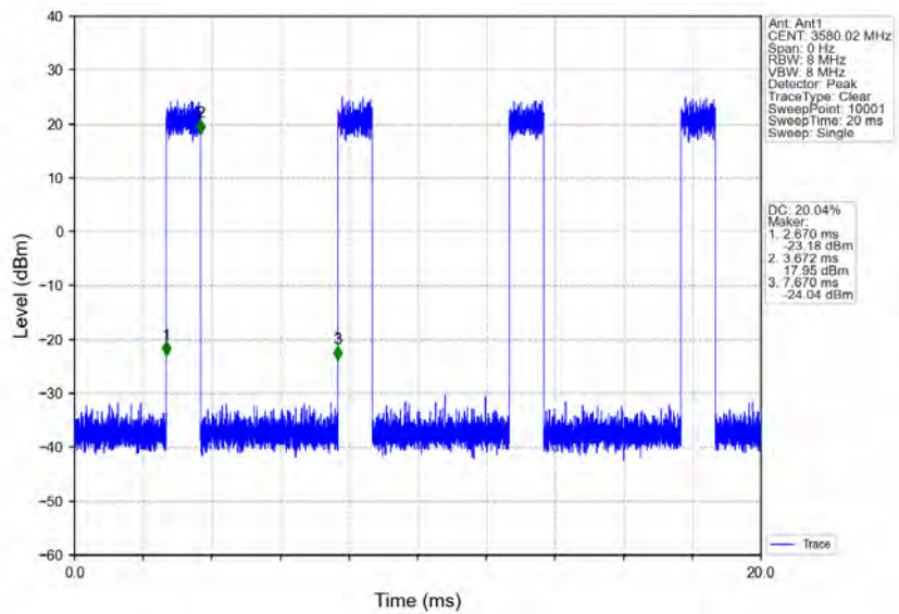
n78d_30kHz_MIMO_NTNV_60MHz_CP-OFDM 16 QAM_3580.02MHz_Inner_Full
