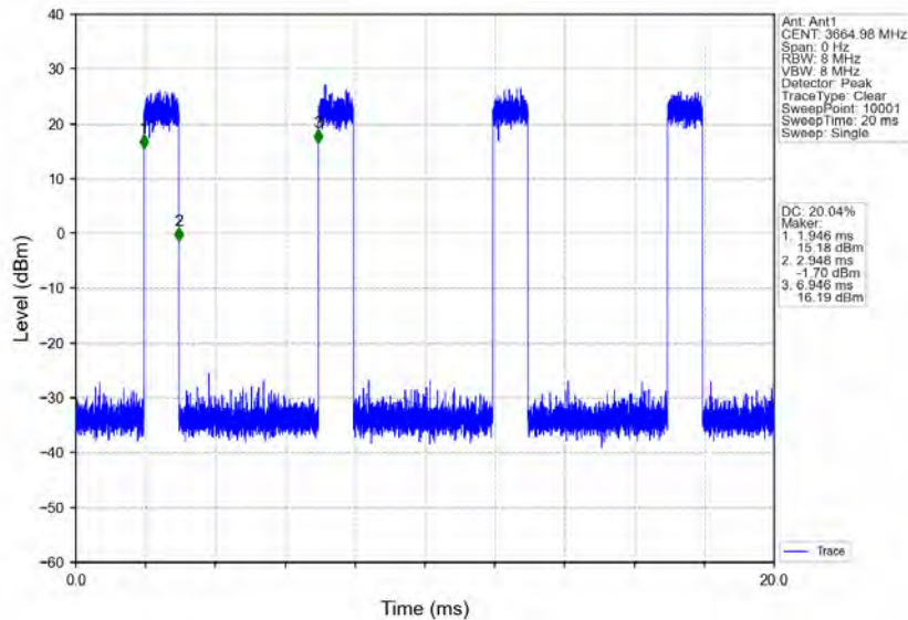
n78d_30kHz_MIMO_NTNV_70MHz_CP-OFDM 64 QAM_3664.98MHz_Inner_Full
