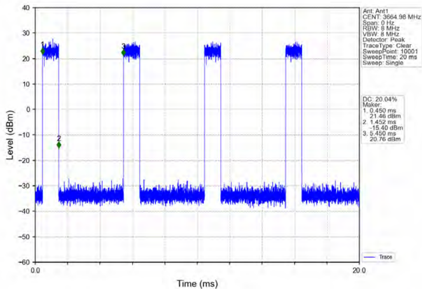
n78d_30kHz_MIMO_NTNV_70MHz_CP-OFDM_QPSK_3664.98MHz_Inner_Full
