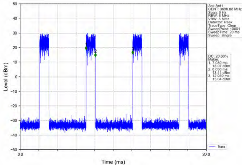
n78d_30kHz_MIMO_NTNV_80MHz_CP-OFDM_64_QAM_3660MHz_Edge_1RB_Right
