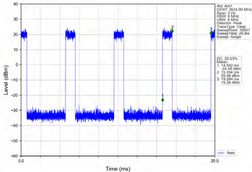
n78d_30kHz_MIMO_NTNV_70MHz_CP-OFDM 256 QAM_3624.99MHz_Inner_Full
