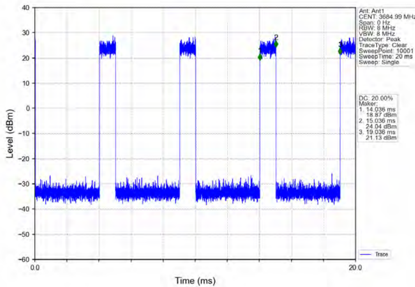
n78d_30kHz_MIMO_NTNV_30MHz_CP-OFDM 16 QAM_3684.99MHz_Inner_Full
