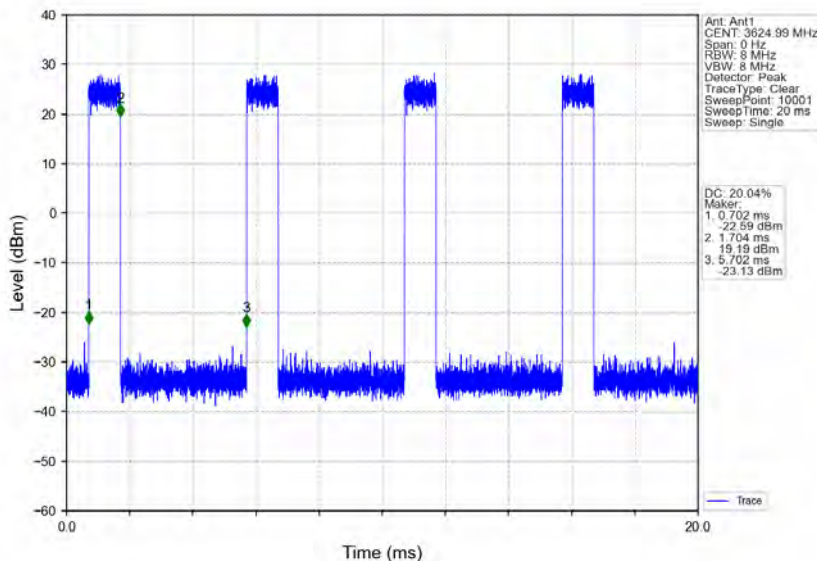
n78d_30kHz_MIMO_NTNV_30MHz_CP-OFDM QPSK_3624.99MHz_Inner_Full
