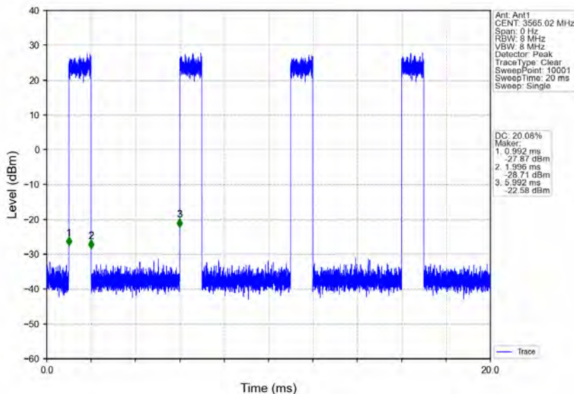
n78d_30kHz_MIMO_NTNV_30MHz_CP-OFDM_16_QAM_3565.02MHz_Inner_Full
