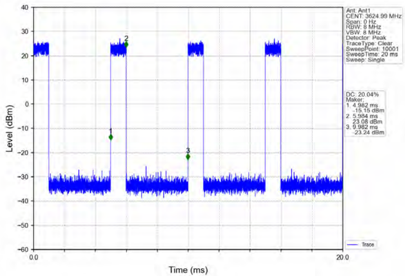
n78d_30kHz_MIMO_NTNV_40MHz_CP-OFDM 16 QAM_3624.99MHz_Inner_Full
