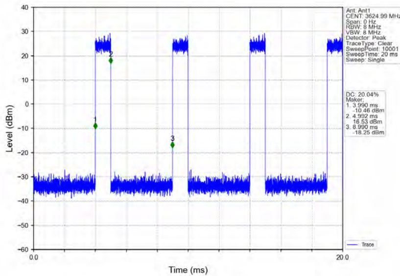
n78d_30kHz_MIMO_NTNV_30MHz_CP-OFDM 16 QAM_3624.99MHz_Inner_Full
