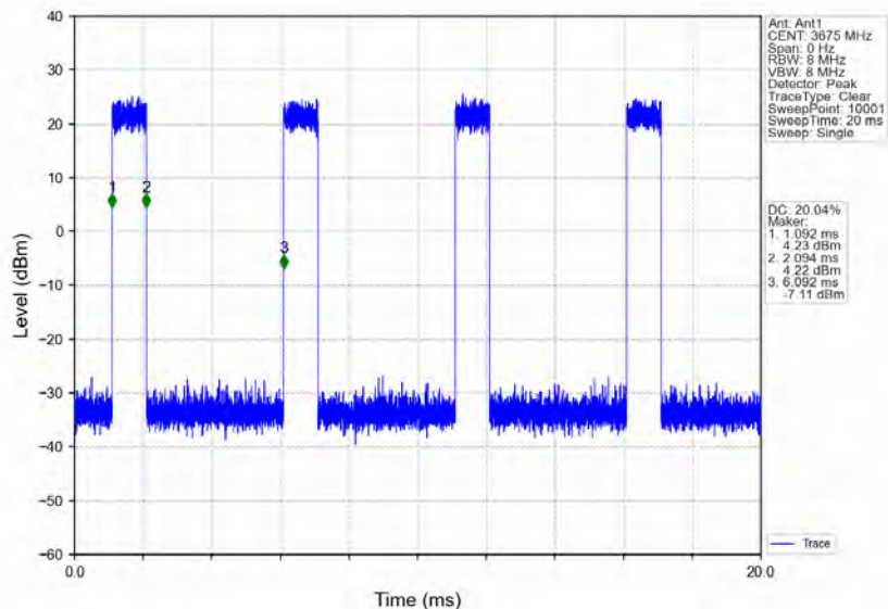
n78d_30kHz_MIMO_NTNV_50MHz_CP-OFDM 16 QAM_3675MHz_Inner_Full
