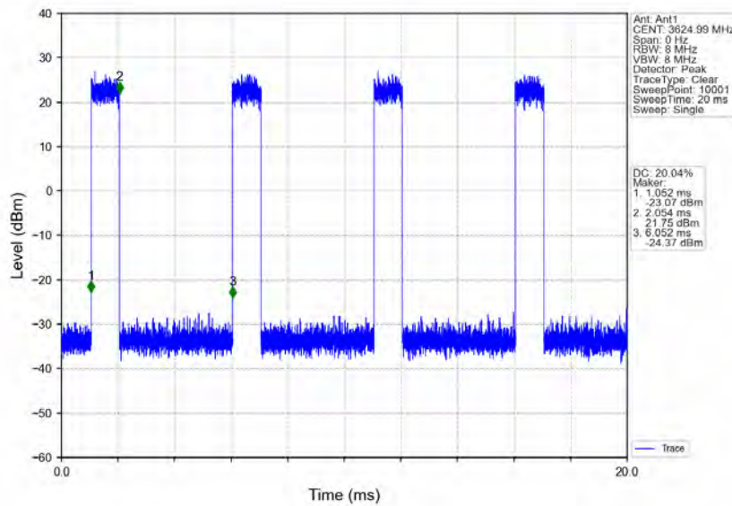
n78d_30kHz_MIMO_NTNV_40MHz_CP-OFDM 64 QAM_3624.99MHz_Inner_Full
