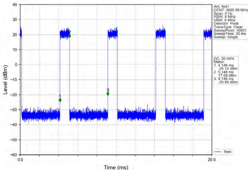
n78d_30kHz_MIMO_NTNV_60MHz_CP-OFDM_QPSK_3669.99MHz_Inner_Full
