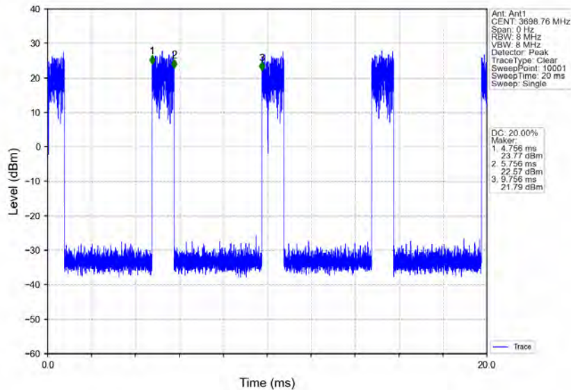
n78d_30kHz_MIMO_NTNV_50MHz_CP-OFDM 256 QAM_3675MHz_Edge_1RB_Right
