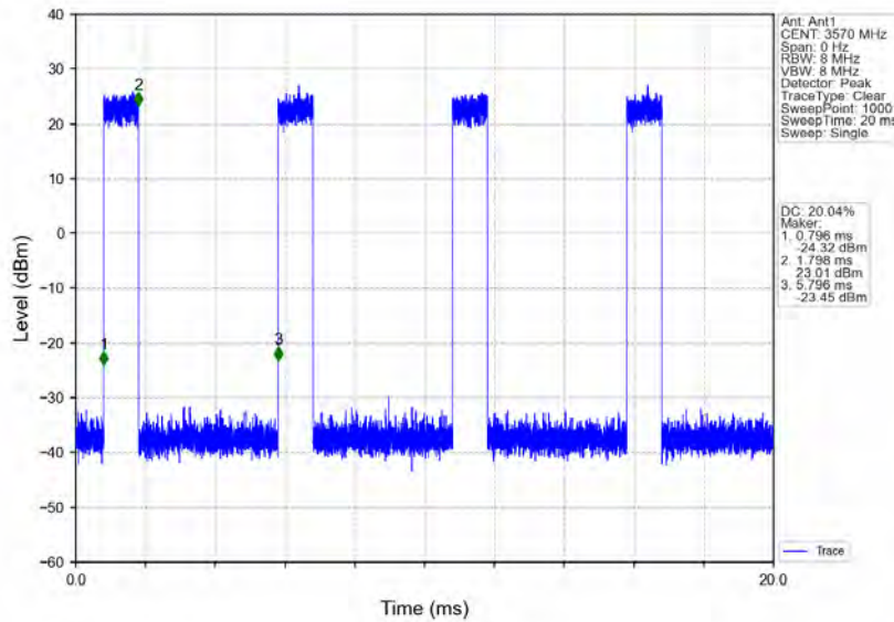
n78d_30kHz_MIMO_NTNV_40MHz_CP-OFDM 16 QAM_3570MHz_Inner_Full
