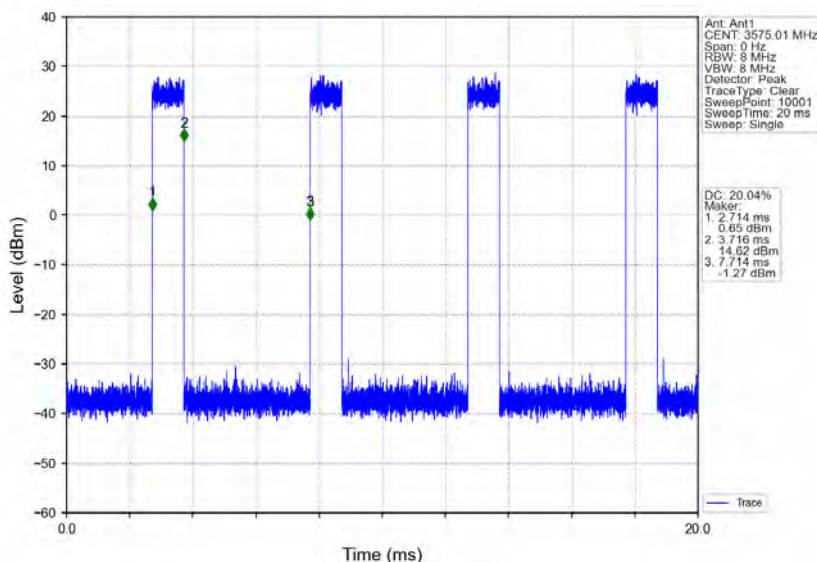
n78d_30kHz_MIMO_NTNV_50MHz_CP-OFDM_QPSK_3575.01MHz_Inner_Full
