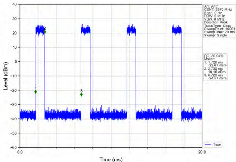
n78d_30kHz_MIMO_NTNV_40MHz_CP-OFDM 64 QAM_3570MHz_Inner_Full
