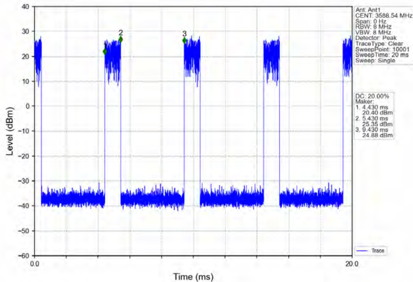
n78d_30kHz_MIMO_NTNV_40MHz_CP-OFDM 256 QAM_3570MHz_Inner_1RB_Right
