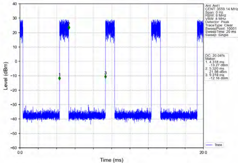
n78d_30kHz_MIMO_NTNV_10MHz_CP-OFDM_16 QAM_3555MHz_Edge_1RB_Right
