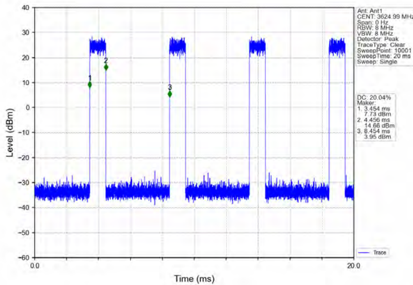
n78d_30kHz_MIMO_NTNV_10MHz_CP-OFDM 256 QAM_3624.99MHz_Inner_Full
