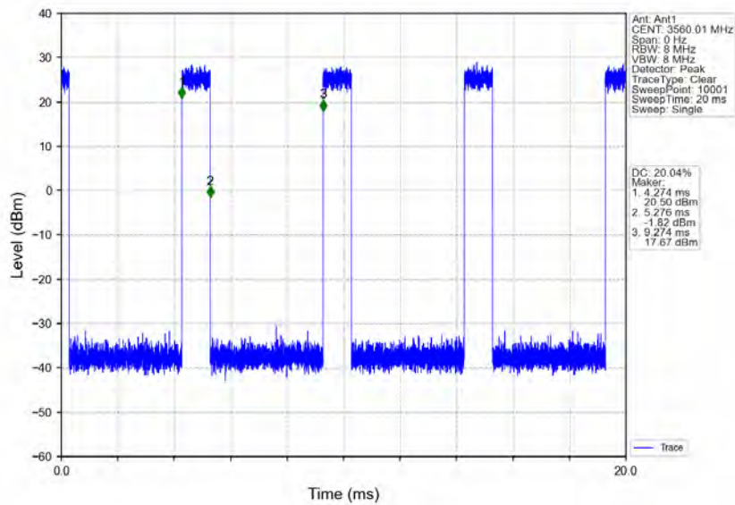
n78d_30kHz_MIMO_NTNV_20MHz_CP-OFDM QPSK_3560.01MHz_Inner_Full
