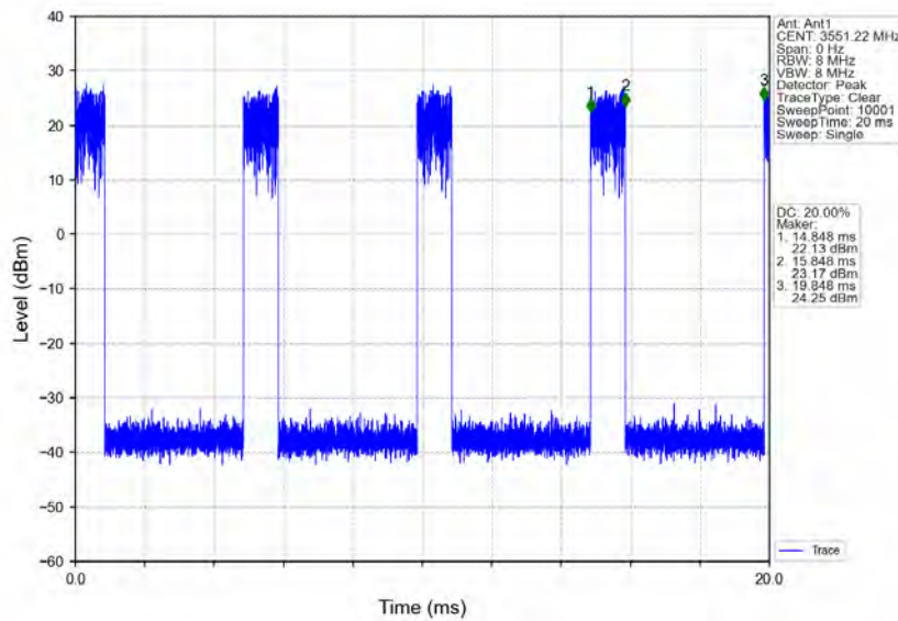
n78d_30kHz_MIMO_NTNV_10MHz_CP-OFDM 256 QAM_3555MHz_Inner_1RB_Right
