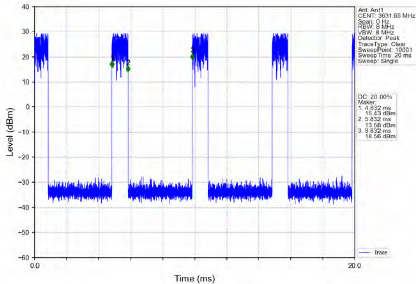
n78d_30kHz_MIMO_NTNV_15MHz_CP-OFDM 64 QAM_3624.99MHz_Edge_1RB_Right
