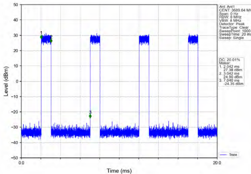
n78d_30kHz_MIMO_NTNV_20MHz_CP-OFDM 64 QAM_3690MHz_Inner_Full
