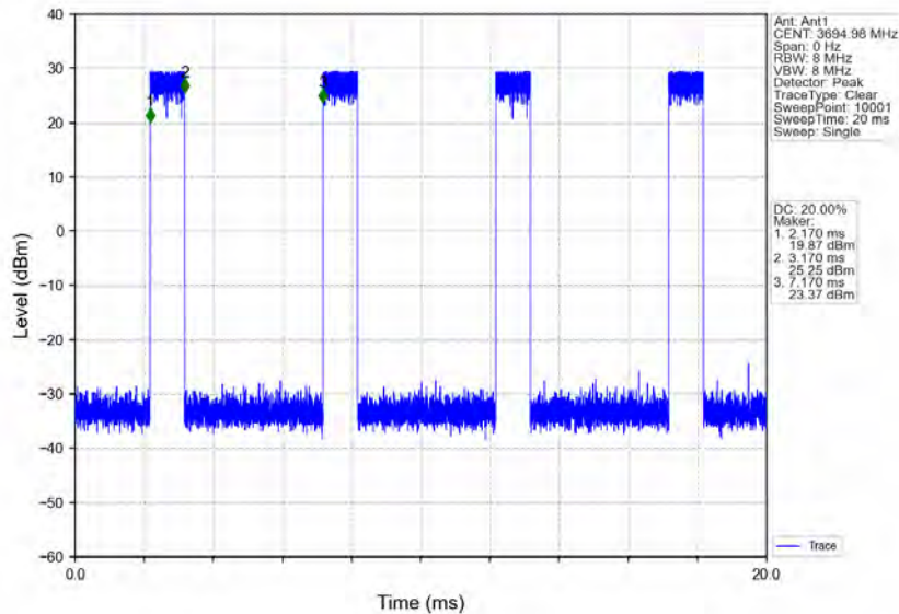
n78d_30kHz_MIMO_NTNV_10MHz_CP-OFDM 64 QAM_3694.98MHz_Inner_Full
