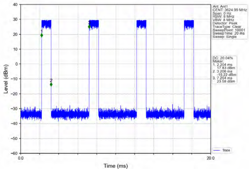
n78d_30kHz_MIMO_NTNV_10MHz_CP-OFDM 64 QAM_3624.99MHz_Inner_Full
