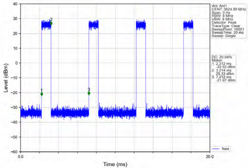
n78d_30kHz_MIMO_NTNV_20MHz_CP-OFDM 16 QAM_3624.99MHz_Inner_Full
