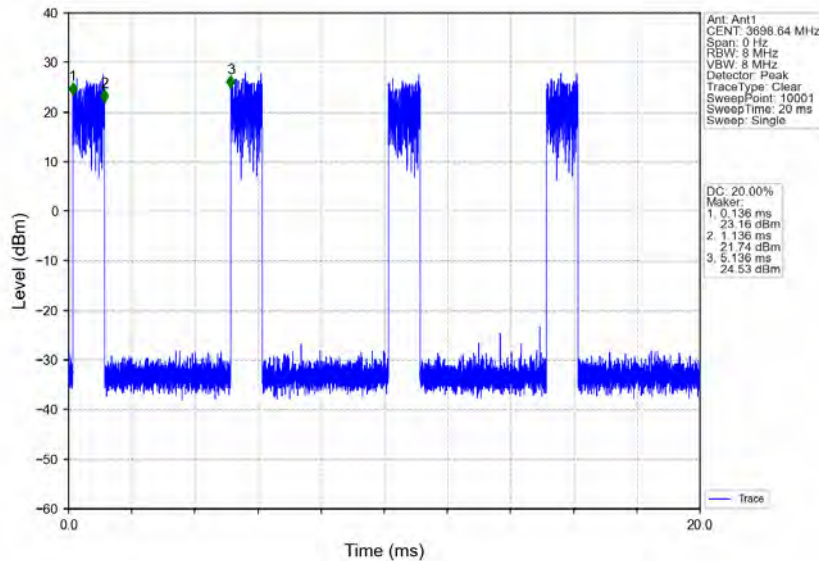
n78d_30kHz_MIMO_NTNV_20MHz_CP-OFDM 256 QAM_3690MHz_Inner_1RB_Right
