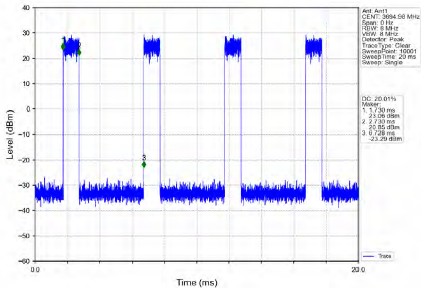
n78d_30kHz_MIMO_NTNV_10MHz_CP-OFDM 256 QAM_3694.98MHz_Inner_Full
