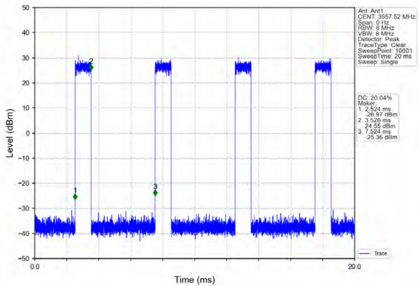
n78d_30kHz_MIMO_NTNV_15MHz_CP-OFDM_QPSK_3557.52MHz_Inner_Full
