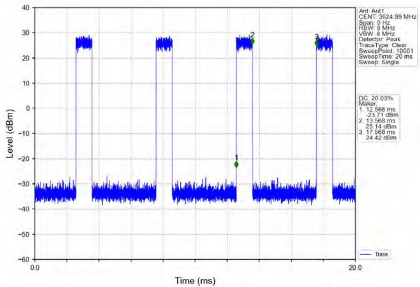
n78d_30kHz_MIMO_NTNV_20MHz_CP-OFDM_QPSK_3624.99MHz_Inner_Full
