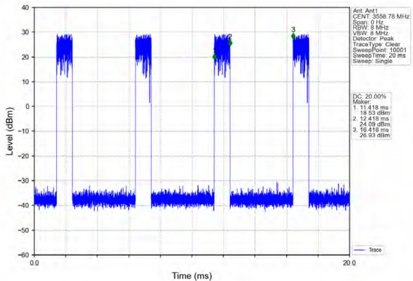
n78d_30kHz_MIMO_NTNV_10MHz_CP-OFDM QPSK_3555MHz_Inner_1RB_Right
