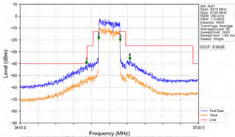
n48_30kHz_MIMO_NTNV_40MHz_CP-OFDM QPSK_3570MHz_Outer_Full
