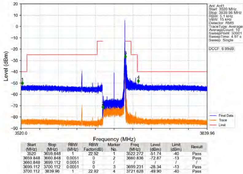
n48_30kHz_MIMO_NTNV_40MHz_CP-OFDM QPSK_3679.98MHz_Inner_1RB_Right
