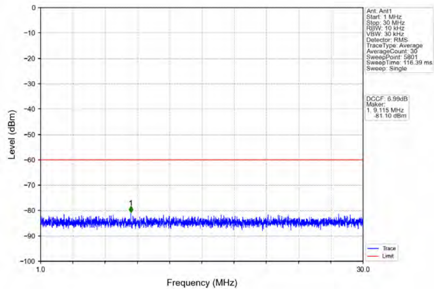
n48_30kHz_MIMO_NTNV_10MHz_CP-OFDM QPSK_3694.98MHz_Outer_Full
