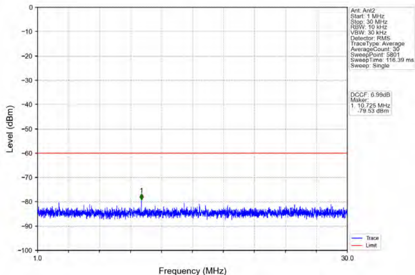
n48_30kHz_MIMO_NTNV_10MHz_CP-OFDM QPSK_3694.98MHz_Edge_1RB_Right
