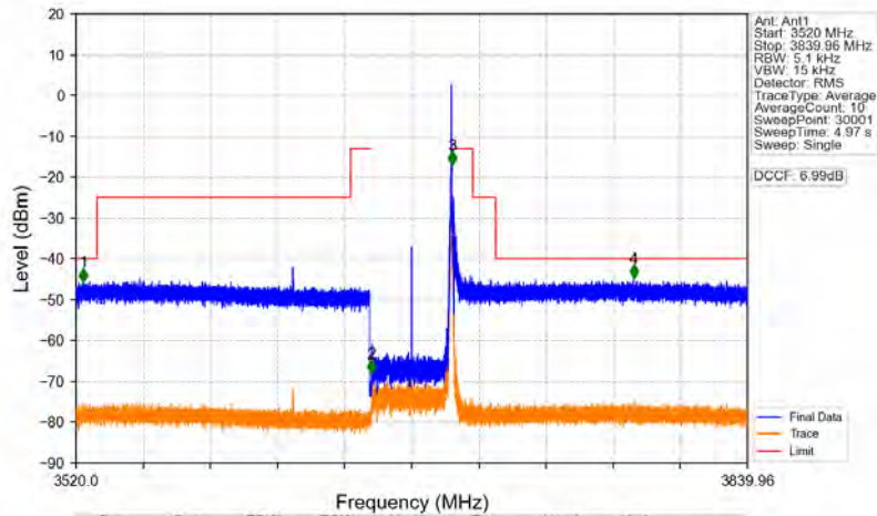
n48_30kHz_MIMO_NTNV_40MHz_CP-OFDM QPSK_3679.98MHz_Edge_1RB_Right
