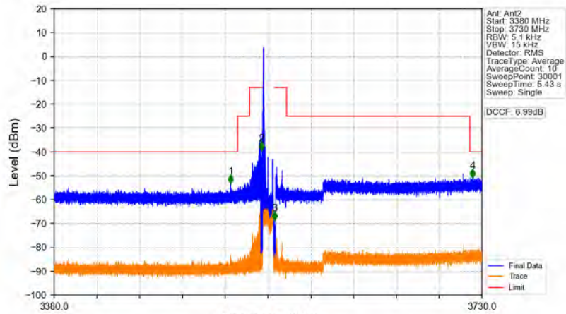
n48_30kHz_MIMO_NTNV_10MHz_CP-OFDM QPSK_3555MHz_Inner_1RB_Left
