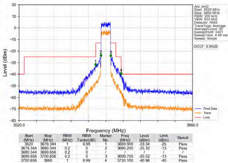
n48_30kHz_MIMO_NTNV_20MHz_CP-OFDM_QPSK_3690MHz_Outer_Full
