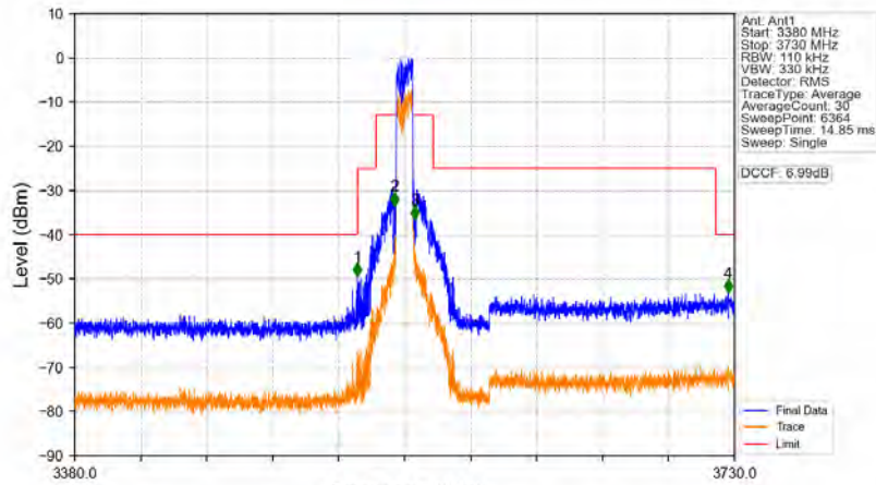
n48_30kHz_MIMO_NTNV_10MHz_CP-OFDM QPSK_3555MHz_Outer_Full
