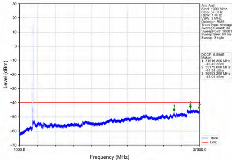
n48_30kHz_MIMO_NTNV_40MHz_CP-OFDM QPSK_3679.98MHz_Edge_1RB_Right
