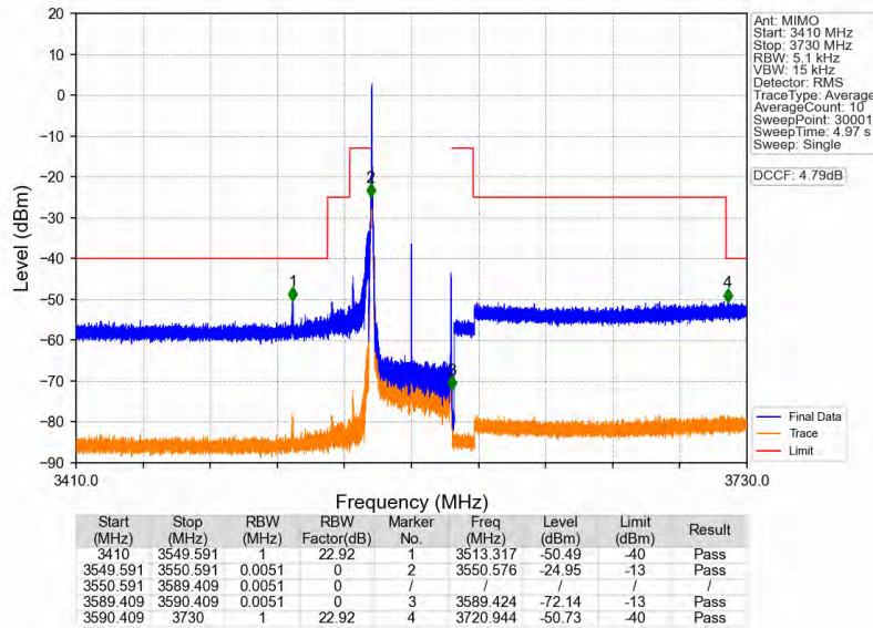
n48_30kHz_MIMO_NTNV_40MHz_CP-OFDM QPSK_3570MHz_Edge_1RB_Left
