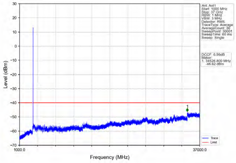
n48_30kHz_MIMO_NTNV_10MHz_CP-OFDM QPSK_3694.98MHz_Edge_1RB_Right
