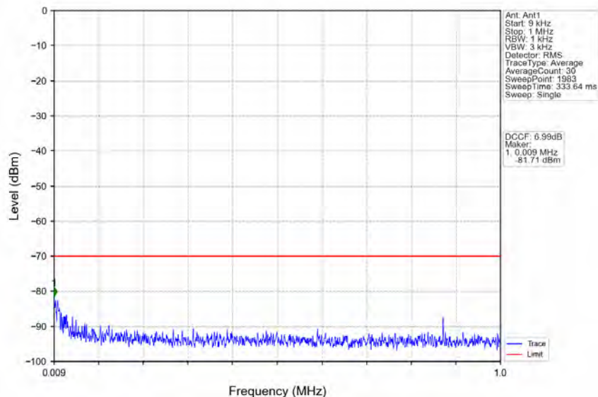
n48_30kHz_MIMO_NTNV_20MHz_CP-OFDM QPSK_3560.01MHz_Outer_Full
