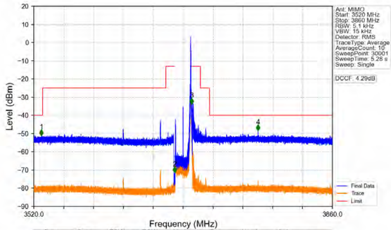
n48_30kHz_MIMO_NTNV_20MHz_CP-OFDM_QPSK_3690MHz_Inner_1RB_Right
