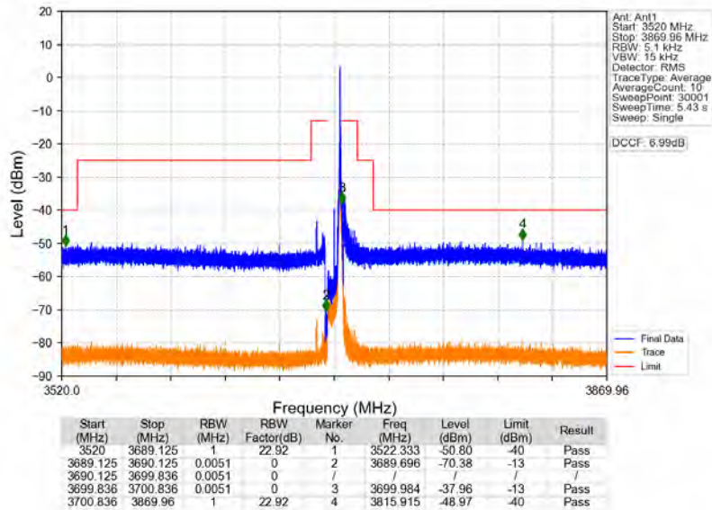
n48_30kHz_MIMO_NTNV_10MHz_CP-OFDM_QPSK_3694.98MHz_Inner_1RB_Right
