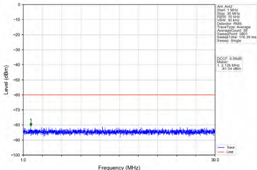
n48_30kHz_MIMO_NTNV_20MHz_CP-OFDM_QPSK_3560.01MHz_Edge_1RB_Left
