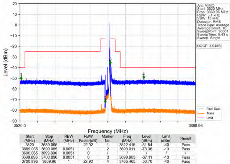
n48_30kHz_MIMO_NTNV_10MHz_CP-OFDM QPSK_3694.98MHz_Edge_1RB_Right
