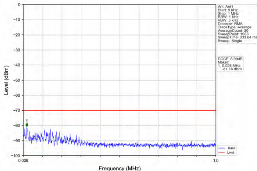
n48_30kHz_MIMO_NTNV_40MHz_CP-OFDM QPSK_3679.98MHz_Inner_1RB_Right
