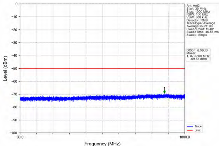
n48_30kHz_MIMO_NTNV_40MHz_CP-OFDM QPSK_3679.98MHz_Outer_Full
