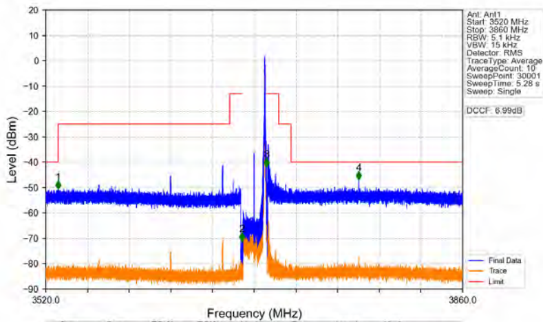
n48_30kHz_MIMO_NTNV_20MHz_CP-OFDM_QPSK_3690MHz_Inner_1RB_Right
