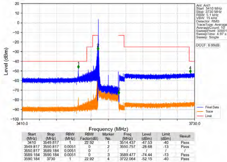
n48_30kHz_MIMO_NTNV_40MHz_CP-OFDM QPSK_3570MHz_Inner_1RB_Left
