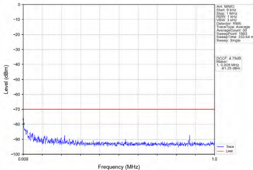
n48_30kHz_MIMO_NTNV_40MHz_CP-OFDM QPSK_3570MHz_Edge_1RB_Left
