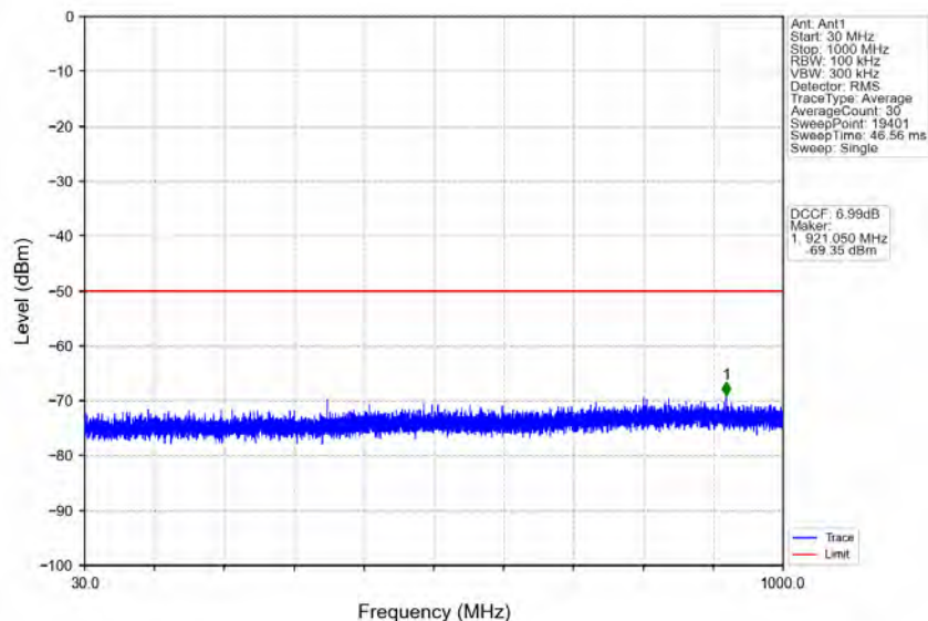
n48_30kHz_MIMO_NTNV_20MHz_CP-OFDM QPSK_3560.01MHz_Outer_Full
