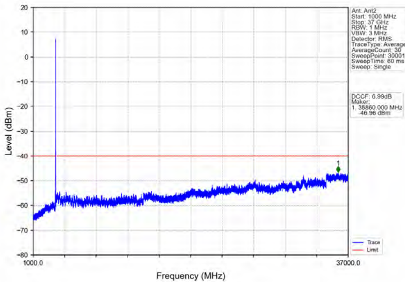
n48_30kHz_MIMO_NTNV_10MHz_CP-OFDM_QPSK_3555MHz_Outer_Full
