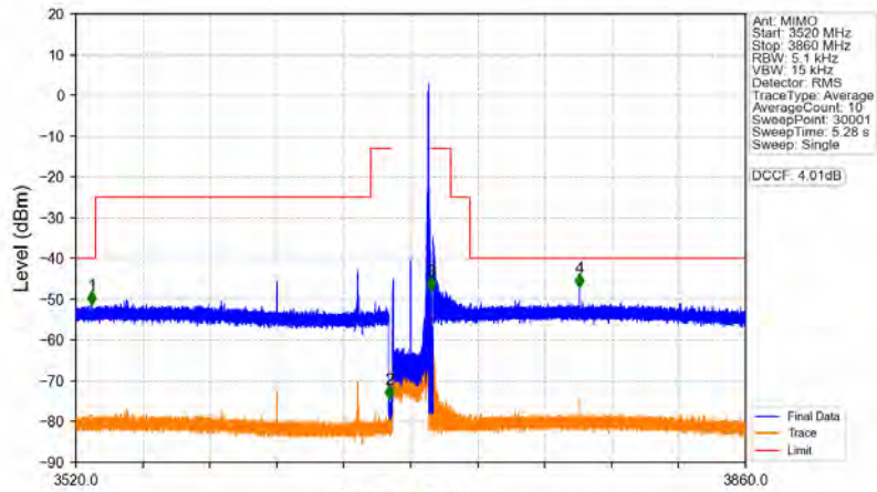
n48_30kHz_MIMO_NTNV_20MHz_CP-OFDM QPSK_3690MHz_Edge_1RB_Right
