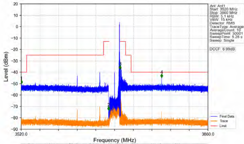
n48_30kHz_MIMO_NTNV_20MHz_CP-OFDM QPSK_3690MHz_Edge_1RB_Right
