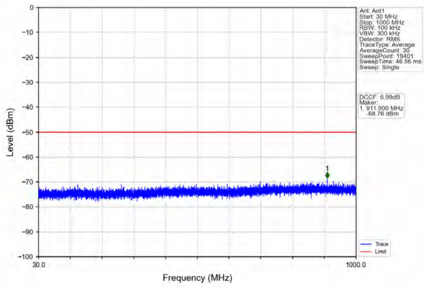
n48_30kHz_MIMO_NTNV_10MHz_CP-OFDM QPSK_3694.98MHz_Edge_1RB_Right
