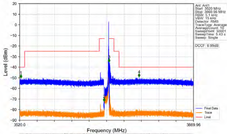
n48_30kHz_MIMO_NTNV_10MHz_CP-OFDM QPSK_3694.98MHz_Edge_1RB_Right
