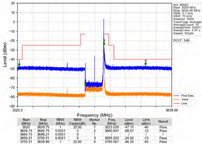
n48_30kHz_MIMO_NTNV_40MHz_CP-OFDM QPSK_3679.98MHz_Edge_1RB_Right
