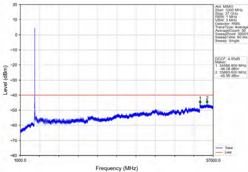
n48_30kHz_MIMO_NTNV_20MHz_CP-OFDM_QPSK_3690MHz_Inner_1RB_Right
