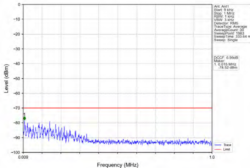
n48_30kHz_MIMO_NTNV_40MHz_CP-OFDM QPSK_3570MHz_Inner_1RB_Left
