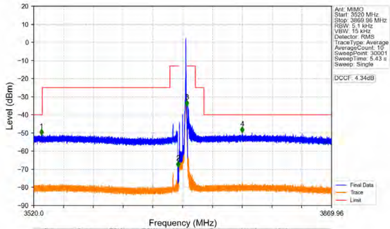
n48_30kHz_MIMO_NTNV_10MHz_CP-OFDM QPSK_3694.98MHz_Inner_1RB_Right
