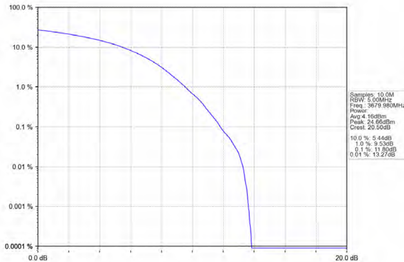
n48_30kHz_MIMO_NTNV_40MHz_CP-OFDM_256_QAM_3679.98MHz_Outer_Full
