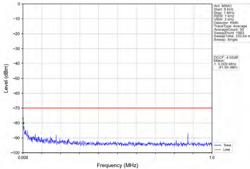
n48_30kHz_MIMO_NTNV_10MHz_CP-OFDM QPSK_3555MHz_Edge_1RB_Left
