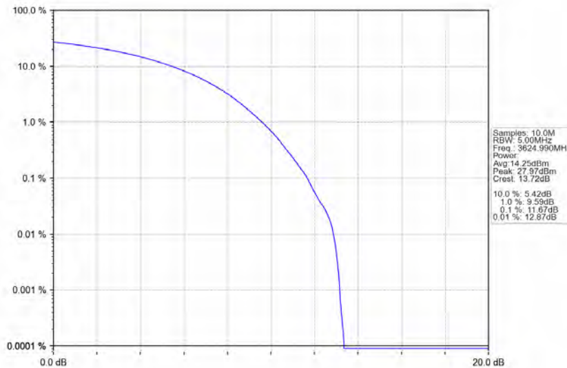
n48_30kHz_MIMO_NTNV_10MHz_CP-OFDM QPSK_3624.99MHz_Outer_Full
