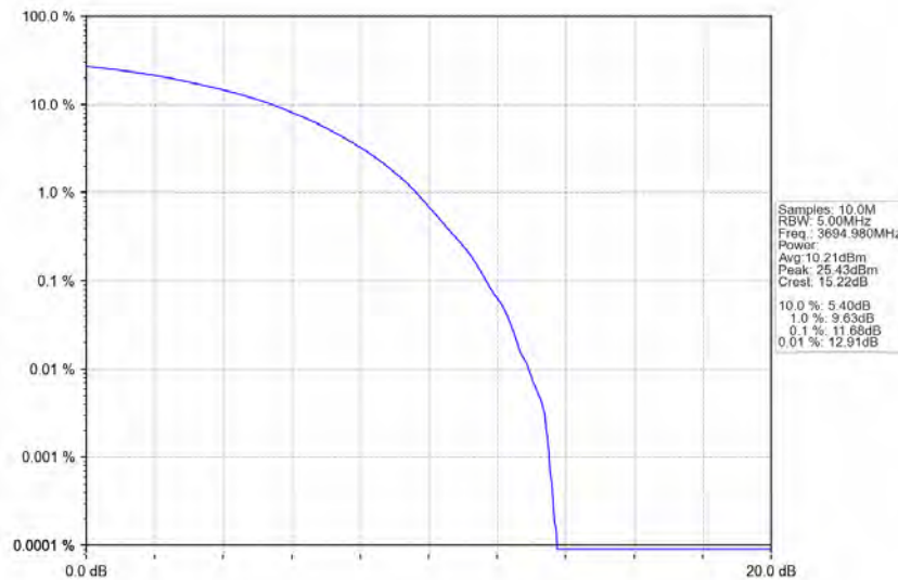
n48_30kHz_MIMO_NTNV_10MHz_CP-OFDM_256_QAM_3694.98MHz_Outer_Full
