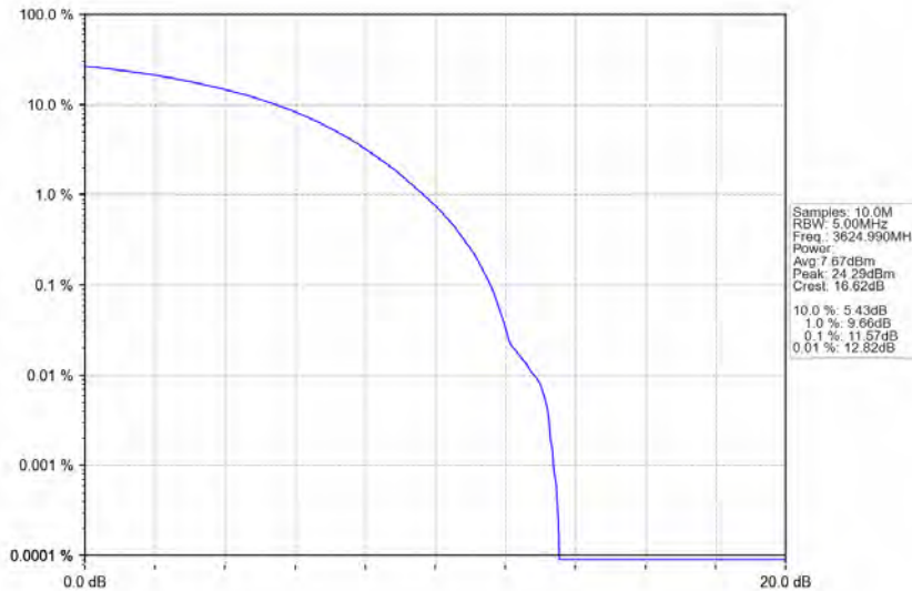
n48_30kHz_MIMO_NTNV_40MHz_CP-OFDM 64 QAM_3624.99MHz_Outer_Full
