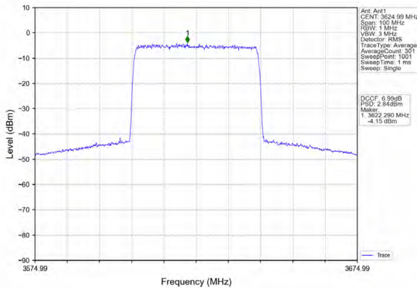
n48_30kHz_MIMO_NTNV_40MHz_CP-OFDM 256 QAM_3624.99MHz_Inner_Full
