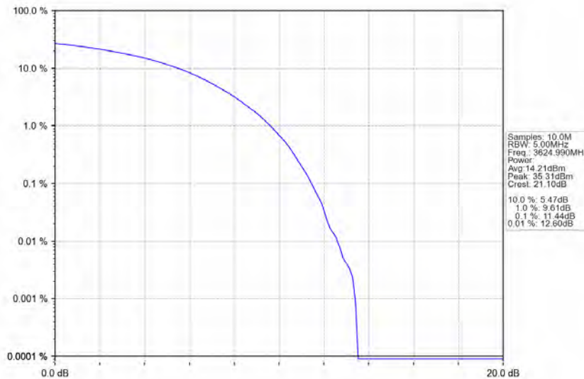
n48_30kHz_MIMO_NTNV_10MHz_CP-OFDM_16 QAM_3624.99MHz_Outer_Full
