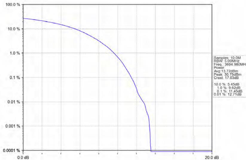
n48_30kHz_MIMO_NTNV_10MHz_CP-OFDM 16 QAM_3694.98MHz_Outer_Full
