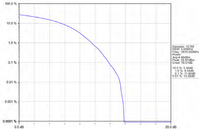
n48_30kHz_MIMO_NTNV_40MHz_CP-OFDM 256 QAM_3570MHz_Outer_Full
