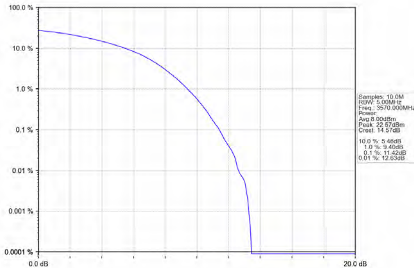
n48_30kHz_MIMO_NTNV_40MHz_CP-OFDM_16 QAM_3570MHz_Outer_Full
