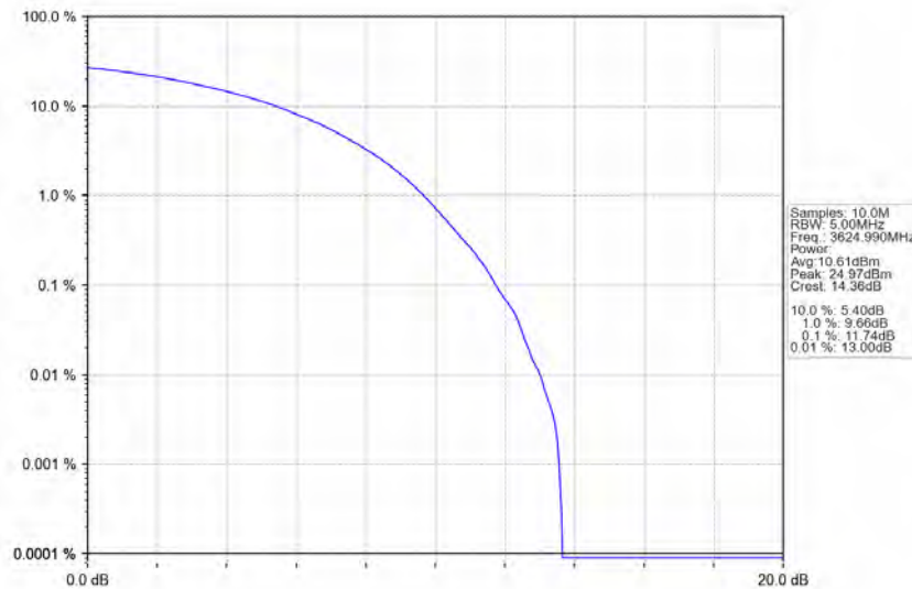
n48_30kHz_MIMO_NTNV_10MHz_CP-OFDM 256 QAM_3624.99MHz_Outer_Full
