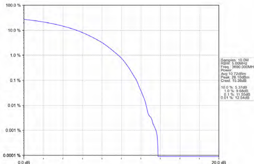
n48_30kHz_MIMO_NTNV_20MHz_CP-OFDM QPSK_3690MHz_Outer_Full
