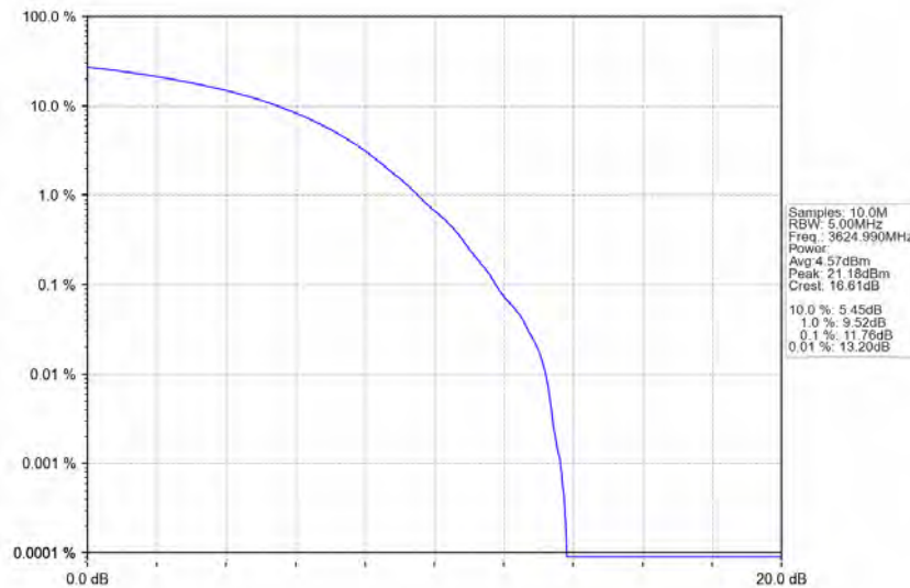
n48_30kHz_MIMO_NTNV_40MHz_CP-OFDM 256 QAM_3624.99MHz_Outer_Full
