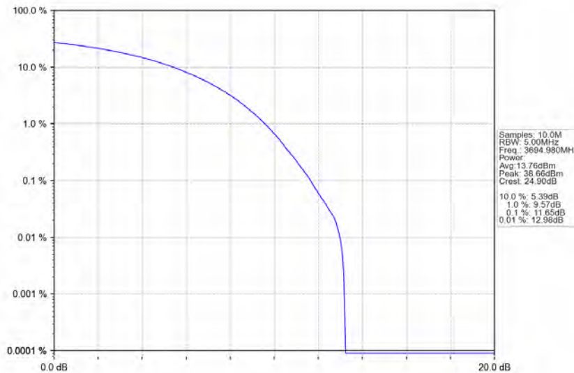
n48_30kHz_MIMO_NTNV_10MHz_CP-OFDM QPSK_3694.98MHz_Outer_Full
