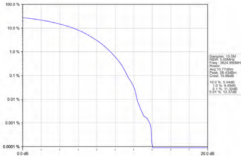
n48_30kHz_MIMO_NTNV_20MHz_CP-OFDM 64 QAM_3624.99MHz_Outer_Full
