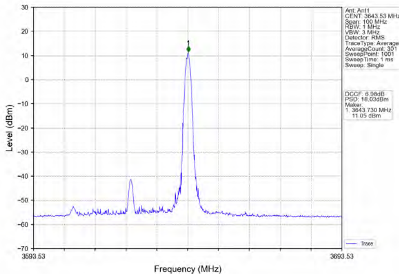
n48_30kHz_MIMO_NTNV_40MHz_CP-OFDM 16 QAM_3624.99MHz_Inner_1RB_Right
