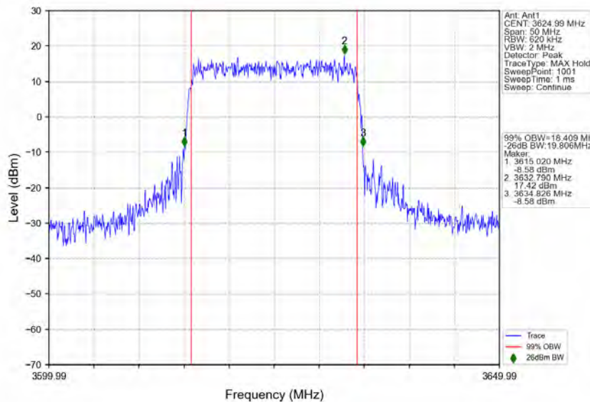
n48_30kHz_MIMO_NTNV_20MHz_CP-OFDM_16 QAM_3624.99MHz_Outer_Full
