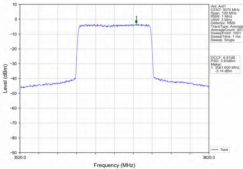
n48_30kHz_MIMO_NTNV_40MHz_CP-OFDM QPSK_3570MHz_Inner_Full
