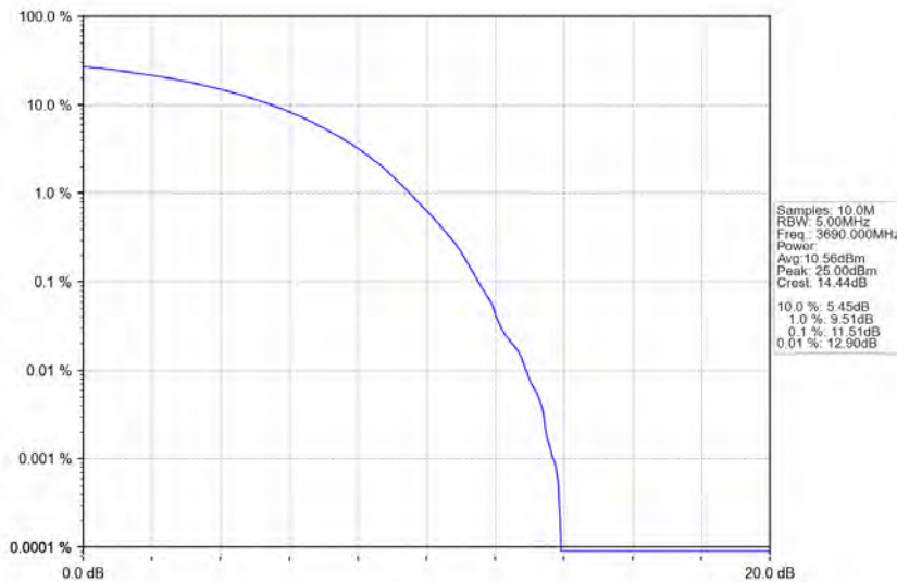
n48_30kHz_MIMO_NTNV_20MHz_CP-OFDM 16 QAM_3690MHz_Outer_Full
