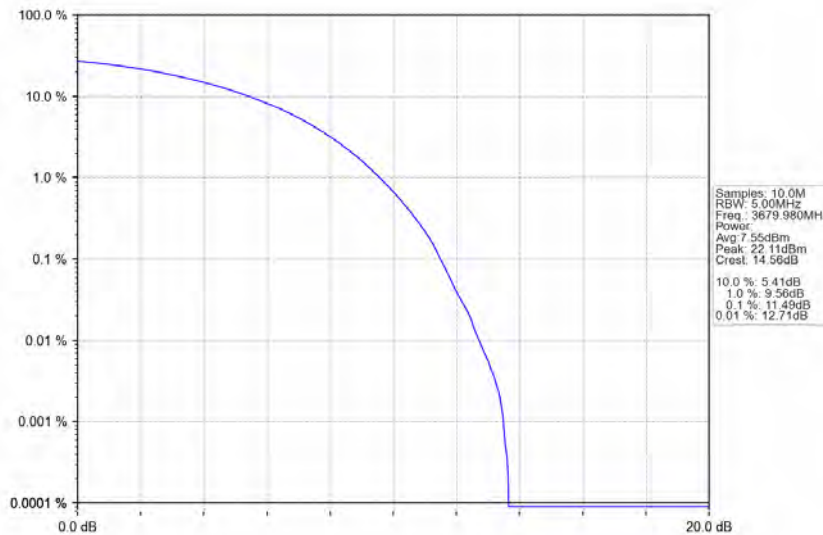
n48_30kHz_MIMO_NTNV_40MHz_CP-OFDM QPSK_3679.98MHz_Outer_Full
