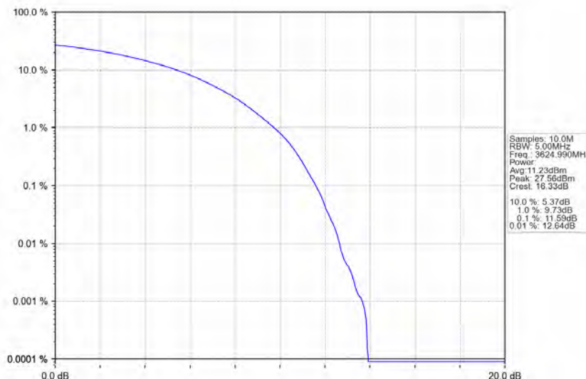
n48_30kHz_MIMO_NTNV_20MHz_CP-OFDM QPSK_3624.99MHz_Outer_Full
