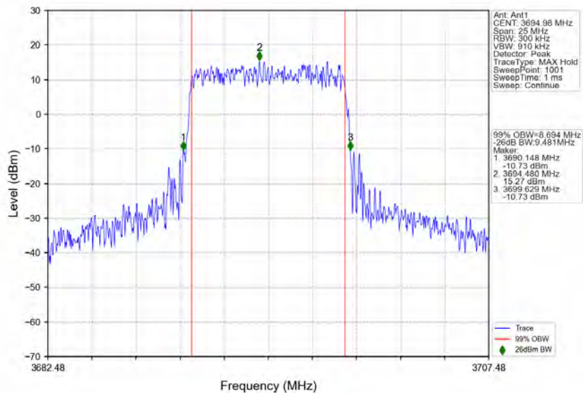
n48_30kHz_MIMO_NTNV_10MHz_CP-OFDM 64 QAM_3694.98MHz_Outer_Full
