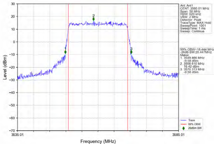
n48_30kHz_MIMO_NTNV_20MHz_CP-OFDM 64 QAM_3560.01MHz_Outer_Full
