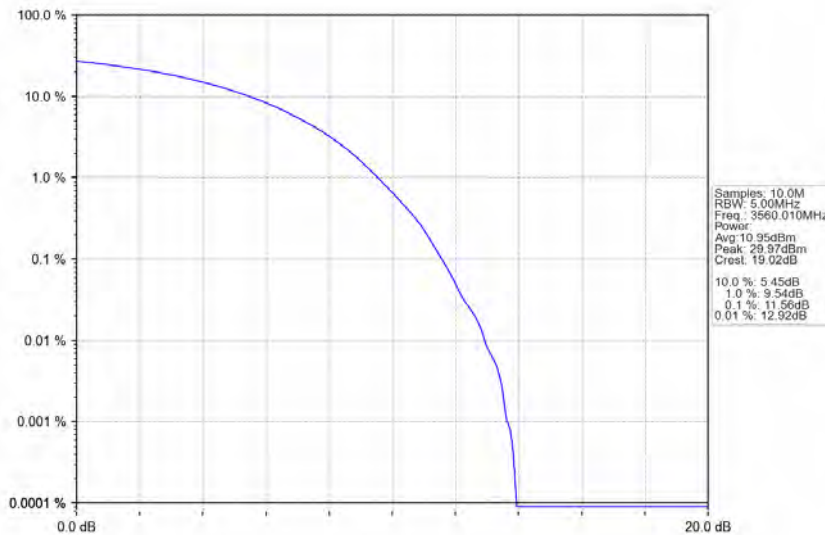
n48_30kHz_MIMO_NTNV_20MHz_CP-OFDM_16 QAM_3560.01MHz_Outer_Full
