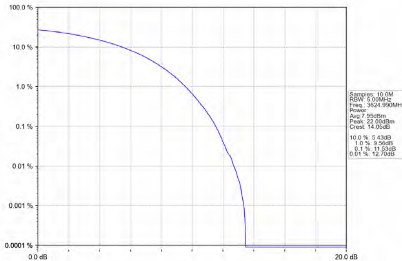
n48_30kHz_MIMO_NTNV_40MHz_CP-OFDM QPSK_3624.99MHz_Outer_Full
