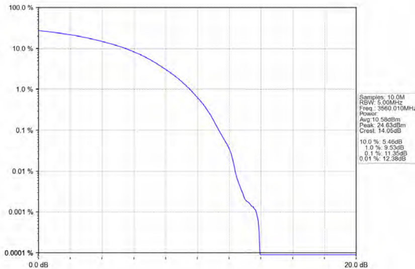
n48_30kHz_MIMO_NTNV_20MHz_CP-OFDM 64 QAM_3560.01MHz_Outer_Full
