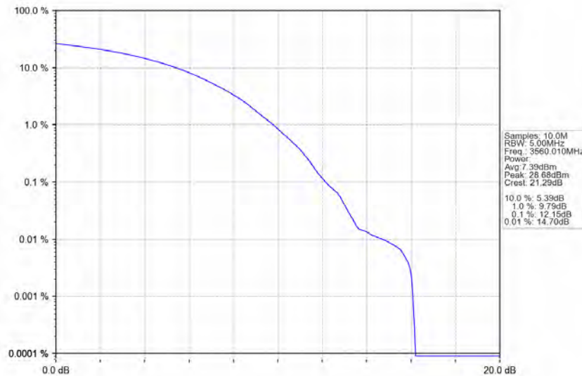
n48_30kHz_MIMO_NTNV_20MHz_CP-OFDM_256_QAM_3560.01MHz_Outer_Full
