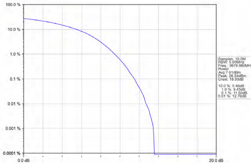
n48_30kHz_MIMO_NTNV_40MHz_CP-OFDM 16 QAM_3679.98MHz_Outer_Full
