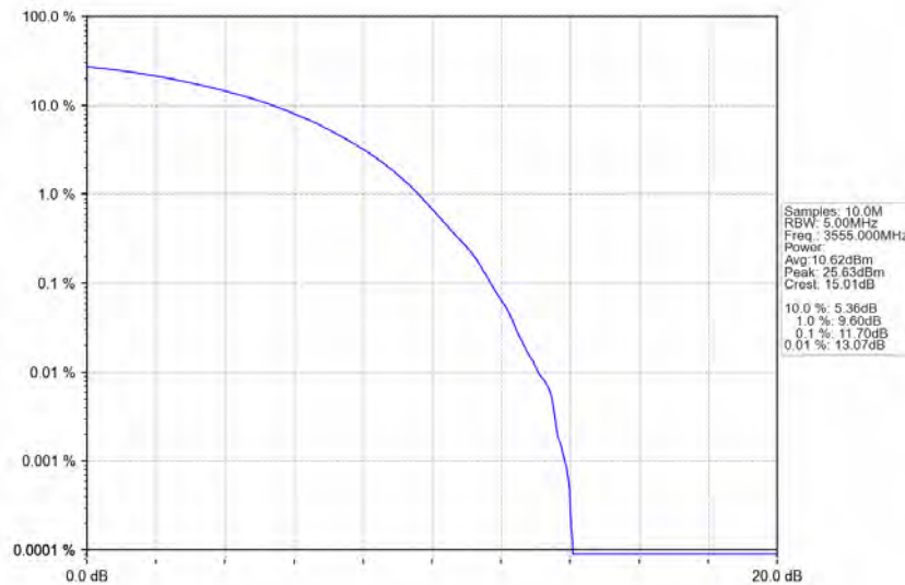
n48_30kHz_MIMO_NTNV_10MHz_CP-OFDM 256 QAM_3555MHz_Outer_Full
