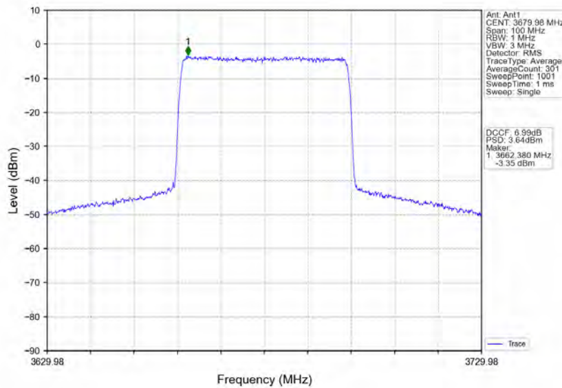
n48_30kHz_MIMO_NTNV_40MHz_CP-OFDM 16 QAM_3679.98MHz_Inner_Full
