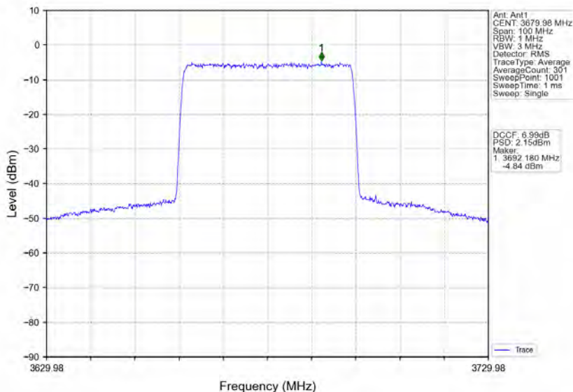
n48_30kHz_MIMO_NTNV_40MHz_CP-OFDM 256 QAM_3679.98MHz_Inner_Full
