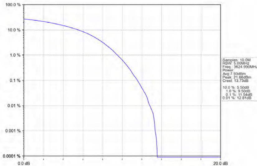
n48_30kHz_MIMO_NTNV_40MHz_CP-OFDM_16 QAM_3624.99MHz_Outer_Full
