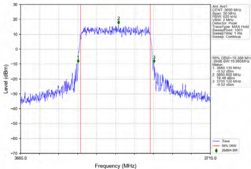
n48_30kHz_MIMO_NTNV_20MHz_CP-OFDM 64 QAM_3690MHz_Outer_Full
