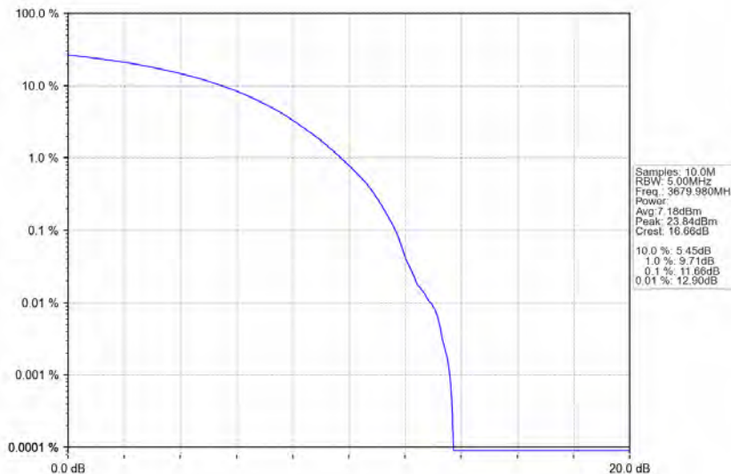
n48_30kHz_MIMO_NTNV_40MHz_CP-OFDM 64 QAM_3679.98MHz_Outer_Full
