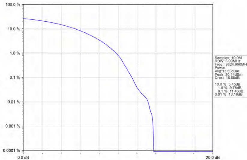
n48_30kHz_MIMO_NTNV_10MHz_CP-OFDM 64 QAM_3624.99MHz_Outer_Full
