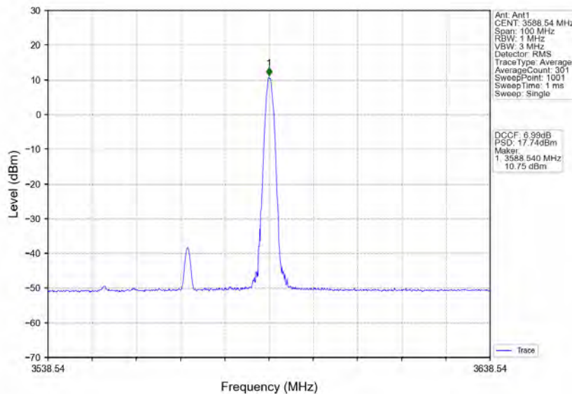
n48_30kHz_MIMO_NTNV_40MHz_CP-OFDM 256 QAM_3570MHz_Inner_1RB_Right
