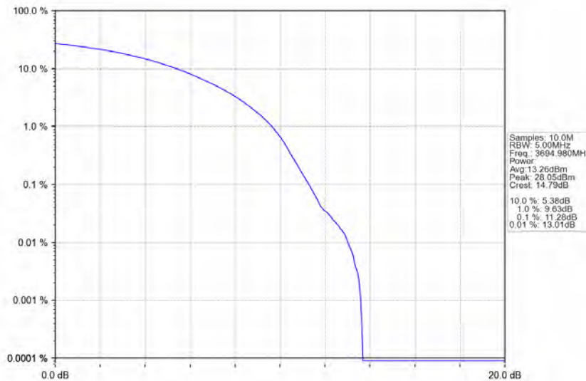
n48_30kHz_MIMO_NTNV_10MHz_CP-OFDM 64 QAM_3694.98MHz_Outer_Full
