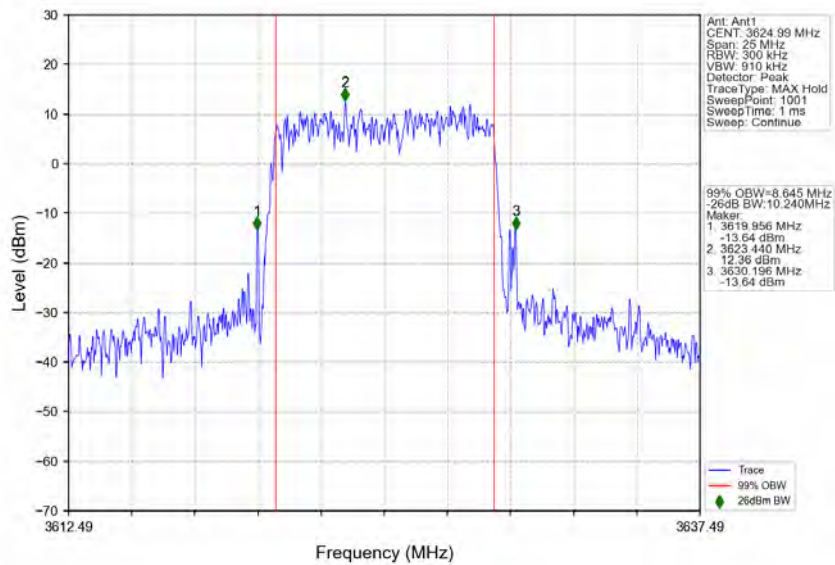
n48_30kHz_MIMO_NTNV_10MHz_CP-OFDM 256 QAM_3624.99MHz_Outer_Full
