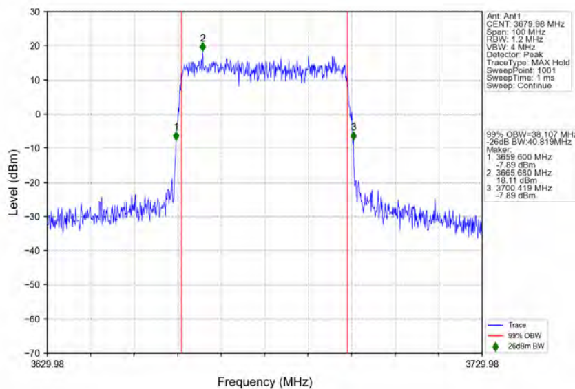
n48_30kHz_MIMO_NTNV_40MHz_CP-OFDM QPSK_3679.98MHz_Outer_Full
