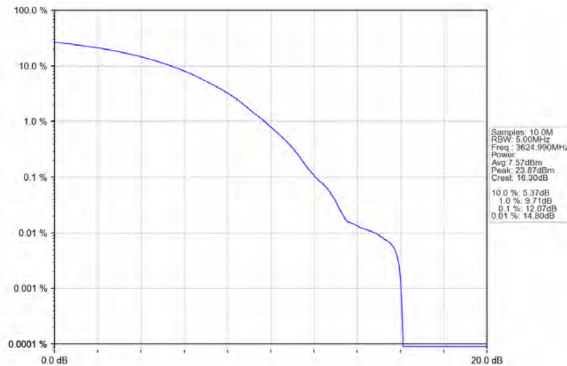
n48_30kHz_MIMO_NTNV_20MHz_CP-OFDM_256_QAM_3624.99MHz_Outer_Full
