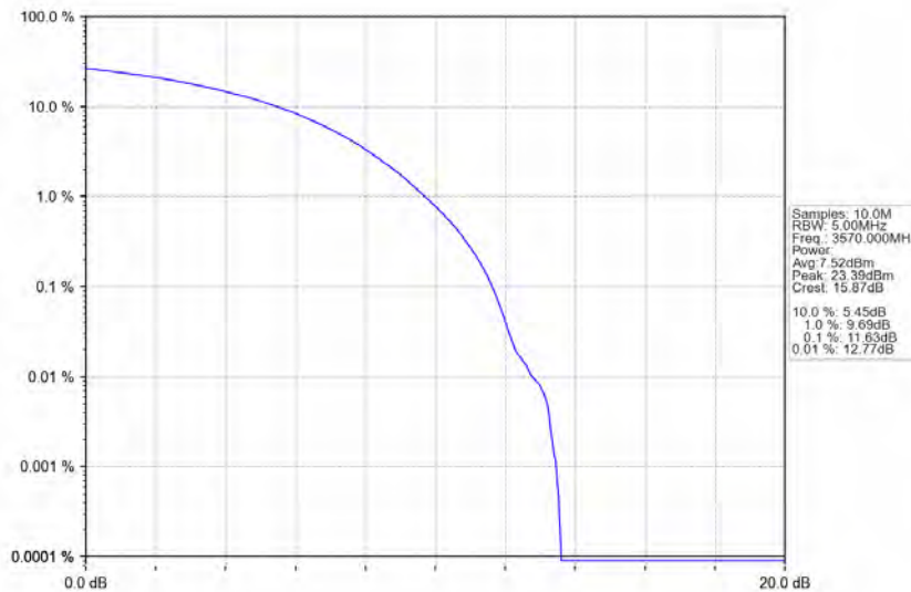
n48_30kHz_MIMO_NTNV_40MHz_CP-OFDM 64 QAM_3570MHz_Outer_Full
