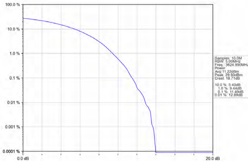
n48_30kHz_MIMO_NTNV_20MHz_CP-OFDM_16 QAM_3624.99MHz_Outer_Full
