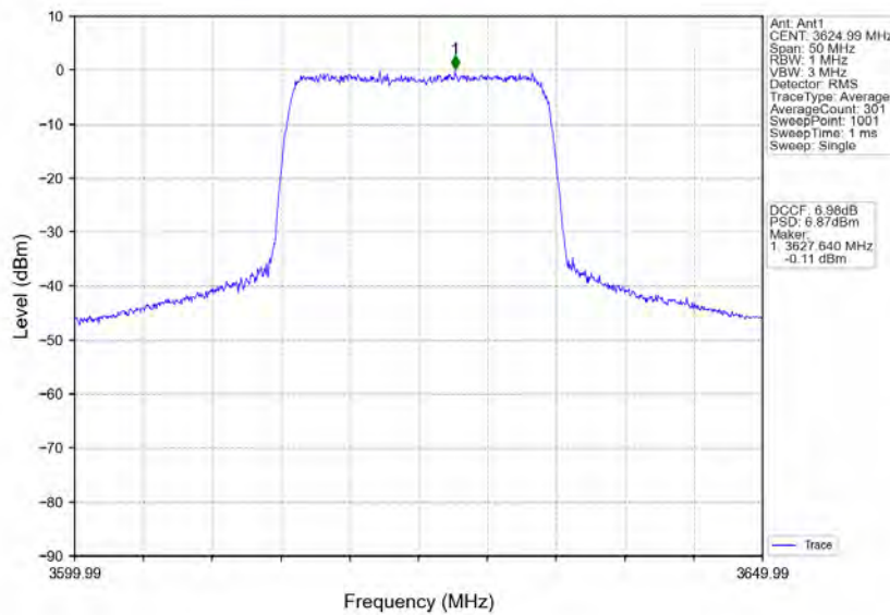
n48_30kHz_MIMO_NTNV_20MHz_CP-OFDM 64 QAM_3624.99MHz_Inner_Full
