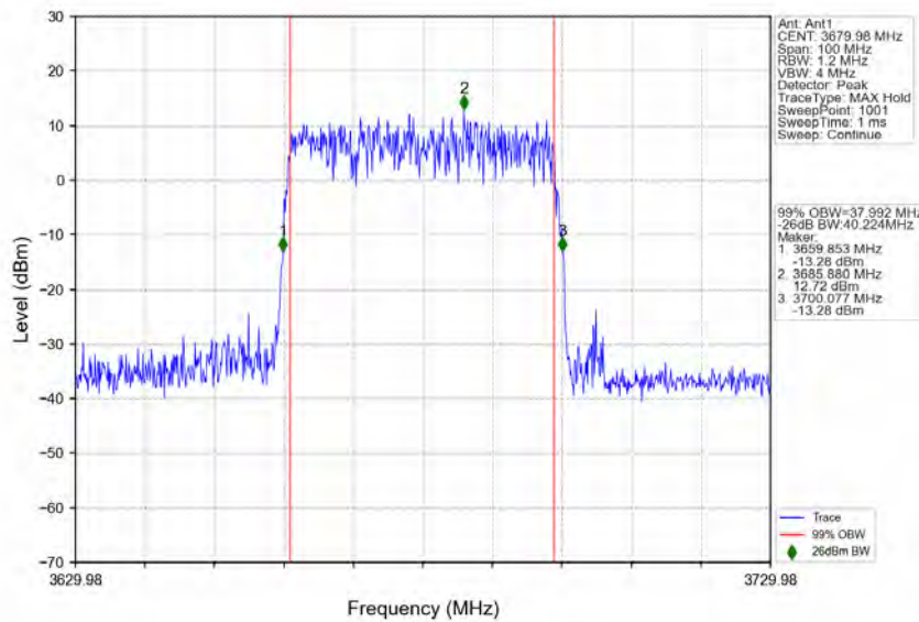
n48_30kHz_MIMO_NTNV_40MHz_CP-OFDM_256_QAM_3679.98MHz_Outer_Full
