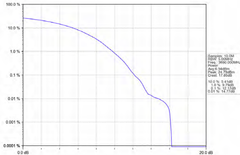
n48_30kHz_MIMO_NTNV_20MHz_CP-OFDM_256 QAM_3690MHz_Outer_Full
