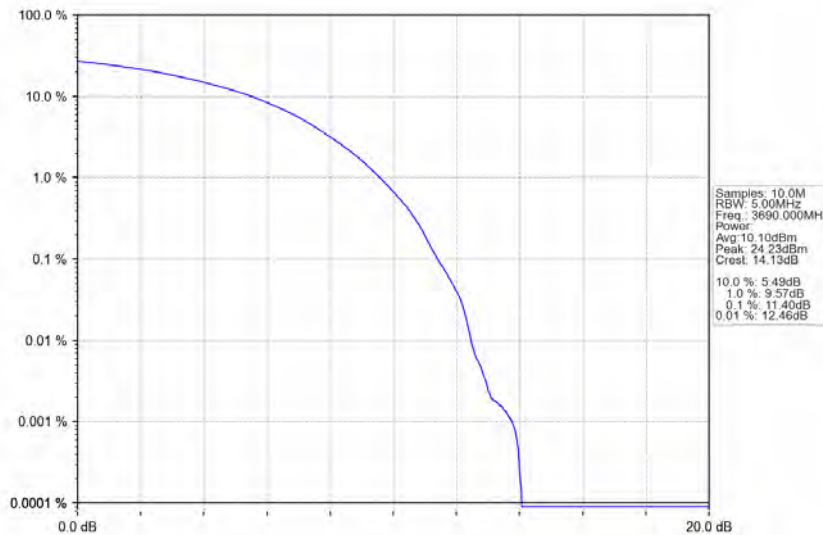
n48_30kHz_MIMO_NTNV_20MHz_CP-OFDM 64 QAM_3690MHz_Outer_Full
