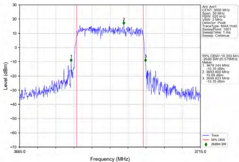
n48_30kHz_MIMO_NTNV_20MHz_CP-OFDM QPSK_3690MHz_Outer_Full
