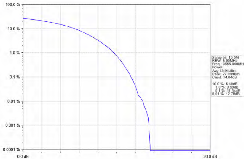
n48_30kHz_MIMO_NTNV_10MHz_CP-OFDM_16 QAM_3555MHz_Outer_Full
