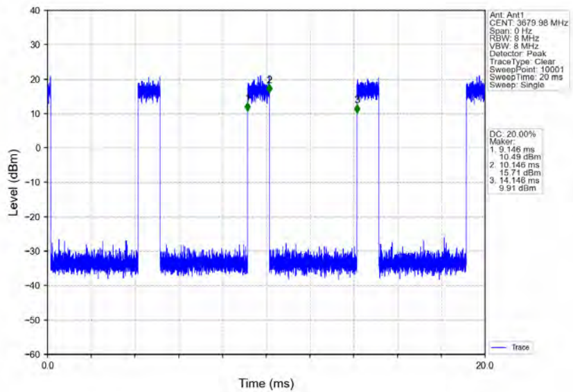
n48_30kHz_MIMO_NTNV_40MHz_CP-OFDM_256_QAM_3679.98MHz_Inner_Full
