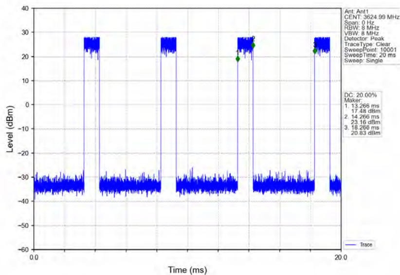
n48_30kHz_MIMO_NTNV_10MHz_CP-OFDM 64 QAM_3624.99MHz_Inner_Full
