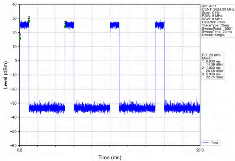
n48_30kHz_MIMO_NTNV_10MHz_CP-OFDM QPSK_3624.99MHz_Inner_Full
