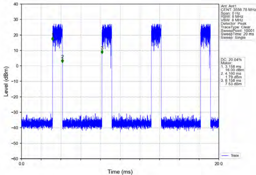
n48_30kHz_MIMO_NTNV_10MHz_CP-OFDM 64 QAM_3555MHz_Inner_1RB_Right
