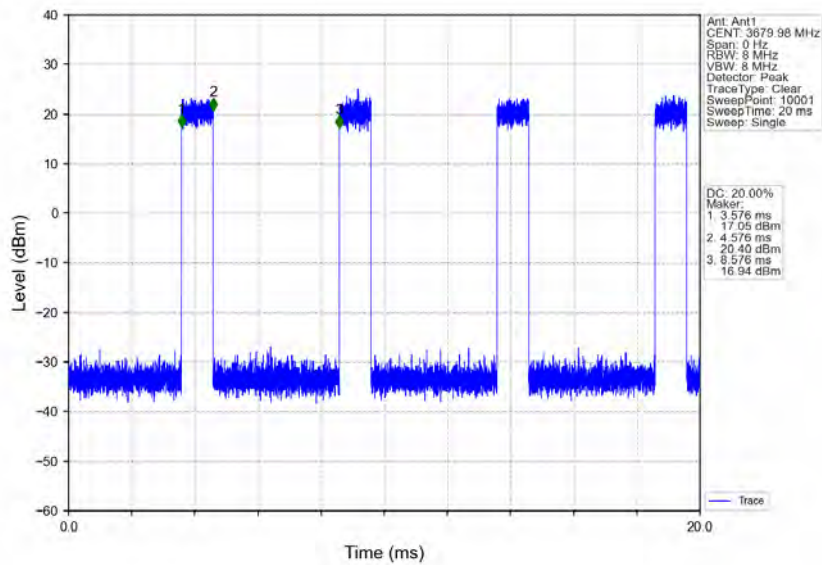
n48_30kHz_MIMO_NTNV_40MHz_CP-OFDM 16 QAM_3679.98MHz_Inner_Full
