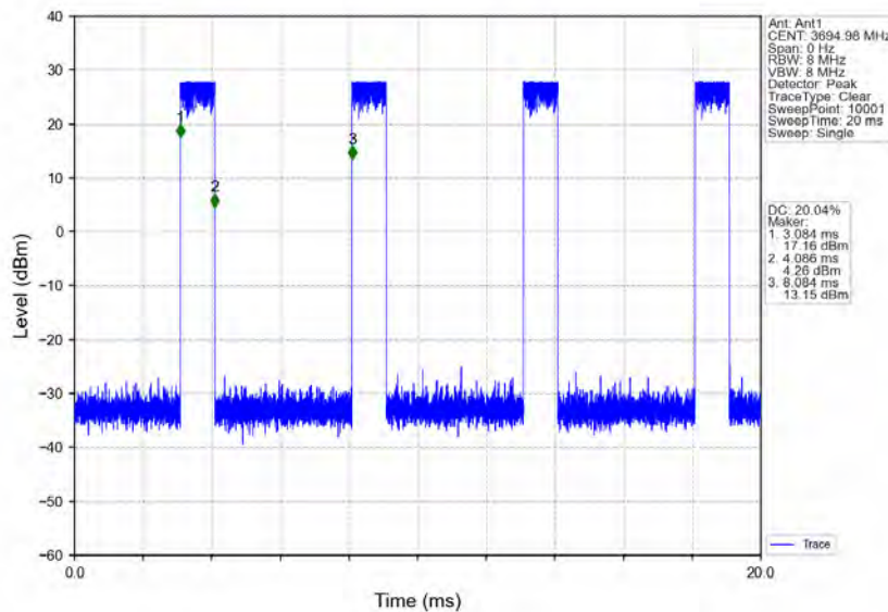
n48_30kHz_MIMO_NTNV_10MHz_CP-OFDM 16 QAM_3694.98MHz_Inner_Full
