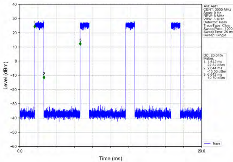
n48_30kHz_MIMO_NTNV_10MHz_CP-OFDM QPSK_3555MHz_Inner_Full
