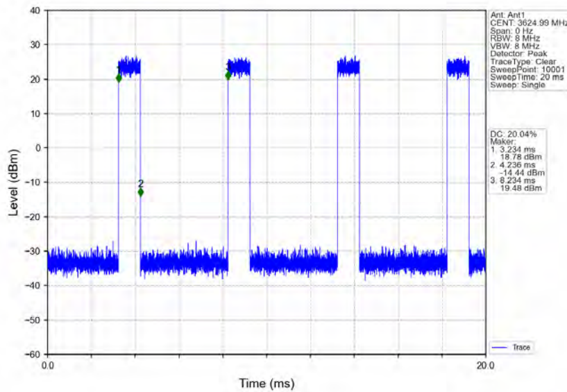
n48_30kHz_MIMO_NTNV_20MHz_CP-OFDM QPSK_3624.99MHz_Inner_Full
