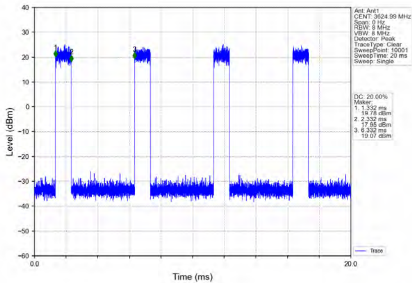
n48_30kHz_MIMO_NTNV_40MHz_CP-OFDM_QPSK_3624.99MHz_Inner_Full
