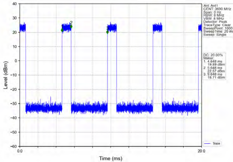
n48_30kHz_MIMO_NTNV_20MHz_CP-OFDM_16 QAM_3690MHz_Inner_Full
