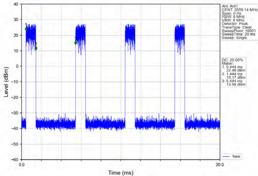
n48_30kHz_MIMO_NTNV_10MHz_CP-OFDM 64 QAM_3555MHz_Edge_1RB_Right
