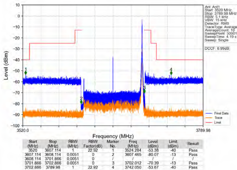
n78d_30kHz_MIMO_NTNV_90MHz_CP-OFDM_QPSK_3654.99MHz_Inner_1RB_Right
