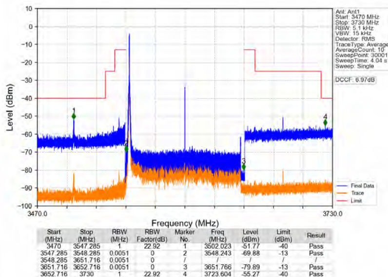
n78d_30kHz_MIMO_NTNV_100MHz_CP-OFDM_QPSK_3600MHz_Edge_1RB_Left
