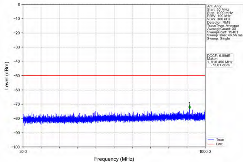
n78d_30kHz_MIMO_NTNV_80MHz_CP-OFDM_QPSK_3590.01MHz_Outer_Full
