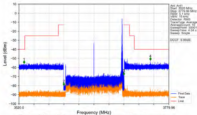
n78d_30kHz_MIMO_NTNV_100MHz_CP-OFDM_QPSK_3649.98MHz_Edge_1RB_Right
