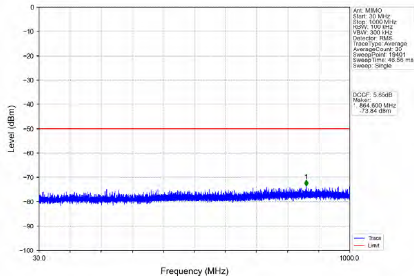
n78d_30kHz_MIMO_NTNV_70MHz_CP-OFDM QPSK_3664.98MHz_Inner_1RB_Right
