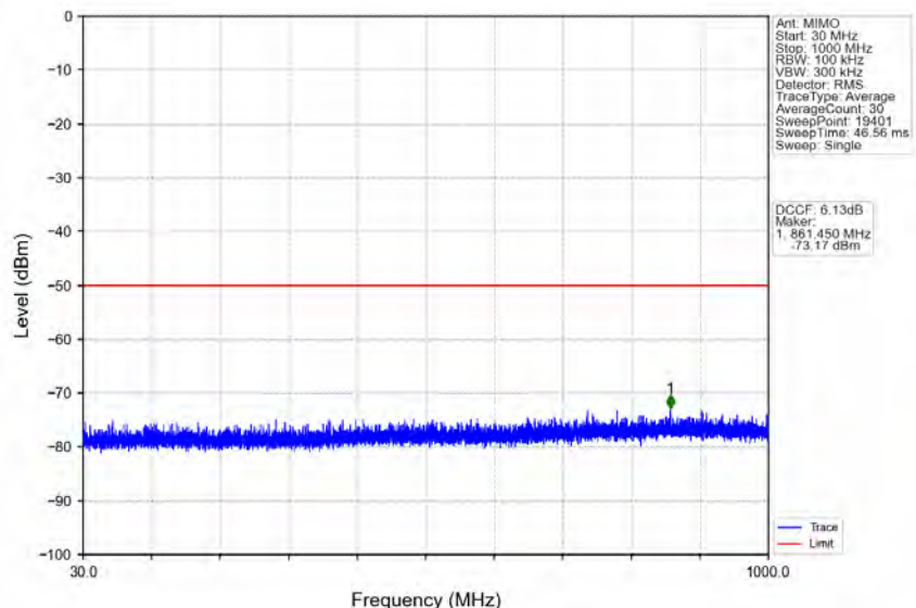
n78d_30kHz_MIMO_NTNV_90MHz_CP-OFDM_QPSK_3595.02MHz_Edge_1RB_Left
