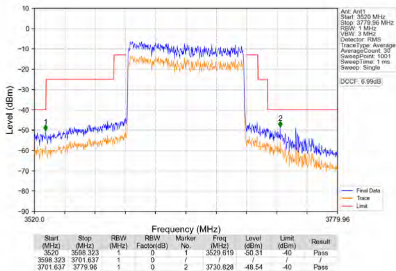
n78d_30kHz_MIMO_NTNV_100MHz_CP-OFDM QPSK_3649.98MHz_Outer_Full
