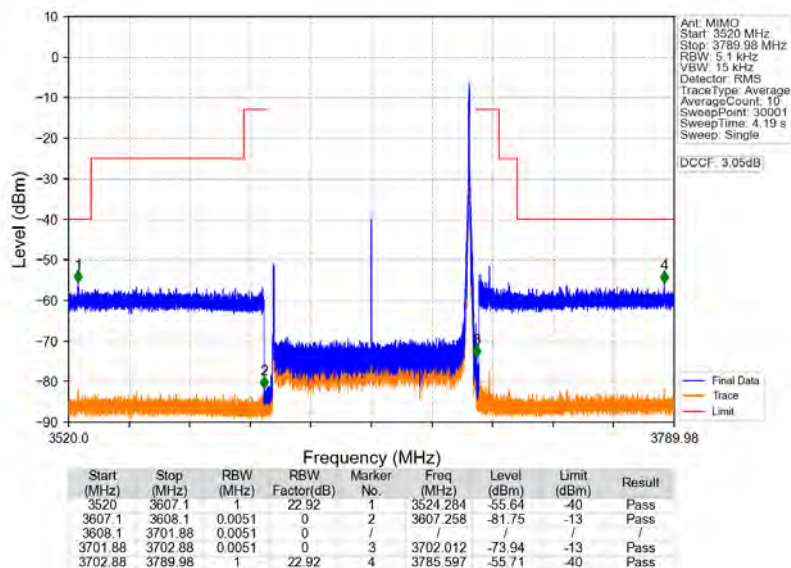
n78d_30kHz_MIMO_NTNV_90MHz_CP-OFDM_QPSK_3654.99MHz_Inner_1RB_Right
