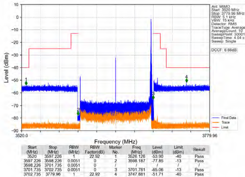
n78d_30kHz_MIMO_NTNV_100MHz_CP-OFDM_QPSK_3649.98MHz_Edge_1RB_Right
