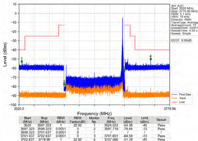
n78d_30kHz_MIMO_NTNV_100MHz_CP-OFDM_QPSK_3649.98MHz_Inner_1RB_Right
