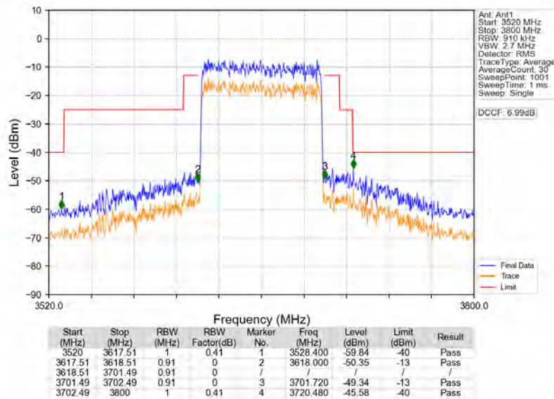
n78d_30kHz_MIMO_NTNV_80MHz_CP-OFDM_QPSK_3660MHz_Outer_Full
