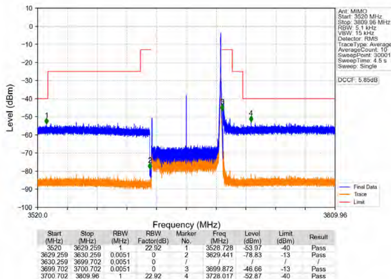
n78d_30kHz_MIMO_NTNV_70MHz_CP-OFDM_QPSK_3664.98MHz_Inner_1RB_Right
