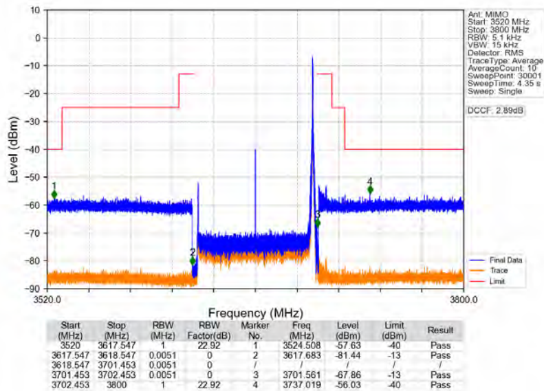
n78d_30kHz_MIMO_NTNV_80MHz_CP-OFDM_QPSK_3660MHz_Inner_1RB_Right
