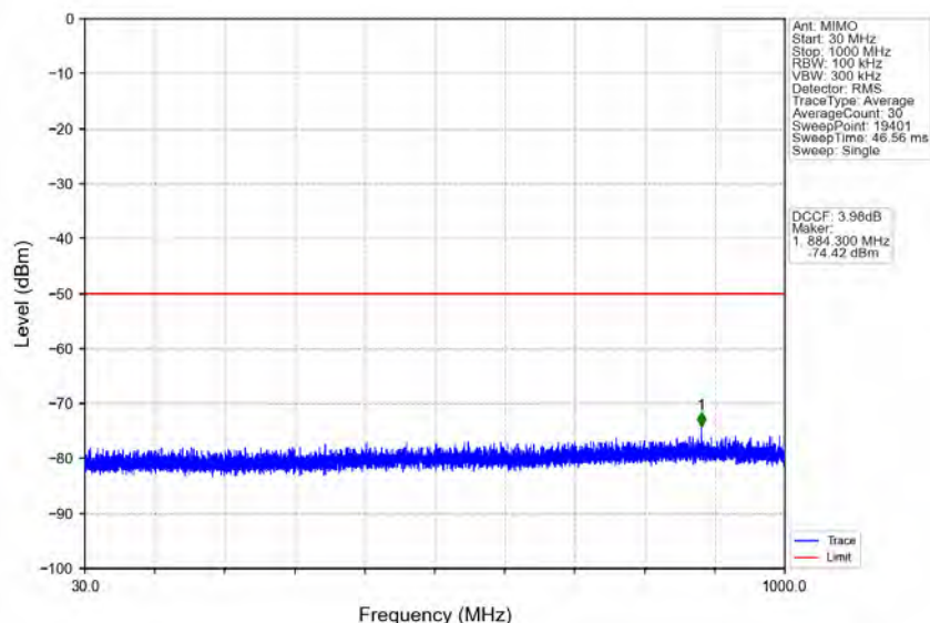
n78d_30kHz_MIMO_NTNV_80MHz_CP-OFDM_QPSK_3590.01MHz_Edge_1RB_Left
