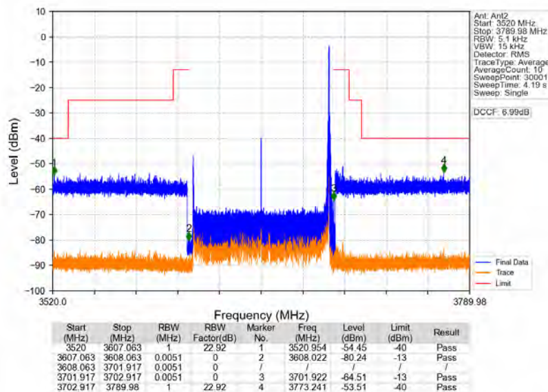
n78d_30kHz_MIMO_NTNV_90MHz_CP-OFDM_QPSK_3654.99MHz_Edge_1RB_Right
