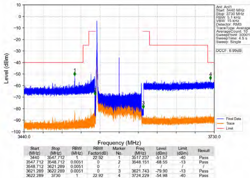
n78d 30kHz MIMO_NTNV_70MHz_CP-OFDM QPSK_3585MHz_Edge_1RB_Left
