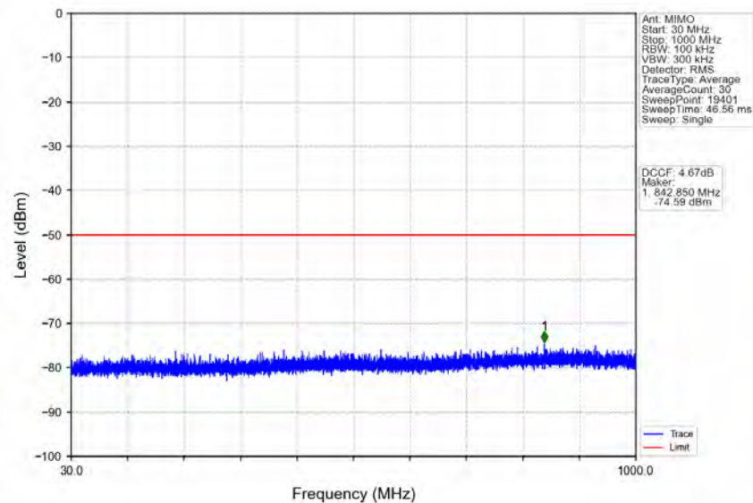
n78d_30kHz_MIMO_NTNV_70MHz_CP-OFDM QPSK_3664.98MHz_Outer_Full
