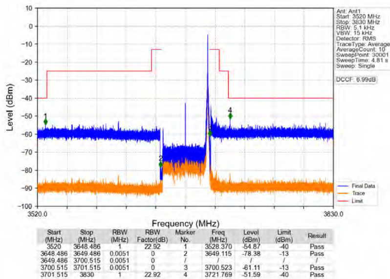
n78d_30kHz_MIMO_NTNV_50MHz_CP-OFDM_QPSK_3675MHz_Inner_1RB_Right
