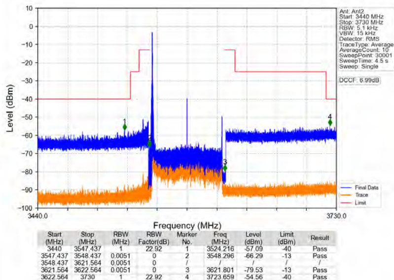
n78d_30kHz_MIMO_NTNV_70MHz_CP-OFDM_QPSK_3585MHz_Edge_1RB_Left
