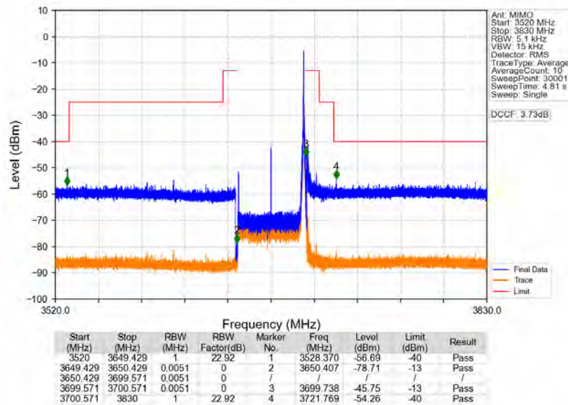
n78d_30kHz_MIMO_NTNV_50MHz_CP-OFDM_QPSK_3675MHz_Inner_1RB_Right
