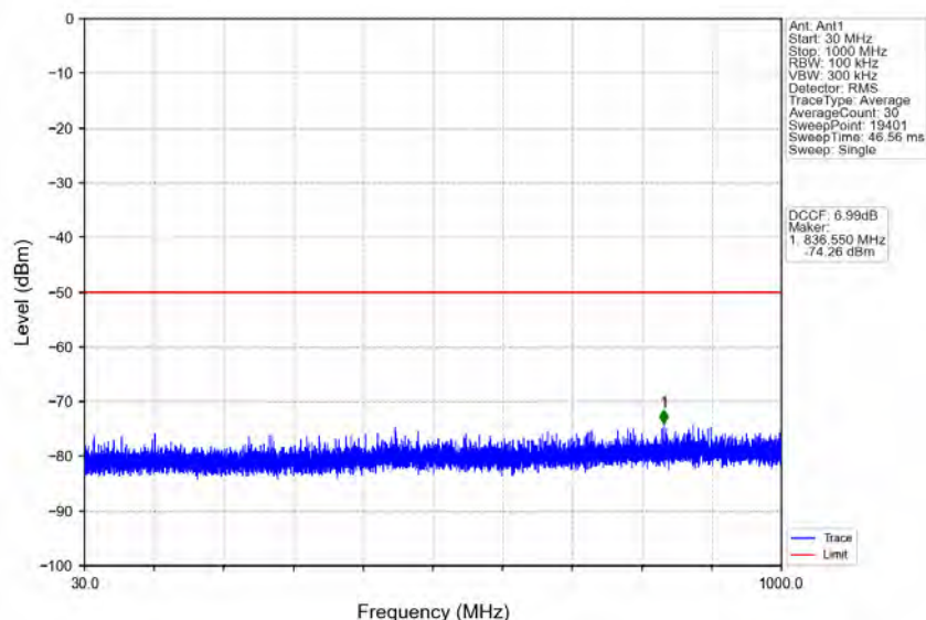
n78d_30kHz_MIMO_NTNV_70MHz_CP-OFDM_QPSK_3585MHz_Inner_1RB_Left
