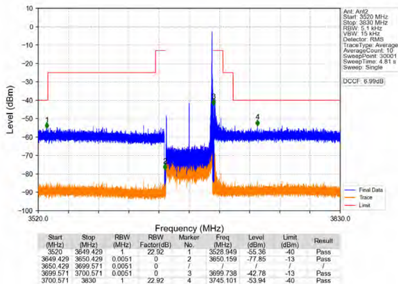
n78d_30kHz_MIMO_NTNV_50MHz_CP-OFDM_QPSK_3675MHz_Inner_1RB_Right
