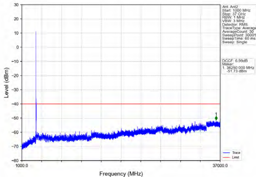
n78d_30kHz_MIMO_NTNV_70MHz_CP-OFDM QPSK_3585MHz_Inner_1RB_Left
