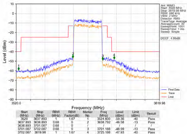
n78d_30kHz_MIMO_NTNV_60MHz_CP-OFDM_QPSK_3669.99MHz_Outer_Full
