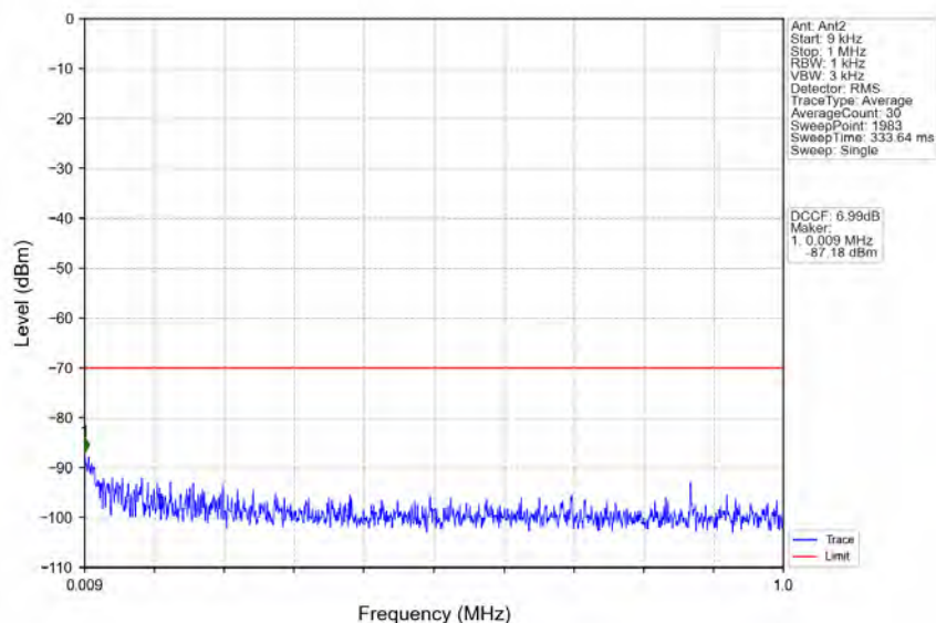
n78d_30kHz_MIMO_NTNV_60MHz_CP-OFDM_QPSK_3580.02MHz_Inner_1RB_Left
