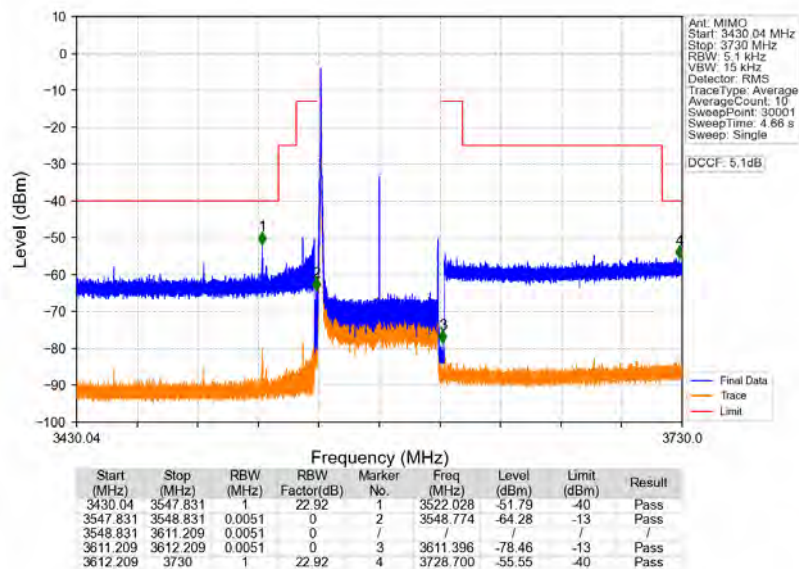
n78d_30kHz_MIMO_NTNV_60MHz_CP-OFDM_QPSK_3580.02MHz_Edge_1RB_Left
