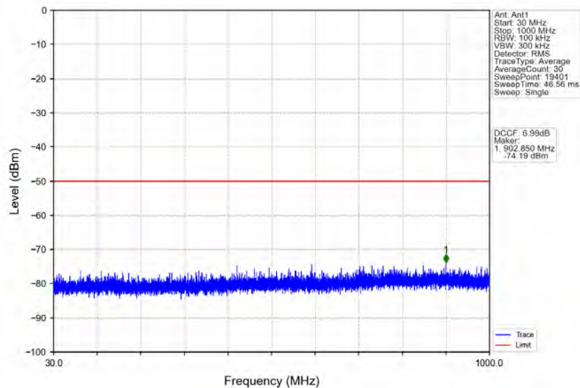
n78d_30kHz_MIMO_NTNV_60MHz_CP-OFDM_QPSK_3669.99MHz_Outer_Full
