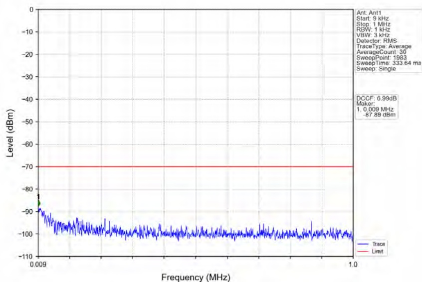
n78d 30kHz MIMO_NTNV_70MHz_CP-OFDM QPSK_3585MHz_Edge_1RB_Left
