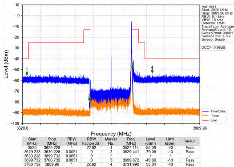
n78d_30kHz_MIMO_NTNV_70MHz_CP-OFDM_QPSK_3664.98MHz_Inner_1RB_Right
