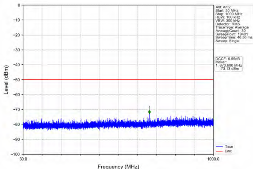
n78d_30kHz_MIMO_NTNV_70MHz_CP-OFDM_QPSK_3585MHz_Outer_Full
