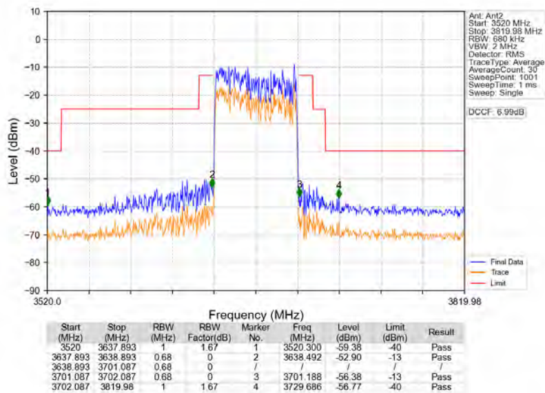
n78d_30kHz_MIMO_NTNV_60MHz_CP-OFDM_QPSK_3669.99MHz_Outer_Full
