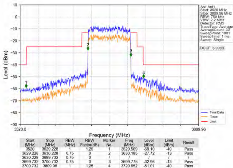
n78d_30kHz_MIMO_NTNV_70MHz_CP-OFDM_QPSK_3664.98MHz_Outer_Full
