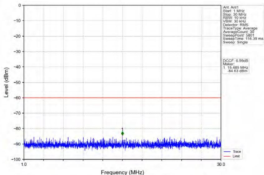
n78d_30kHz_MIMO_NTNV_70MHz_CP-OFDM_QPSK_3664.98MHz_Outer_Full
