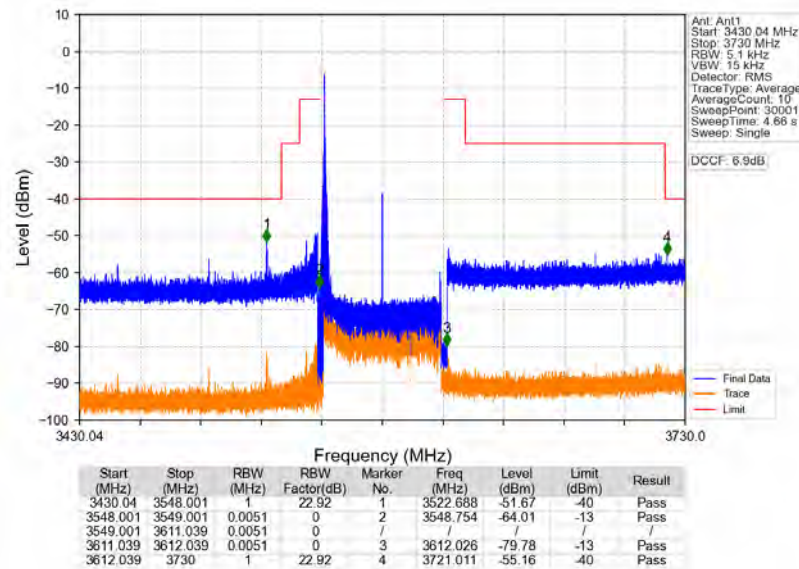
n78d_30kHz_MIMO_NTNV_60MHz_CP-OFDM_QPSK_3580.02MHz_Inner_1RB_Left
