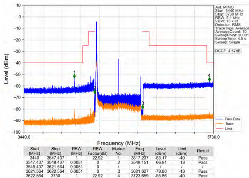
n78d_30kHz_MIMO_NTNV_70MHz_CP-OFDM_QPSK_3585MHz_Edge_1RB_Left
