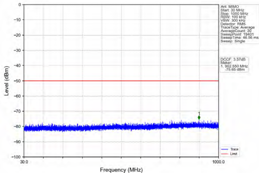
n78d_30kHz_MIMO_NTNV_60MHz_CP-OFDM_QPSK_3580.02MHz_Outer_Full
