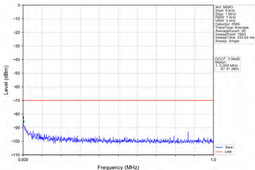
n78d_30kHz_MIMO_NTNV_60MHz_CP-OFDM_QPSK_3669.99MHz_Edge_1RB_Right
