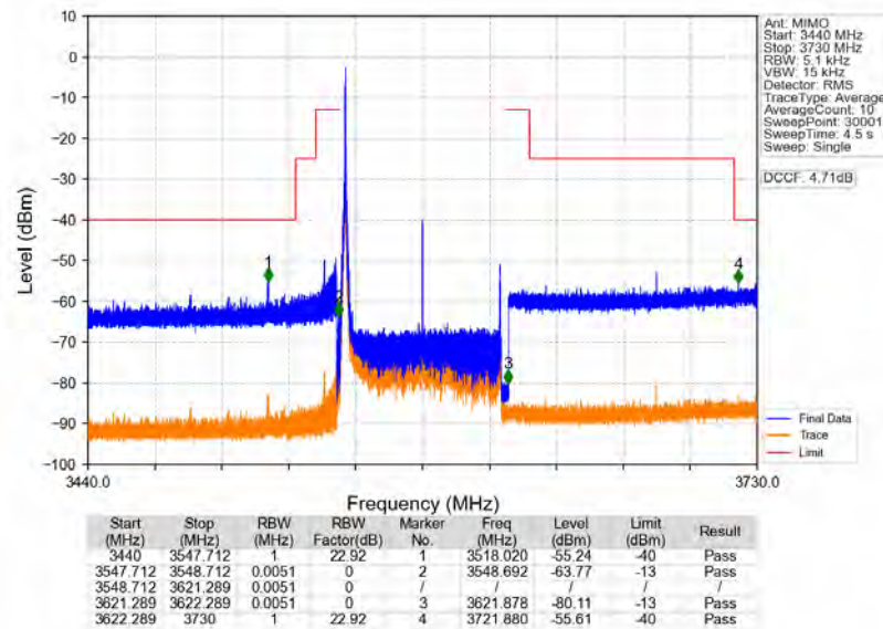
n78d_30kHz_MIMO_NTNV_70MHz_CP-OFDM_QPSK_3585MHz_Inner_1RB_Left
