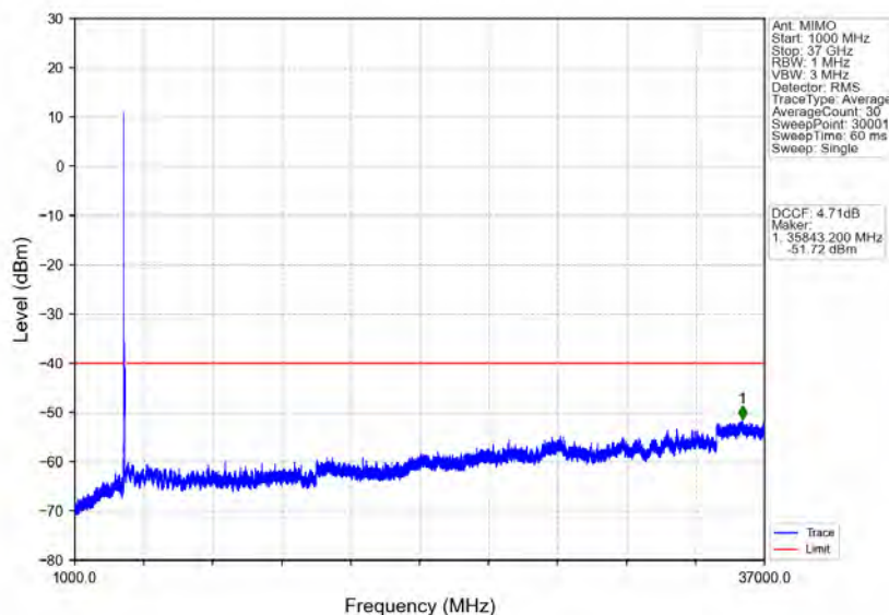
n78d_30kHz_MIMO_NTNV_70MHz_CP-OFDM QPSK_3664.98MHz_Edge_1RB_Right
