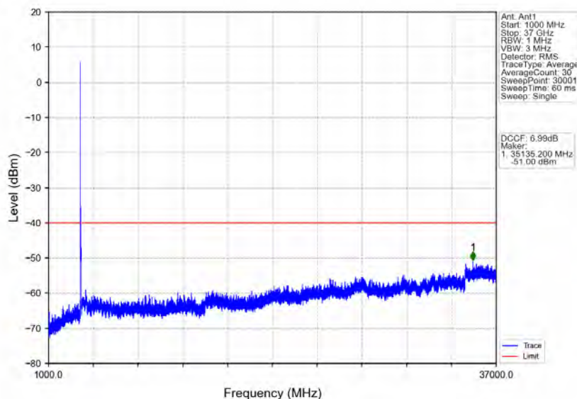
n78d_30kHz_MIMO_NTNV_70MHz_CP-OFDM_QPSK_3585MHz_Edge_1RB_Left
