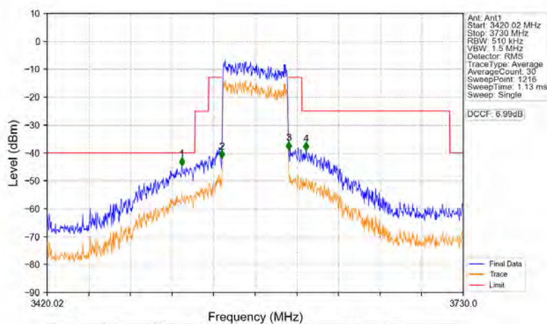
n78d 30kHz MIMO NTNV 50MHz CP-OFDM QPSK 3575.01MHz Outer Full
