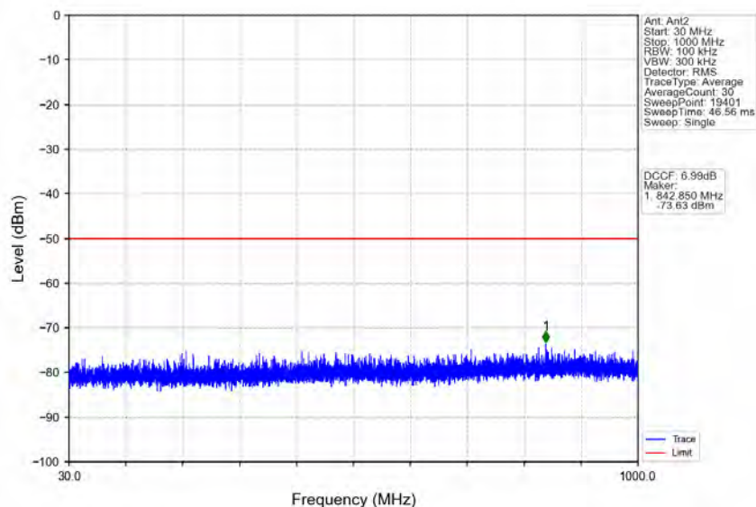
n78d_30kHz_MIMO_NTNV_70MHz_CP-OFDM_QPSK_3664.98MHz_Outer_Full
