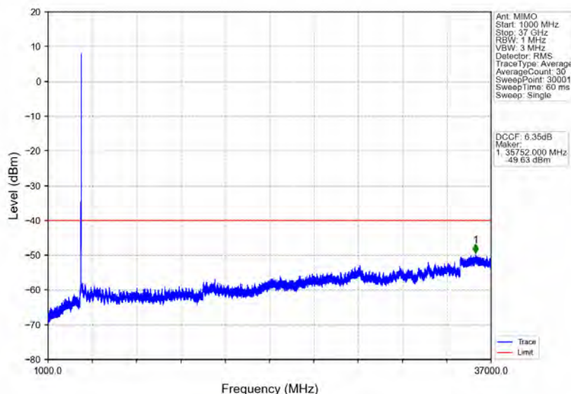
n78d_30kHz_MIMO_NTNV_60MHz_CP-OFDM QPSK_3669.99MHz_Inner_1RB_Right
