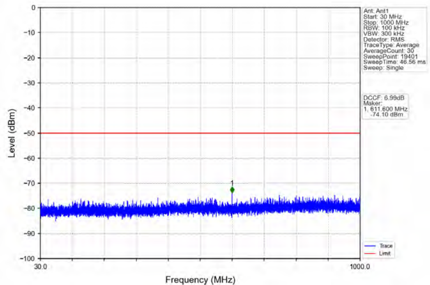
n78d_30kHz_MIMO_NTNV_70MHz_CP-OFDM_QPSK_3585MHz_Edge_1RB_Left
