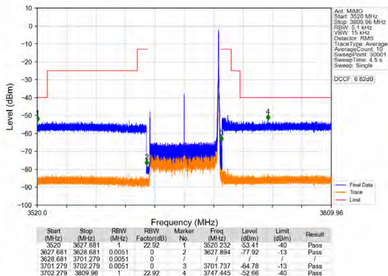
n78d_30kHz_MIMO_NTNV_70MHz_CP-OFDM_QPSK_3664.98MHz_Edge_1RB_Right
