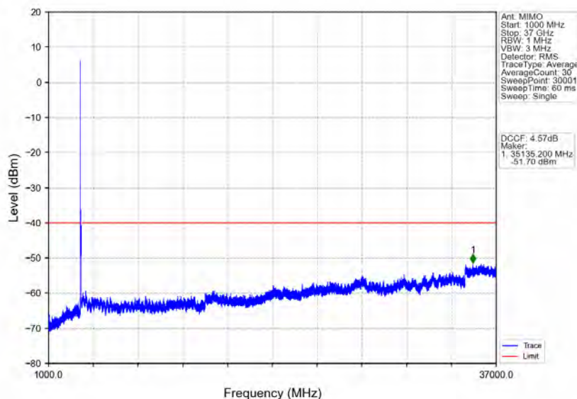
n78d_30kHz_MIMO_NTNV_70MHz_CP-OFDM QPSK_3585MHz_Outer_Full
