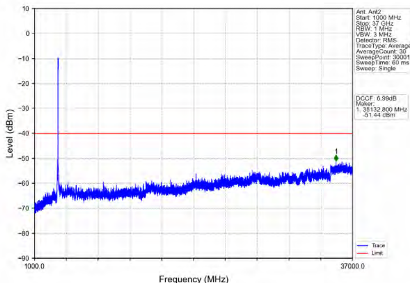
n78d_30kHz_MIMO_NTNV_70MHz_CP-OFDM_QPSK_3664.98MHz_Outer_Full
