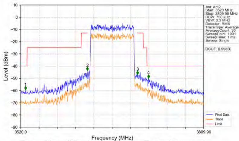
n78d_30kHz_MIMO_NTNV_70MHz_CP-OFDM_QPSK_3664.98MHz_Outer_Full
