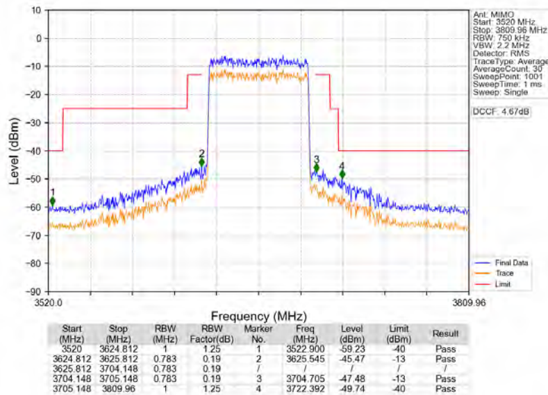
n78d_30kHz_MIMO_NTNV_70MHz_CP-OFDM_QPSK_3664.98MHz_Outer_Full
