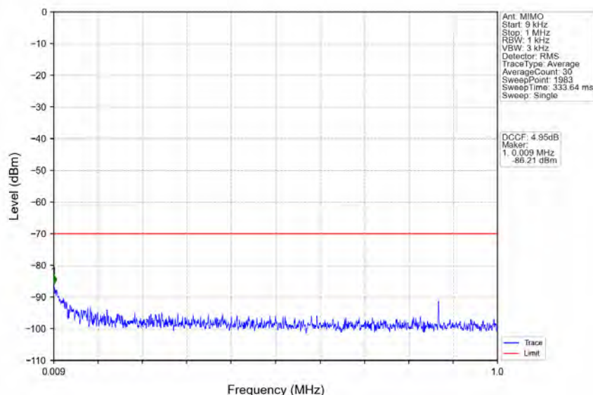
n78d_30kHz_MIMO_NTNV_60MHz_CP-OFDM_QPSK_3669.99MHz_Outer_Full
