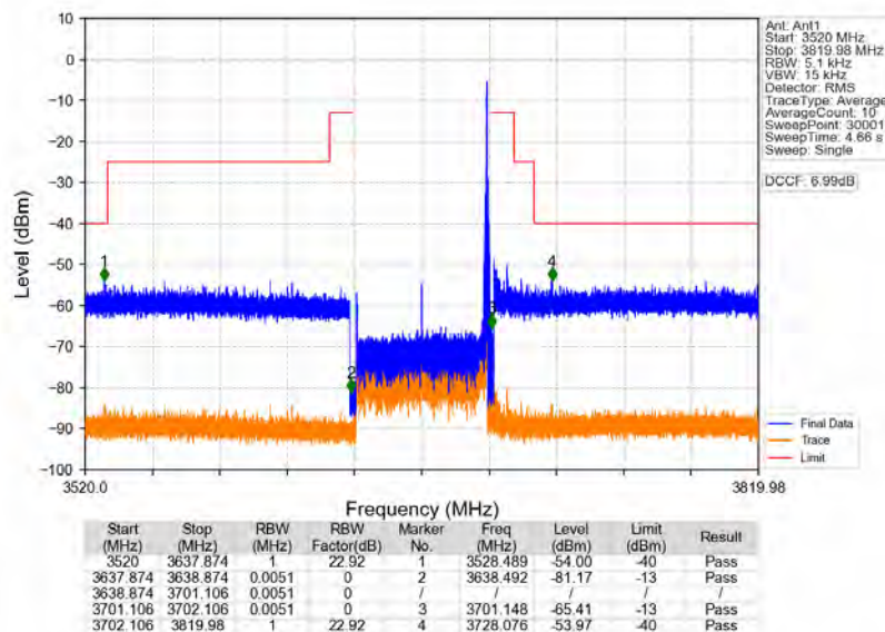
n78d_30kHz_MIMO_NTNV_60MHz_CP-OFDM_QPSK_3669.99MHz_Edge_1RB_Right
