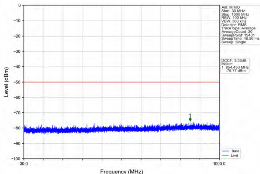
n78d_30kHz_MIMO_NTNV_60MHz_CP-OFDM_QPSK_3580.02MHz_Inner_1RB_Left
