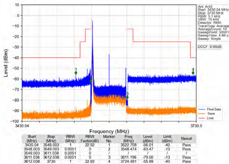
n78d_30kHz_MIMO_NTNV_60MHz_CP-OFDM_QPSK_3580.02MHz_Inner_1RB_Left
