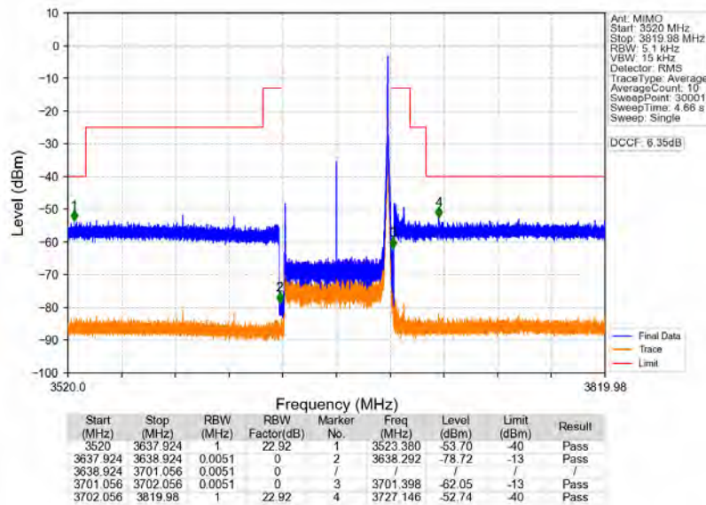
n78d_30kHz_MIMO_NTNV_60MHz_CP-OFDM_QPSK_3669.99MHz_Inner_1RB_Right
