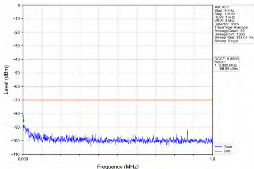
n78d_30kHz_MIMO_NTNV_60MHz_CP-OFDM_QPSK_3669.99MHz_Outer_Full
