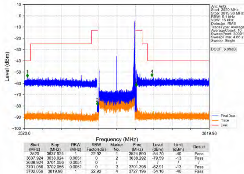
n78d_30kHz_MIMO_NTNV_60MHz_CP-OFDM_QPSK_3669.99MHz_Inner_1RB_Right
