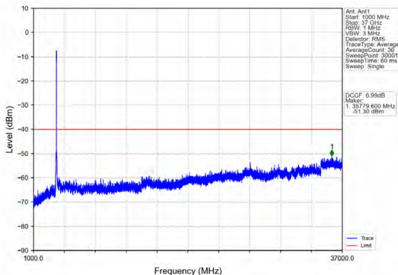
n78d_30kHz_MIMO_NTNV_60MHz_CP-OFDM_QPSK_3669.99MHz_Outer_Full
