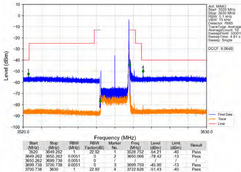
n78d_30kHz_MIMO_NTNV_50MHz_CP-OFDM_QPSK_3675MHz_Edge_1RB_Right
