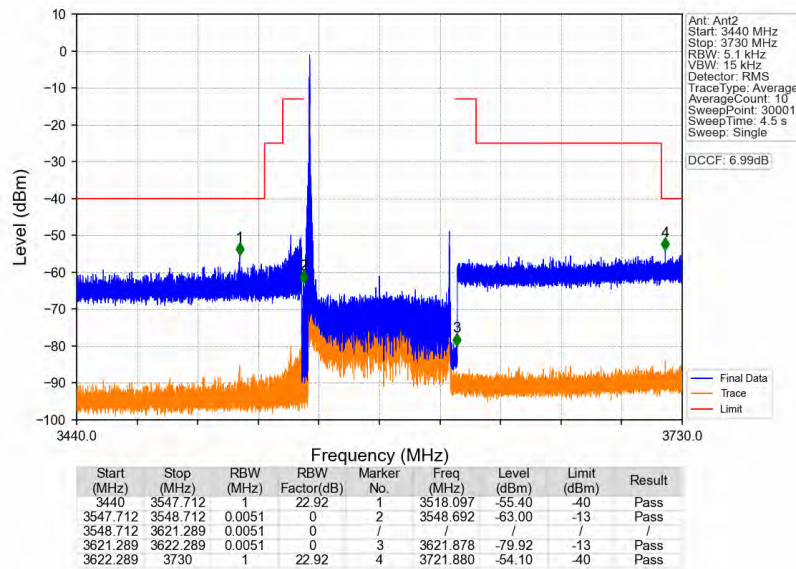
n78d_30kHz_MIMO_NTNV_70MHz_CP-OFDM_QPSK_3585MHz_Inner_1RB_Left
