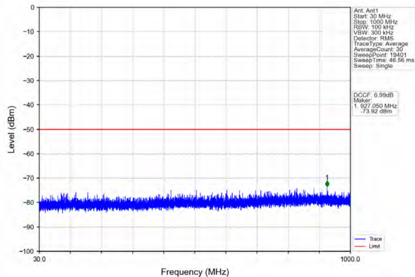
n78d_30kHz_MIMO_NTNV_50MHz_CP-OFDM_QPSK_3675MHz_Edge_1RB_Right
