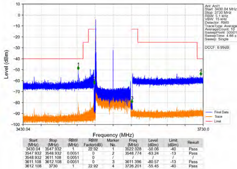
n78d 30kHz MIMO_NTNV_60MHz_CP-OFDM QPSK_3580.02MHz_Edge_1RB_Left
