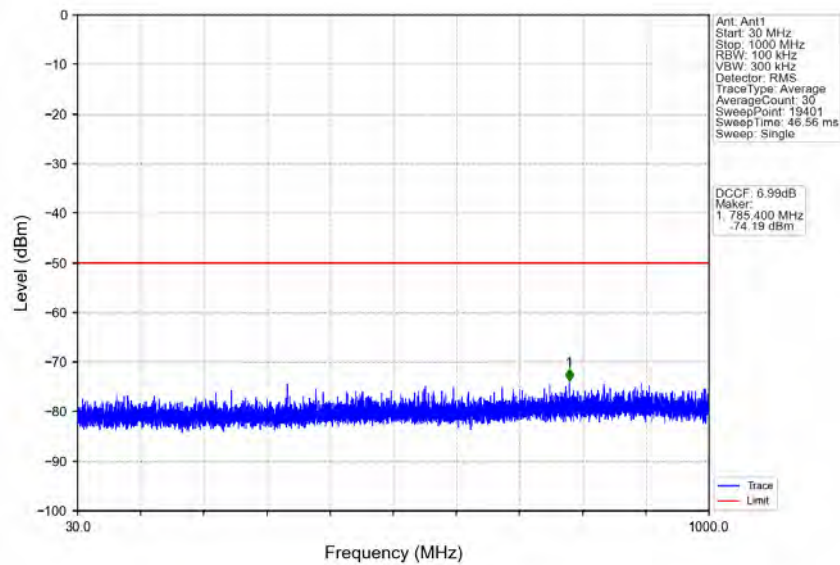
n78d_30kHz_MIMO_NTNV_60MHz_CP-OFDM_QPSK_3669.99MHz_Edge_1RB_Right
