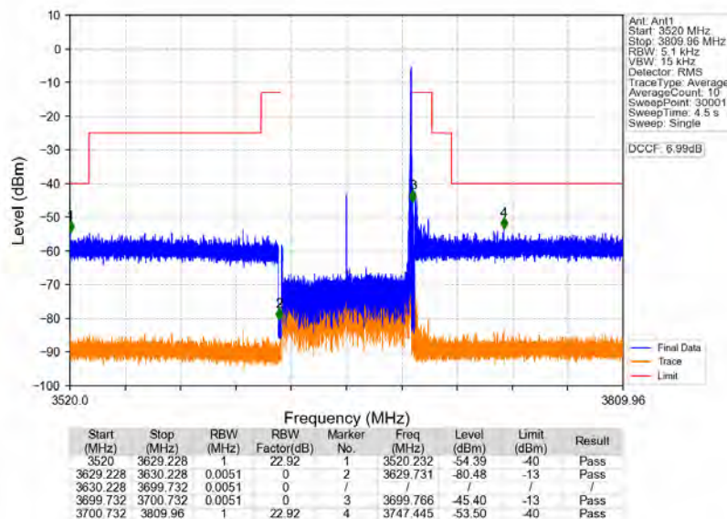
n78d_30kHz_MIMO_NTNV_70MHz_CP-OFDM QPSK_3664.98MHz_Edge_1RB_Right
