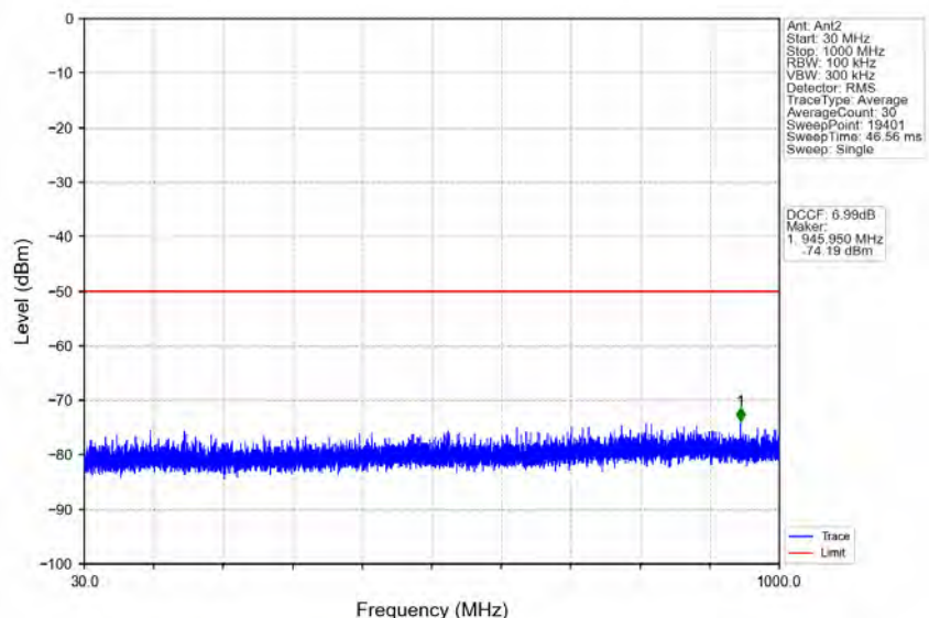
n78d_30kHz_MIMO_NTNV_60MHz_CP-OFDM_QPSK_3580.02MHz_Outer_Full
