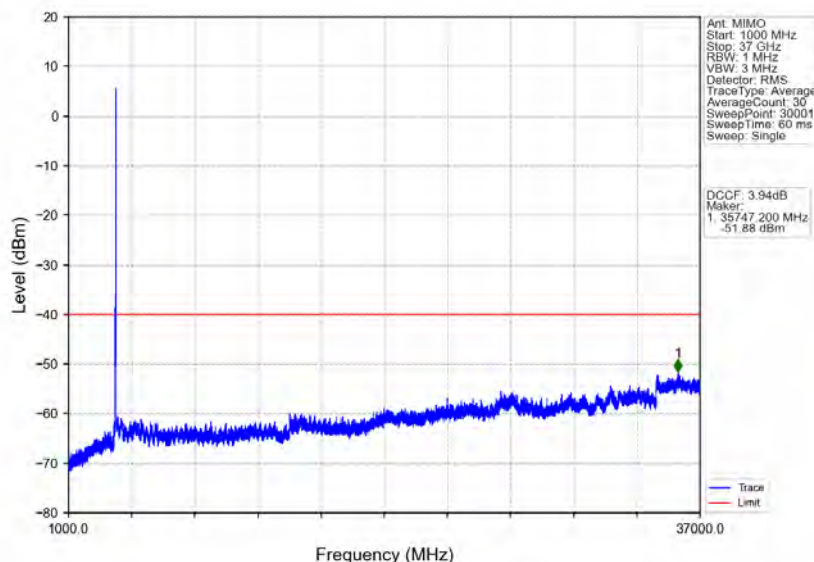
n78d_30kHz_MIMO_NTNV_60MHz_CP-OFDM QPSK_3669.99MHz_Edge_1RB_Right
