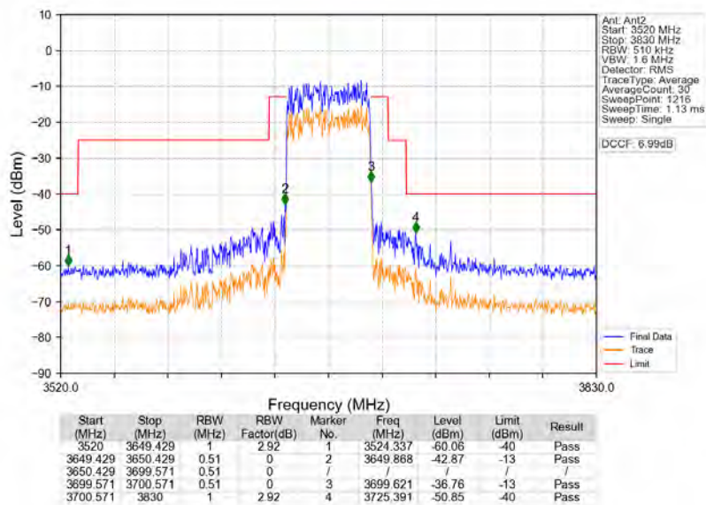
n78d_30kHz_MIMO_NTNV_50MHz_CP-OFDM_QPSK_3675MHz_Outer_Full
