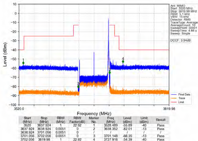
n78d_30kHz_MIMO_NTNV_60MHz_CP-OFDM_QPSK_3669.99MHz_Edge_1RB_Right
