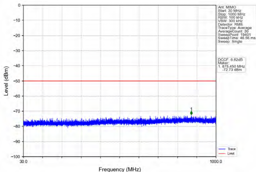
n78d_30kHz_MIMO_NTNV_70MHz_CP-OFDM QPSK_3664.98MHz_Edge_1RB_Right
