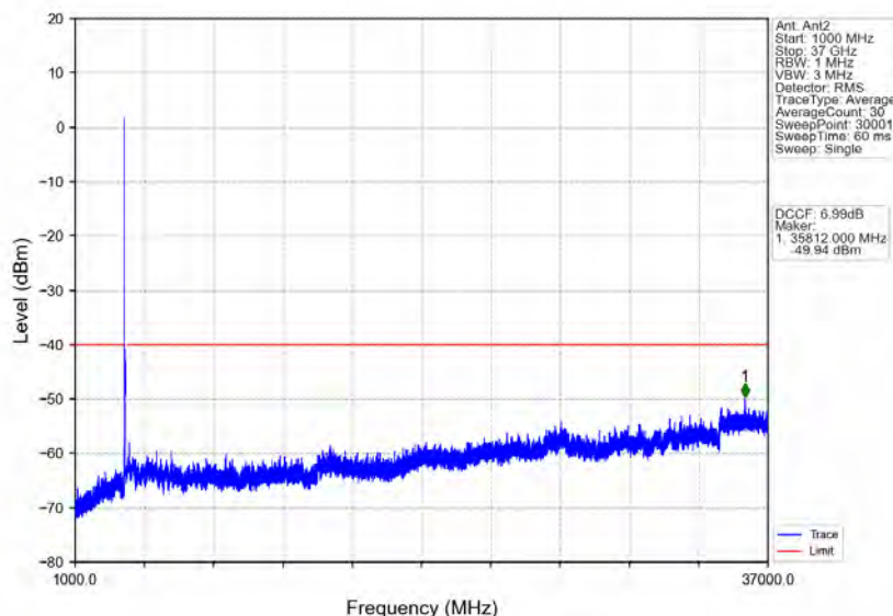
n78d_30kHz_MIMO_NTNV_60MHz_CP-OFDM_QPSK_3580.02MHz_Inner_1RB_Left
