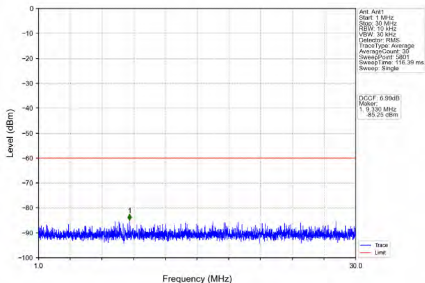
n78d_30kHz_MIMO_NTNV_70MHz_CP-OFDM_QPSK_3585MHz_Inner_1RB_Left
