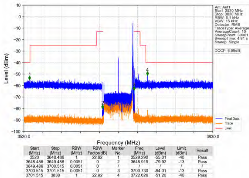
n78d_30kHz_MIMO_NTNV_50MHz_CP-OFDM_QPSK_3675MHz_Edge_1RB_Right
