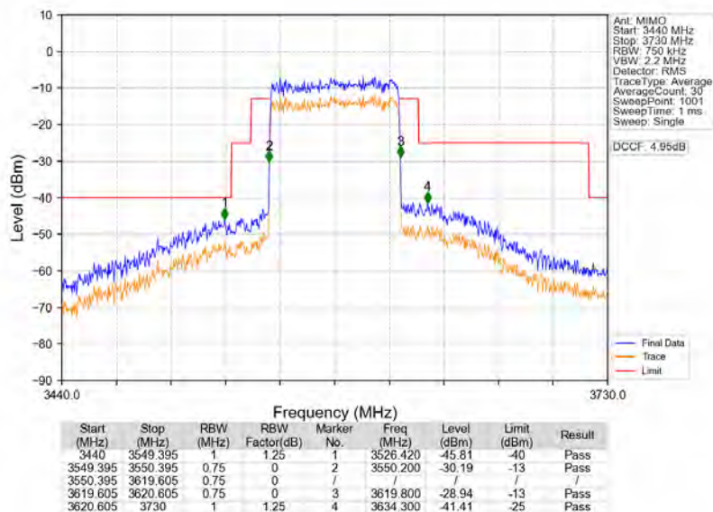
n78d_30kHz_MIMO_NTNV_70MHz_CP-OFDM_QPSK_3585MHz_Outer_Full
