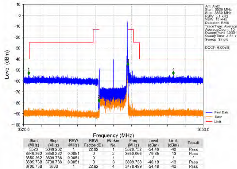
n78d_30kHz_MIMO_NTNV_50MHz_CP-OFDM_QPSK_3675MHz_Edge_1RB_Right
