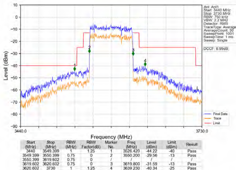
n78d_30kHz_MIMO_NTNV_70MHz_CP-OFDM QPSK_3585MHz_Outer_Full
