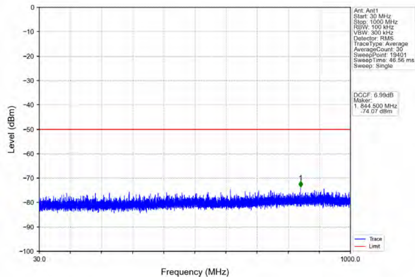
n78d_30kHz_MIMO_NTNV_70MHz_CP-OFDM_QPSK_3585MHz_Outer_Full
