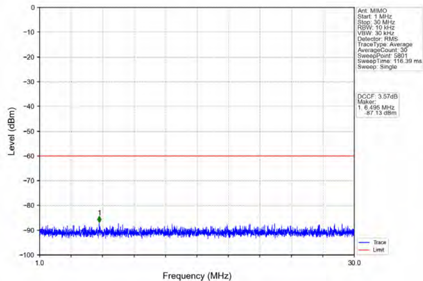
n78d_30kHz_MIMO_NTNV_60MHz_CP-OFDM_QPSK_3580.02MHz_Outer_Full
