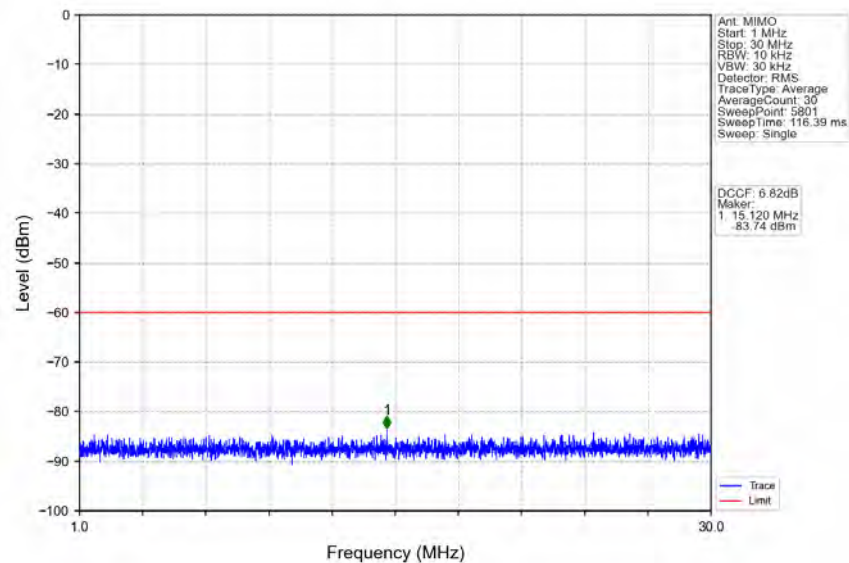
n78d_30kHz_MIMO_NTNV_70MHz_CP-OFDM QPSK_3664.98MHz_Edge_1RB_Right
