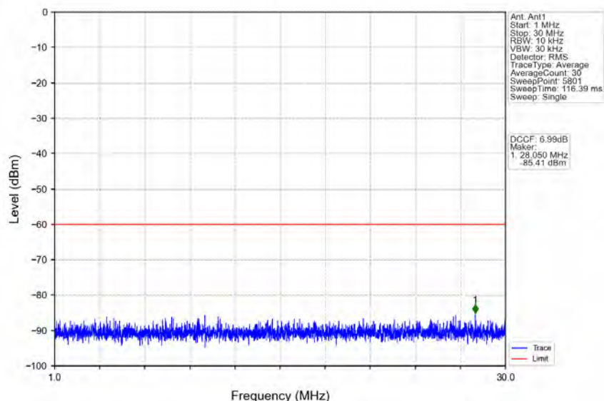
n78d_30kHz_MIMO_NTNV_70MHz_CP-OFDM_QPSK_3585MHz_Outer_Full
