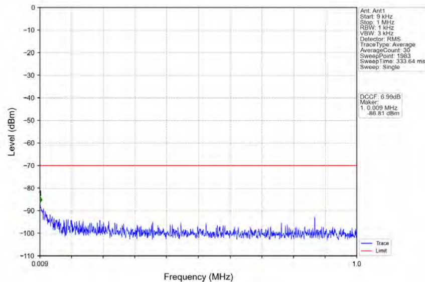
n78d_30kHz_MIMO_NTNV_60MHz_CP-OFDM_QPSK_3669.99MHz_Inner_1RB_Right
