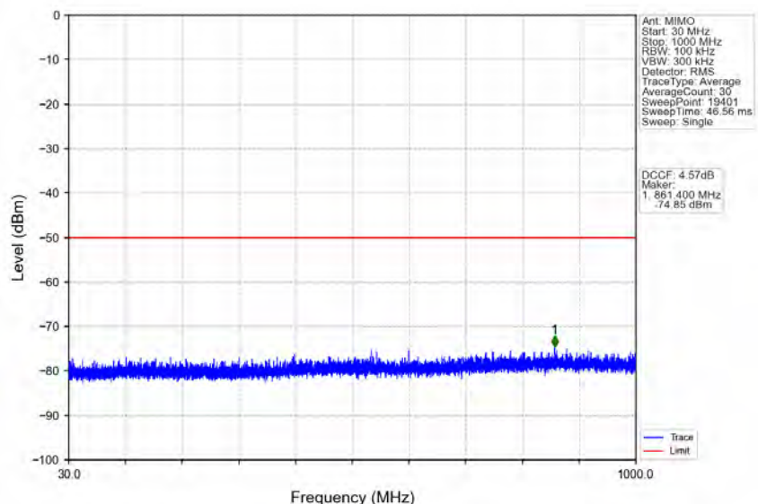
n78d_30kHz_MIMO_NTNV_70MHz_CP-OFDM_QPSK_3585MHz_Edge_1RB_Left
