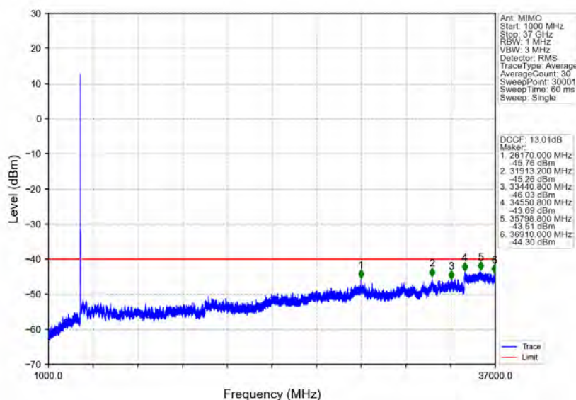
n78d 30kHz MIMO NTNV 50MHz CP-OFDM QPSK 3575.01MHz Outer Full
