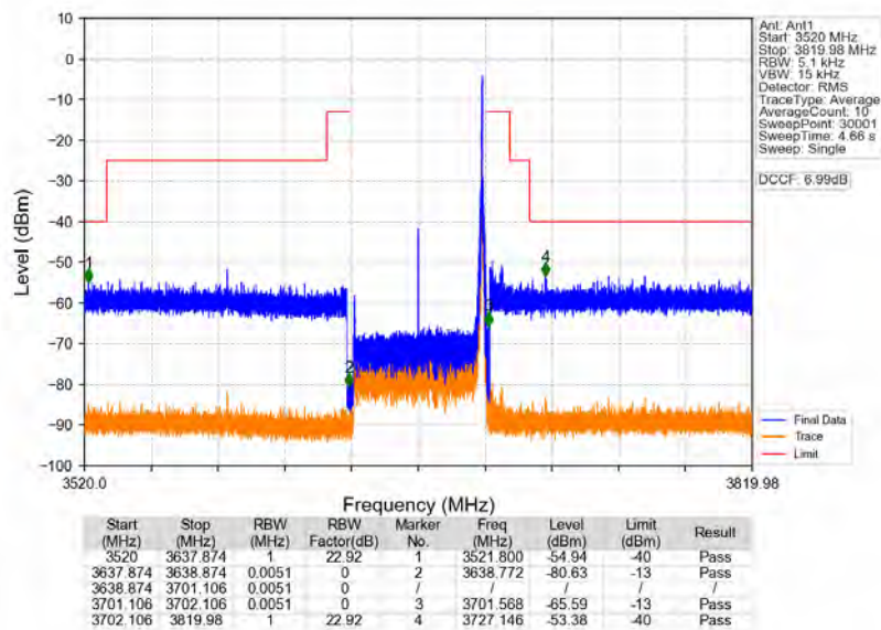
n78d_30kHz_MIMO_NTNV_60MHz_CP-OFDM_QPSK_3669.99MHz_Inner_1RB_Right
