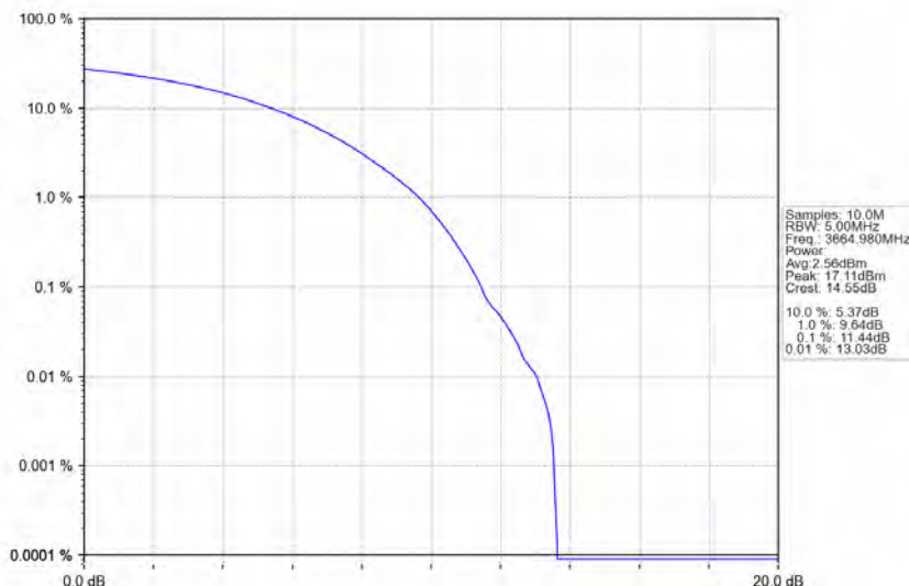
n78d_30kHz_MIMO_NTNV_70MHz_CP-OFDM_16_QAM_3664.98MHz_Outer_Full
