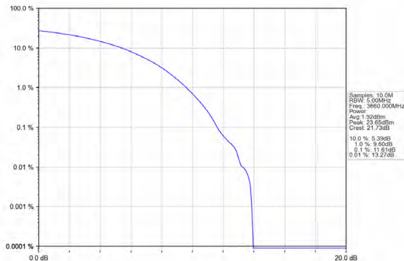
n78d_30kHz_MIMO_NTNV_80MHz_CP-OFDM_16_QAM_3660MHz_Outer_Full
