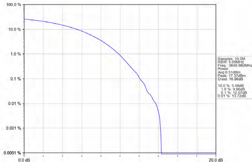
n78d_30kHz_MIMO_NTNV_100MHz_CP-OFDM 16 QAM_3649.98MHz_Outer_Full
