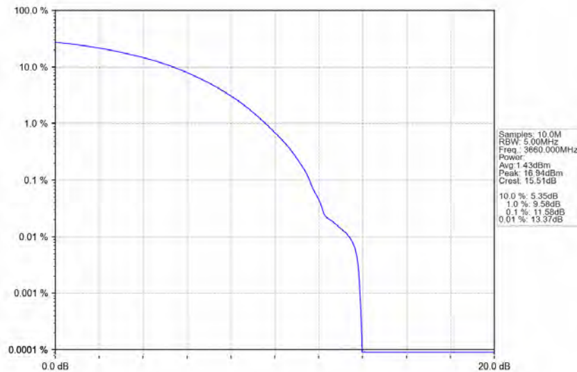
n78d_30kHz_MIMO_NTNV_80MHz_CP-OFDM_64_QAM_3660MHz_Outer_Full
