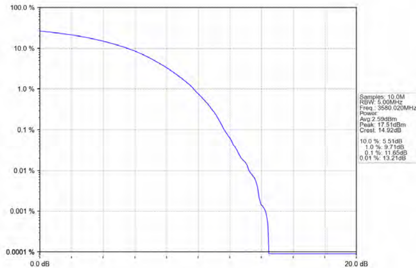
n78d_30kHz_MIMO_NTNV_60MHz_CP-OFDM_64_QAM_3580.02MHz_Outer_Full
