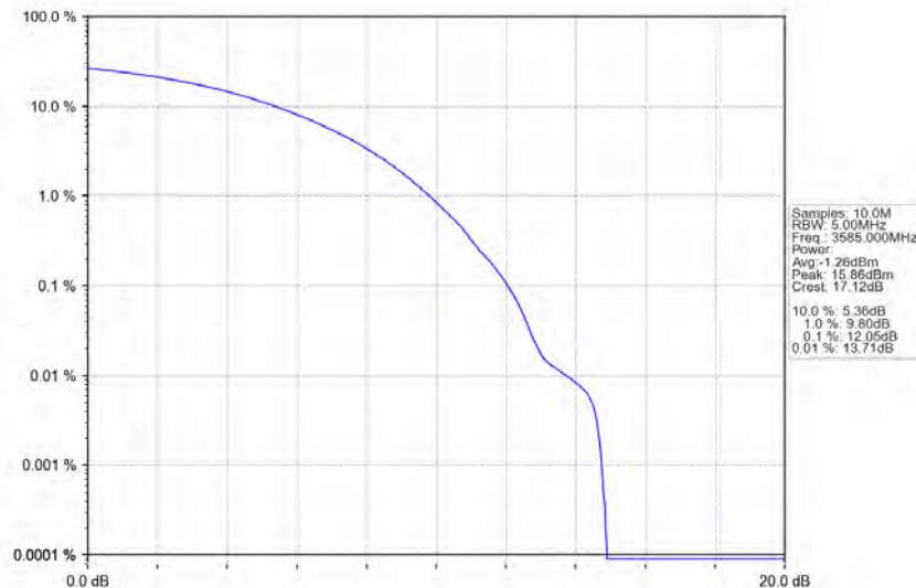
n78d_30kHz_MIMO_NTNV_70MHz_CP-OFDM_256_QAM_3585MHz_Outer_Full
