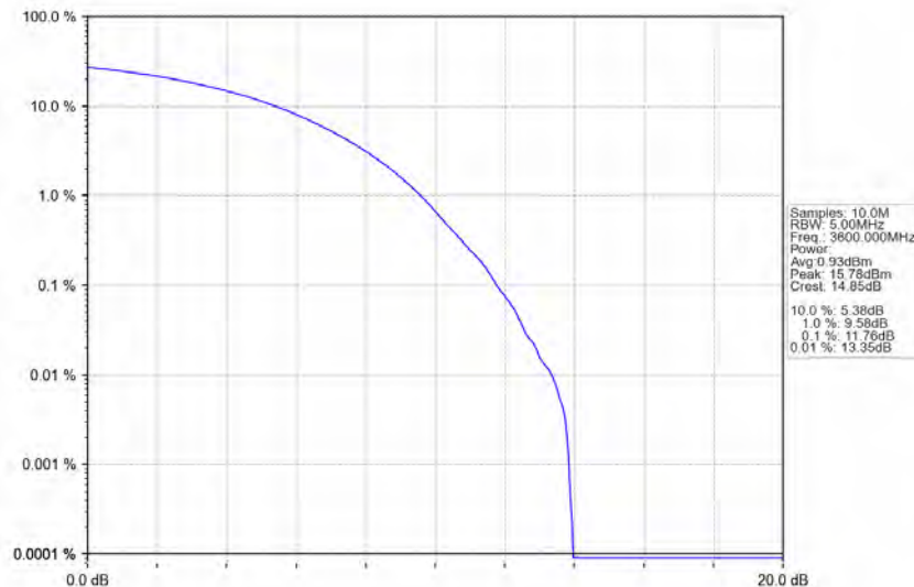
n78d_30kHz_MIMO_NTNV_100MHz_CP-OFDM_16_QAM_3600MHz_Outer_Full
