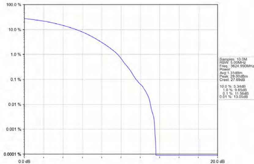
n78d_30kHz_MIMO_NTNV_90MHz_CP-OFDM_16_QAM_3624.99MHz_Outer_Full
