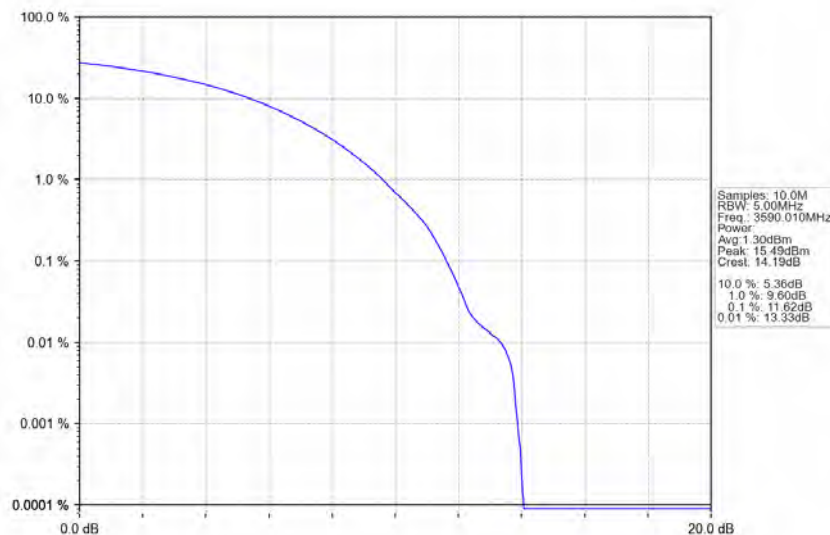
n78d_30kHz_MIMO_NTNV_80MHz_CP-OFDM_64_QAM_3590.01MHz_Outer_Full
