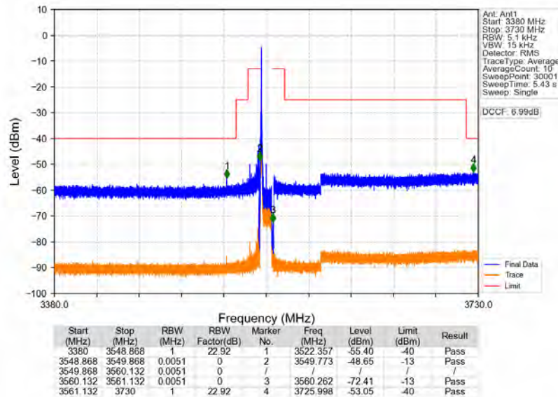
n78d 30kHz MIMO_NTNV_10MHz_CP-OFDM QPSK 3555MHz Edge_1RB Left
