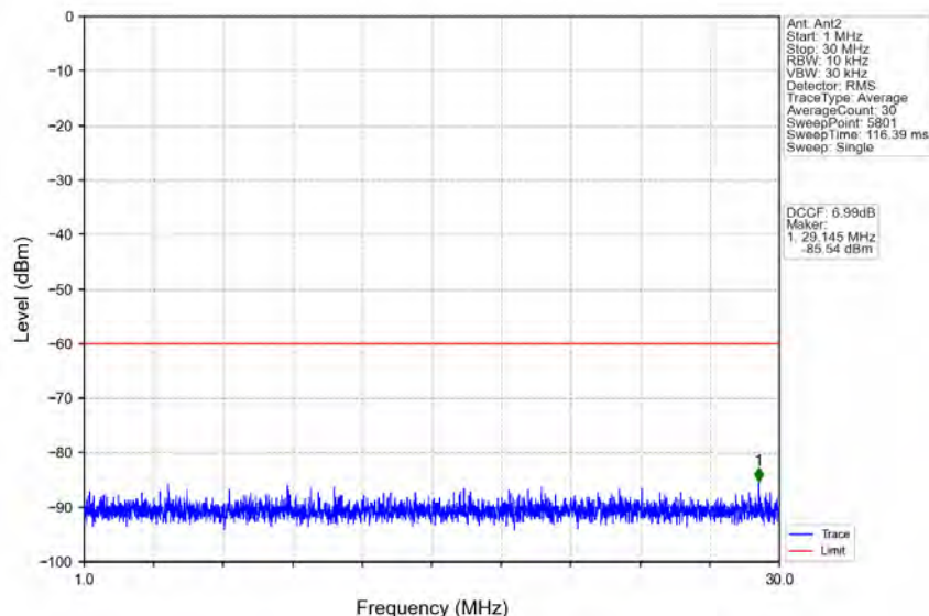
n78d_30kHz_MIMO_NTNV_15MHz_CP-OFDM_QPSK_3557.52MHz_Inner_1RB_Left
