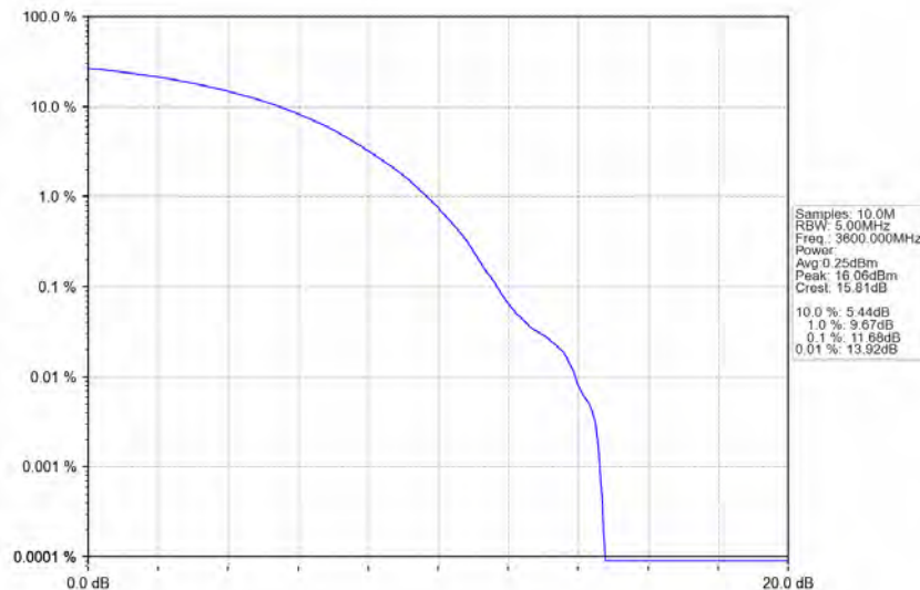
n78d_30kHz_MIMO_NTNV_100MHz_CP-OFDM 64 QAM_3600MHz_Outer_Full
