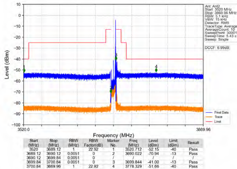
n78d_30kHz_MIMO_NTNV_10MHz_CP-OFDM_QPSK_3694.98MHz_Edge_1RB_Right
