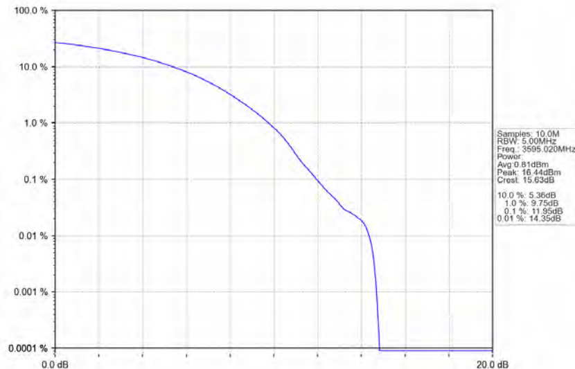
n78d_30kHz_MIMO_NTNV_90MHz_CP-OFDM_64_QAM_3595.02MHz_Outer_Full
