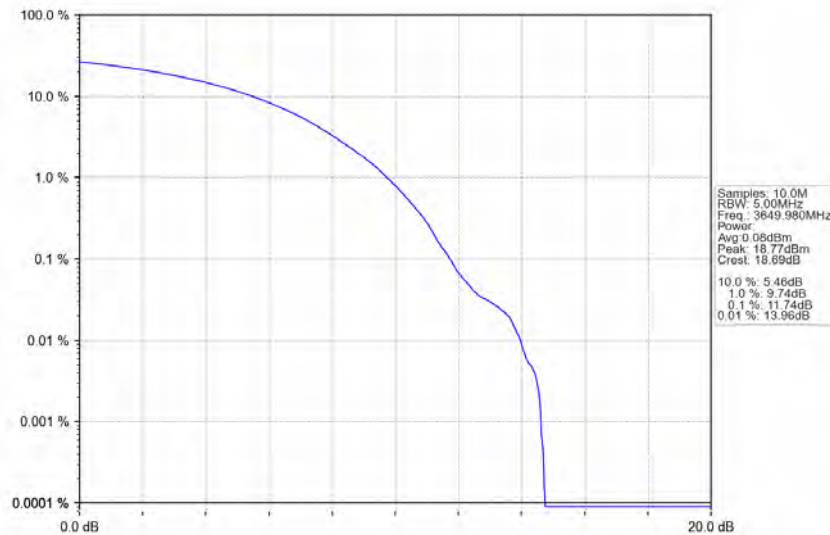
n78d_30kHz_MIMO_NTNV_100MHz_CP-OFDM 64 QAM_3649.98MHz_Outer_Full
