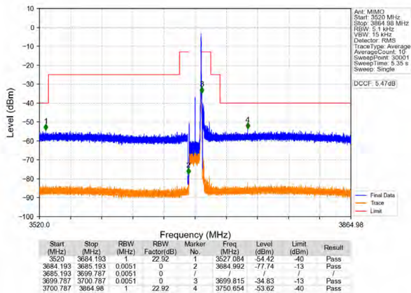
n78d_30kHz_MIMO_NTNV_15MHz_CP-OFDM_QPSK_3692.49MHz_Edge_1RB_Right
