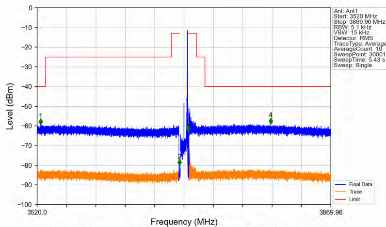
n78d_30kHz_MIMO_NTNV_10MHz_CP-OFDM QPSK_3694.98MHz_Edge_1RB_Right
