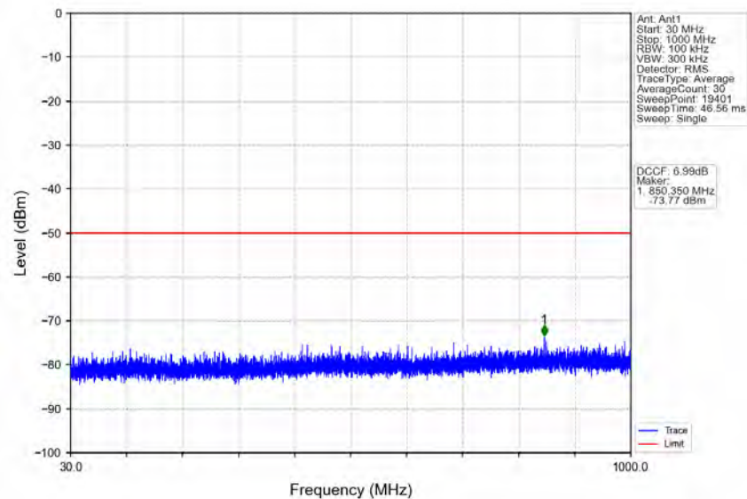
n78d_30kHz_MIMO_NTNV_20MHz_CP-OFDM_QPSK_3560.01MHz_Outer_Full
