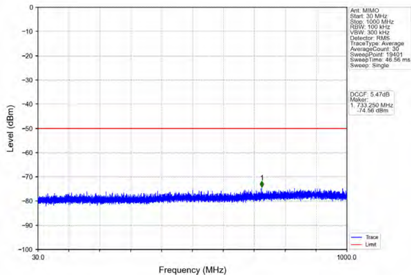
n78d_30kHz_MIMO_NTNV_15MHz_CP-OFDM_QPSK_3557.52MHz_Outer_Full
