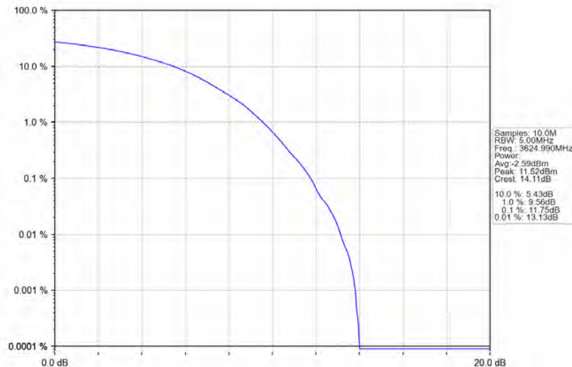
n78d_30kHz_MIMO_NTNV_100MHz_CP-OFDM_256_QAM_3624.99MHz_Outer_Full
