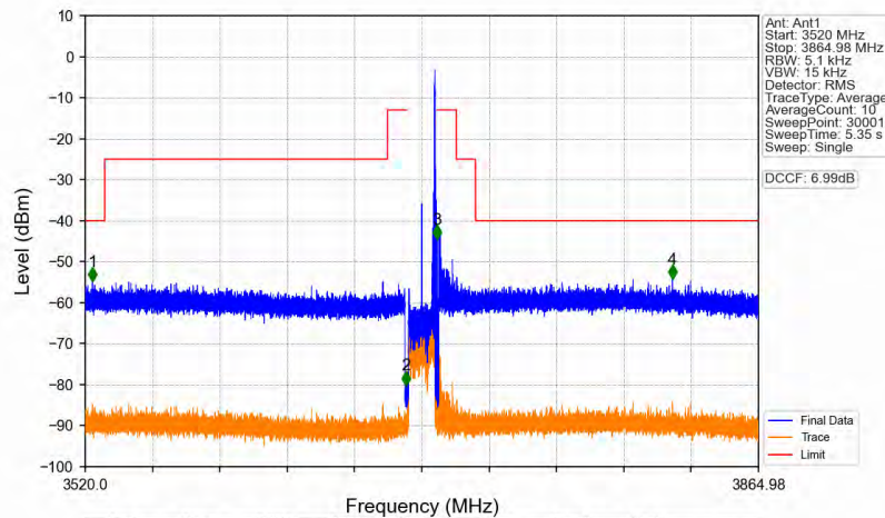
n78d_30kHz_MIMO_NTNV_15MHz_CP-OFDM_QPSK_3692.49MHz_Edge_1RB_Right
