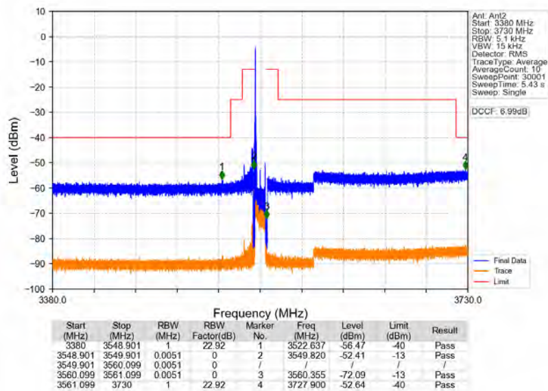
n78d_30kHz_MIMO_NTNV_10MHz_CP-OFDM_QPSK_3555MHz_Edge_1RB_Left
