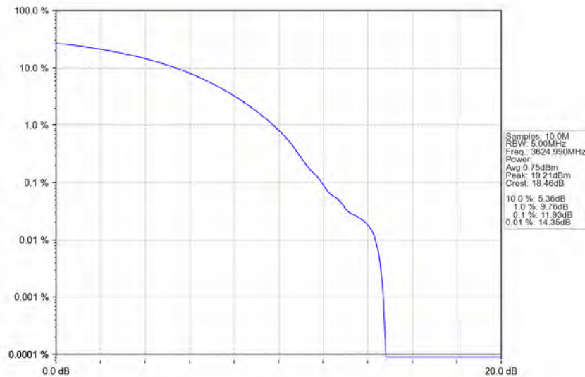
n78d_30kHz_MIMO_NTNV_90MHz_CP-OFDM_64_QAM_3624.99MHz_Outer_Full
