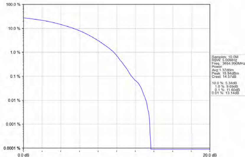
n78d_30kHz_MIMO_NTNV_90MHz_CP-OFDM_16_QAM_3654.99MHz_Outer_Full
