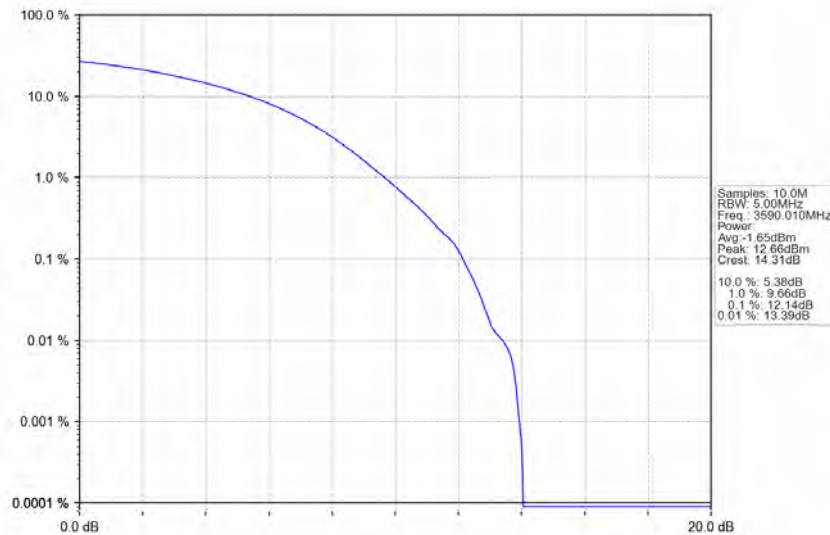
n78d_30kHz_MIMO_NTNV_80MHz_CP-OFDM_256_QAM_3590.01MHz_Outer_Full
