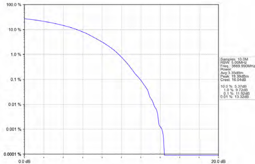
n78d_30kHz_MIMO_NTNV_60MHz_CP-OFDM_16_QAM_3669.99MHz_Outer_Full
