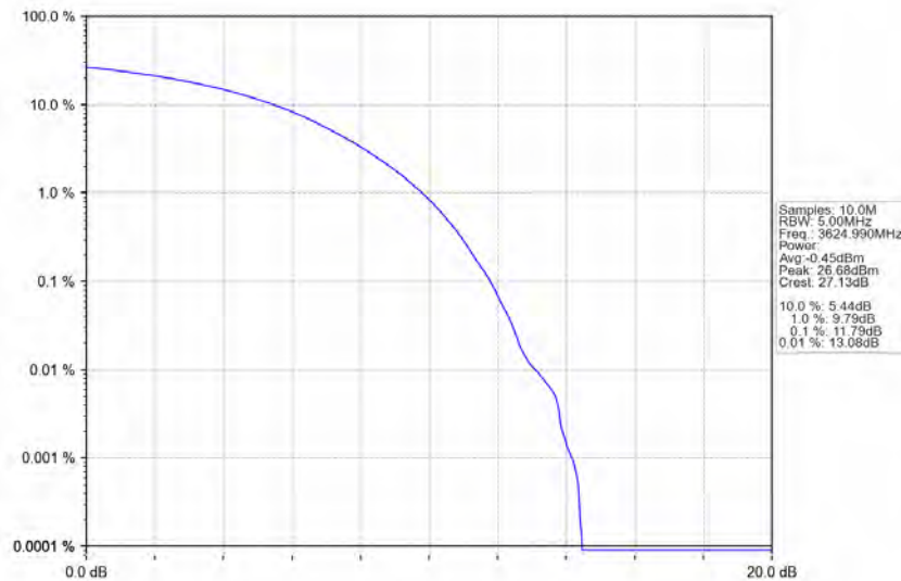
n78d_30kHz_MIMO_NTNV_60MHz_CP-OFDM_256_QAM_3624.99MHz_Outer_Full
