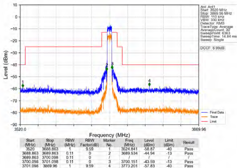
n78d_30kHz_MIMO_NTNV_10MHz_CP-OFDM_QPSK_3694.98MHz_Outer_Full
