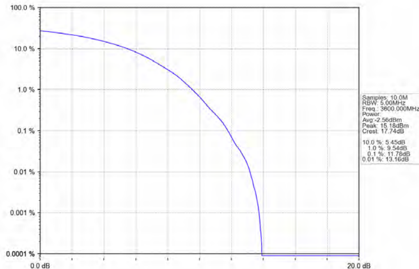
n78d_30kHz_MIMO_NTNV_100MHz_CP-OFDM_256_QAM_3600MHz_Outer_Full
