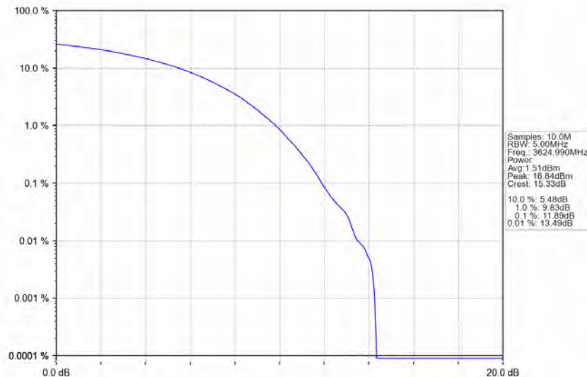
n78d_30kHz_MIMO_NTNV_80MHz_CP-OFDM_16_QAM_3624.99MHz_Outer_Full
