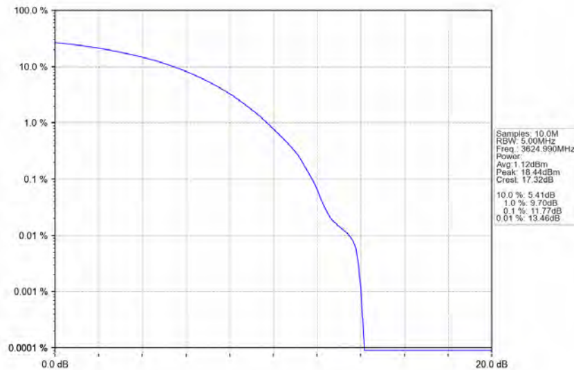
n78d_30kHz_MIMO_NTNV_80MHz_CP-OFDM_64_QAM_3624.99MHz_Outer_Full
