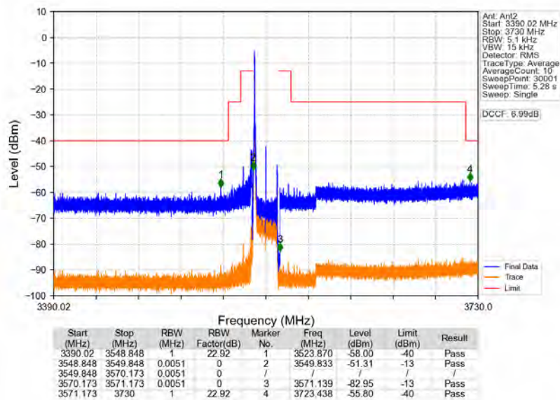
n78d_30kHz_MIMO_NTNV_20MHz_CP-OFDM_QPSK_3560.01MHz_Edge_1RB_Left
