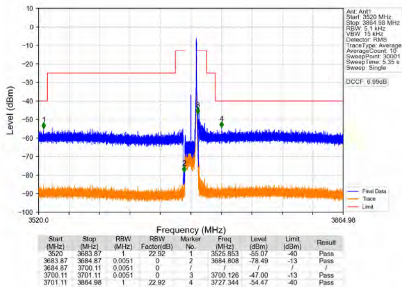
n78d_30kHz_MIMO_NTNV_15MHz_CP-OFDM_QPSK_3692.49MHz_Inner_1RB_Right
