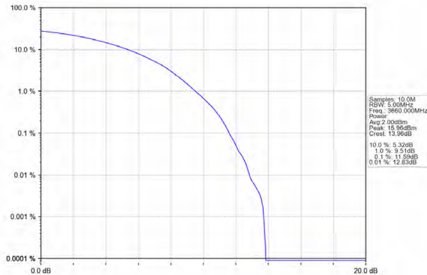
n78d_30kHz_MIMO_NTNV_80MHz_CP-OFDM QPSK_3660MHz_Outer_Full
