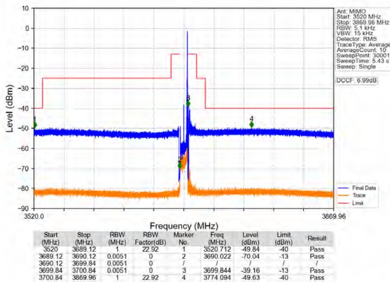
n78d_30kHz_MIMO_NTNV_10MHz_CP-OFDM_QPSK_3694.98MHz_Edge_1RB_Right
