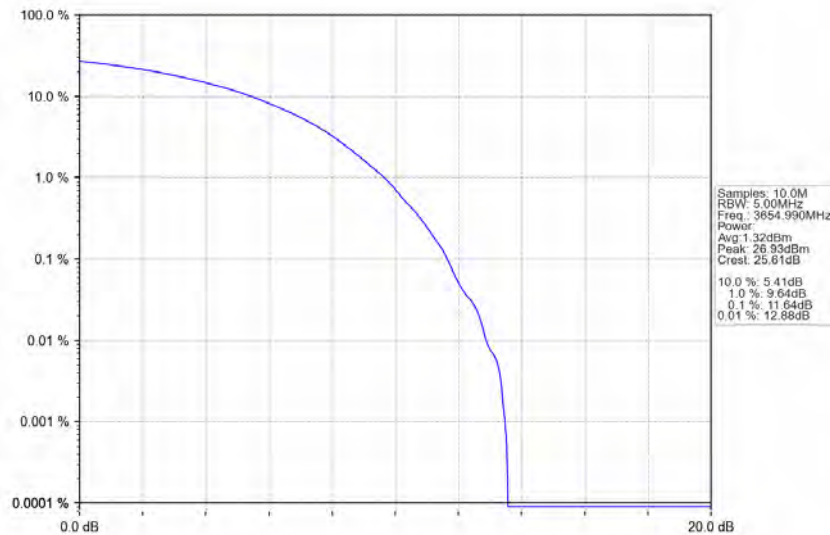
n78d_30kHz_MIMO_NTNV_90MHz_CP-OFDM_QPSK_3654.99MHz_Outer_Full
