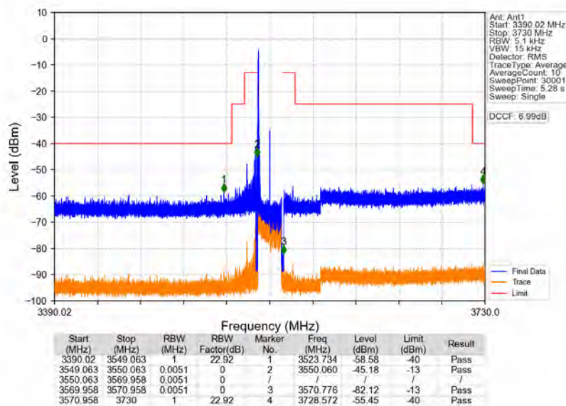
n78d 30kHz MIMO_NTNV_20MHz_CP-OFDM QPSK_3560.01MHz_Edge_1RB_Left
