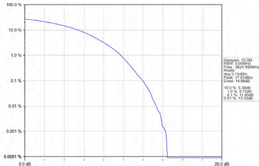
n78d_30kHz_MIMO_NTNV_60MHz_CP-OFDM_16_QAM_3624.99MHz_Outer_Full
