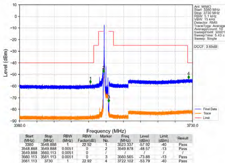
n78d_30kHz_MIMO_NTNV_10MHz_CP-OFDM_QPSK_3555MHz_Inner_1RB_Left
