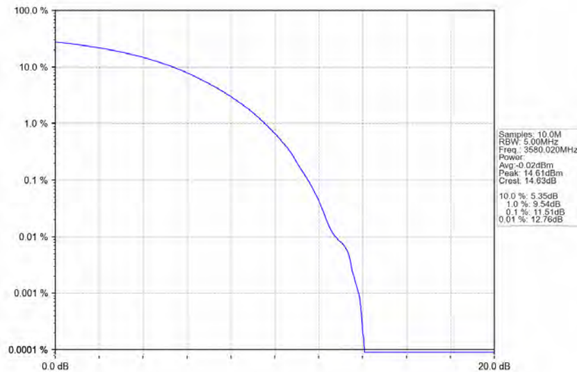
n78d_30kHz_MIMO_NTNV_60MHz_CP-OFDM_256_QAM_3580.02MHz_Outer_Full
