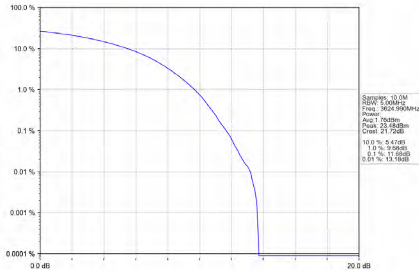
n78d_30kHz_MIMO_NTNV_70MHz_CP-OFDM_64_QAM_3624.99MHz_Outer_Full
