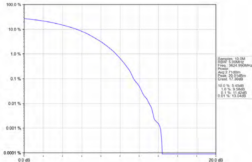
n78d_30kHz_MIMO_NTNV_60MHz_CP-OFDM_64_QAM_3624.99MHz_Outer_Full
