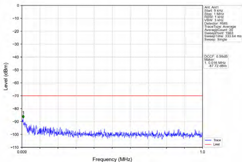
n78d 30kHz MIMO_NTNV_20MHz_CP-OFDM QPSK_3560.01MHz_Edge_1RB_Left
