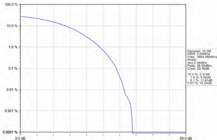
n78d_30kHz_MIMO_NTNV_70MHz_CP-OFDM_QPSK_3664.98MHz_Outer_Full
