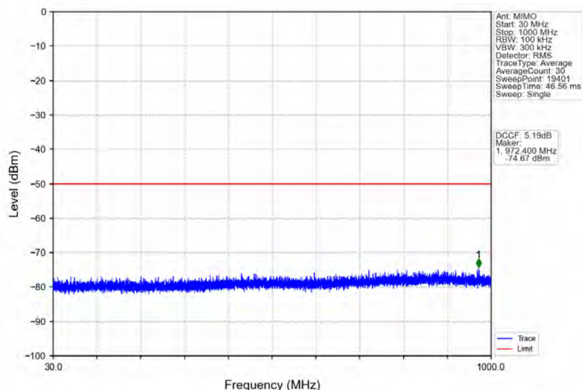
n78d_30kHz_MIMO_NTNV_15MHz_CP-OFDM_QPSK_3557.52MHz_Inner_1RB_Left
