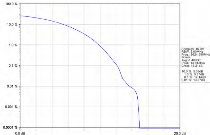
n78d_30kHz_MIMO_NTNV_70MHz_CP-OFDM_256_QAM_3624.99MHz_Outer_Full
