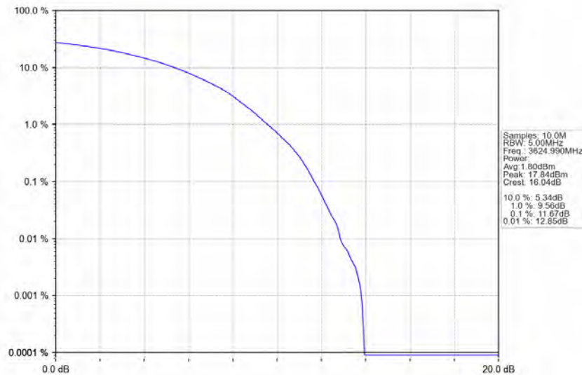
n78d_30kHz_MIMO_NTNV_80MHz_CP-OFDM QPSK_3624.99MHz_Outer_Full
