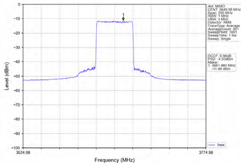
n78d_30kHz_MIMO_NTNV_100MHz_CP-OFDM 64 QAM_3649.98MHz_Inner_Full
