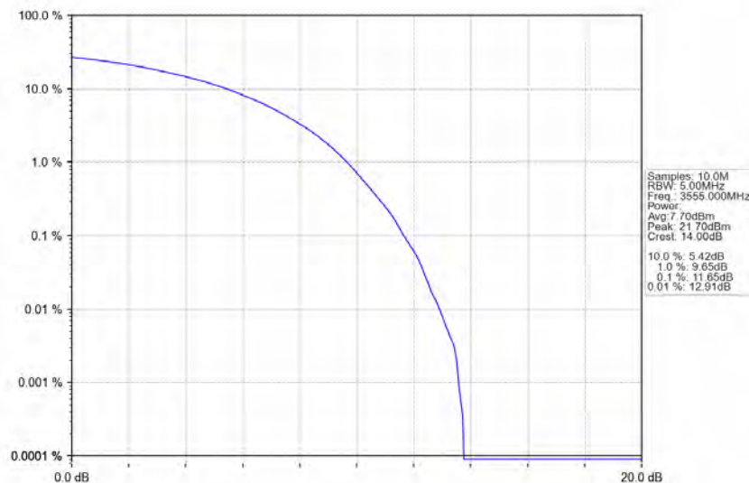
n78d_30kHz_MIMO_NTNV_10MHz_CP-OFDM_256_QAM_3555MHz_Outer_Full
