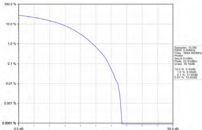
n78d_30kHz_MIMO_NTNV_30MHz_CP-OFDM QPSK_3684.99MHz_Outer_Full
