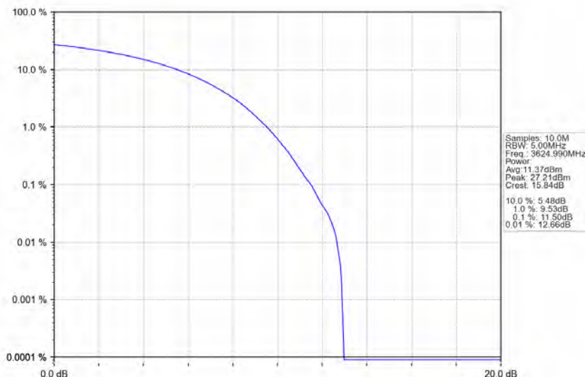
n78d_30kHz_MIMO_NTNV_10MHz_CP-OFDM_QPSK_3624.99MHz_Outer_Full
