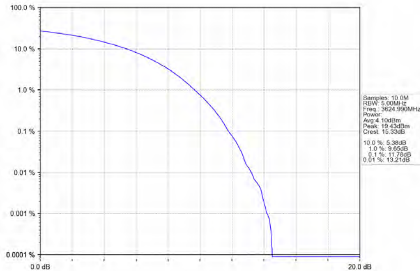
n78d_30kHz_MIMO_NTNV_50MHz_CP-OFDM QPSK_3624.99MHz_Outer_Full
