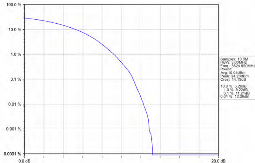
n78d_30kHz_MIMO_NTNV_15MHz_CP-OFDM_16_QAM_3624.99MHz_Outer_Full
