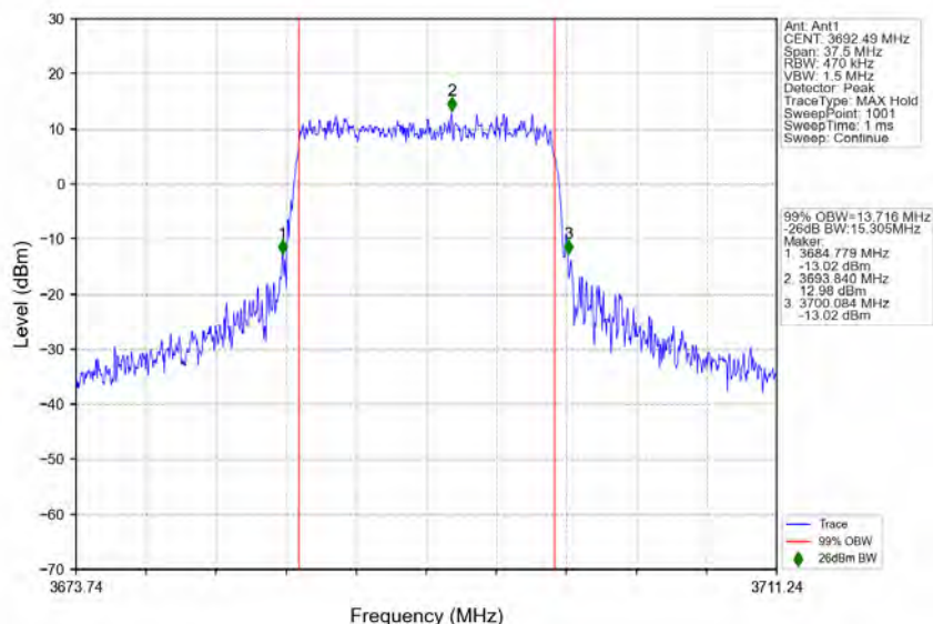
n78d_30kHz_MIMO_NTNV_15MHz_CP-OFDM_64_QAM_3692.49MHz_Outer_Full
