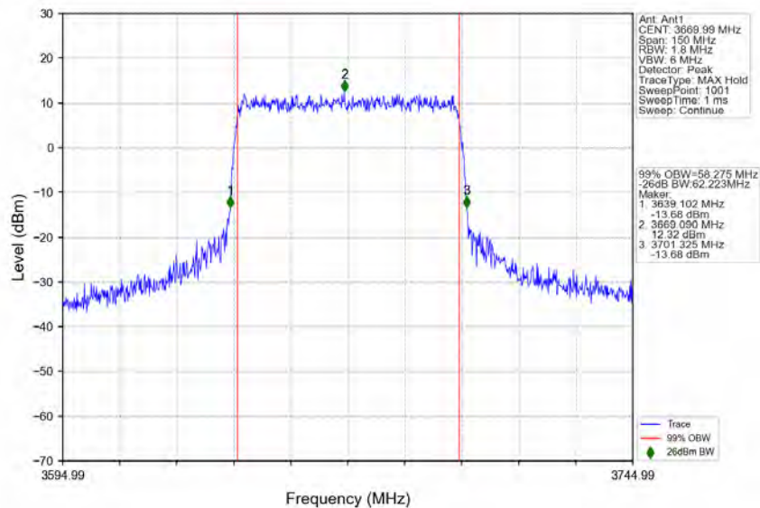
n78d_30kHz_MIMO_NTNV_60MHz_CP-OFDM_64_QAM_3669.99MHz_Outer_Full
