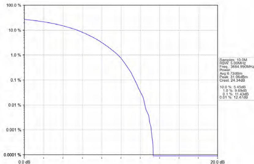
n78d_30kHz_MIMO_NTNV_30MHz_CP-OFDM 16 QAM_3684.99MHz_Outer_Full
