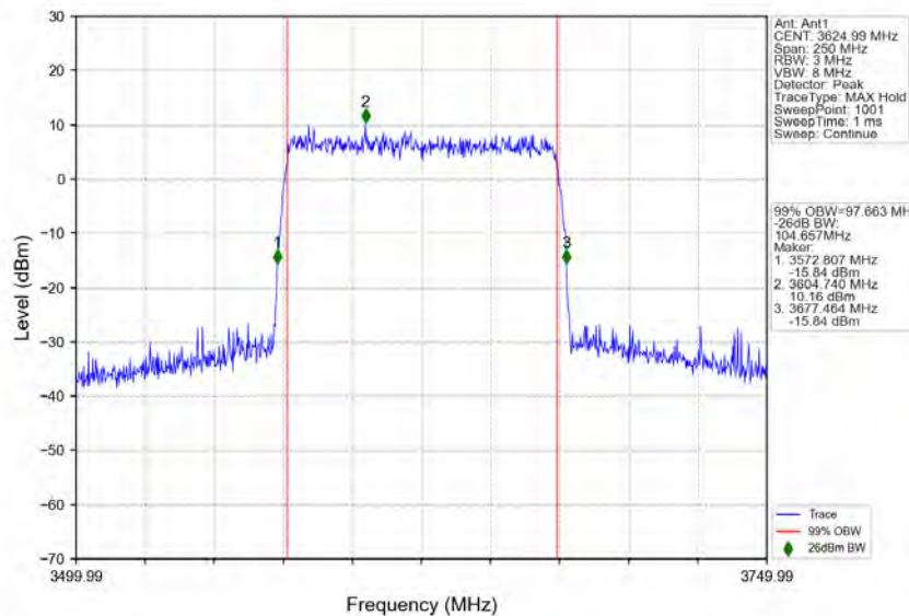
n78d_30kHz_MIMO_NTNV_100MHz_CP-OFDM_256_QAM_3624.99MHz_Outer_Full
