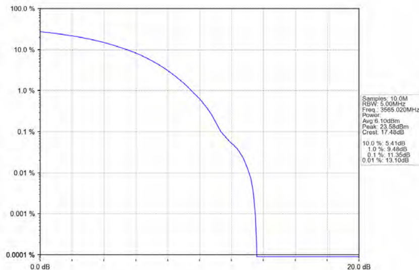
n78d_30kHz_MIMO_NTNV_30MHz_CP-OFDM 64 QAM_3565.02MHz_Outer_Full
