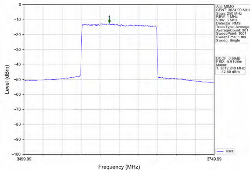
n78d_30kHz_MIMO_NTNV_100MHz_CP-OFDM_16_QAM_3624.99MHz_Inner_Full
