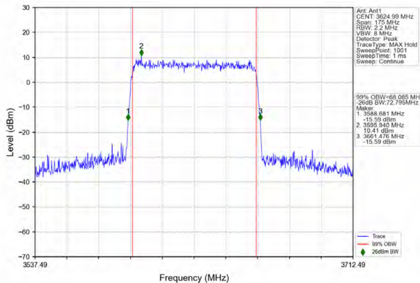
n78d_30kHz_MIMO_NTNV_70MHz_CP-OFDM_256_QAM_3624.99MHz_Outer_Full
