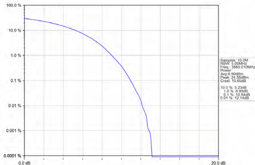
n78d_30kHz_MIMO_NTNV_20MHz_CP-OFDM_16_QAM_3560.01MHz_Outer_Full
