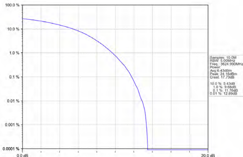
n78d_30kHz_MIMO_NTNV_30MHz_CP-OFDM QPSK_3624.99MHz_Outer_Full
