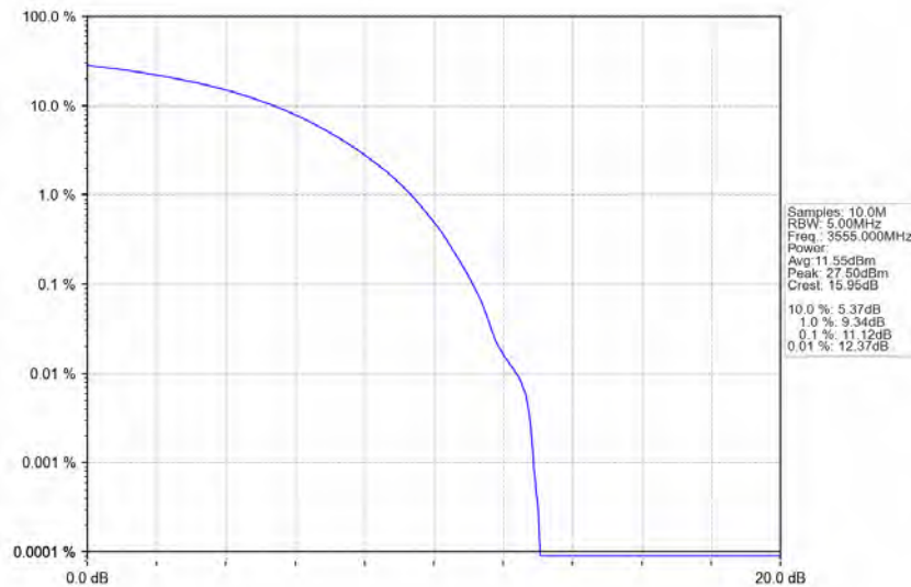
n78d_30kHz_MIMO_NTNV_10MHz_CP-OFDM_16_QAM_3555MHz_Outer_Full
