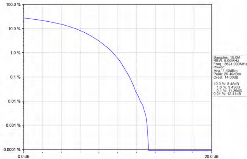
n78d_30kHz_MIMO_NTNV_10MHz_CP-OFDM_16_QAM_3624.99MHz_Outer_Full
