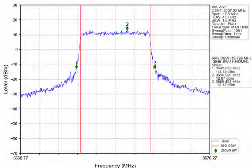
n78d_30kHz_MIMO_NTNV_15MHz_CP-OFDM_64_QAM_3557.52MHz_Outer_Full
