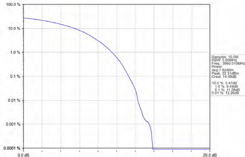
n78d_30kHz_MIMO_NTNV_20MHz_CP-OFDM_64_QAM_3560.01MHz_Outer_Full
