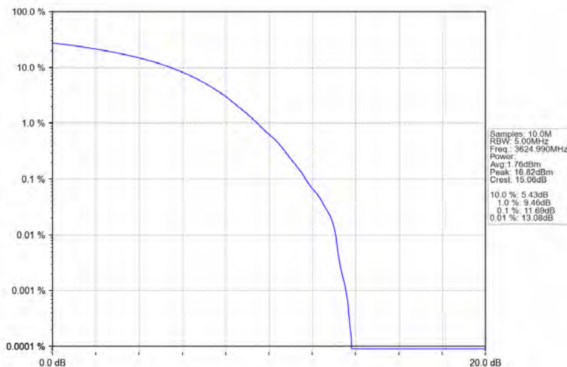
n78d_30kHz_MIMO_NTNV_40MHz_CP-OFDM_256_QAM_3624.99MHz_Outer_Full
