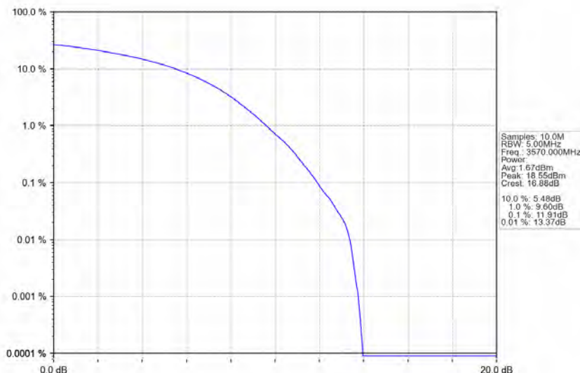
n78d_30kHz_MIMO_NTNV_40MHz_CP-OFDM_256_QAM_3570MHz_Outer_Full
