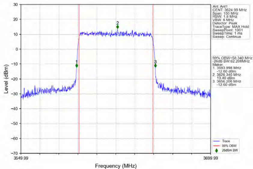
n78d_30kHz_MIMO_NTNV_60MHz_CP-OFDM_16_QAM_3624.99MHz_Outer_Full
