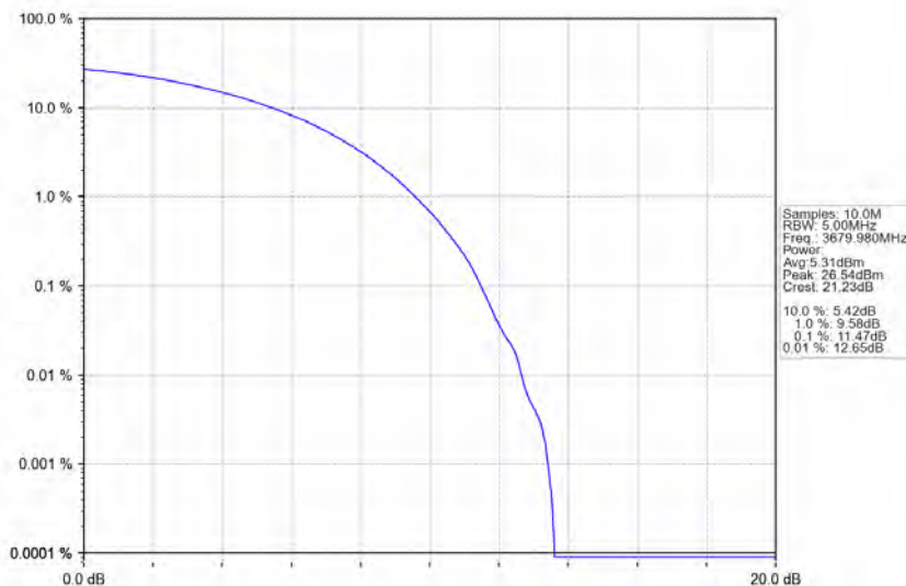
n78d_30kHz_MIMO_NTNV_40MHz_CP-OFDM QPSK_3679.98MHz_Outer_Full
