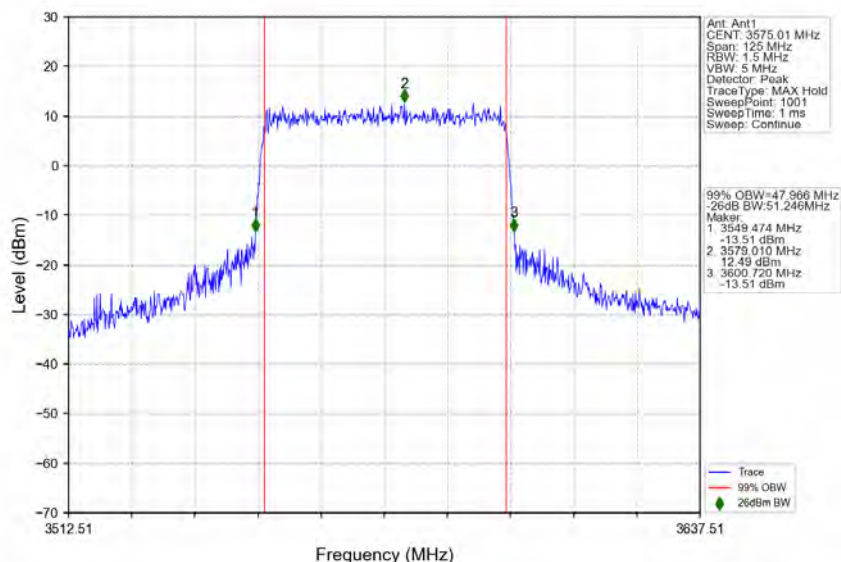
n78d_30kHz_MIMO_NTNV_50MHz_CP-OFDM_64_QAM_3575.01MHz_Outer_Full
