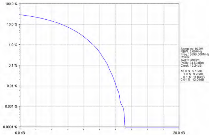
n78d_30kHz_MIMO_NTNV_20MHz_CP-OFDM QPSK_3690MHz_Outer_Full
