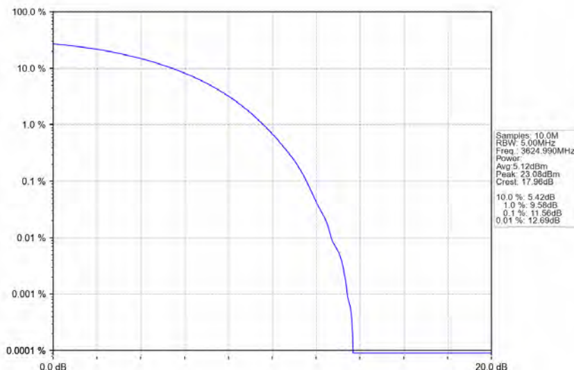
n78d_30kHz_MIMO_NTNV_40MHz_CP-OFDM QPSK_3624.99MHz_Outer_Full
