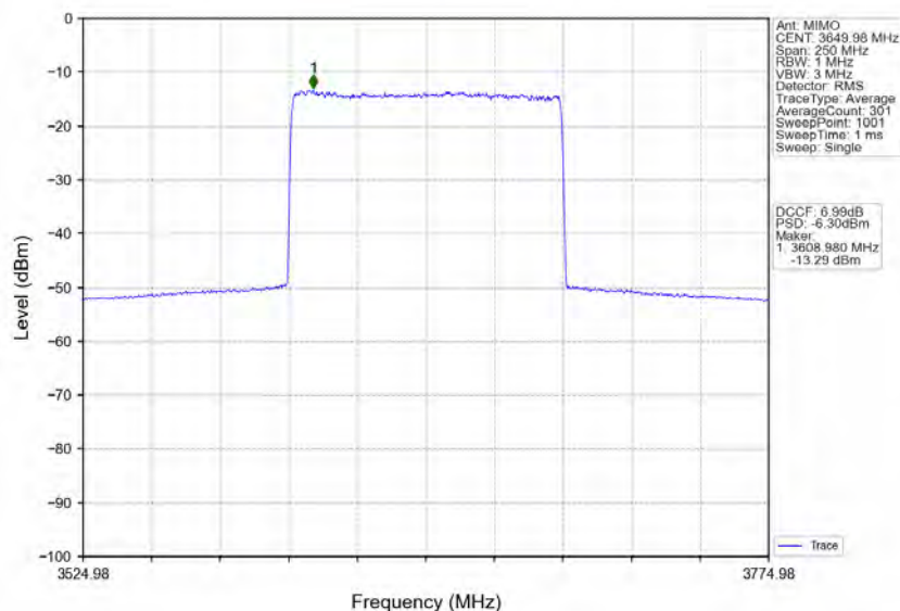
n78d_30kHz_MIMO_NTNV_100MHz_CP-OFDM_16_QAM_3649.98MHz_Inner_Full
