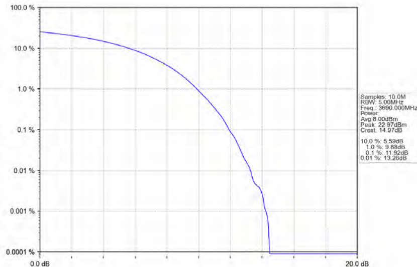
n78d_30kHz_MIMO_NTNV_20MHz_CP-OFDM_16_QAM_3690MHz_Outer_Full
