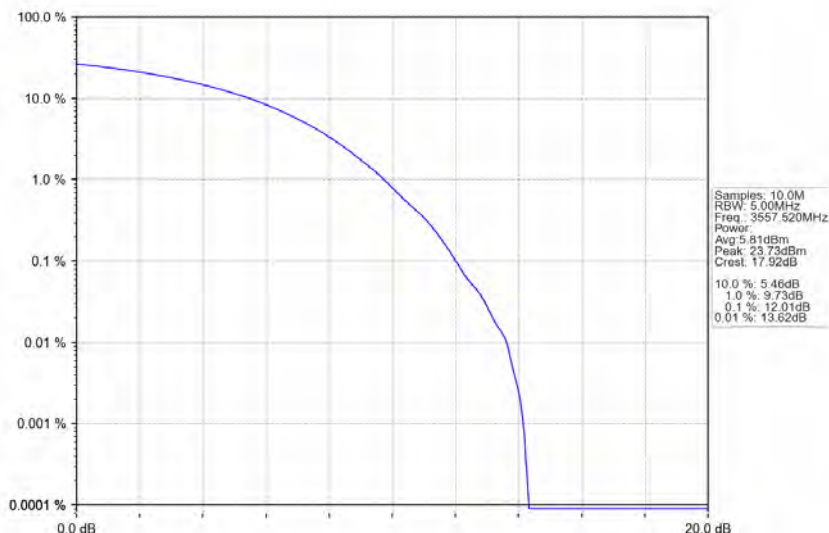
n78d_30kHz_MIMO_NTNV_15MHz_CP-OFDM_256_QAM_3557.52MHz_Outer_Full
