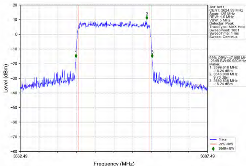
n78d_30kHz_MIMO_NTNV_50MHz_CP-OFDM_256_QAM_3624.99MHz_Outer_Full
