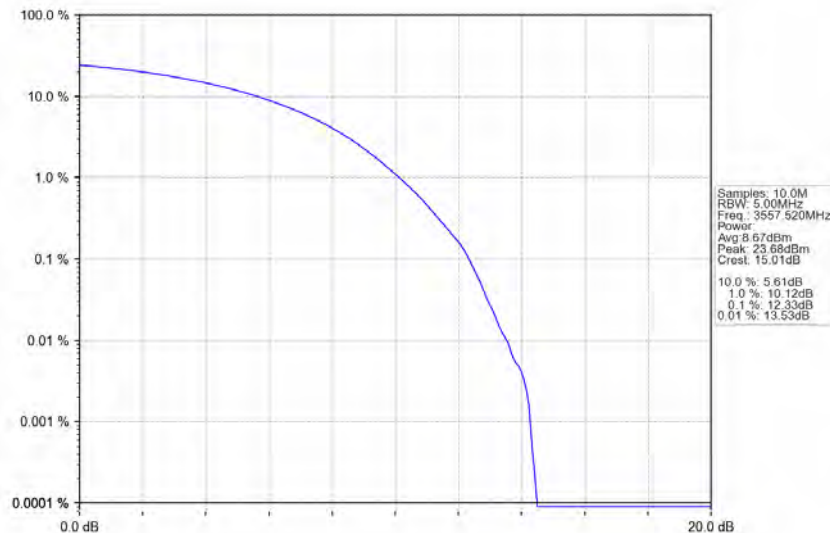
n78d_30kHz_MIMO_NTNV_15MHz_CP-OFDM_16_QAM_3557.52MHz_Outer_Full
