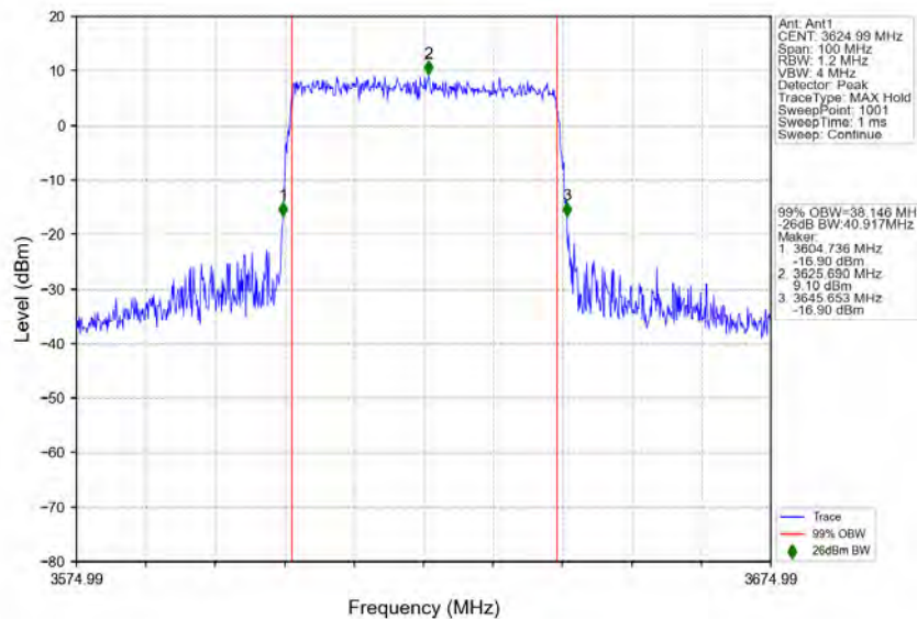
n78d_30kHz_MIMO_NTNV_40MHz_CP-OFDM_256_QAM_3624.99MHz_Outer_Full
