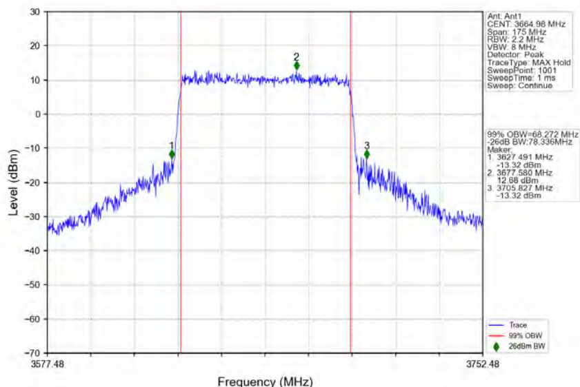
n78d_30kHz_MIMO_NTNV_70MHz_CP-OFDM_64_QAM_3664.98MHz_Outer_Full
