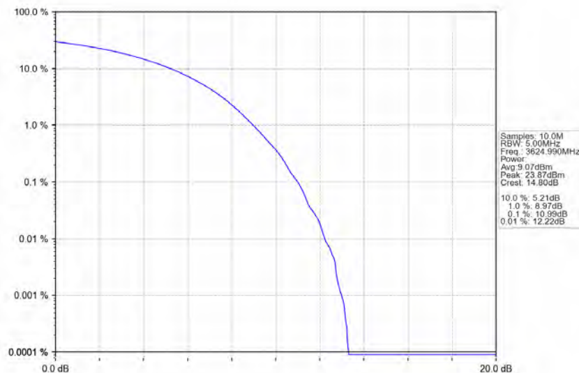
n78d_30kHz_MIMO_NTNV_20MHz_CP-OFDM_16_QAM_3624.99MHz_Outer_Full
