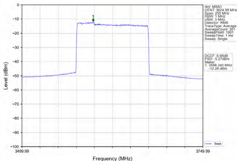
n78d_30kHz_MIMO_NTNV_100MHz_CP-OFDM 64 QAM_3624.99MHz_Inner_Full
