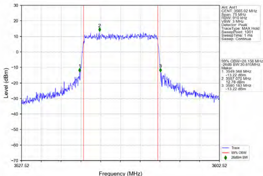
n78d_30kHz_MIMO_NTNV_30MHz_CP-OFDM 64 QAM_3565.02MHz_Outer_Full
