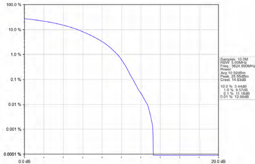
n78d_30kHz_MIMO_NTNV_10MHz_CP-OFDM_64_QAM_3624.99MHz_Outer_Full
