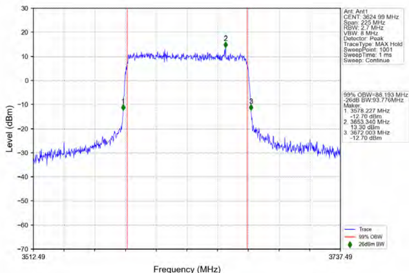
n78d_30kHz_MIMO_NTNV_90MHz_CP-OFDM_16_QAM_3624.99MHz_Outer_Full
