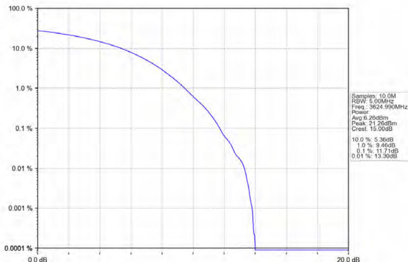
n78d_30kHz_MIMO_NTNV_15MHz_CP-OFDM_256_QAM_3624.99MHz_Outer_Full
