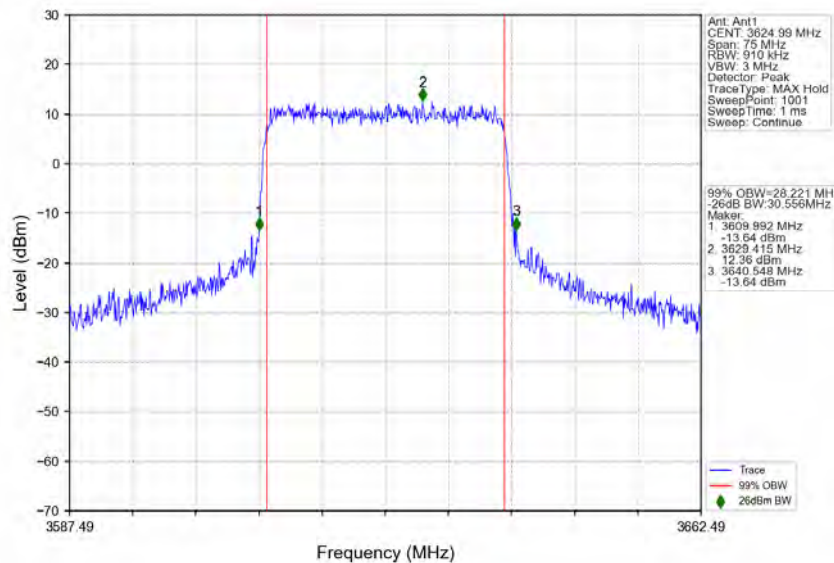
n78d_30kHz_MIMO_NTNV_30MHz_CP-OFDM_16_QAM_3624.99MHz_Outer_Full
