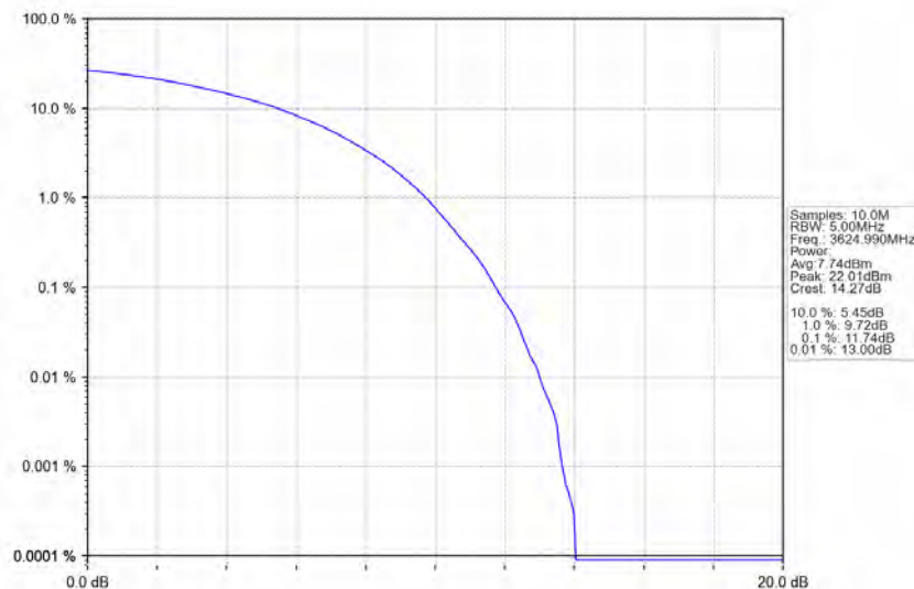
n78d_30kHz_MIMO_NTNV_10MHz_CP-OFDM_256_QAM_3624.99MHz_Outer_Full
