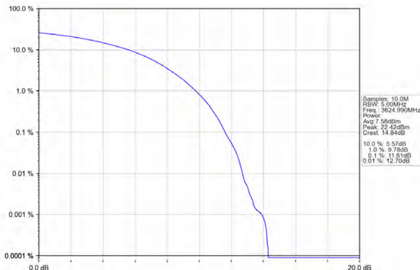
n78d_30kHz_MIMO_NTNV_20MHz_CP-OFDM 64 QAM_3624.99MHz_Outer_Full
