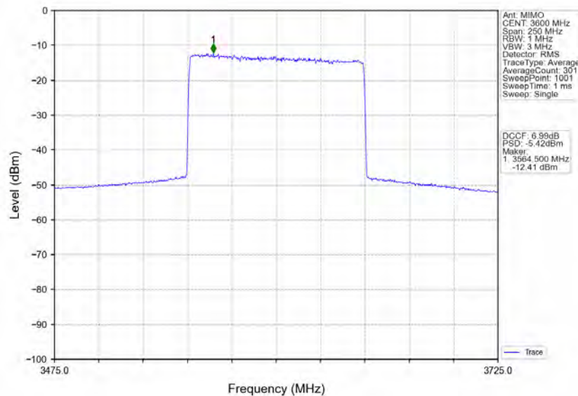
n78d_30kHz_MIMO_NTNV_100MHz_CP-OFDM 64 QAM_3600MHz_Inner_Full
