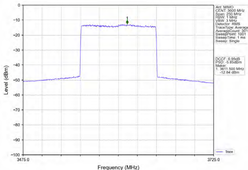
n78d_30kHz_MIMO_NTNV_100MHz_CP-OFDM_256_QAM_3600MHz_Inner_Full
