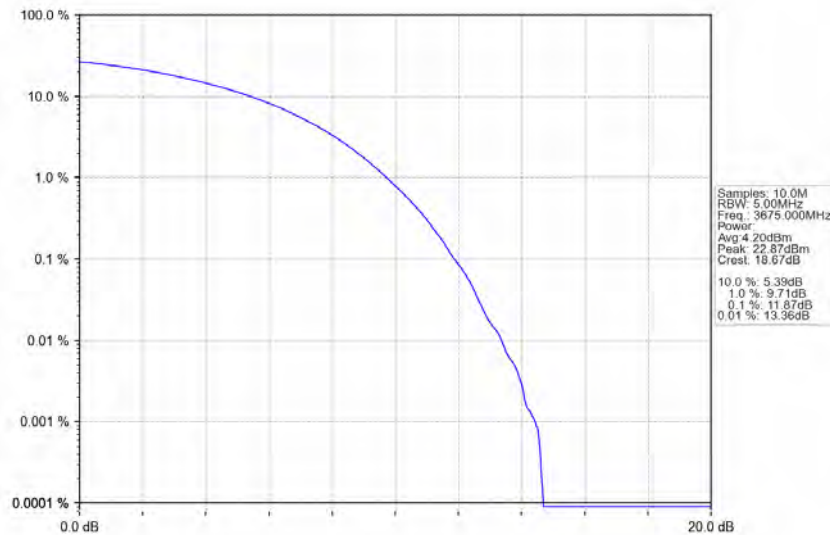
n78d_30kHz_MIMO_NTNV_50MHz_CP-OFDM QPSK_3675MHz_Outer_Full
