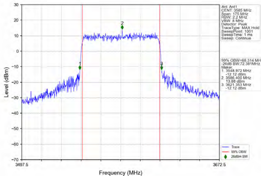
n78d_30kHz_MIMO_NTNV_70MHz_CP-OFDM 64 QAM_3585MHz_Outer_Full
