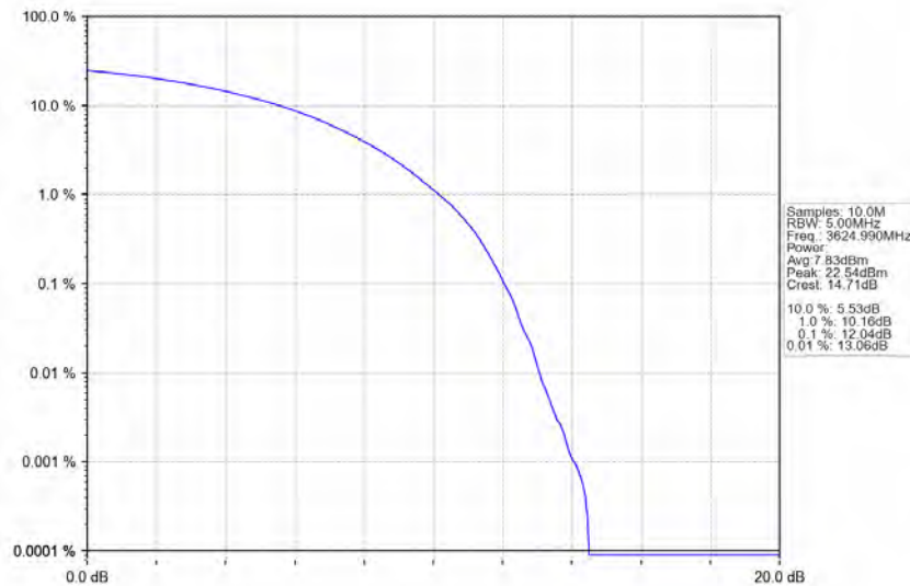
n78d_30kHz_MIMO_NTNV_20MHz_CP-OFDM QPSK_3624.99MHz_Outer_Full
