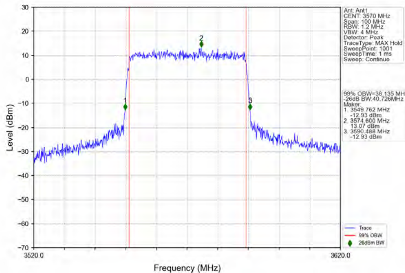
n78d_30kHz_MIMO_NTNV_40MHz_CP-OFDM 64 QAM_3570MHz_Outer_Full
