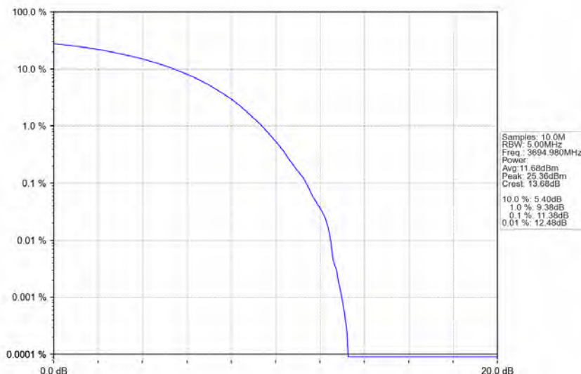
n78d_30kHz_MIMO_NTNV_10MHz_CP-OFDM_QPSK_3694.98MHz_Outer_Full
