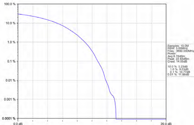
n78d_30kHz_MIMO_NTNV_20MHz_CP-OFDM 64 QAM_3690MHz_Outer_Full
