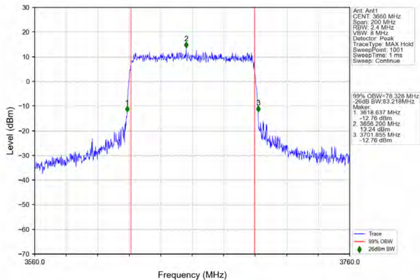
n78d_30kHz_MIMO_NTNV_80MHz_CP-OFDM_64_QAM_3660MHz_Outer_Full
