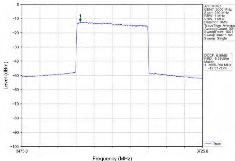
n78d_30kHz_MIMO_NTNV_100MHz_CP-OFDM_16_QAM_3600MHz_Inner_Full
