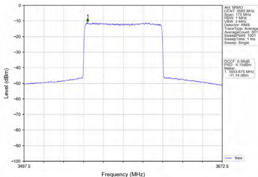
n78d_30kHz_MIMO_NTNV_70MHz_CP-OFDM_256_QAM_3585MHz_Inner_Full
