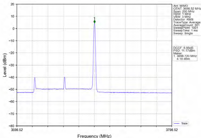
n78d_30kHz_MIMO_NTNV_80MHz_CP-OFDM QPSK_3660MHz_Inner_1RB_Right
