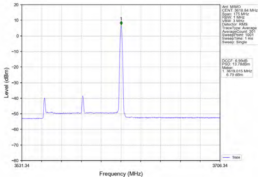
n78d_30kHz_MIMO_NTNV_70MHz_CP-OFDM 64 QAM_3585MHz_Edge_1RB_Right
