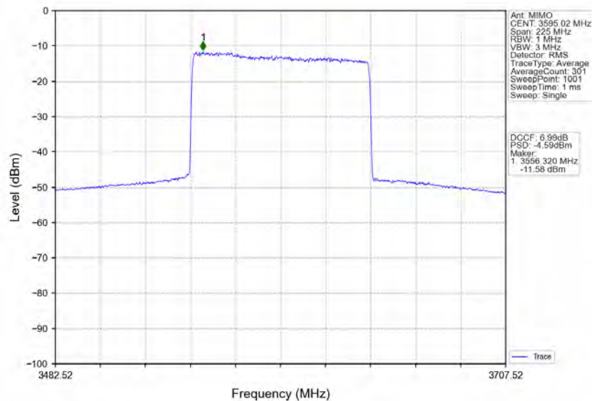
n78d_30kHz_MIMO_NTNV_90MHz_CP-OFDM 64 QAM_3595.02MHz_Inner_Full
