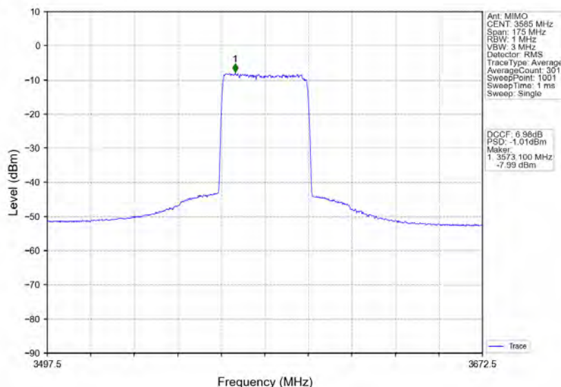
n78d_30kHz_MIMO_NTNV_70MHz_CP-OFDM_256_QAM_3585MHz_Inner_Full
