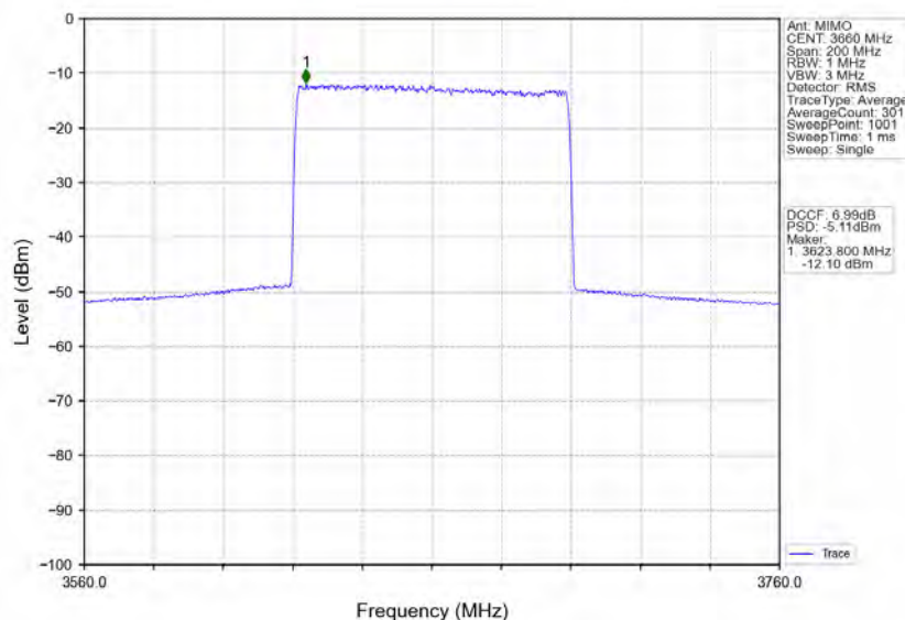
n78d_30kHz_MIMO_NTNV_80MHz_CP-OFDM_256_QAM_3660MHz_Inner_Full
