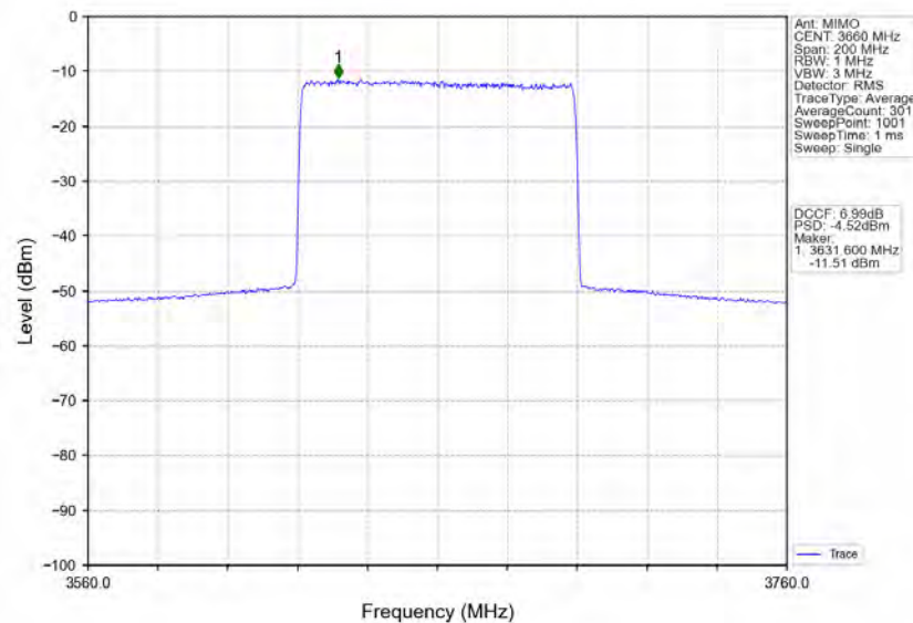
n78d_30kHz_MIMO_NTNV_80MHz_CP-OFDM_QPSK_3660MHz_Inner_Full
