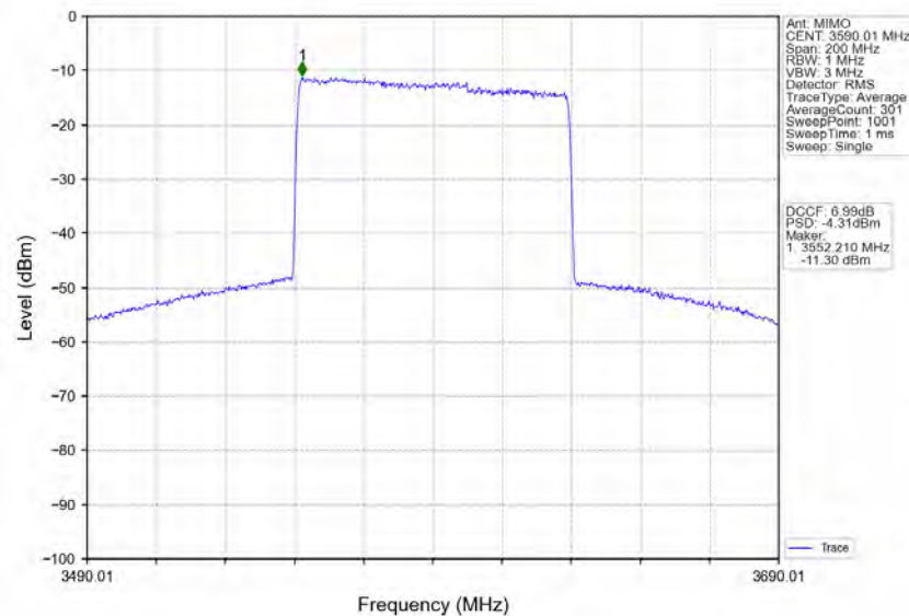
n78d_30kHz_MIMO_NTNV_80MHz_CP-OFDM_256_QAM_3590.01MHz_Inner_Full
