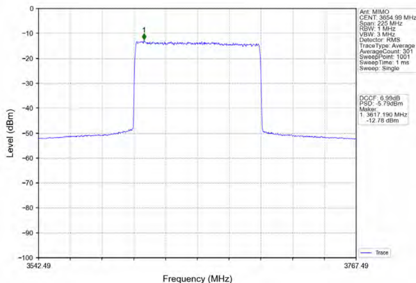
n78d_30kHz_MIMO_NTNV_90MHz_CP-OFDM QPSK_3654.99MHz_Inner_Full
