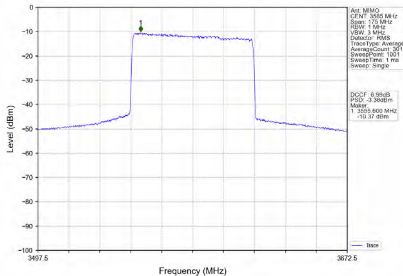
n78d_30kHz_MIMO_NTNV_70MHz_CP-OFDM_16_QAM_3585MHz_Inner_Full
