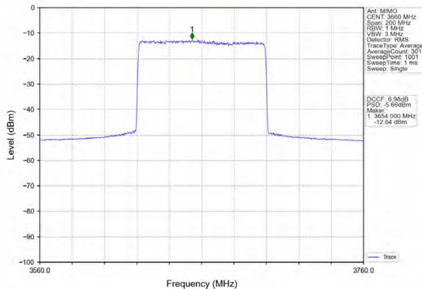
n78d_30kHz_MIMO_NTNV_80MHz_CP-OFDM_64_QAM_3660MHz_Inner_Full
