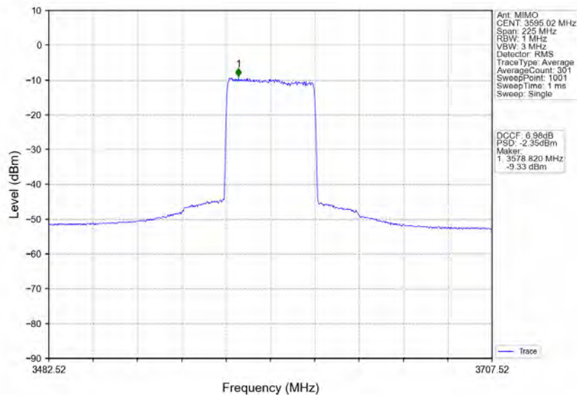
n78d_30kHz_MIMO_NTNV_90MHz_CP-OFDM_256_QAM_3595.02MHz_Inner_Full
