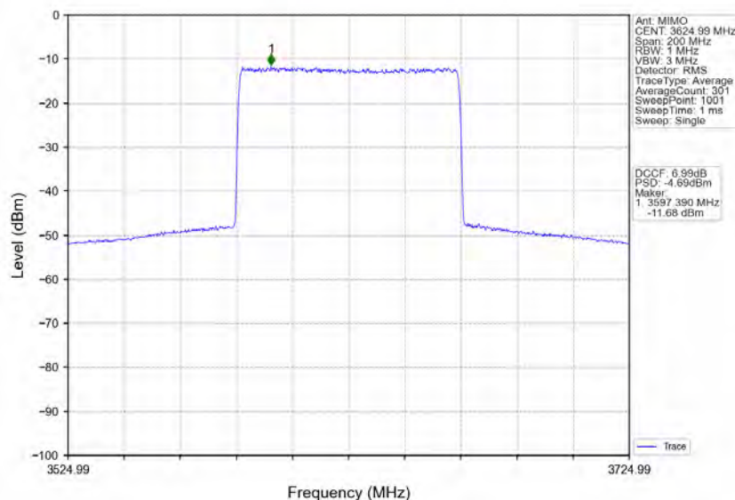
n78d_30kHz_MIMO_NTNV_80MHz_CP-OFDM_256_QAM_3624.99MHz_Inner_Full
