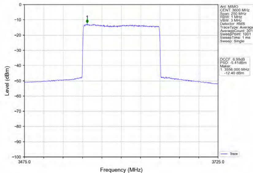
n78d_30kHz_MIMO_NTNV_100MHz_CP-OFDM_QPSK_3600MHz_Inner_Full
