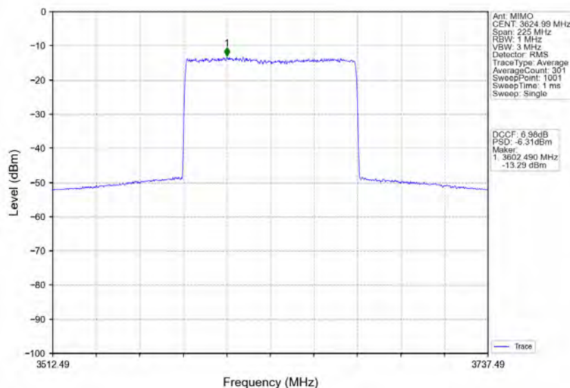
n78d_30kHz_MIMO_NTNV_90MHz_CP-OFDM_256_QAM_3624.99MHz_Inner_Full
