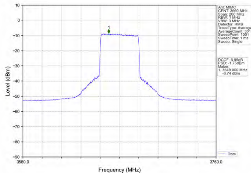
n78d_30kHz_MIMO_NTNV_80MHz_CP-OFDM_QPSK_3660MHz_Inner_Full
