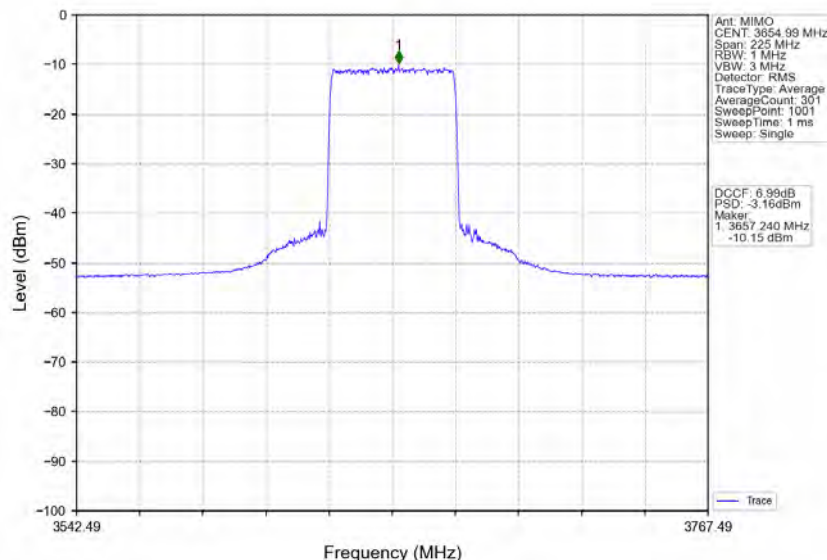
n78d_30kHz_MIMO_NTNV_90MHz_CP-OFDM_16_QAM_3654.99MHz_Inner_Full
