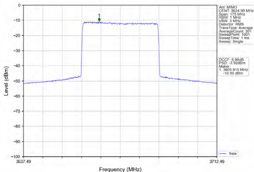
n78d_30kHz_MIMO_NTNV_70MHz_CP-OFDM_16_QAM_3624.99MHz_Inner_Full
