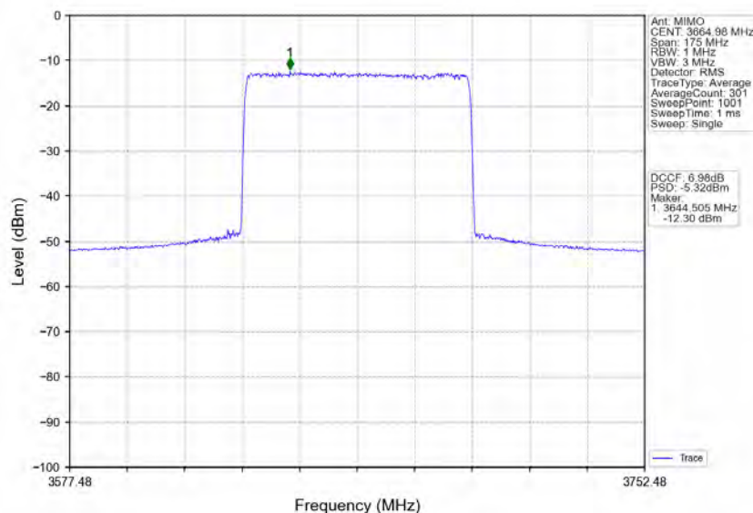
n78d_30kHz_MIMO_NTNV_70MHz_CP-OFDM_16_QAM_3664.98MHz_Inner_Full
