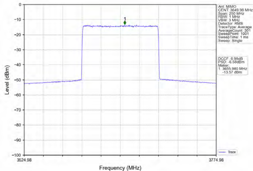
n78d_30kHz_MIMO_NTNV_100MHz_CP-OFDM QPSK_3649.98MHz_Inner_Full
