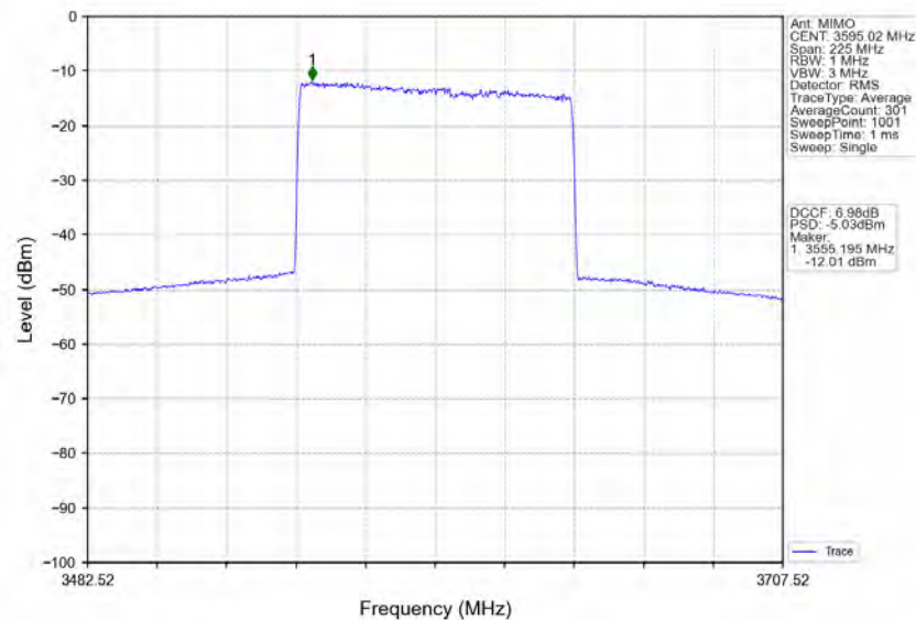
n78d_30kHz_MIMO_NTNV_90MHz_CP-OFDM_256_QAM_3595.02MHz_Inner_Full
