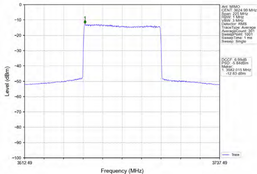
n78d_30kHz_MIMO_NTNV_90MHz_CP-OFDM_16_QAM_3624.99MHz_Inner_Full
