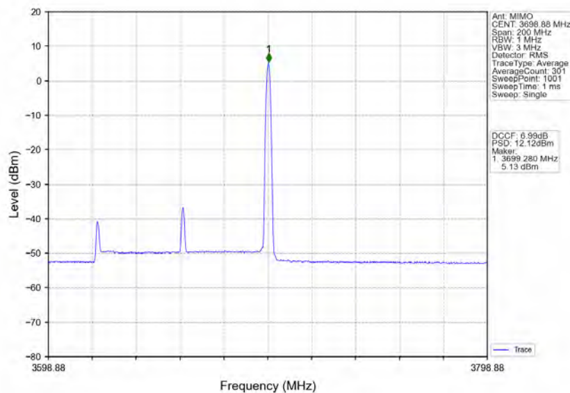
n78d_30kHz_MIMO_NTNV_80MHz_CP-OFDM QPSK_3660MHz_Edge_1RB_Right
