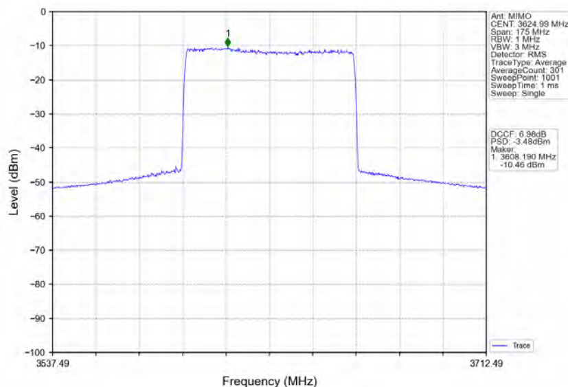
n78d_30kHz_MIMO_NTNV_70MHz_CP-OFDM 64 QAM_3624.99MHz_Inner_Full
