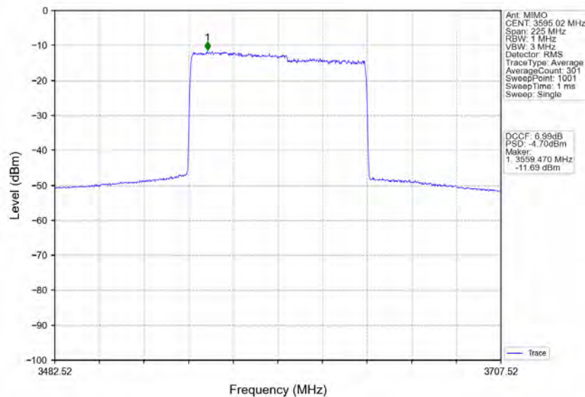
n78d_30kHz_MIMO_NTNV_90MHz_CP-OFDM QPSK_3595.02MHz_Inner_Full
