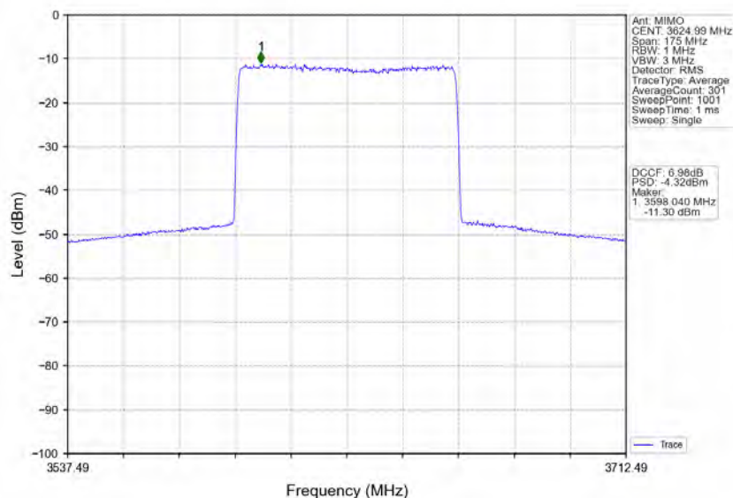
n78d_30kHz_MIMO_NTNV_70MHz_CP-OFDM_256_QAM_3624.99MHz_Inner_Full
