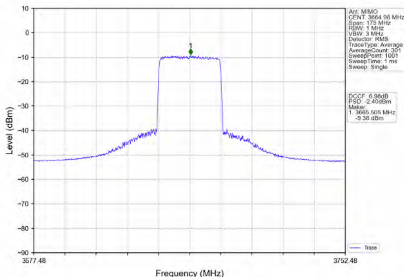
n78d_30kHz_MIMO_NTNV_70MHz_CP-OFDM_16_QAM_3664.98MHz_Inner_Full
