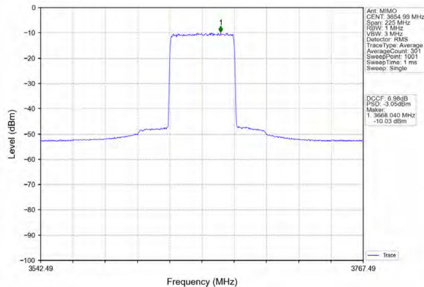
n78d_30kHz_MIMO_NTNV_90MHz_CP-OFDM_256_QAM_3654.99MHz_Inner_Full
