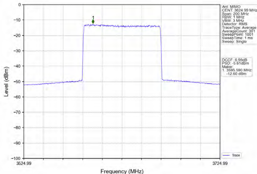
n78d_30kHz_MIMO_NTNV_80MHz_CP-OFDM QPSK_3624.99MHz_Inner_Full
