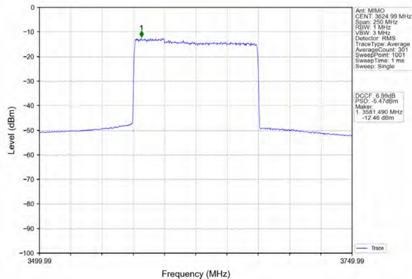
n78d_30kHz_MIMO_NTNV_100MHz_CP-OFDM_QPSK_3624.99MHz_Inner_Full
