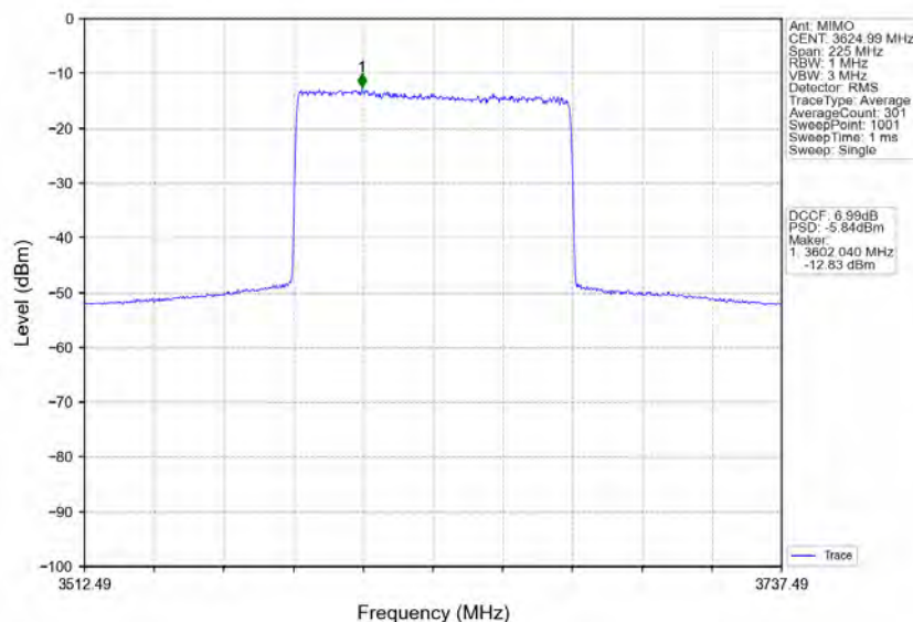
n78d_30kHz_MIMO_NTNV_90MHz_CP-OFDM 64 QAM_3624.99MHz_Inner_Full
