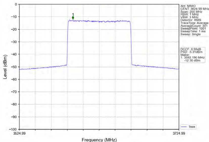
n78d_30kHz_MIMO_NTNV_80MHz_CP-OFDM_16_QAM_3624.99MHz_Inner_Full
