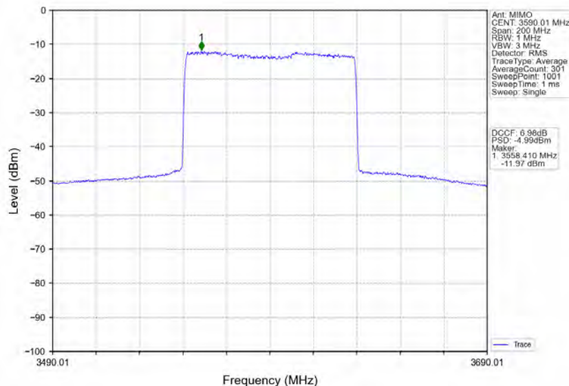
n78d_30kHz_MIMO_NTNV_80MHz_CP-OFDM_QPSK_3590.01MHz_Inner_Full
