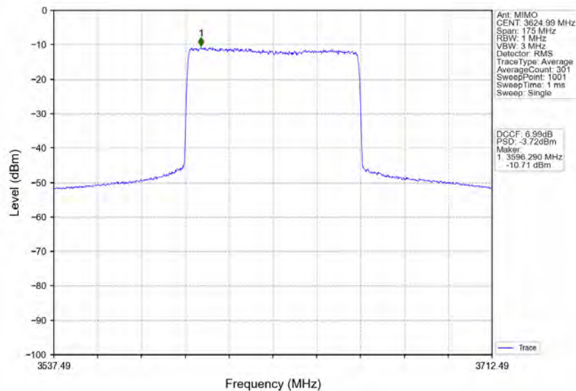
n78d_30kHz_MIMO_NTNV_70MHz_CP-OFDM QPSK_3624.99MHz_Inner_Full
