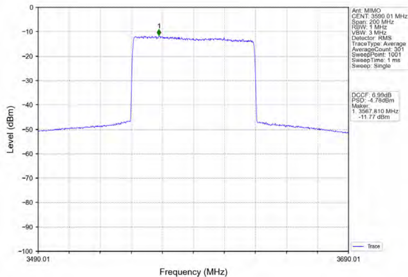
n78d_30kHz_MIMO_NTNV_80MHz_CP-OFDM 64 QAM_3590.01MHz_Inner_Full
