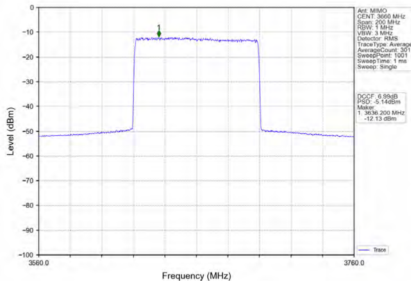
n78d_30kHz_MIMO_NTNV_80MHz_CP-OFDM_16_QAM_3660MHz_Inner_Full
