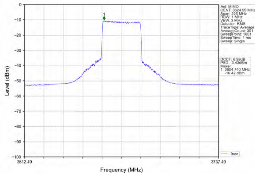
n78d_30kHz_MIMO_NTNV_90MHz_CP-OFDM_QPSK_3624.99MHz_Inner_Full
