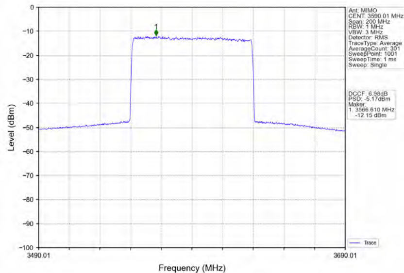
n78d_30kHz_MIMO_NTNV_80MHz_CP-OFDM_16_QAM_3590.01MHz_Inner_Full
