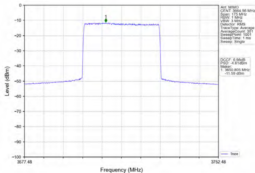
n78d_30kHz_MIMO_NTNV_70MHz_CP-OFDM QPSK_3664.98MHz_Inner_Full
