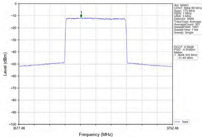
n78d_30kHz_MIMO_NTNV_70MHz_CP-OFDM_256_QAM_3664.98MHz_Inner_Full
