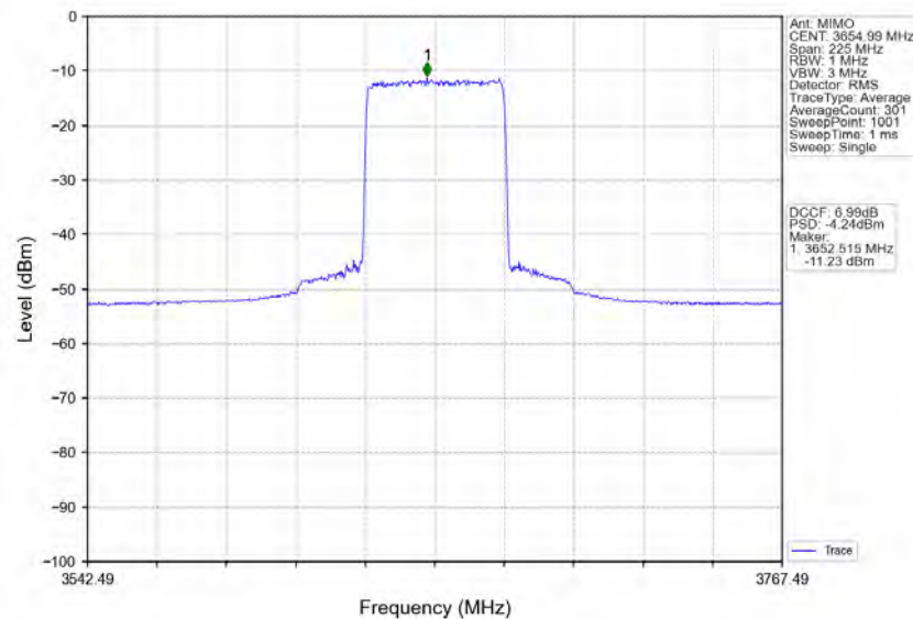
n78d_30kHz_MIMO_NTNV_90MHz_CP-OFDM 64 QAM_3654.99MHz_Inner_Full
