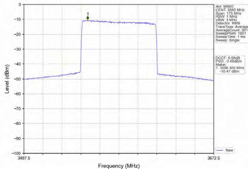
n78d_30kHz_MIMO_NTNV_70MHz_CP-OFDM_64_QAM_3585MHz_Inner_Full
