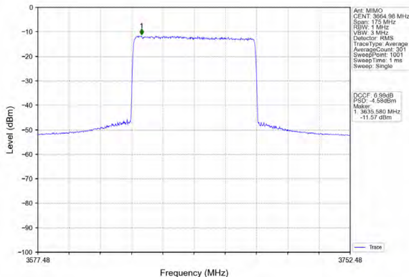
n78d_30kHz_MIMO_NTNV_70MHz_CP-OFDM 64 QAM_3664.98MHz_Inner_Full
