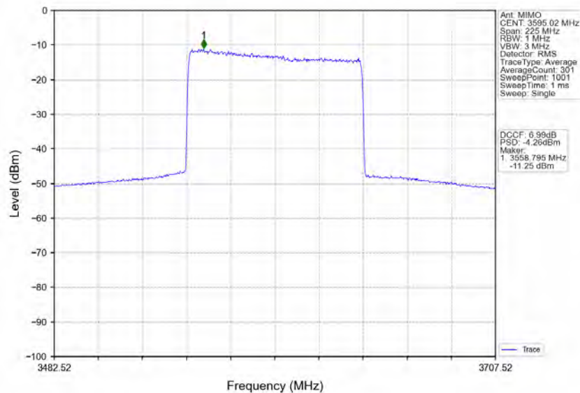
n78d_30kHz_MIMO_NTNV_90MHz_CP-OFDM_16_QAM_3595.02MHz_Inner_Full
