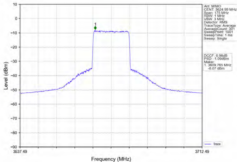
n78d_30kHz_MIMO_NTNV_70MHz_CP-OFDM QPSK_3624.99MHz_Inner_Full
