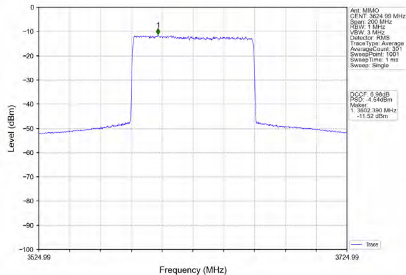
n78d_30kHz_MIMO_NTNV_80MHz_CP-OFDM 64 QAM_3624.99MHz_Inner_Full
