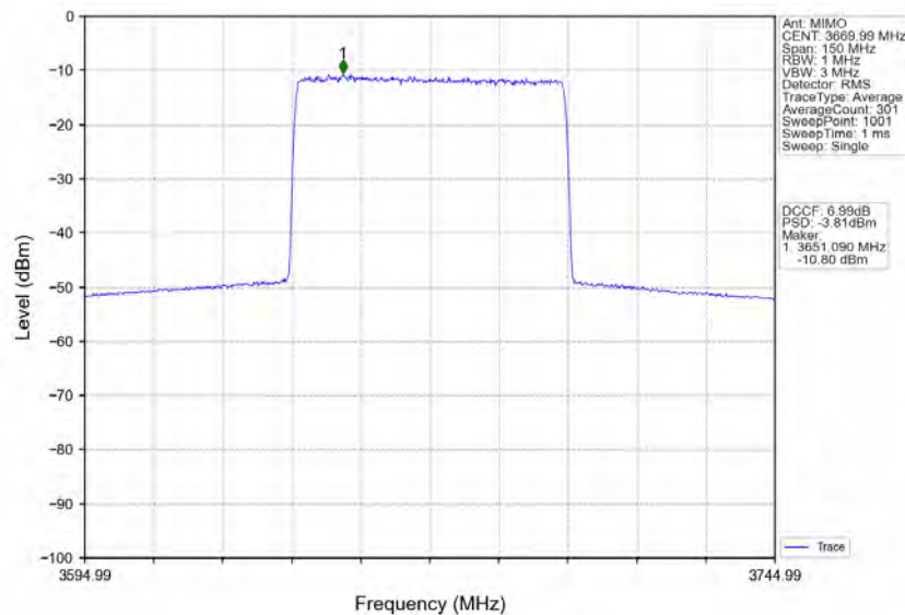
n78d_30kHz_MIMO_NTNV_60MHz_CP-OFDM_256_QAM_3669.99MHz_Inner_Full
