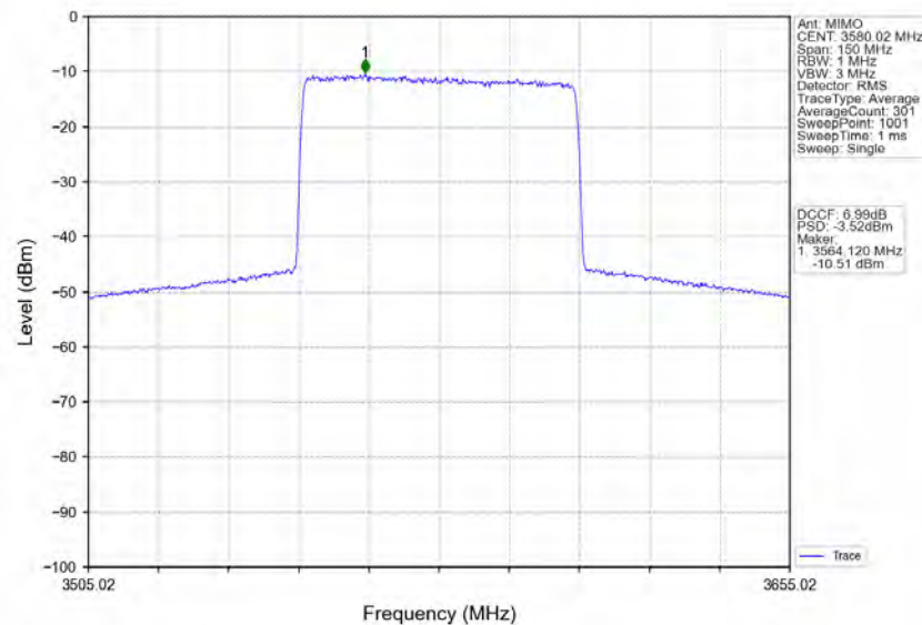
n78d_30kHz_MIMO_NTNV_60MHz_CP-OFDM_256_QAM_3580.02MHz_Inner_Full
