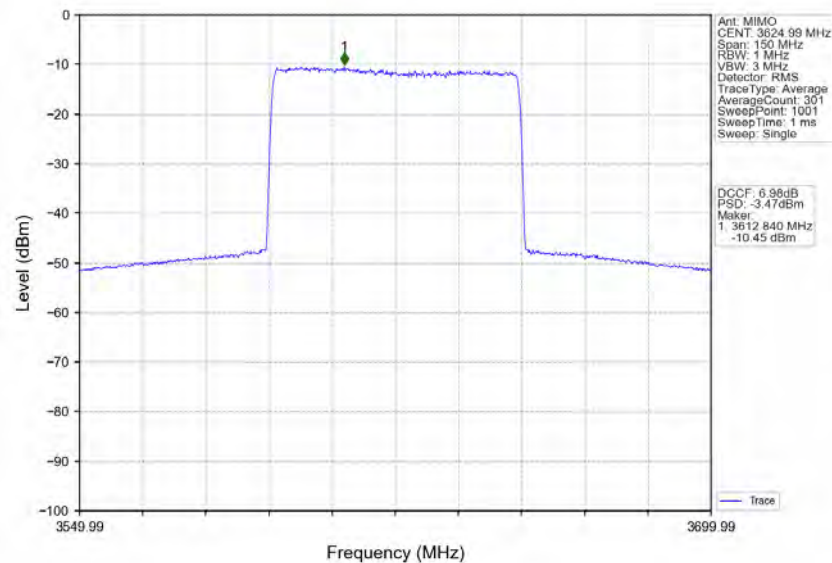
n78d_30kHz_MIMO_NTNV_60MHz_CP-OFDM QPSK_3624.99MHz_Inner_Full
