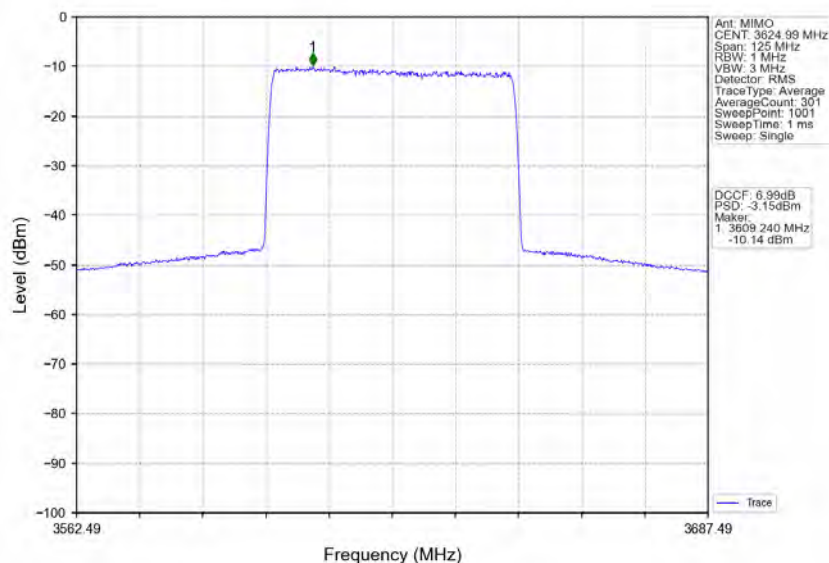
n78d_30kHz_MIMO_NTNV_50MHz_CP-OFDM_256_QAM_3624.99MHz_Inner_Full
